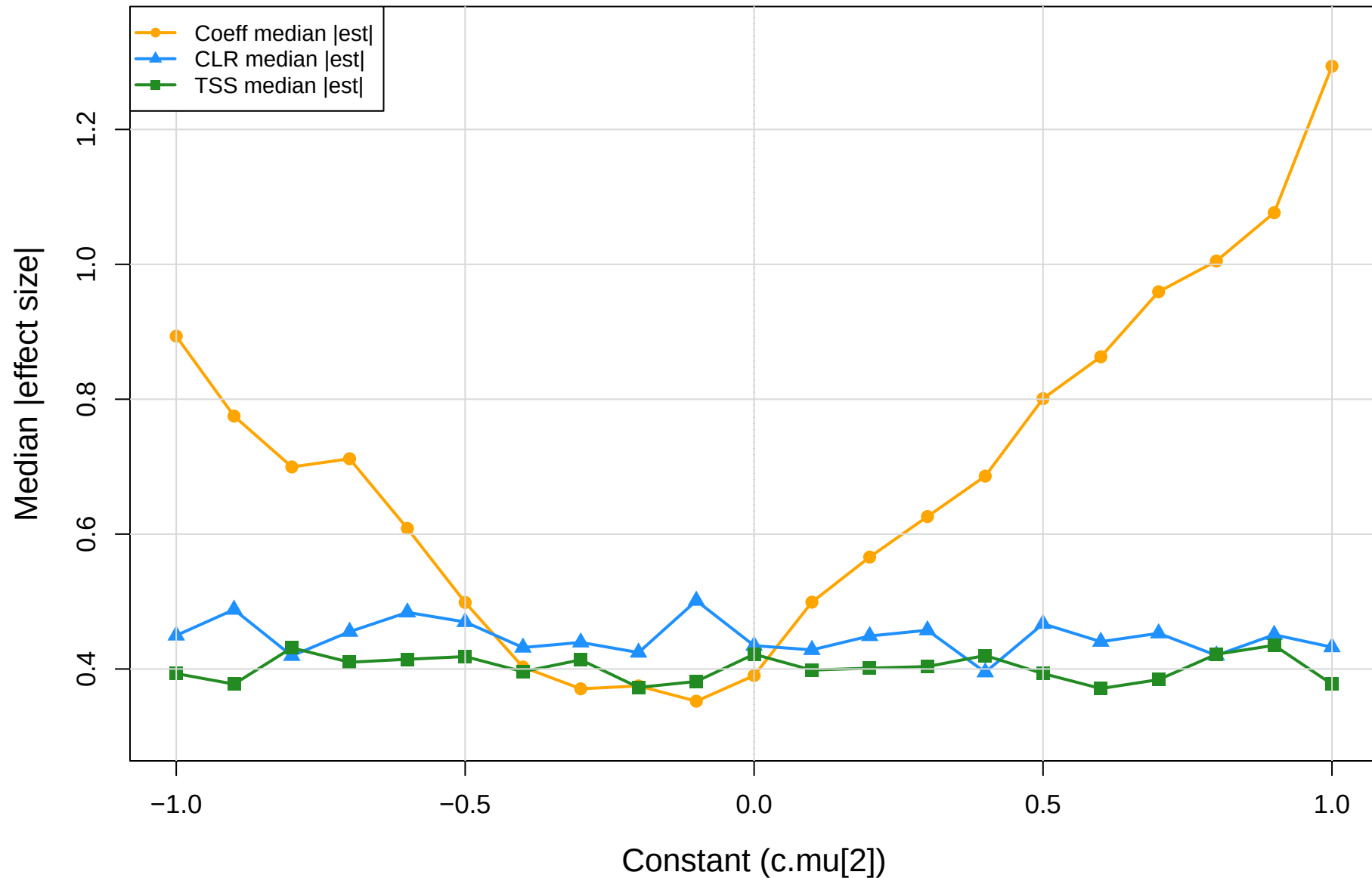
coeff.sm vs CLR vs TSS | mage vs you | gamma=0.3 Median absolute effect size
