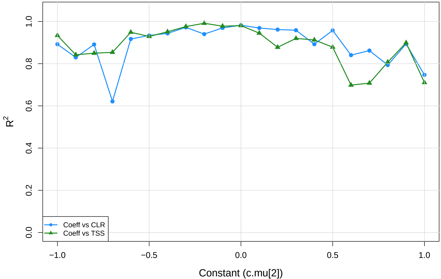
coeff.sm vs CLR vs TSS | mage vs you | gamma=0.3 R-squared of red-dot regression
