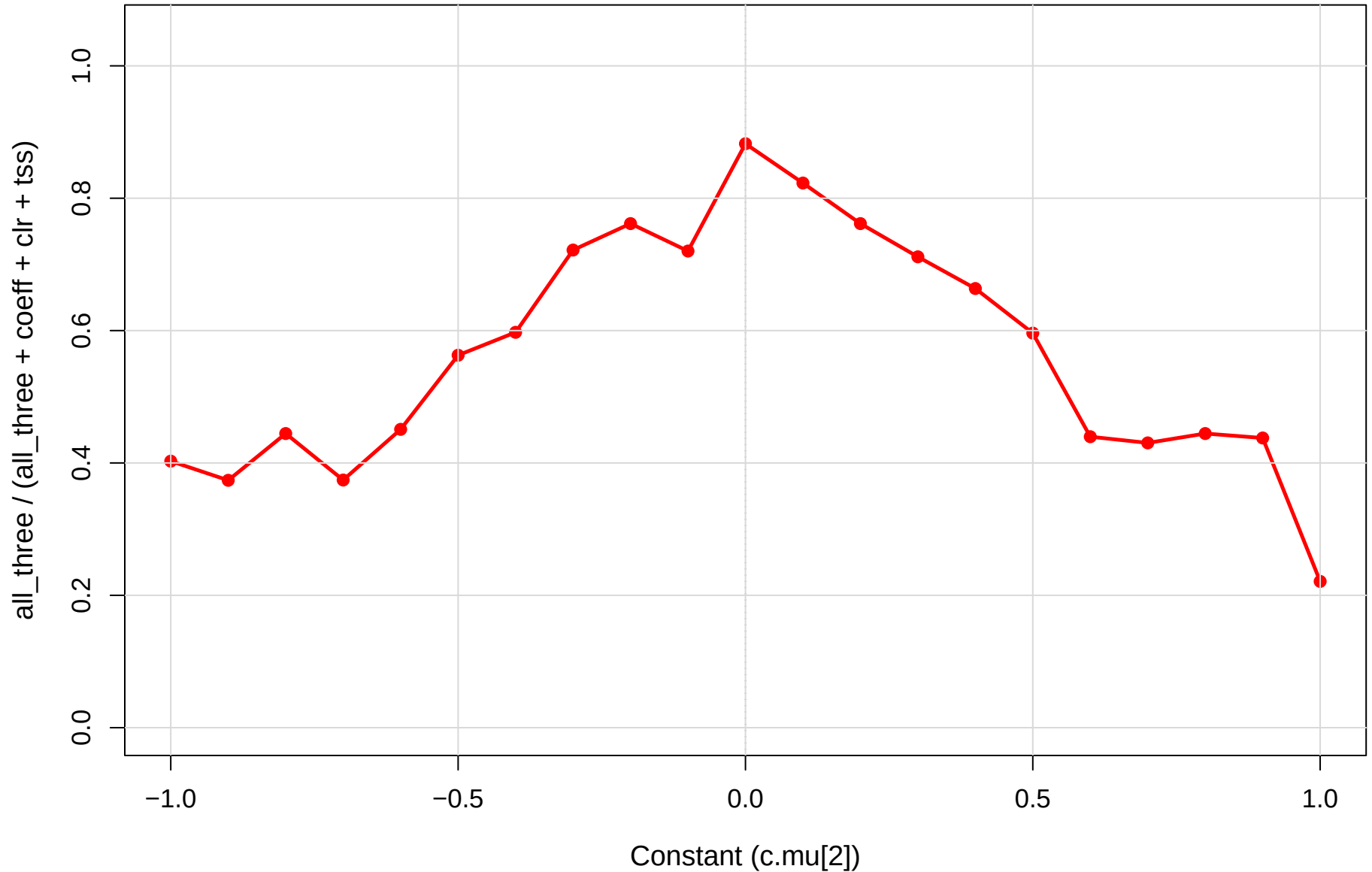
coeff.sm vs CLR vs TSS | mage vs you | gamma=0.3 Robustness (1 = all agree, 0 = max disagreement)
