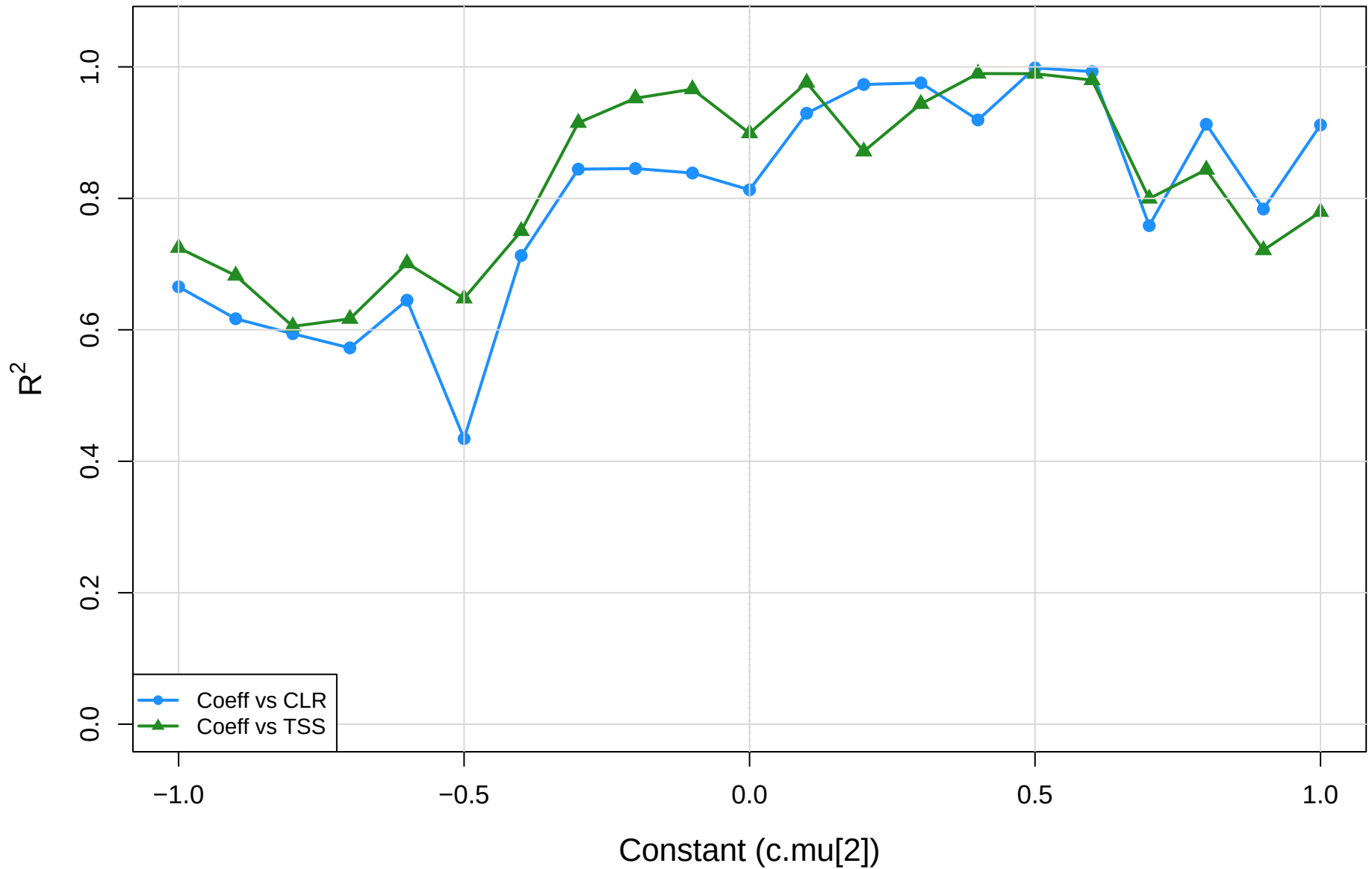
coeff.sm vs CLR vs TSS | mid vs pup | gamma=0.3 R-squared of red-dot regression
