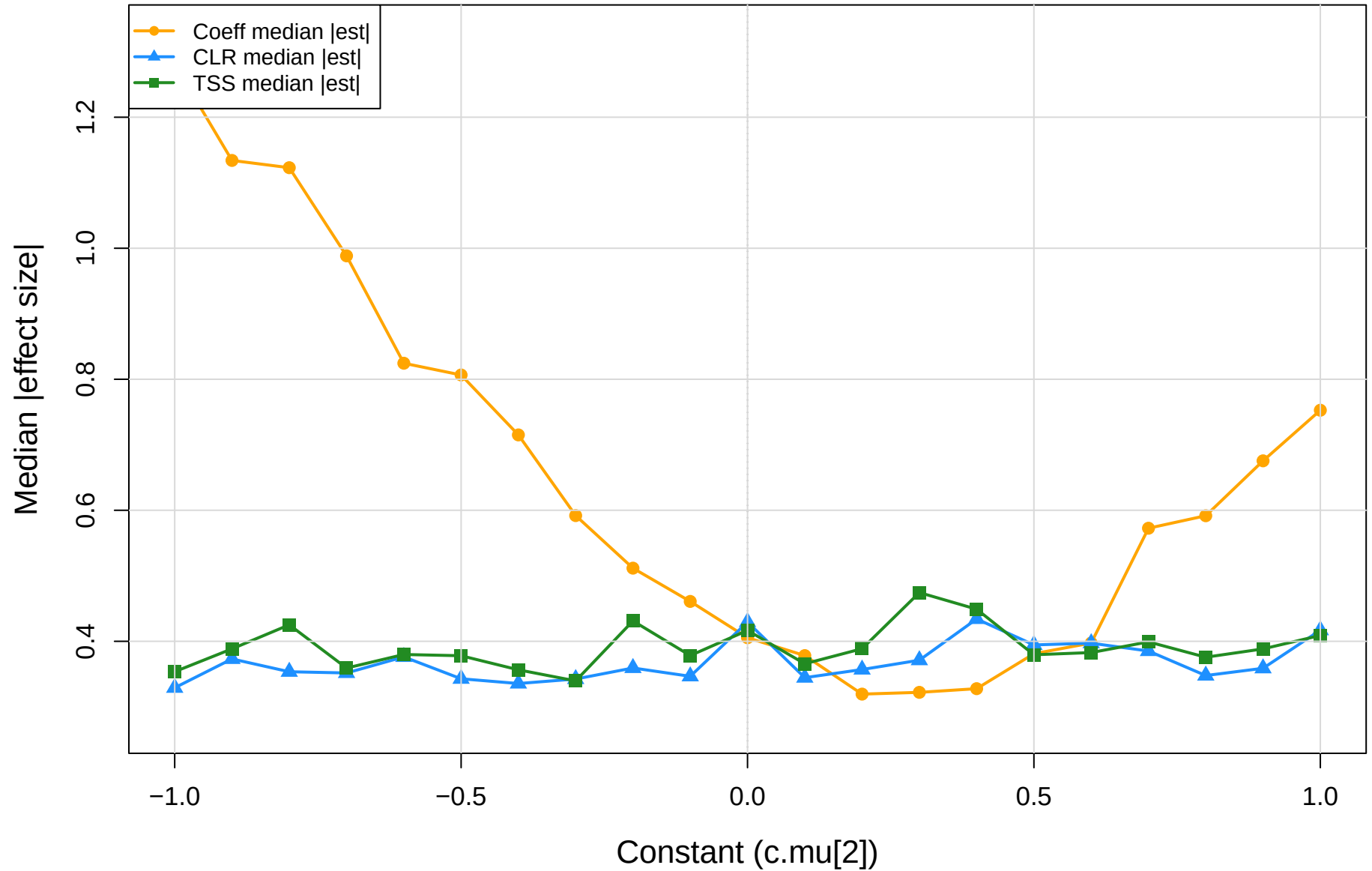
coeff.sm vs CLR vs TSS | mid vs pup | gamma=0.3 Median absolute effect size
