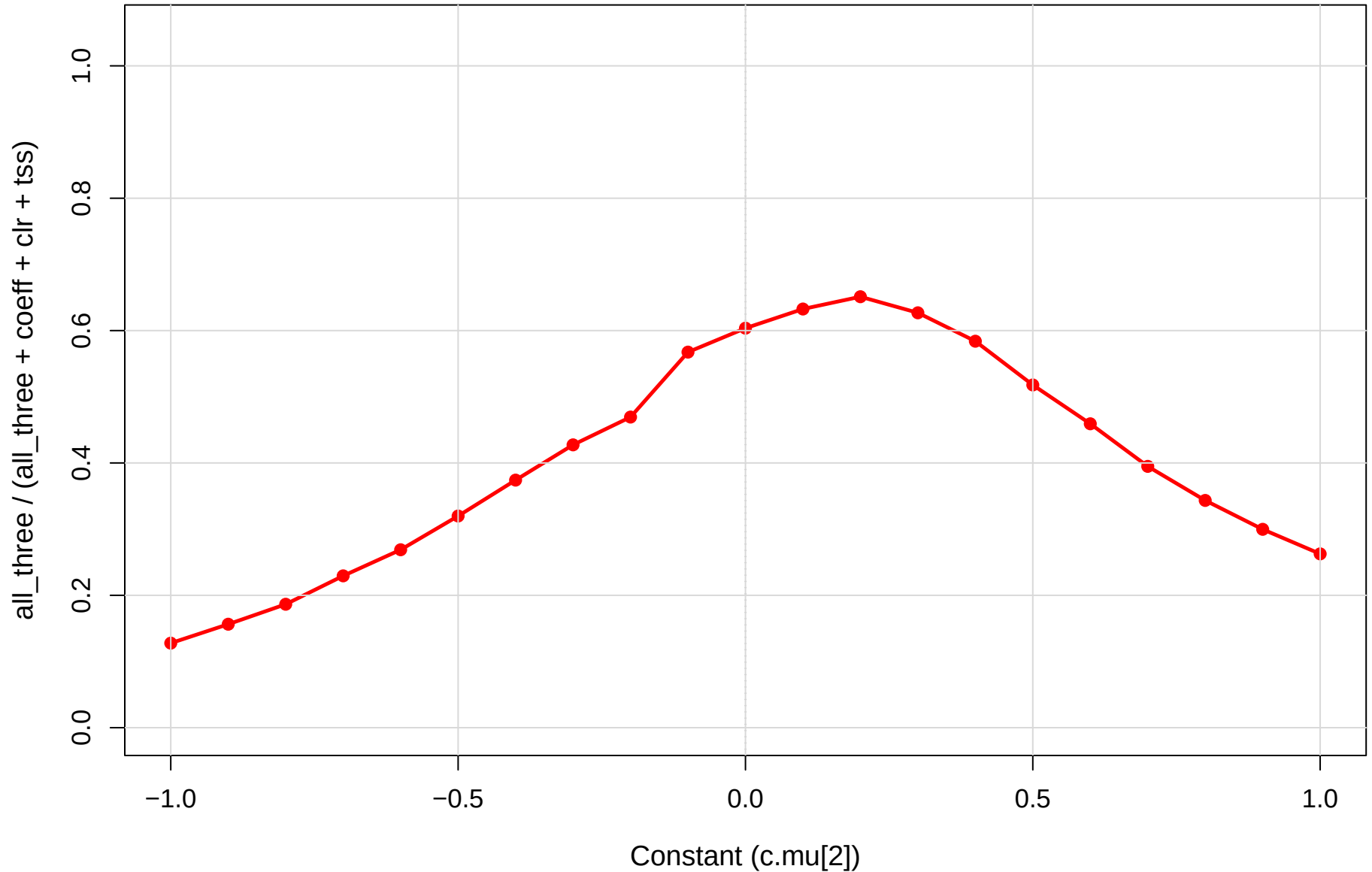
coeff.sm vs CLR vs TSS | cent vs mage | gamma=1e-04 Robustness (1 = all agree, 0 = max disagreement)
