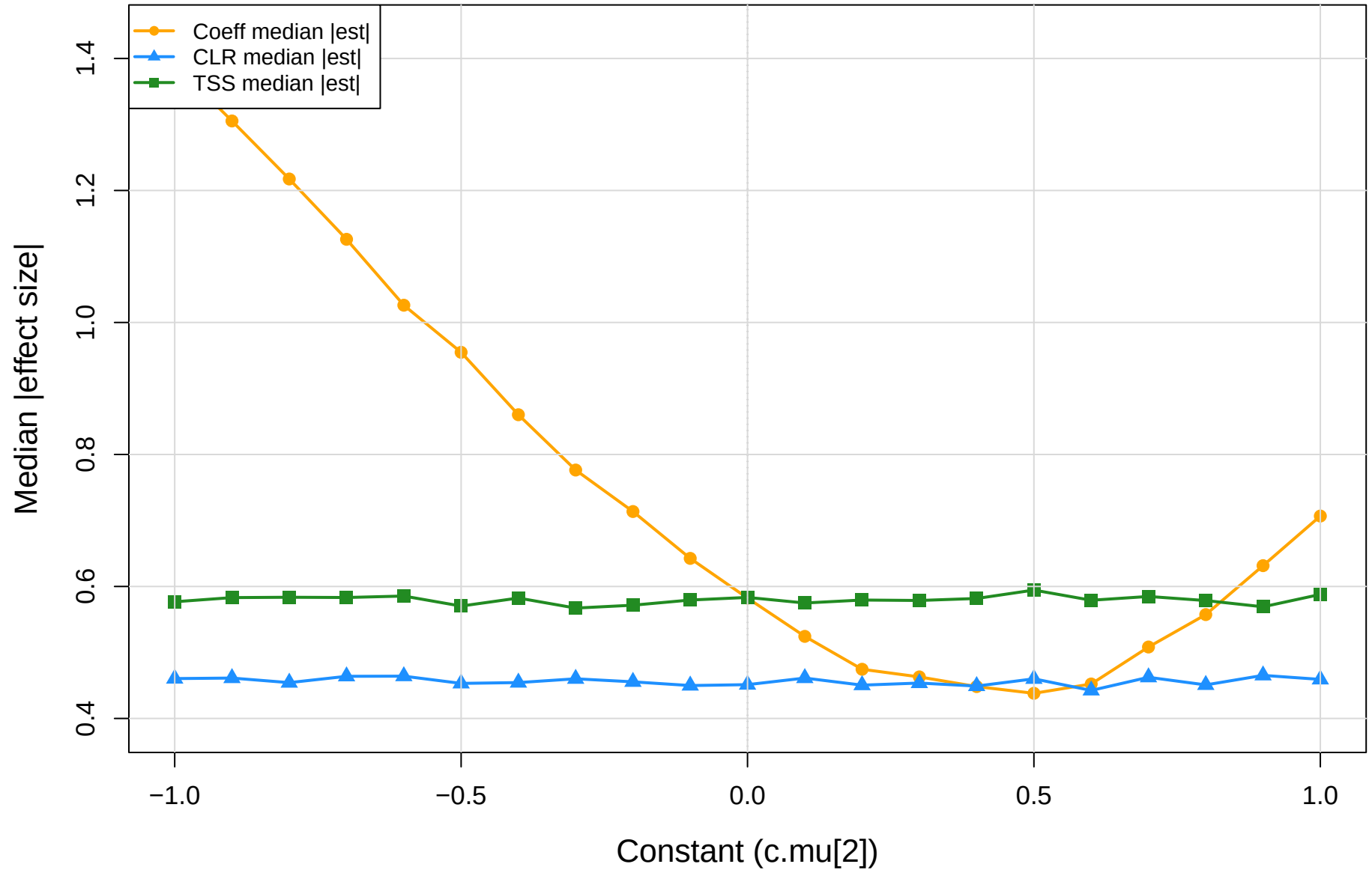
coeff.sm vs CLR vs TSS | cent vs mage | gamma=1e-04 Median absolute effect size
