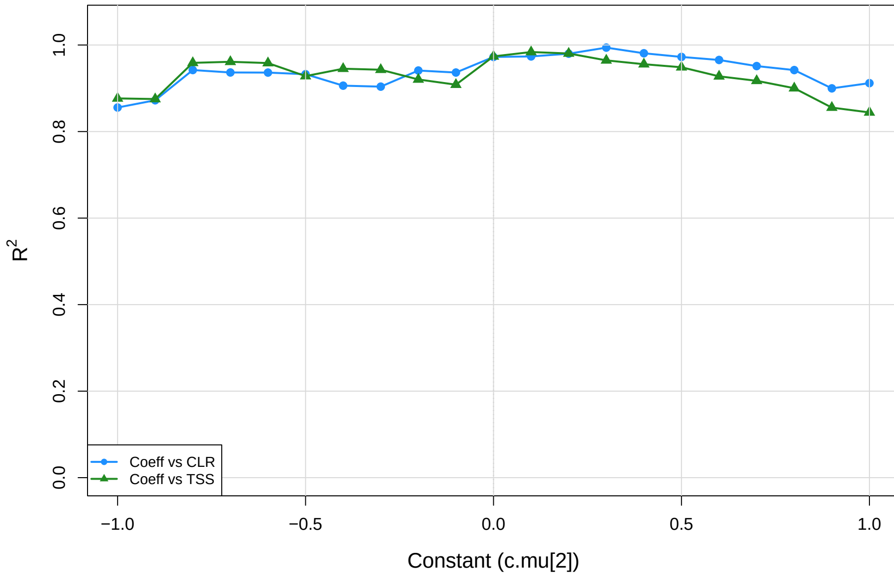
coeff.sm vs CLR vs TSS | cent vs mage | gamma=1e-04 R-squared of red-dot regression
