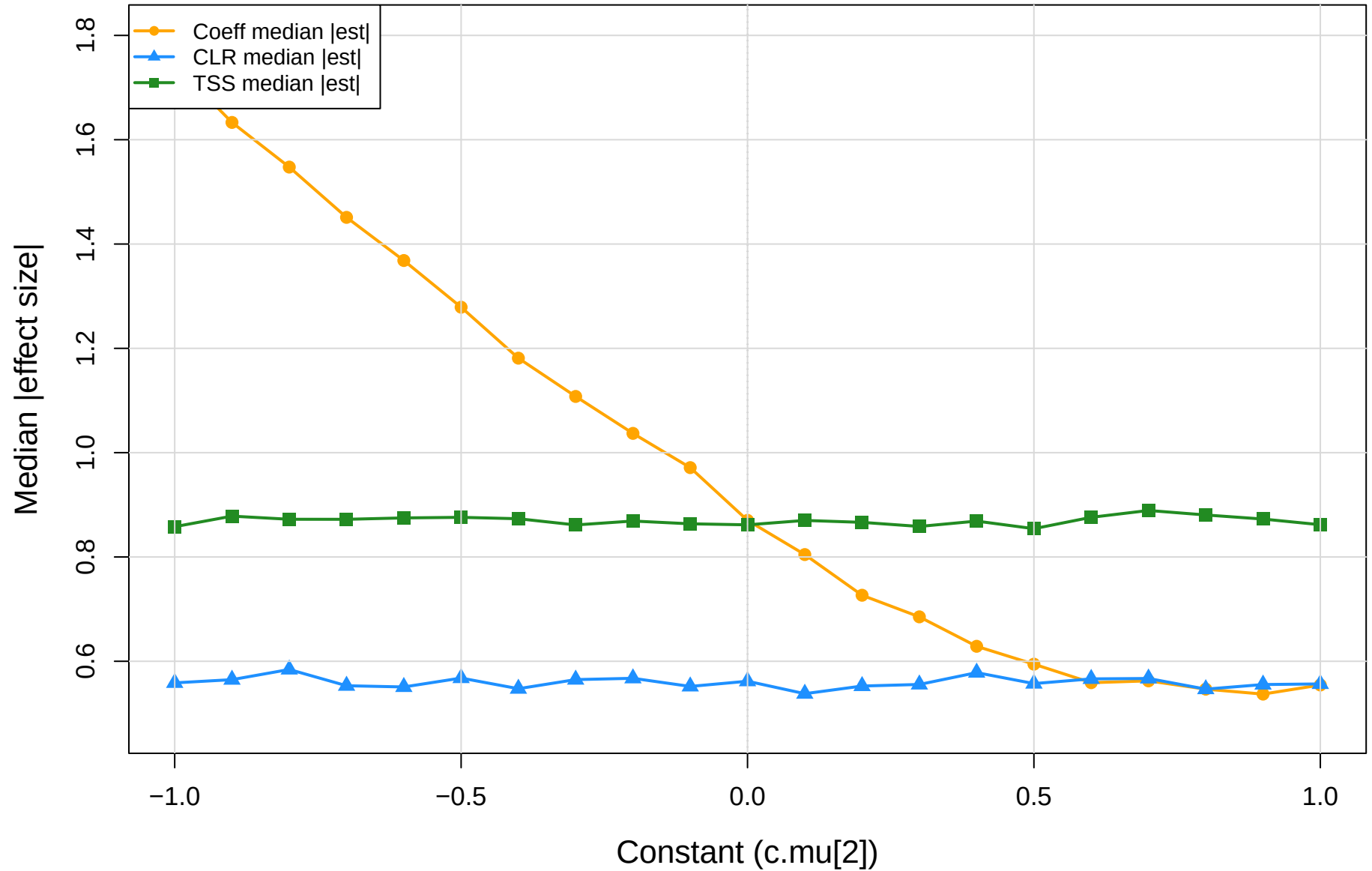
coeff.sm vs CLR vs TSS | cent vs pup | gamma=1e-04 Median absolute effect size
