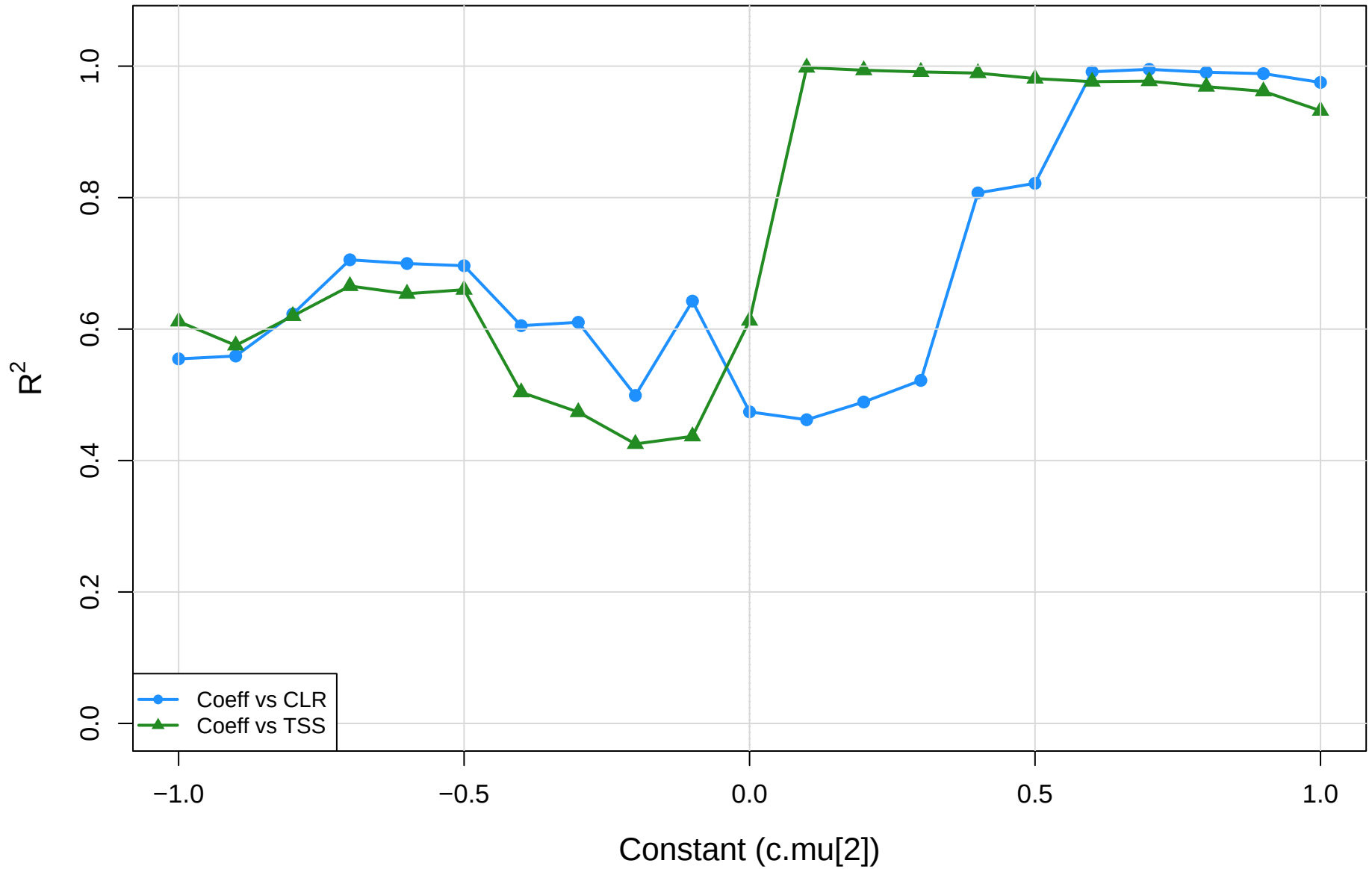
coeff.sm vs CLR vs TSS | cent vs pup | gamma=1e-04 R-squared of red-dot regression
