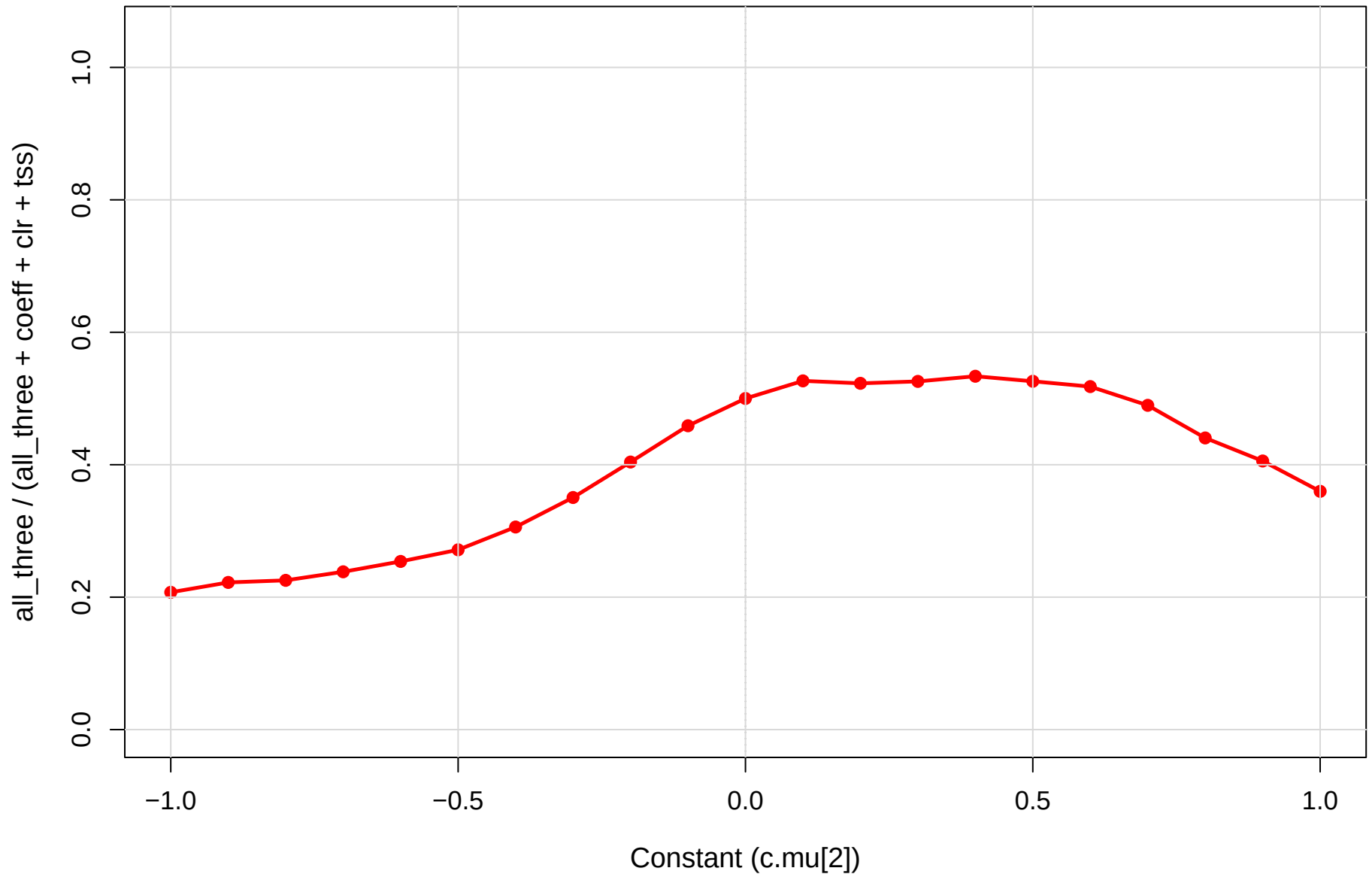
coeff.sm vs CLR vs TSS | cent vs pup | gamma=1e-04 Robustness (1 = all agree, 0 = max disagreement)
