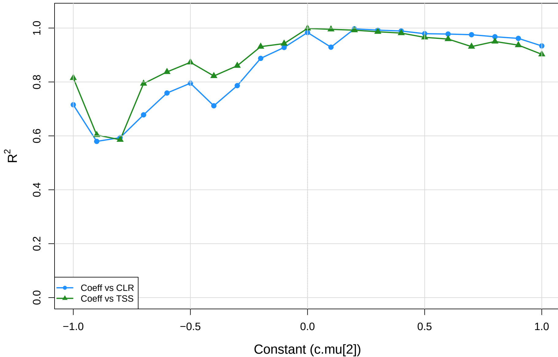
coeff.sm vs CLR vs TSS | eld vs mage | gamma=1e-04 R-squared of red-dot regression
