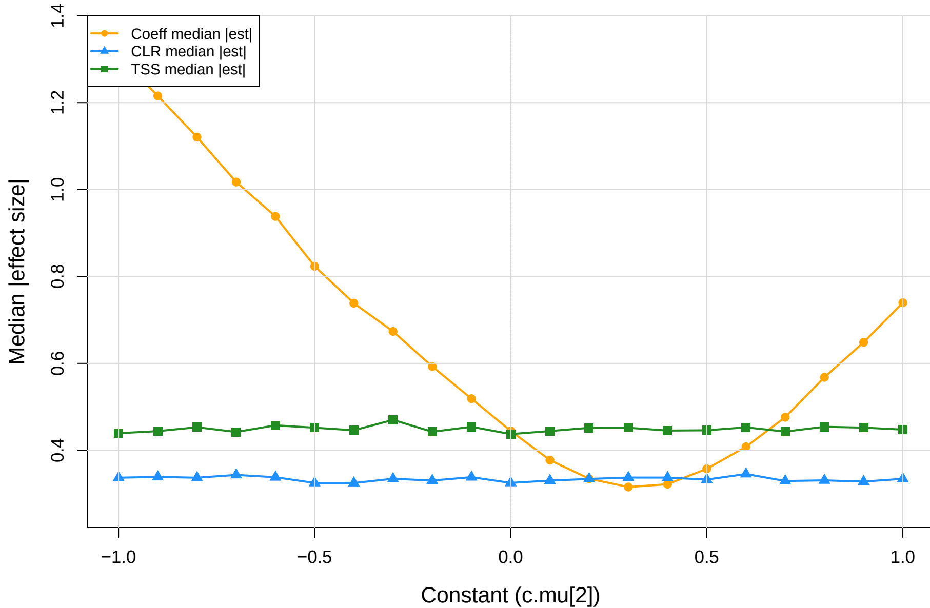
coeff.sm vs CLR vs TSS | eld vs mage | gamma=1e-04 Median absolute effect size
