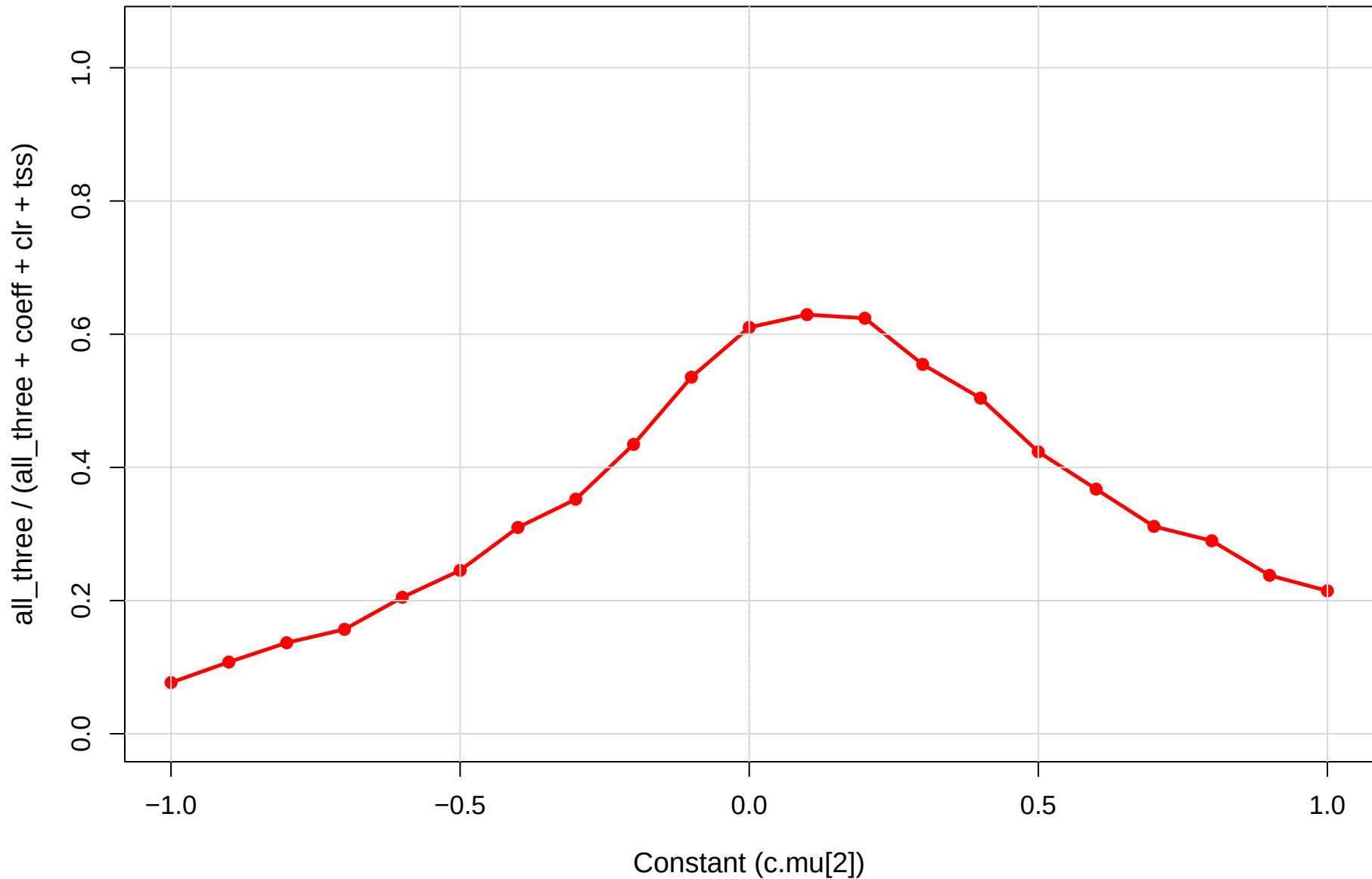
coeff.sm vs CLR vs TSS | eld vs mage | gamma=1e-04 Robustness (1 = all agree, 0 = max disagreement)
