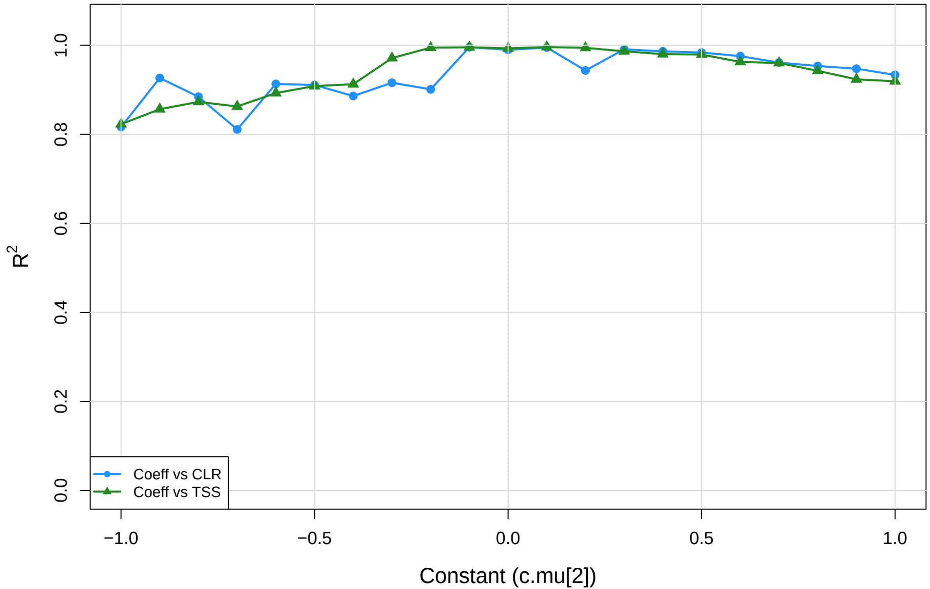
coeff.sm vs CLR vs TSS | eld vs mid | gamma=1e-04 R-squared of red-dot regression
