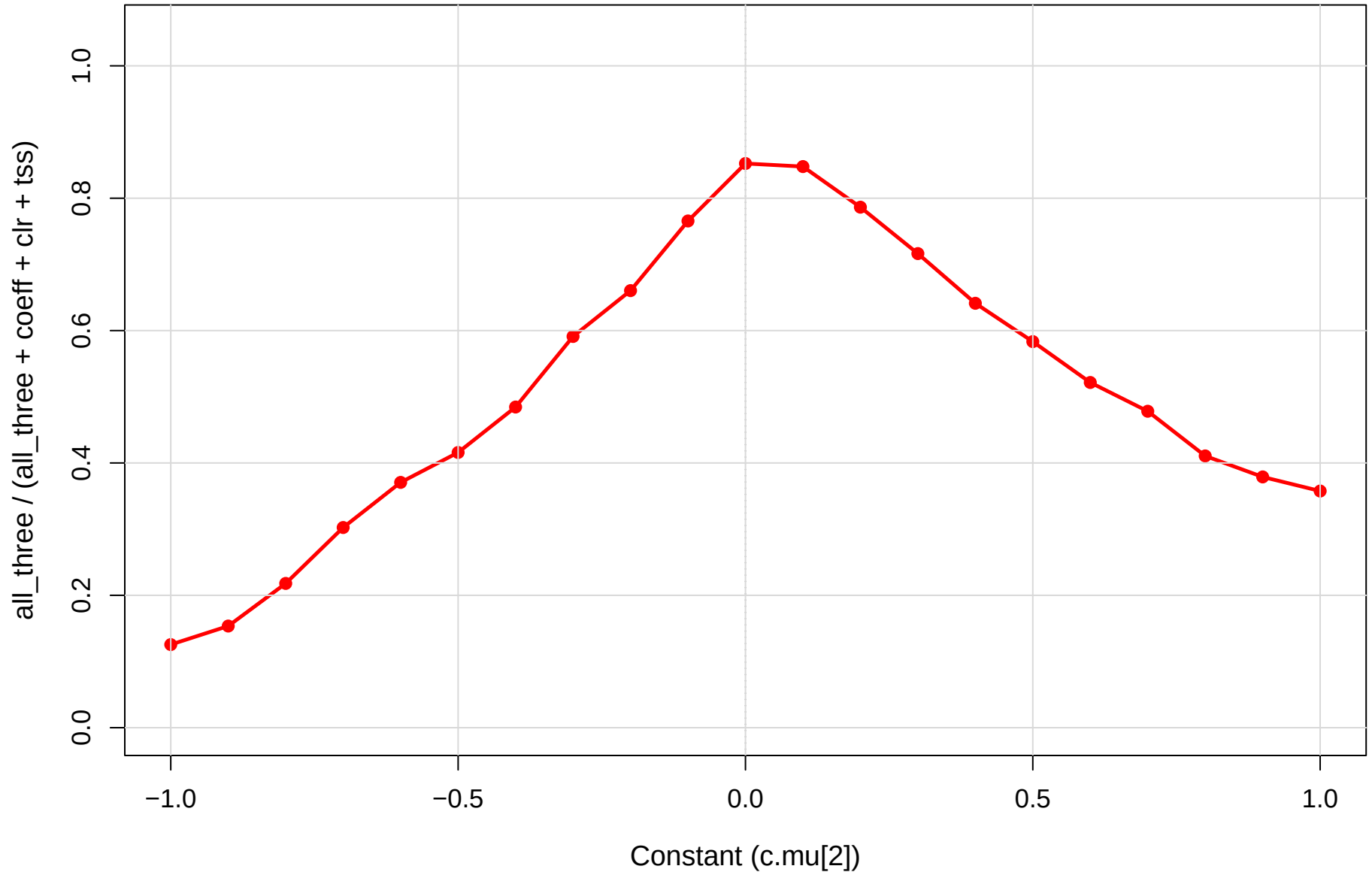
coeff.sm vs CLR vs TSS | eld vs mid | gamma=1e-04 Robustness (1 = all agree, 0 = max disagreement)
