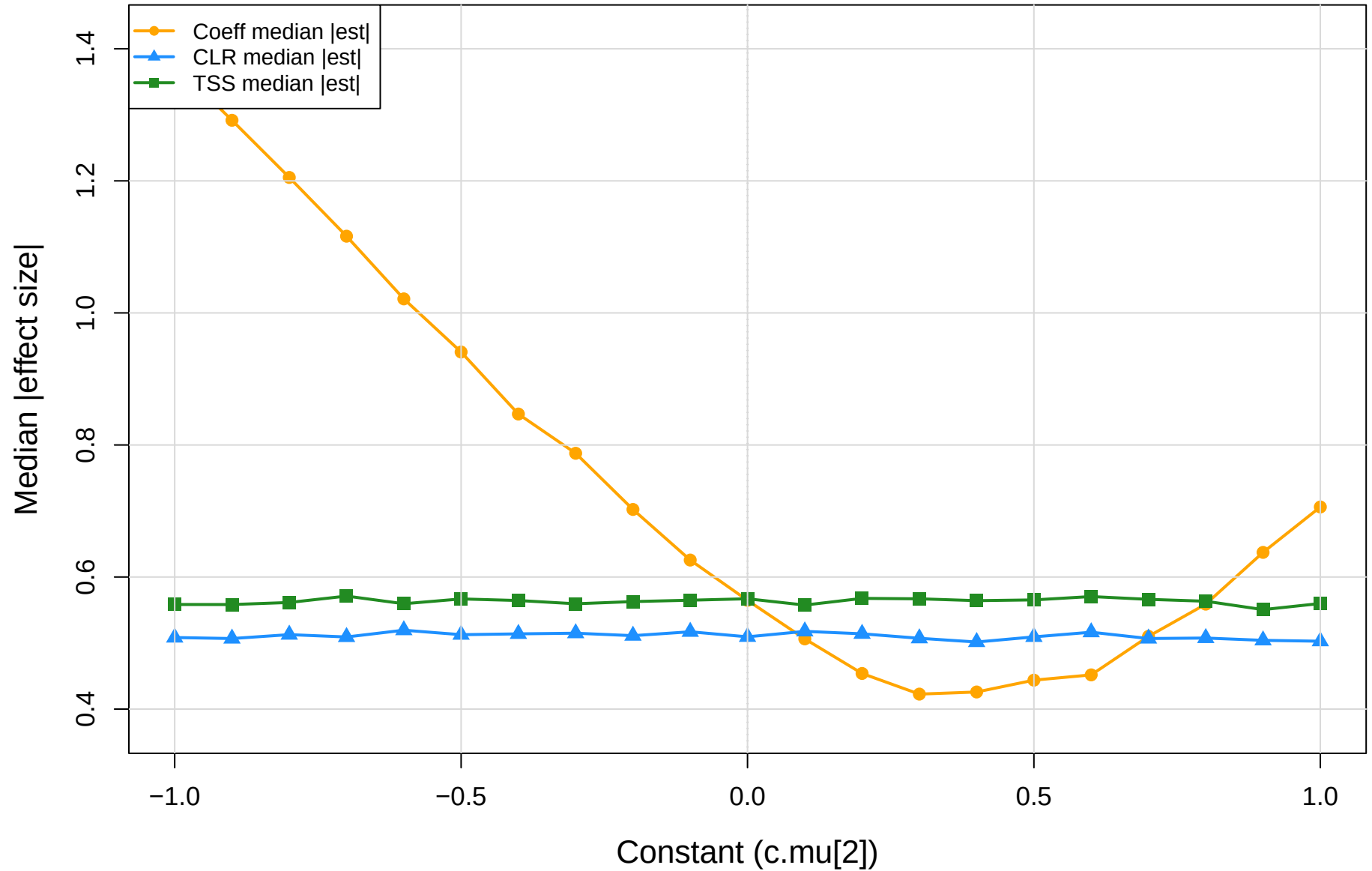
coeff.sm vs CLR vs TSS | eld vs mid | gamma=1e-04 Median absolute effect size
