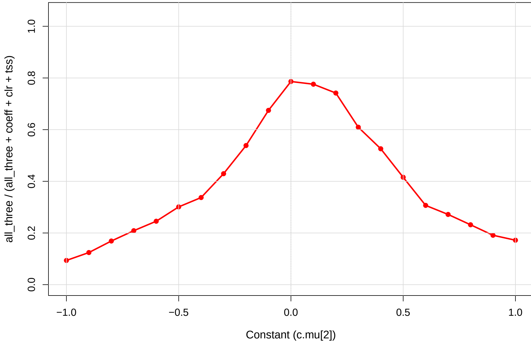
coeff.sm vs CLR vs TSS | kin vs mage | gamma=1e-04 Robustness (1 = all agree, 0 = max disagreement)
