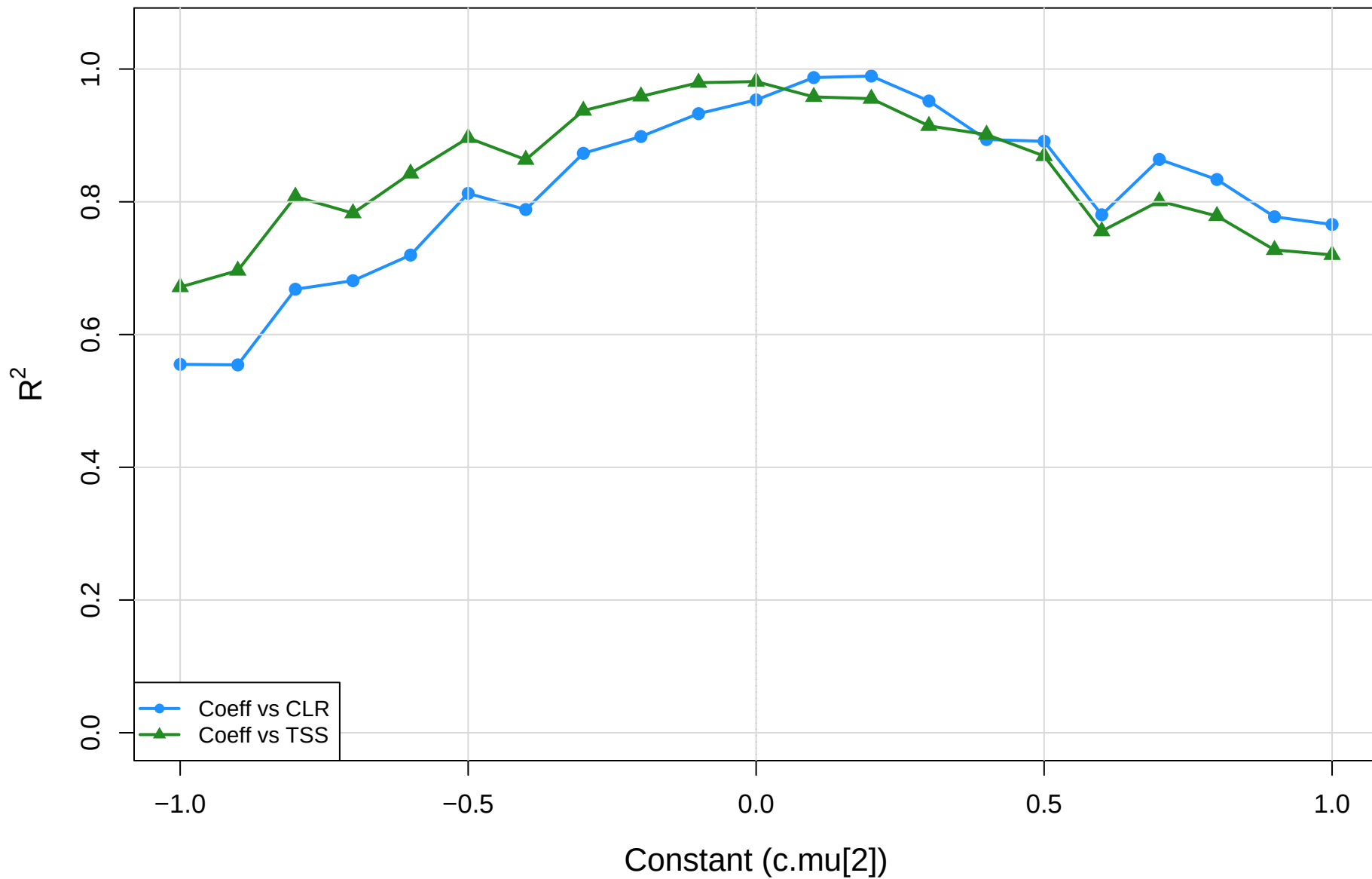
coeff.sm vs CLR vs TSS | kin vs mage | gamma=1e-04 R-squared of red-dot regression
