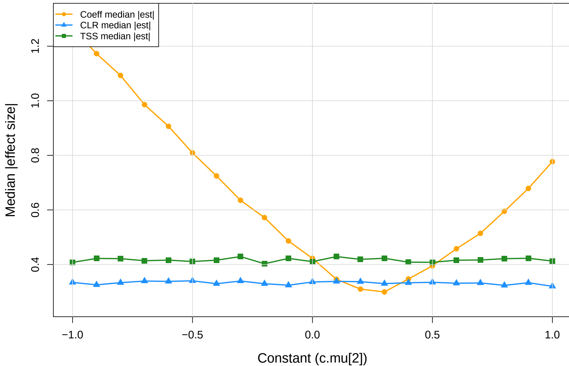
coeff.sm vs CLR vs TSS | kin vs mage | gamma=1e-04 Median absolute effect size
