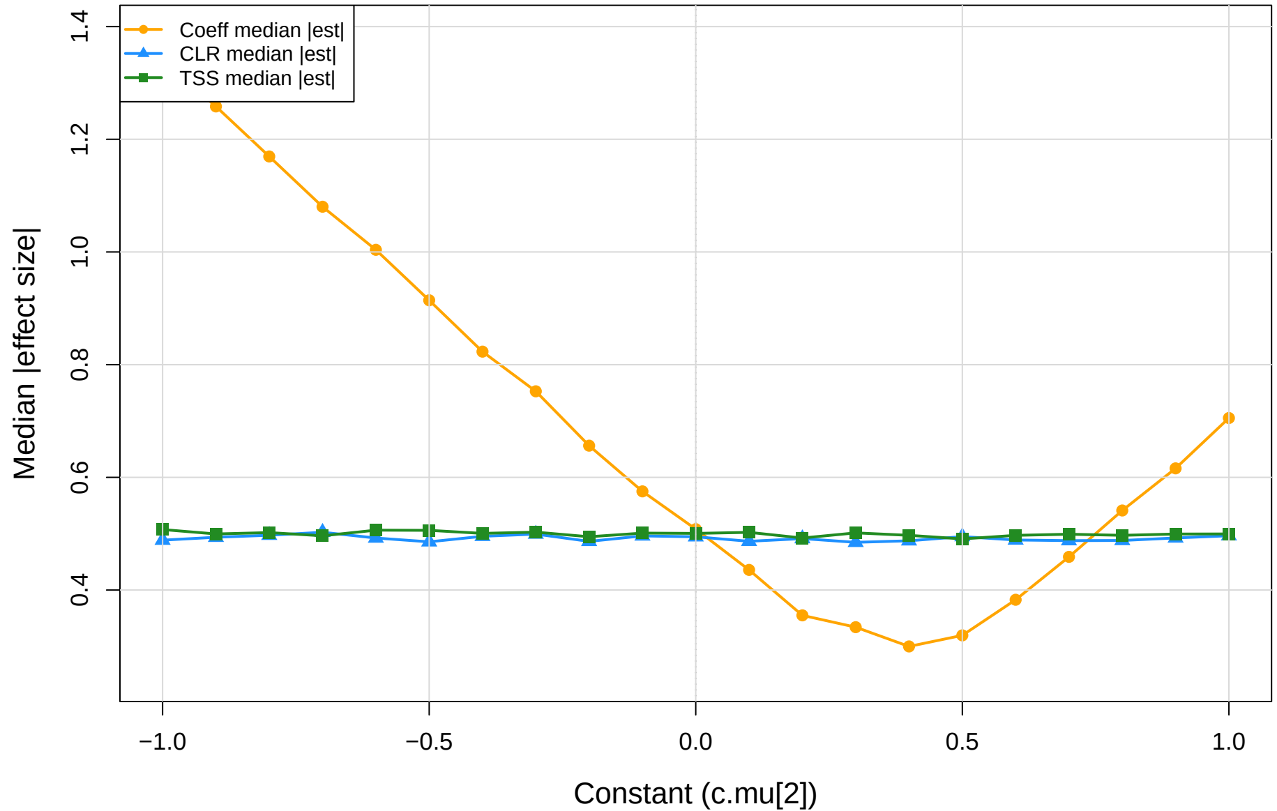
coeff.sm vs CLR vs TSS | kin vs mid | gamma=1e-04 Median absolute effect size
