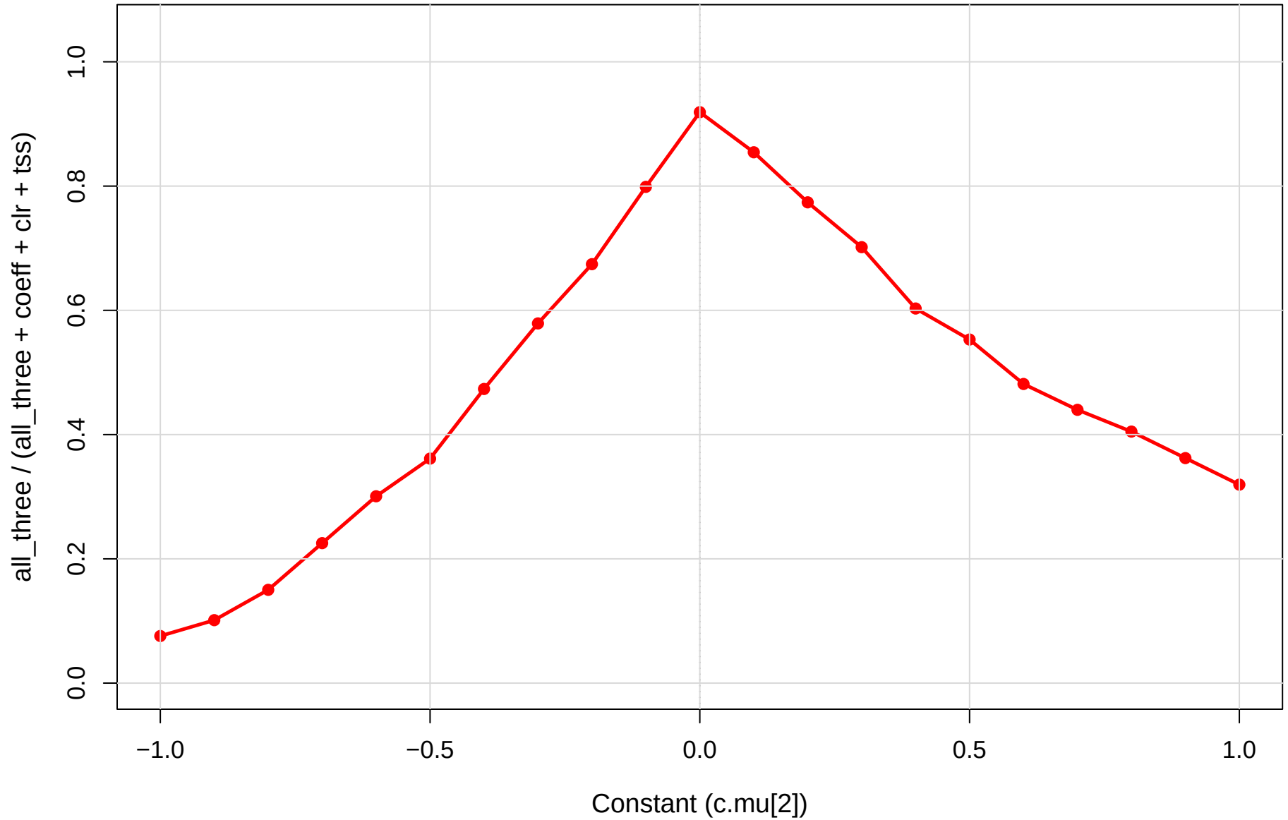
coeff.sm vs CLR vs TSS | kin vs mid | gamma=1e-04 Robustness (1 = all agree, 0 = max disagreement)
