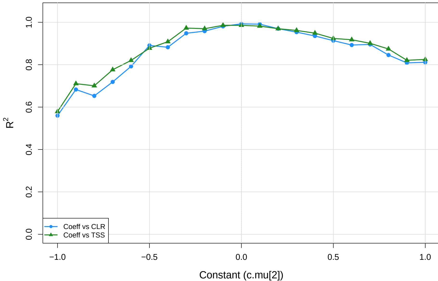
coeff.sm vs CLR vs TSS | kin vs mid | gamma=1e-04 R-squared of red-dot regression
