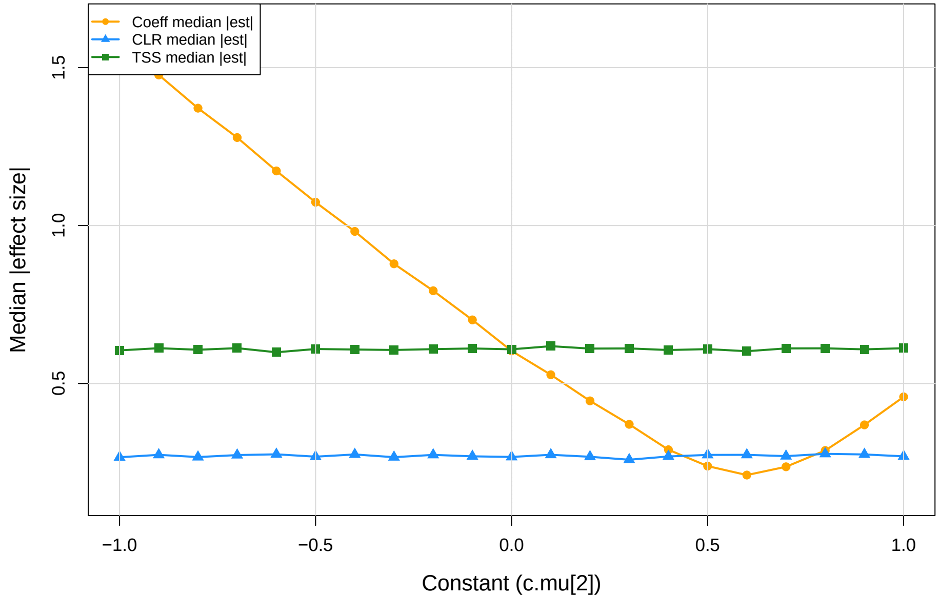
coeff.sm vs CLR vs TSS | kin vs pup | gamma=1e-04 Median absolute effect size
