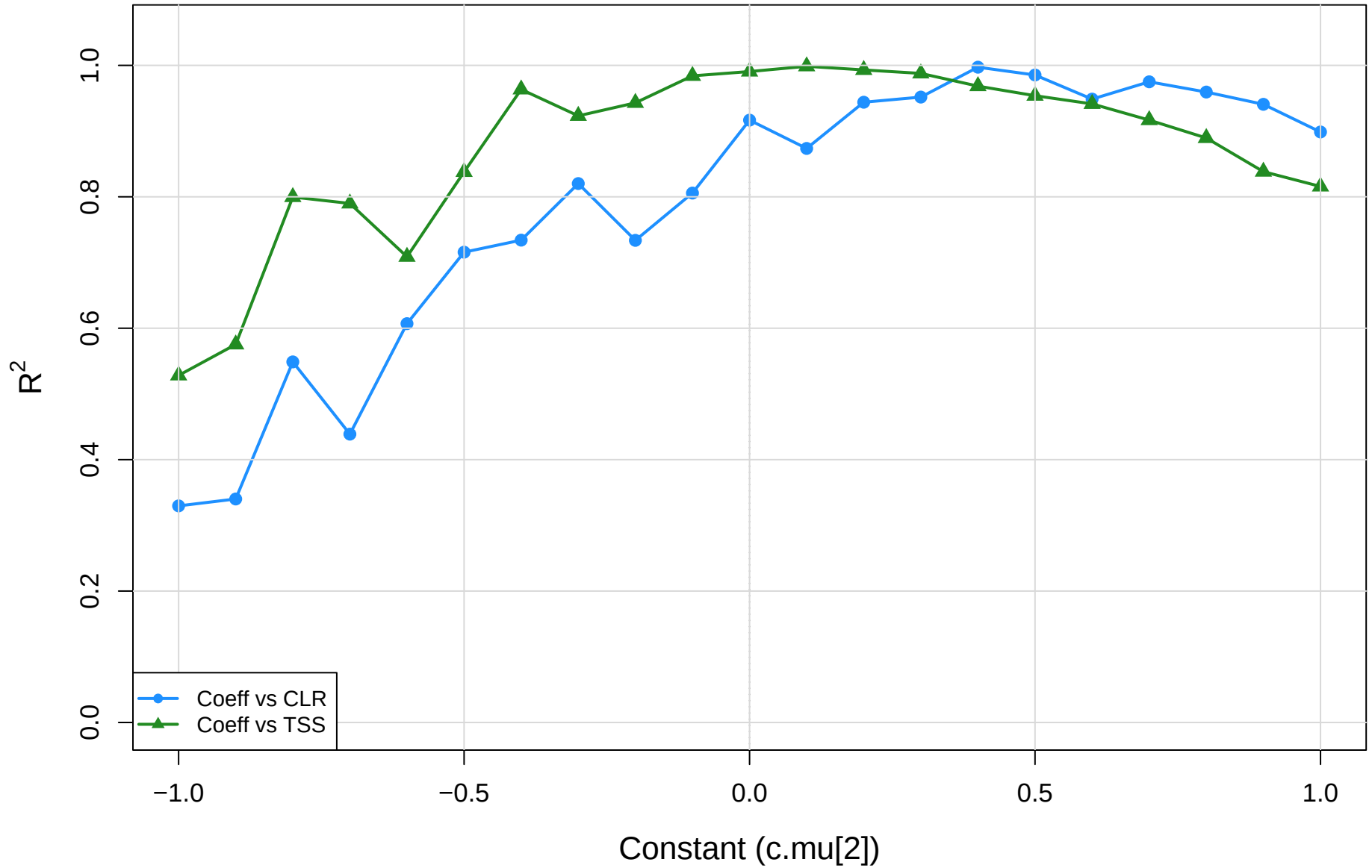
coeff.sm vs CLR vs TSS | kin vs pup | gamma=1e-04 R-squared of red-dot regression
