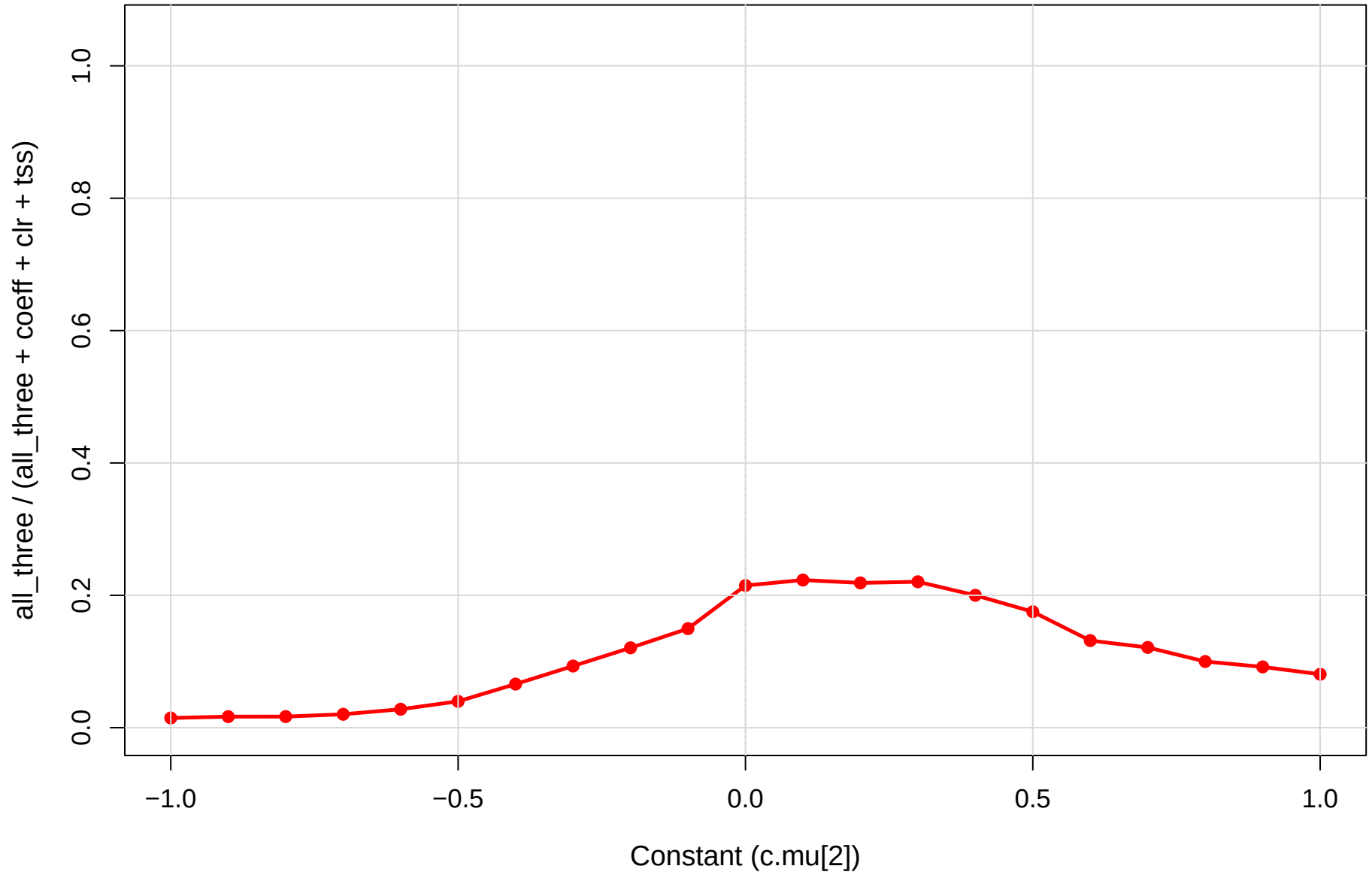
coeff.sm vs CLR vs TSS | kin vs pup | gamma=1e-04 Robustness (1 = all agree, 0 = max disagreement)
