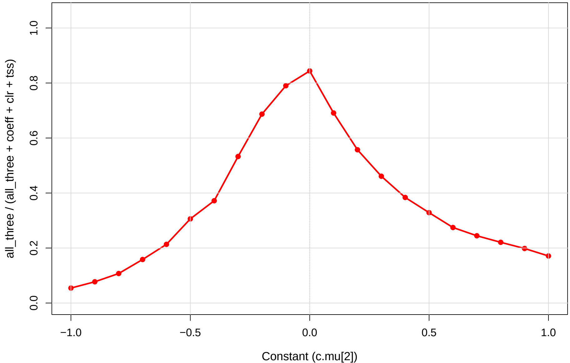
coeff.sm vs CLR vs TSS | mage vs mid | gamma=1e-04 Robustness (1 = all agree, 0 = max disagreement)
