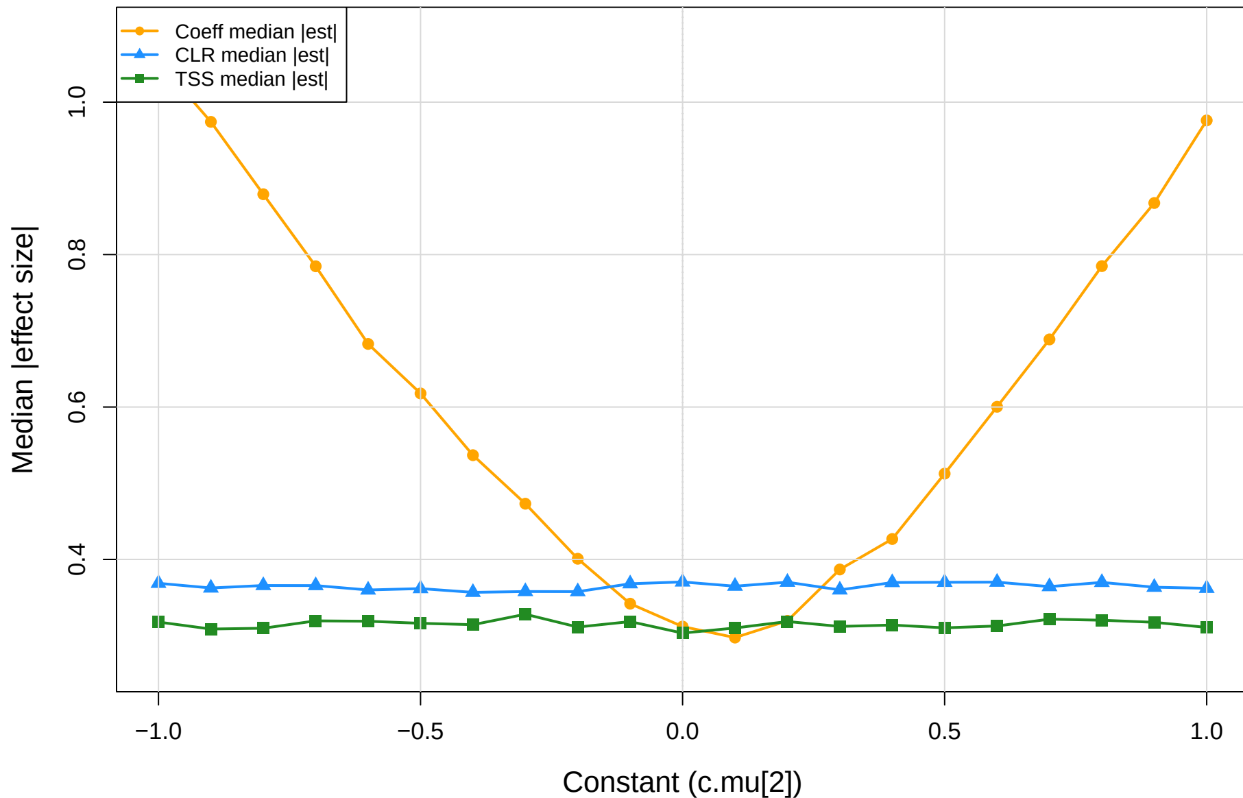
coeff.sm vs CLR vs TSS | mage vs mid | gamma=1e-04 Median absolute effect size
