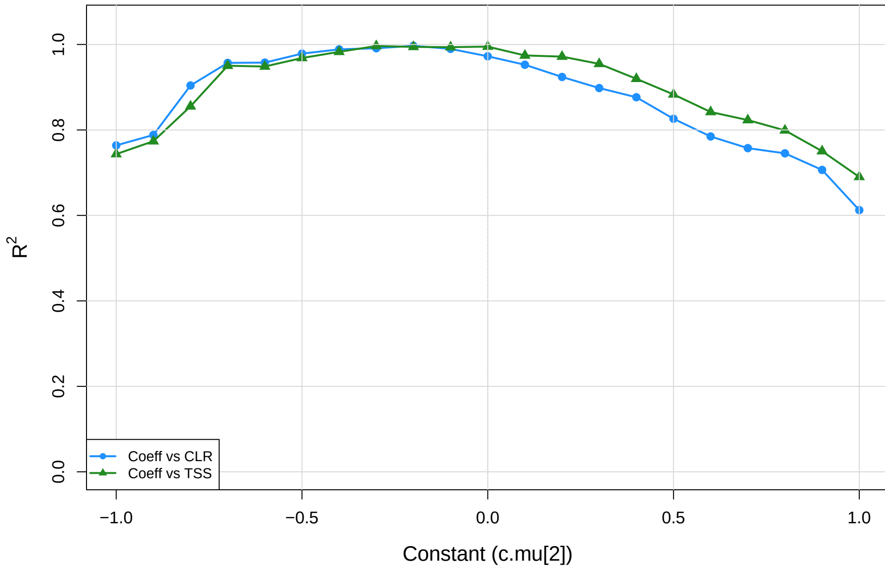
coeff.sm vs CLR vs TSS | mage vs mid | gamma=1e-04 R-squared of red-dot regression
