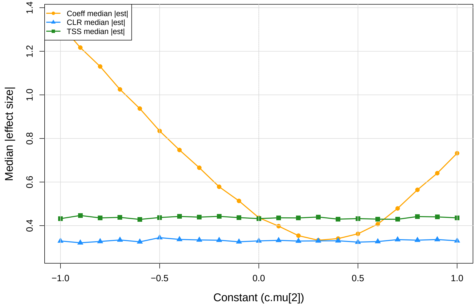
coeff.sm vs CLR vs TSS | mage vs pup | gamma=1e-04 Median absolute effect size
