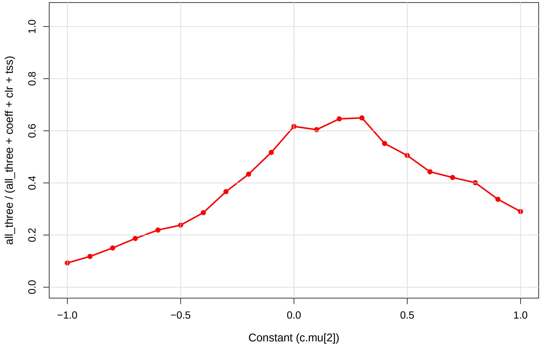
coeff.sm vs CLR vs TSS | mage vs pup | gamma=1e-04 Robustness (1 = all agree, 0 = max disagreement)
