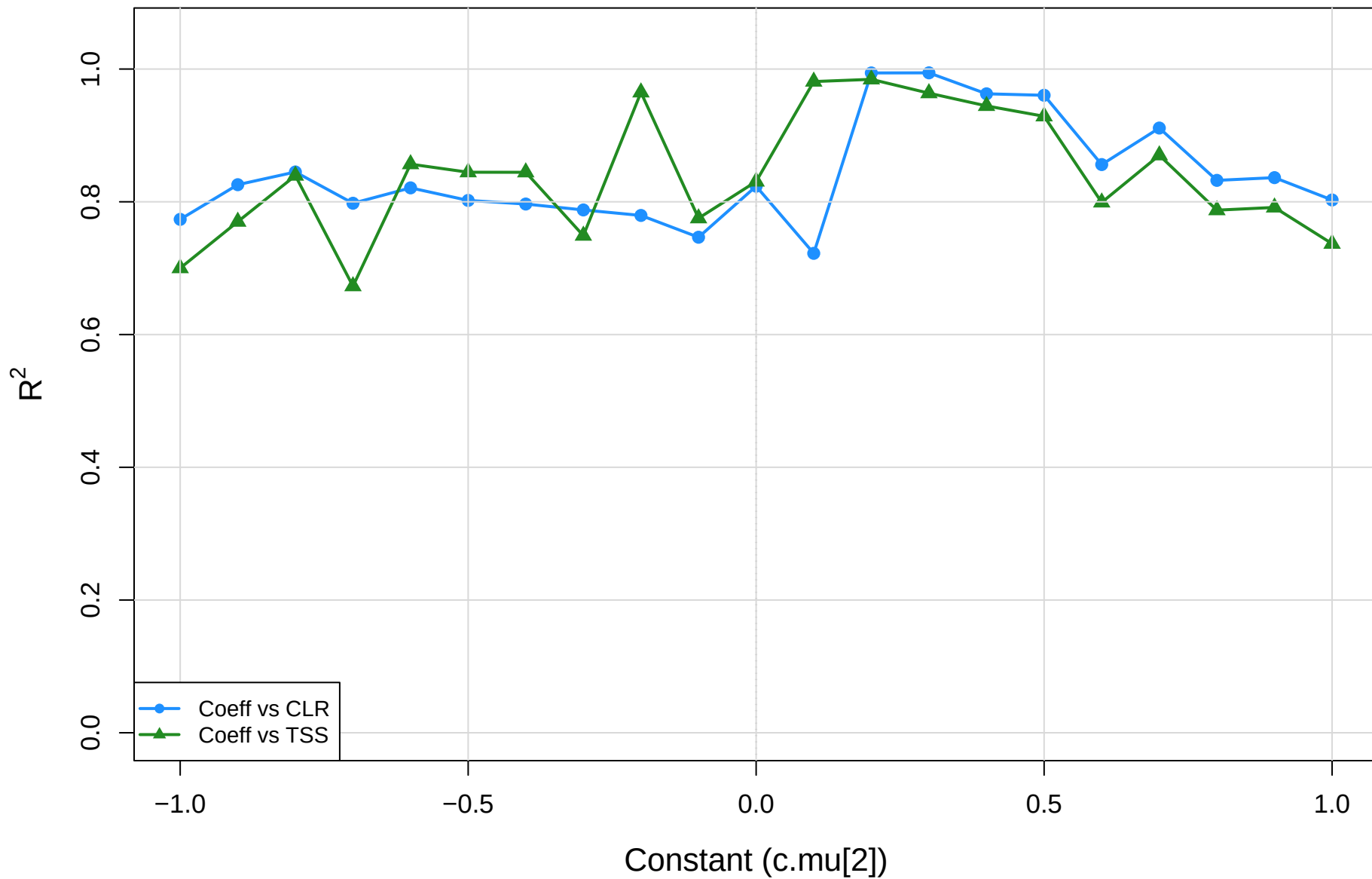
coeff.sm vs CLR vs TSS | mage vs pup | gamma=1e-04 R-squared of red-dot regression
