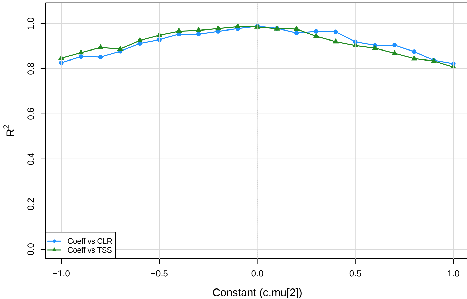
coeff.sm vs CLR vs TSS | mage vs you | gamma=1e-04 R-squared of red-dot regression
