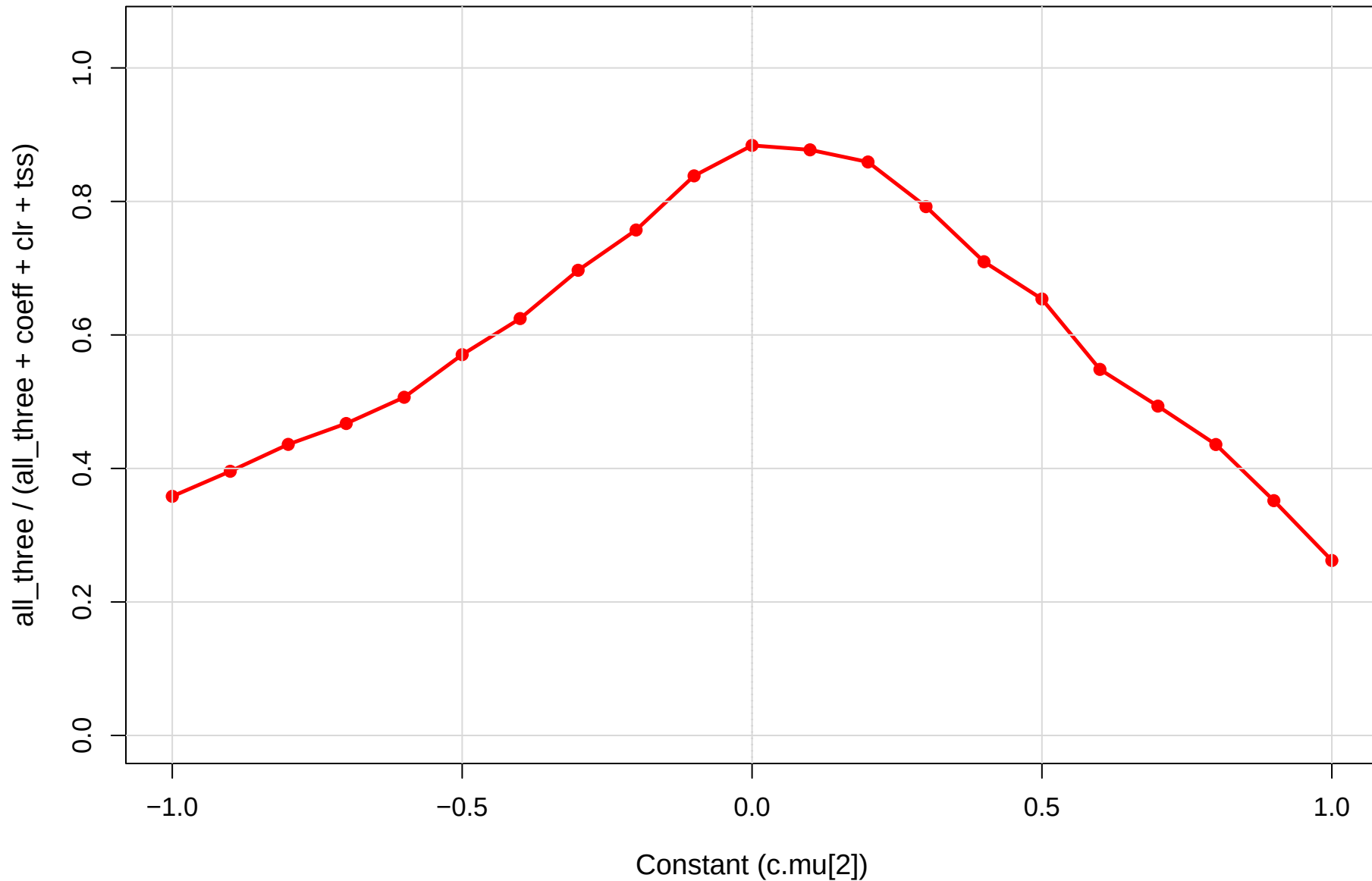
coeff.sm vs CLR vs TSS | mage vs you | gamma=1e-04 Robustness (1 = all agree, 0 = max disagreement)
