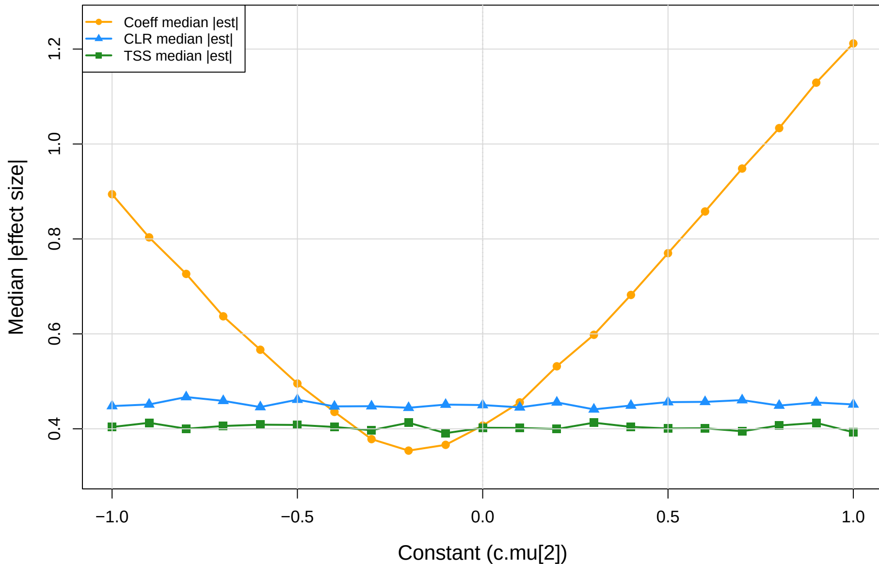
coeff.sm vs CLR vs TSS | mage vs you | gamma=1e-04 Median absolute effect size
