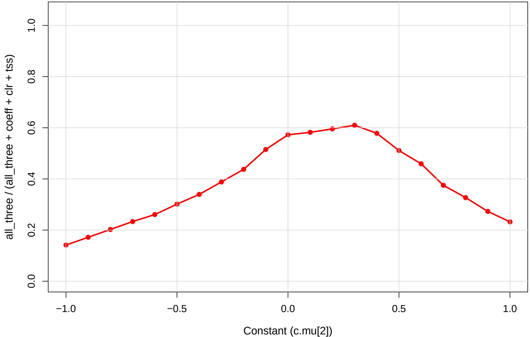
coeff.sm vs CLR vs TSS | mid vs pup | gamma=1e-04 Robustness (1 = all agree, 0 = max disagreement)
