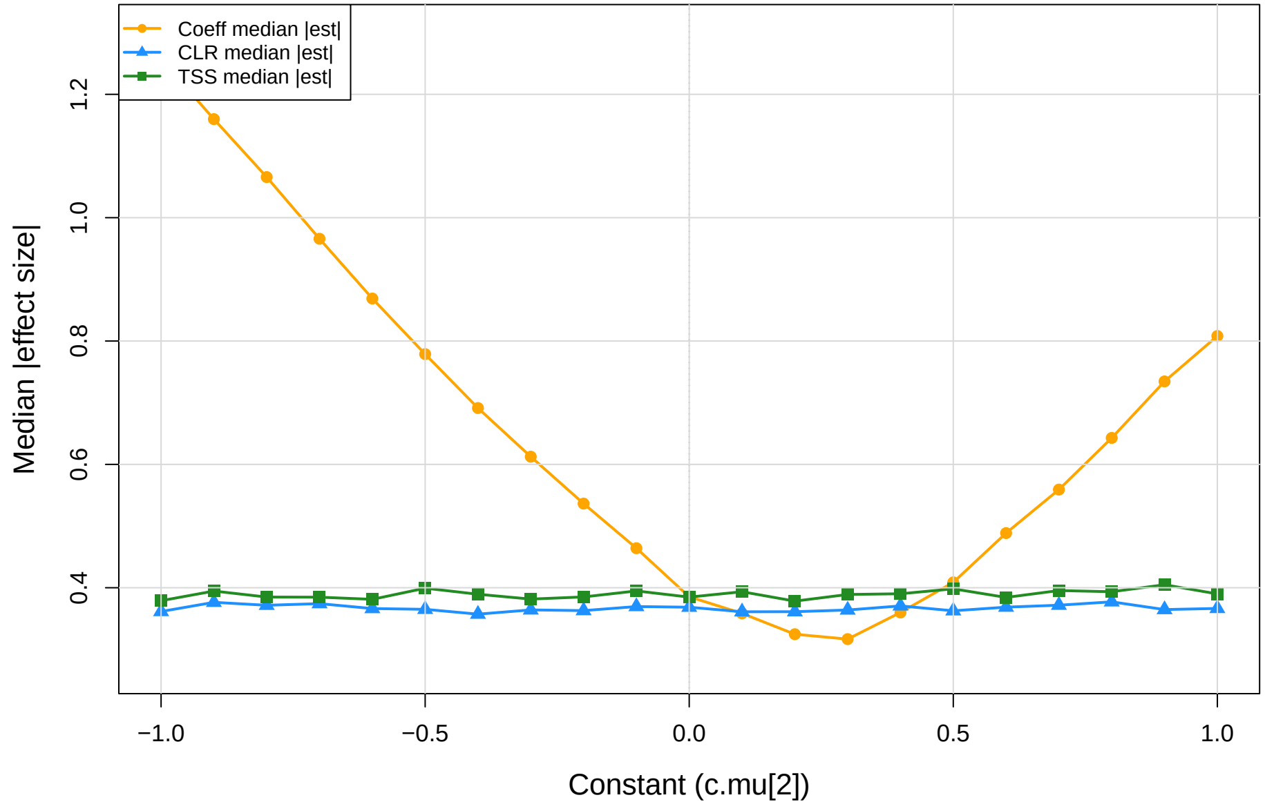
coeff.sm vs CLR vs TSS | mid vs pup | gamma=1e-04 Median absolute effect size
