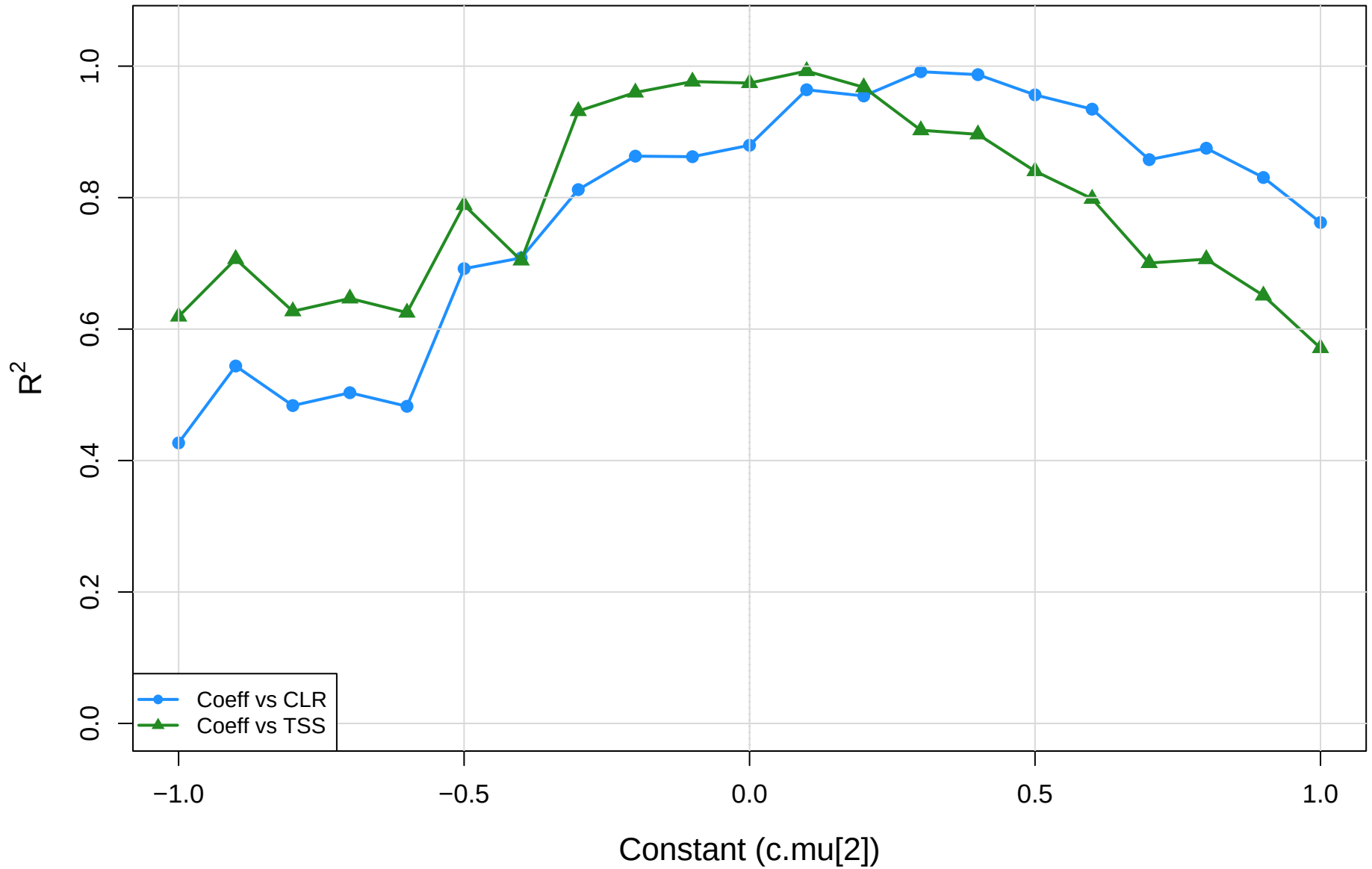
coeff.sm vs CLR vs TSS | mid vs pup | gamma=1e-04 R-squared of red-dot regression
