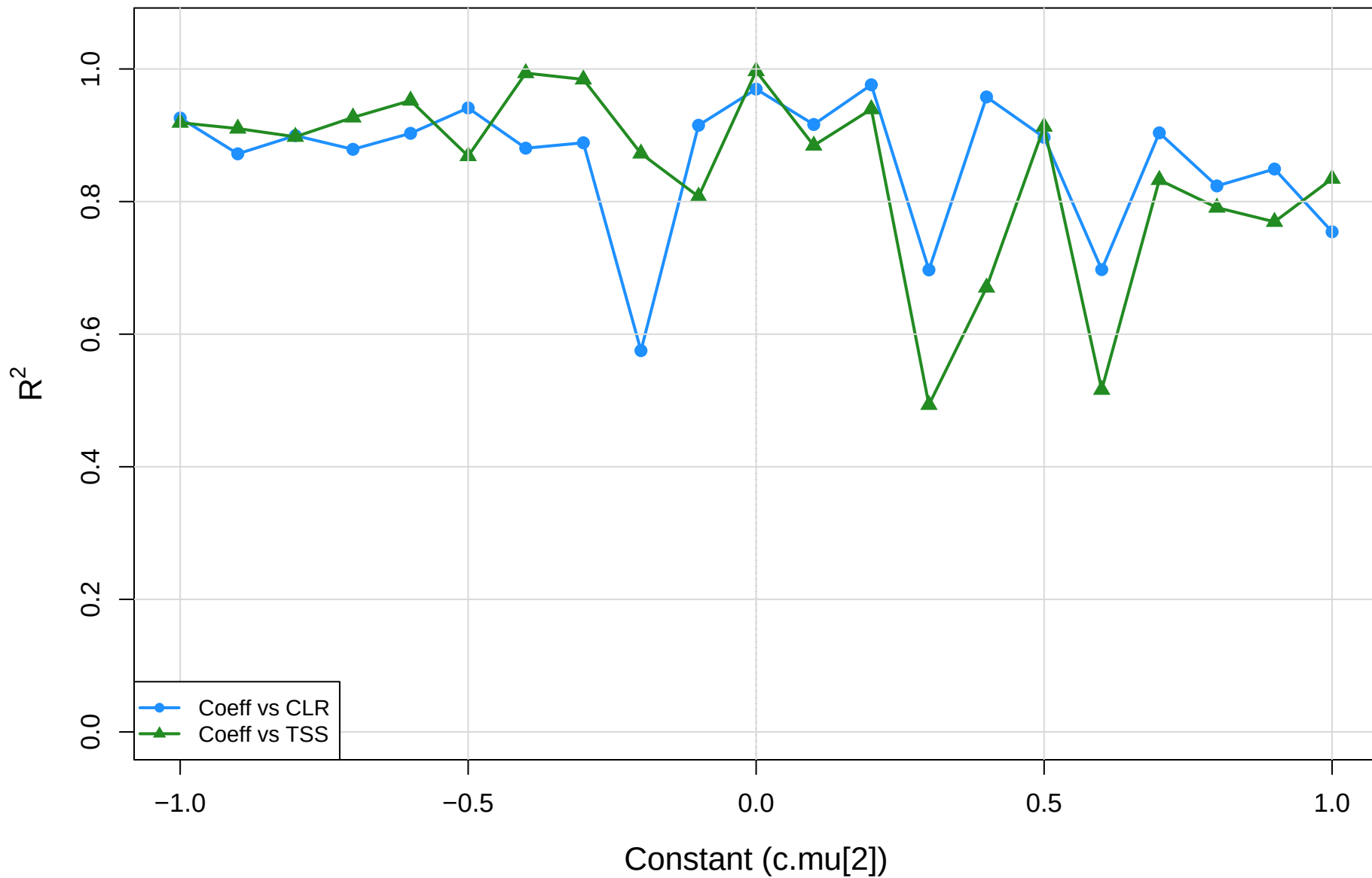
coeff.sm vs CLR vs TSS | cent vs mage | gamma=0.5 R-squared of red-dot regression
