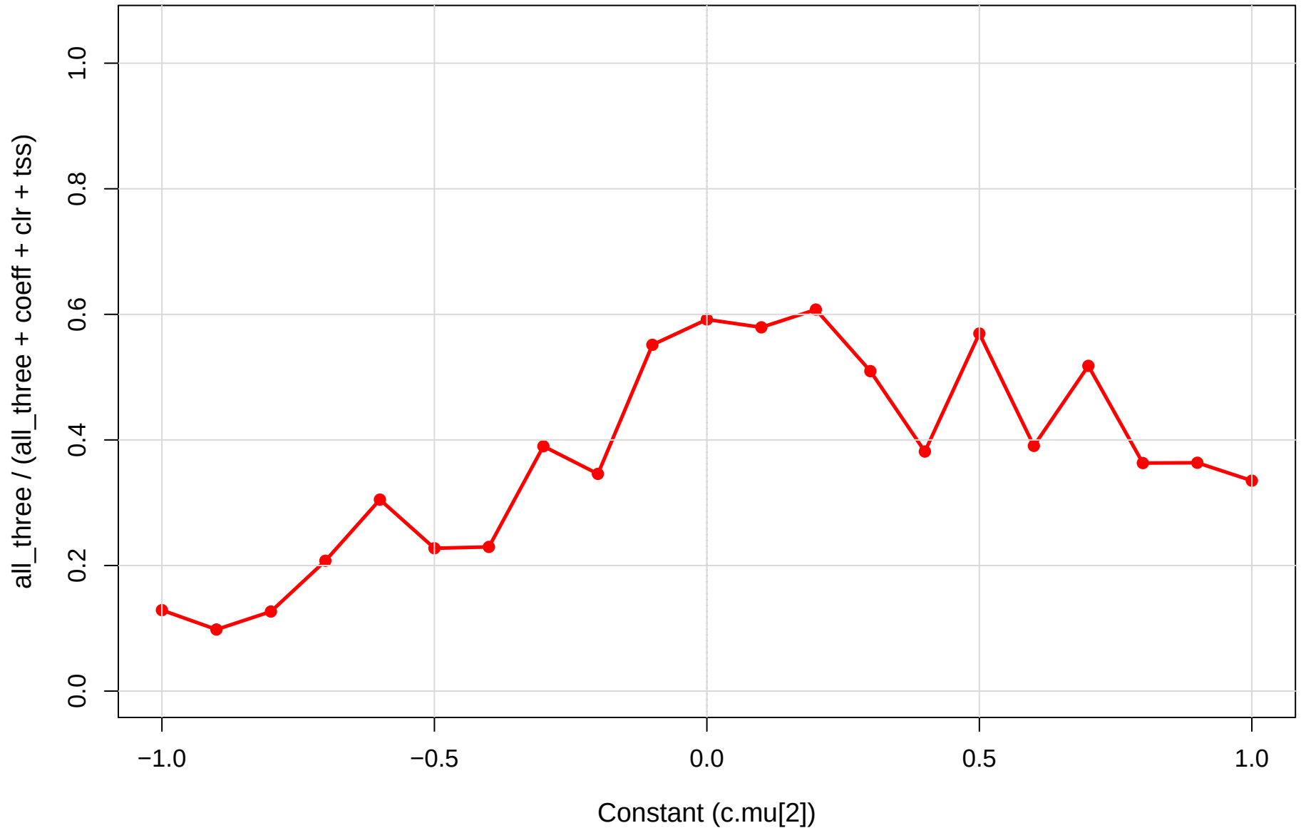
coeff.sm vs CLR vs TSS | cent vs mage | gamma=0.5 Robustness (1 = all agree, 0 = max disagreement)
