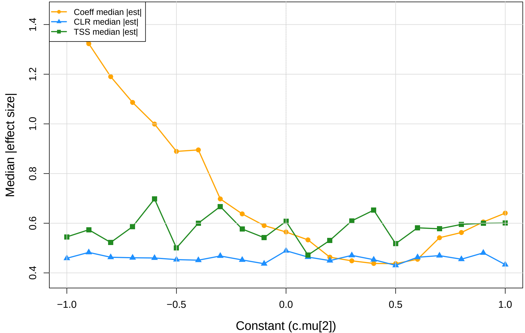
coeff.sm vs CLR vs TSS | cent vs mage | gamma=0.5 Median absolute effect size
