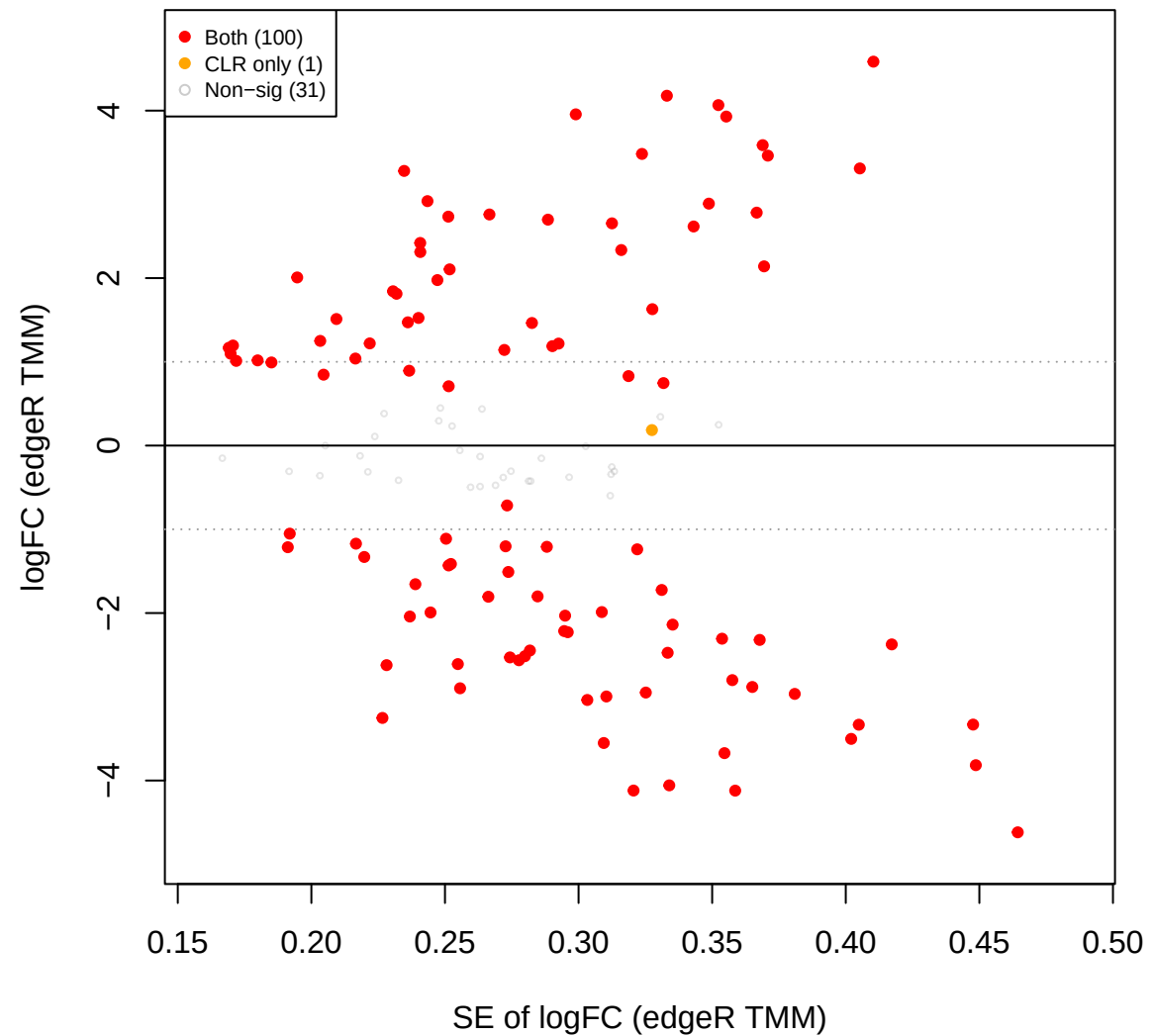
you vs cent – edgeR TMM FILTERED (190 OTUs, CLR sig overlaid)
