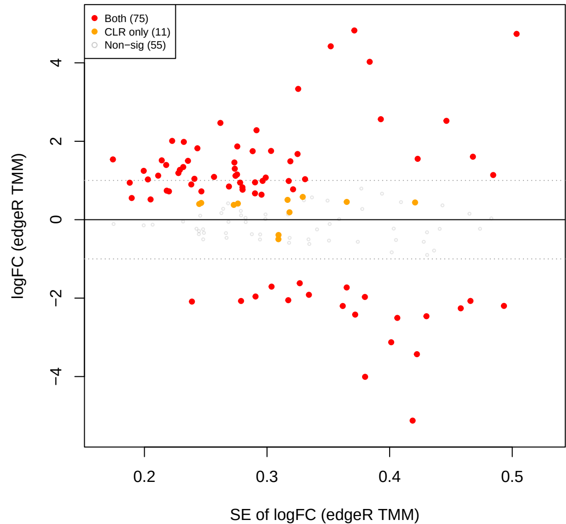
mid vs eld – edgeR TMM FILTERED (209 OTUs, CLR sig overlaid)
