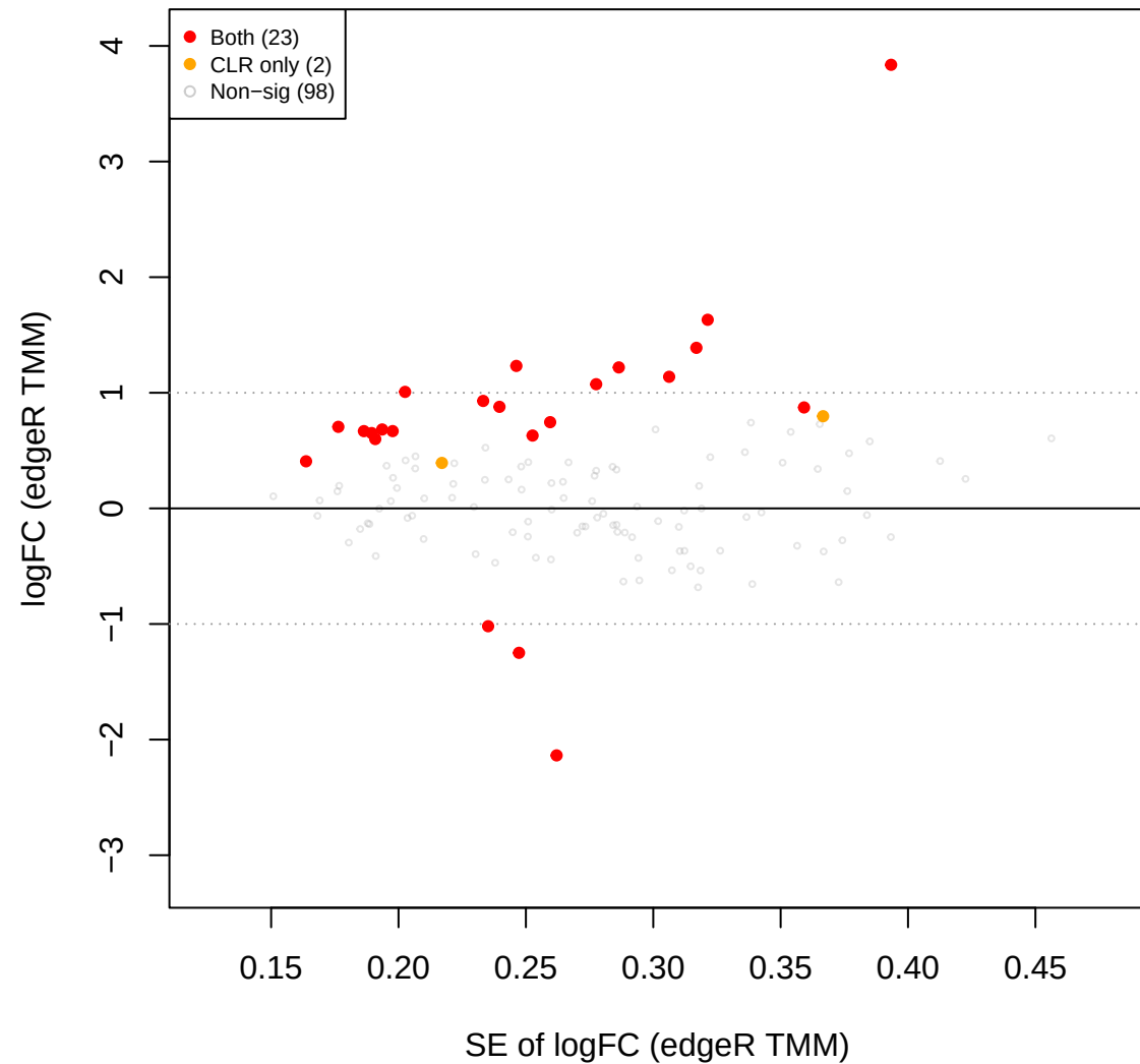
kin vs pup – edgeR TMM FILTERED (185 OTUs, CLR sig overlaid)
