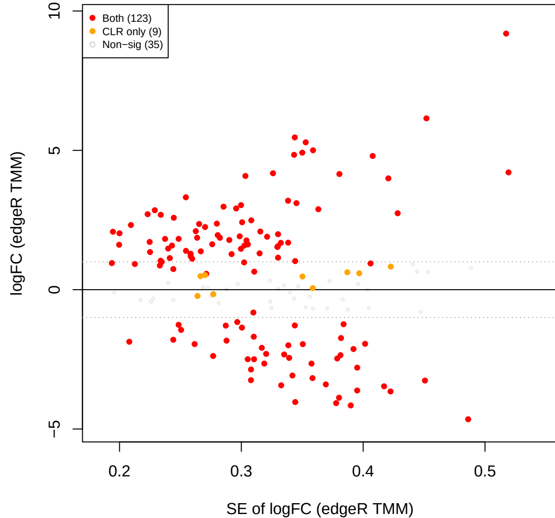
pup vs eld – edgeR TMM FILTERED (220 OTUs, CLR sig overlaid)
