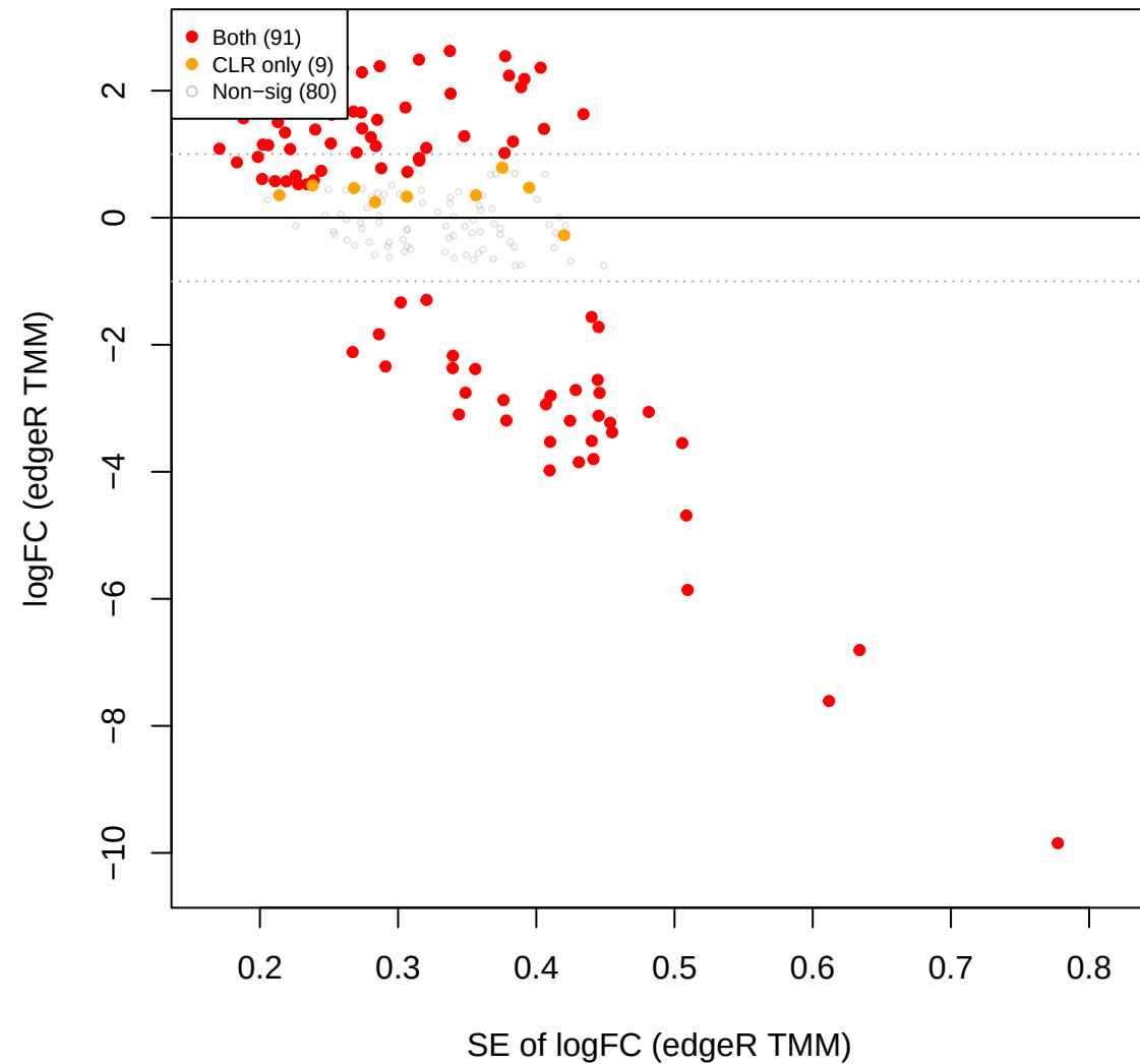
mage vs cent – edgeR TMM FILTERED (251 OTUs, CLR sig over
