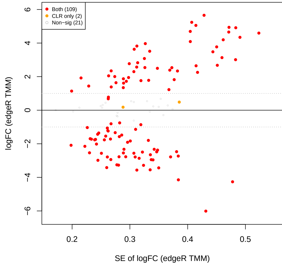
kin vs you – edgeR TMM FILTERED (160 OTUs, CLR sig overlay)
