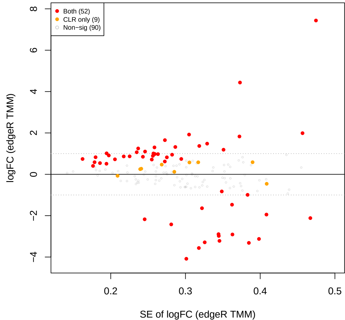
pup vs mage – edgeR TMM FILTERED (218 OTUs, CLR sig over
