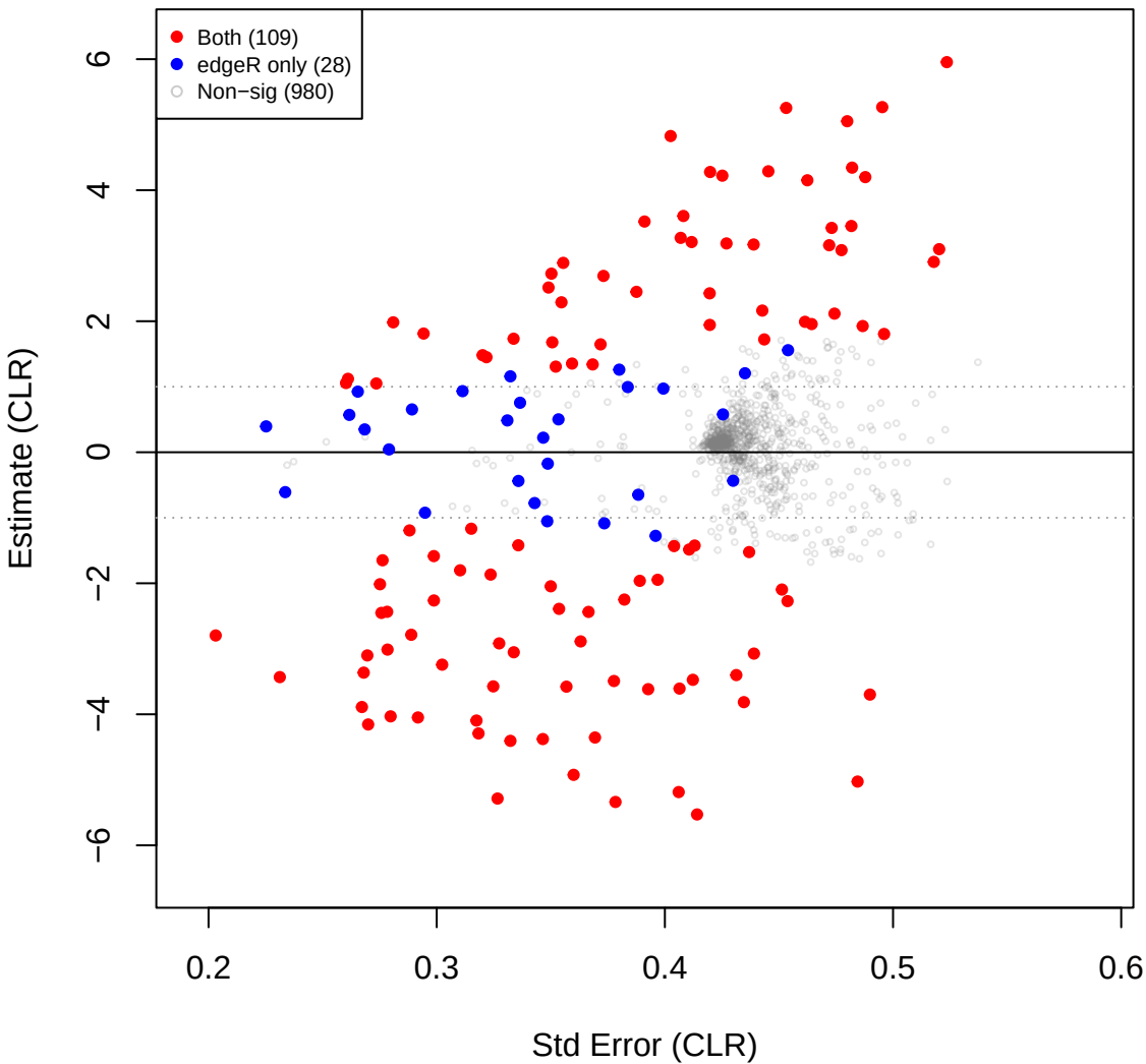
kin vs you – CLR (edgeR TMM sig overlay)
