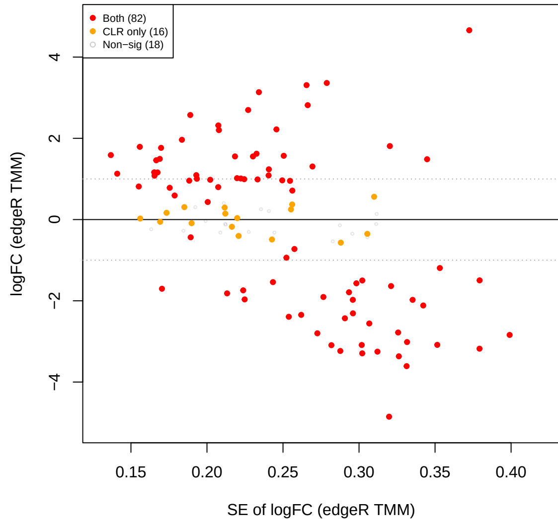
pup vs cent – edgeR TMM FILTERED (173 OTUs, CLR sig overlaid)
