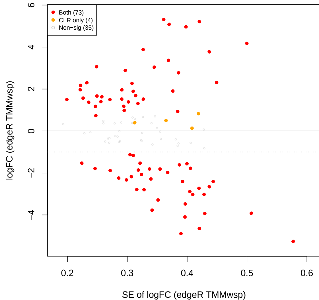
kin vs eld – edgeR TMMwsp FILTERED (156 OTUs, CLR sig over
