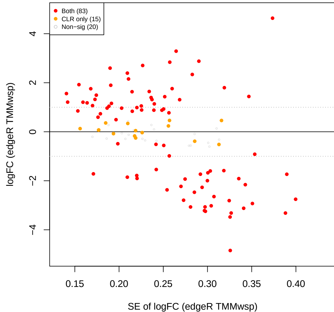
pup vs cent – edgeR TMMwsp FILTERED (173 OTUs, CLR sig overlay)
