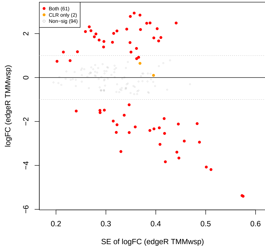
eld vs cent – edgeR TMMwsp FILTERED (252 OTUs, CLR sig overlay)
