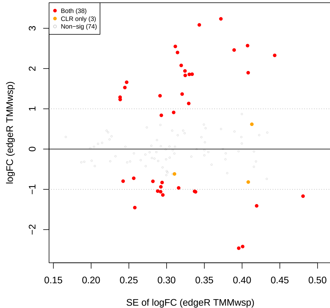
kin vs mage – edgeR TMMwsp FILTERED (166 OTUs, CLR sig ov
