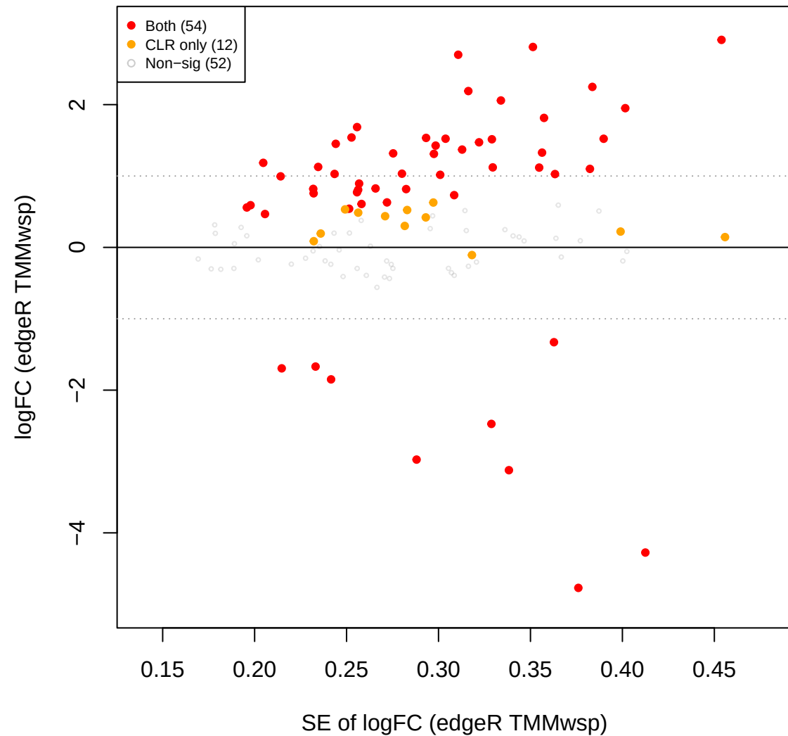
kin vs mid – edgeR TMMwsp FILTERED (179 OTUs, CLR sig over)
