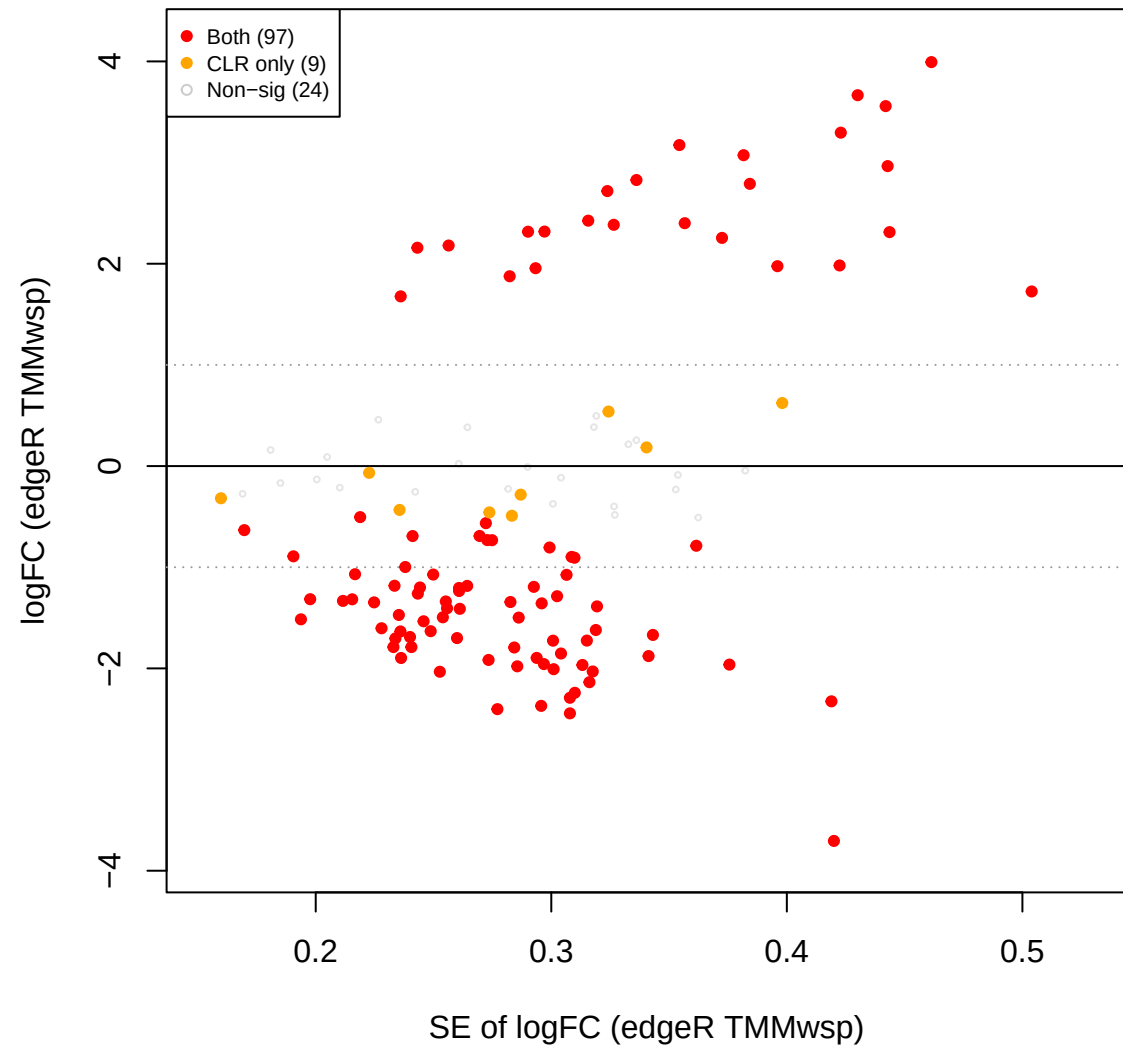
mid vs you – edgeR TMMwsp FILTERED (186 OTUs, CLR sig over)
