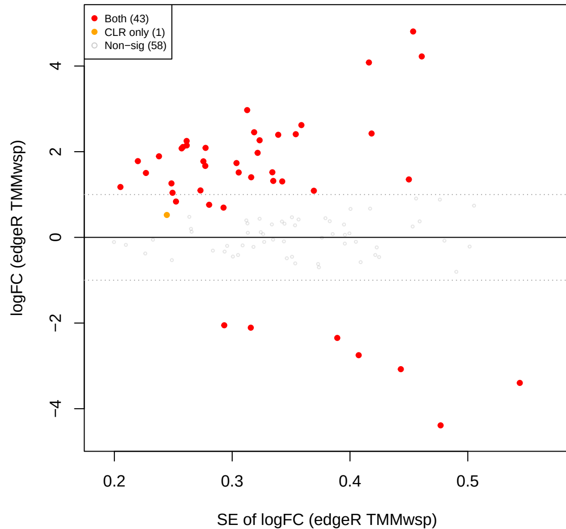
mage vs eld – edgeR TMMwsp FILTERED (173 OTUs, CLR sig ov
