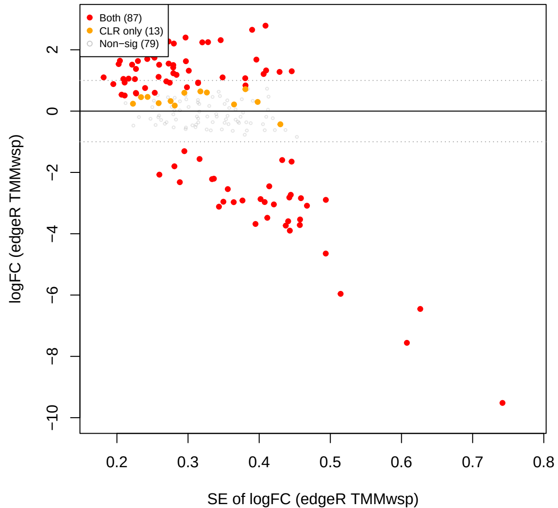
mage vs cent – edgeR TMMwsp FILTERED (251 OTUs, CLR sig ov
