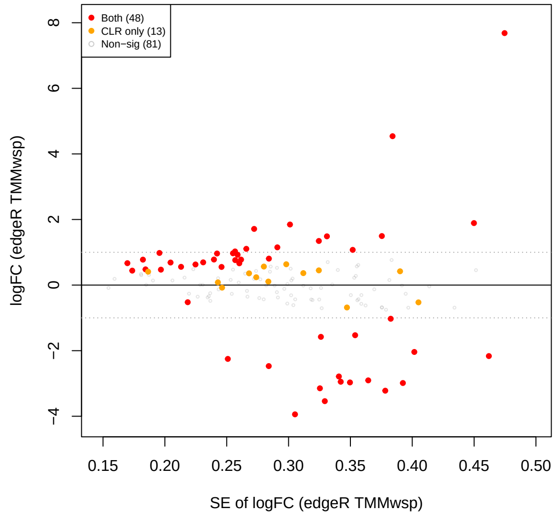
pup vs mage – edgeR TMMwsp FILTERED (218 OTUs, CLR sig ov
