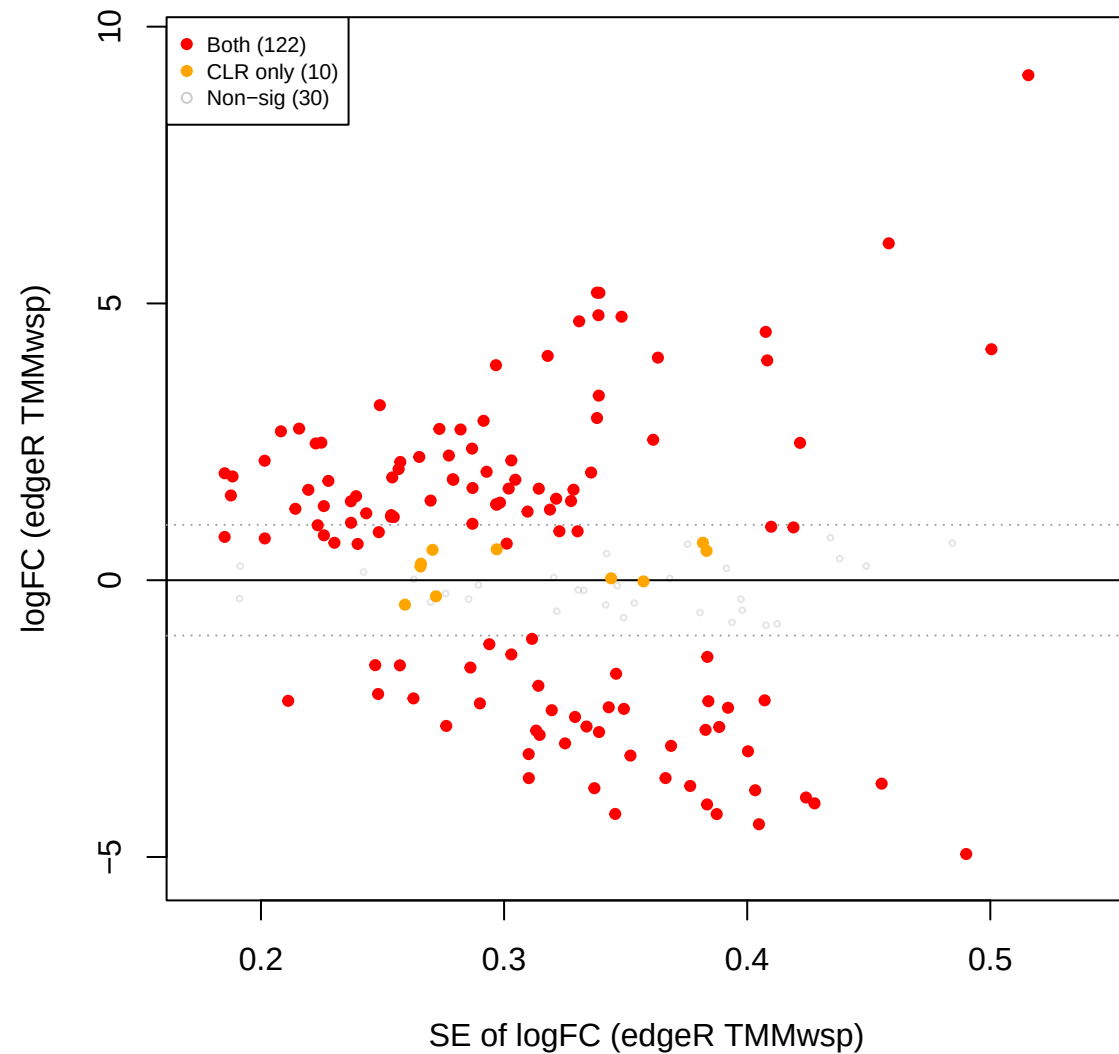
pup vs eld – edgeR TMMwsp FILTERED (220 OTUs, CLR sig over)
