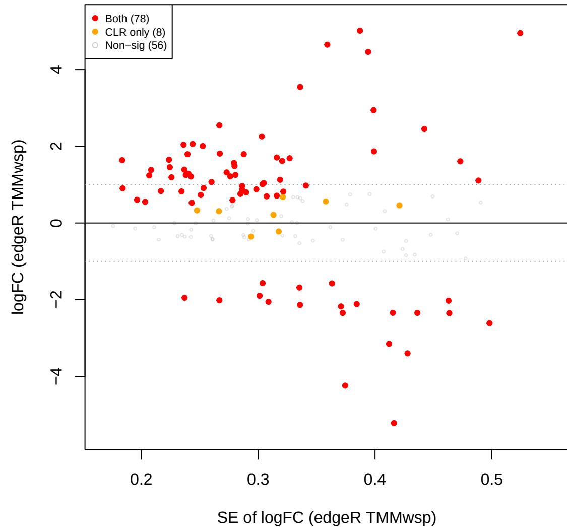
mid vs eld – edgeR TMMwsp FILTERED (209 OTUs, CLR sig over)
