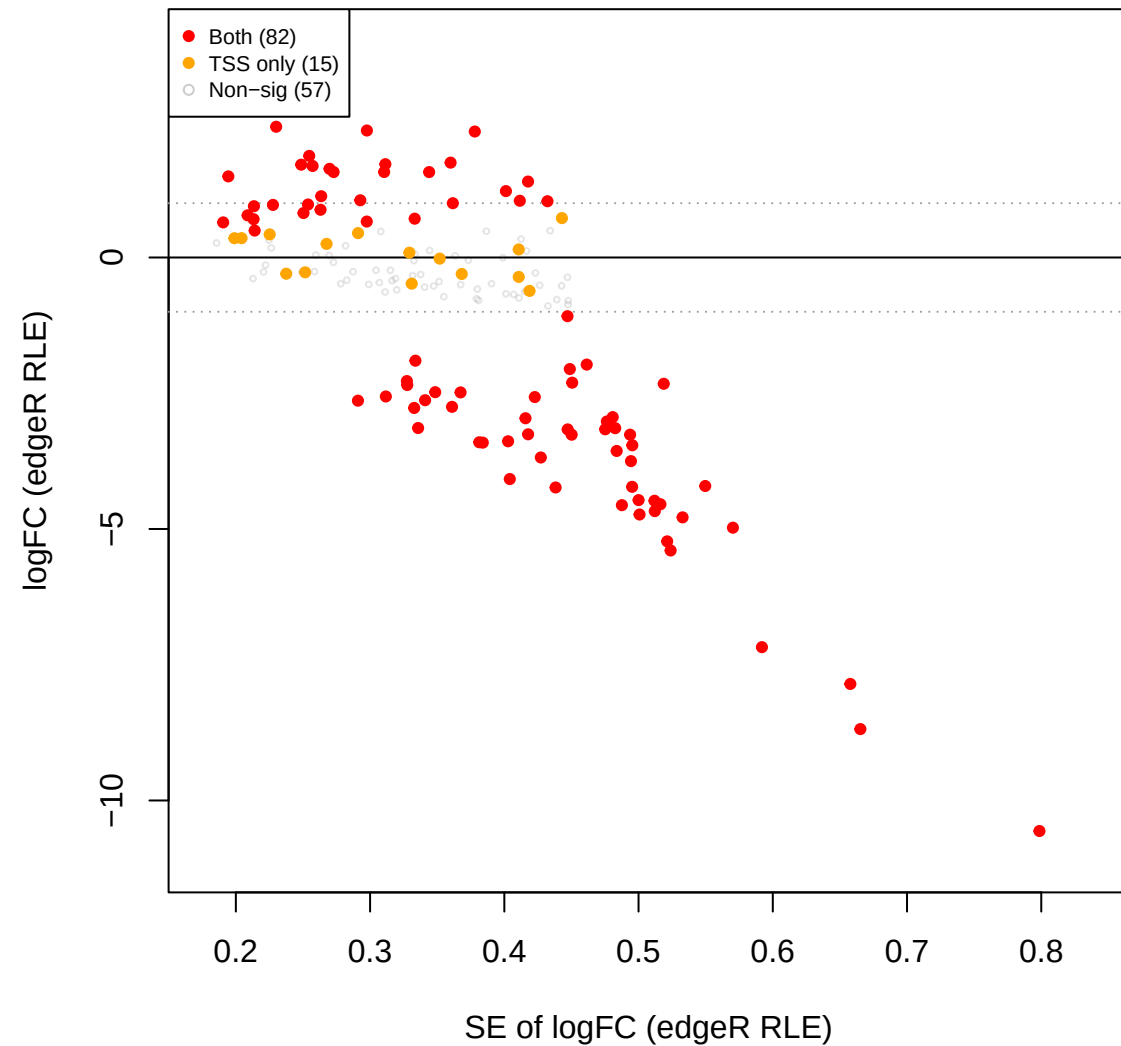
mage vs cent – edgeR RLE FILTERED (251 OTUs, TSS sig over
