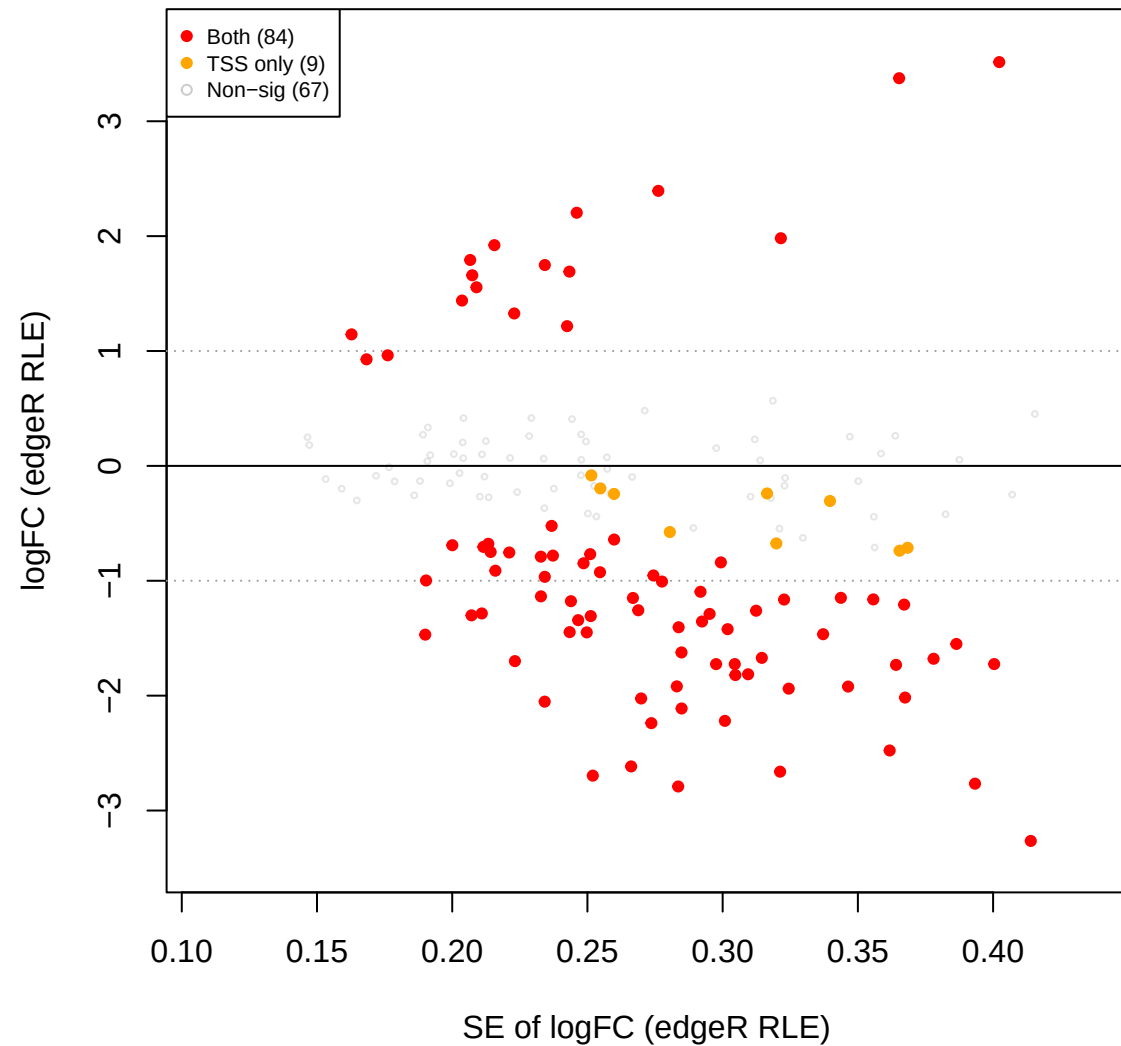
pup vs mid – edgeR RLE FILTERED (207 OTUs, TSS sig overlaid)
