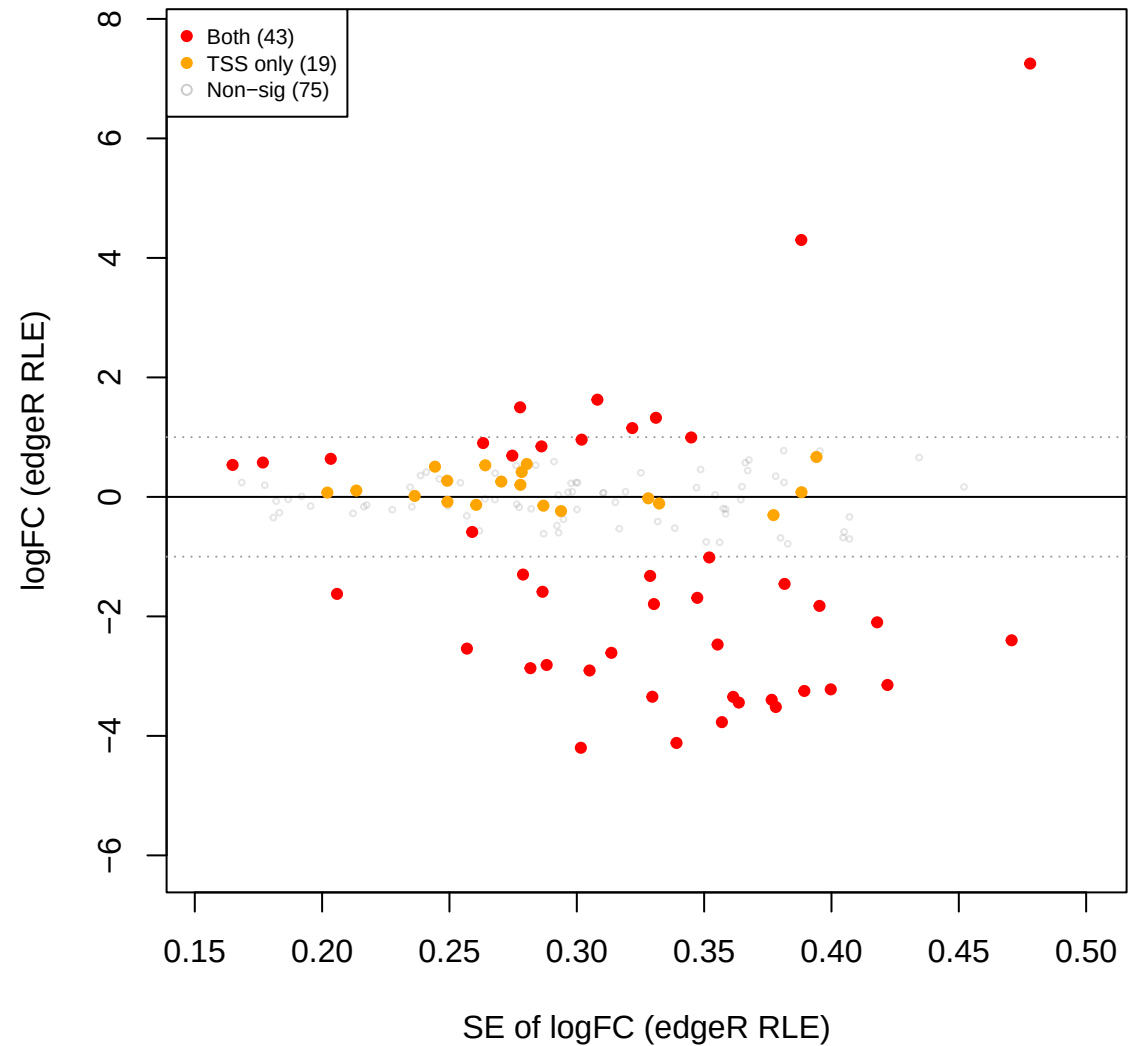
pup vs mage – edgeR RLE FILTERED (218 OTUs, TSS sig over
