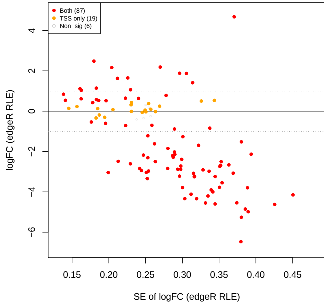
pup vs cent – edgeR RLE FILTERED (173 OTUs, TSS sig overl
