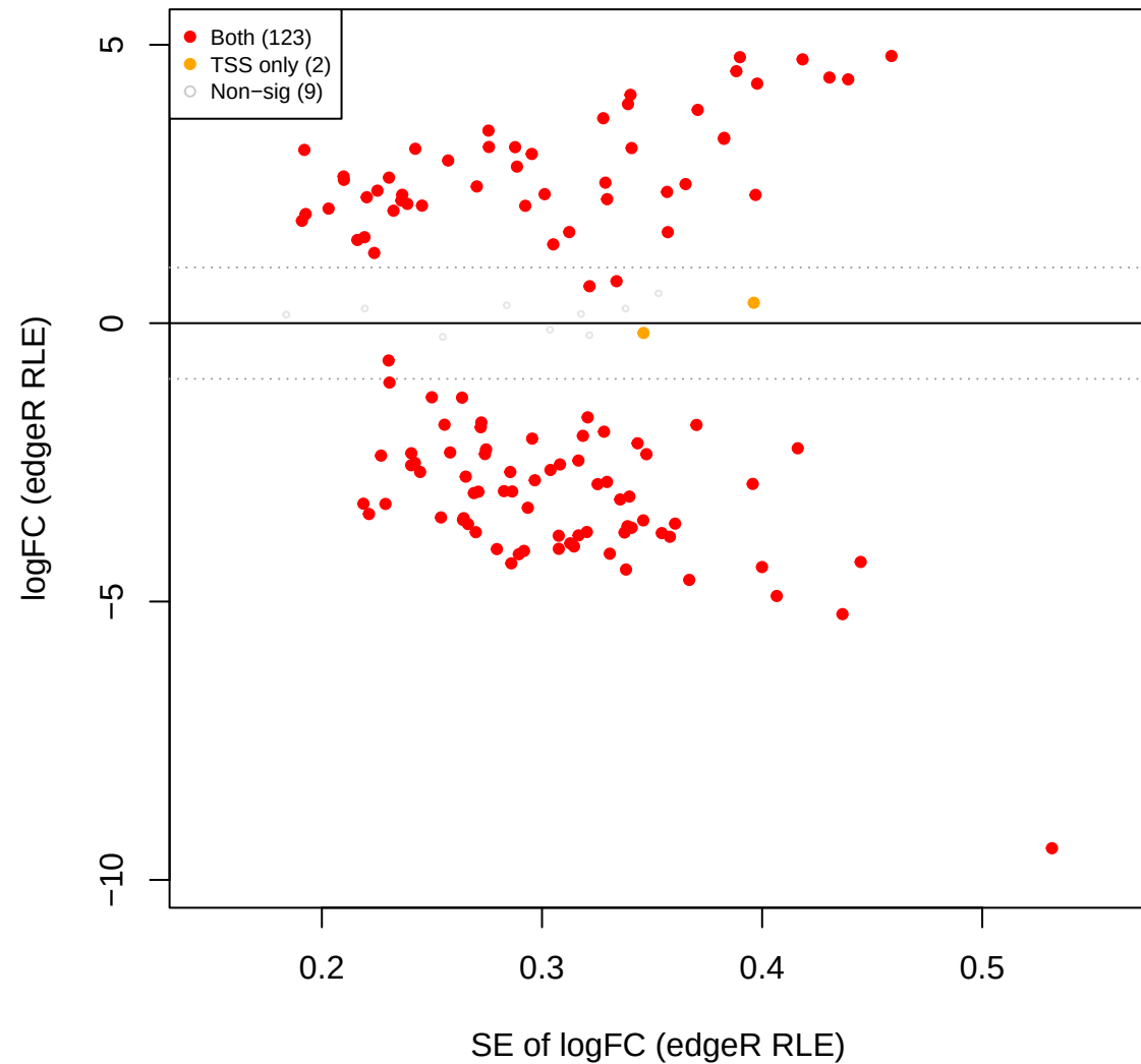
pup vs you – edgeR RLE FILTERED (165 OTUs, TSS sig overlaid)
