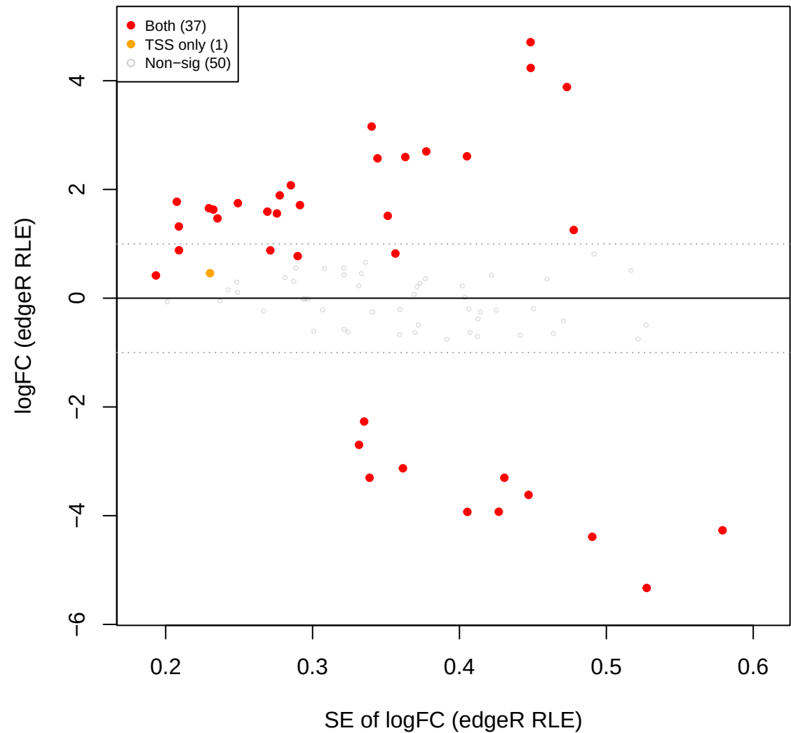
mage vs eld – edgeR RLE FILTERED (173 OTUs, TSS sig overlaid)
