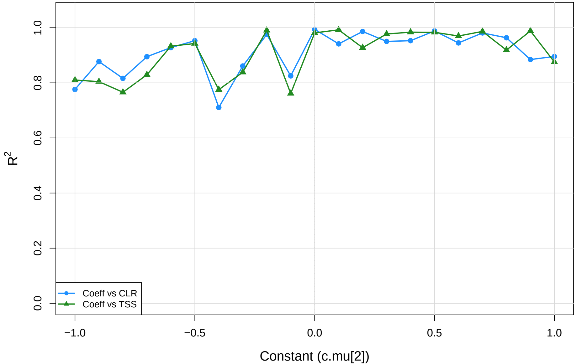
coeff.sm vs CLR vs TSS | eld vs kin | gamma=0.5 R-squared of red-dot regression
