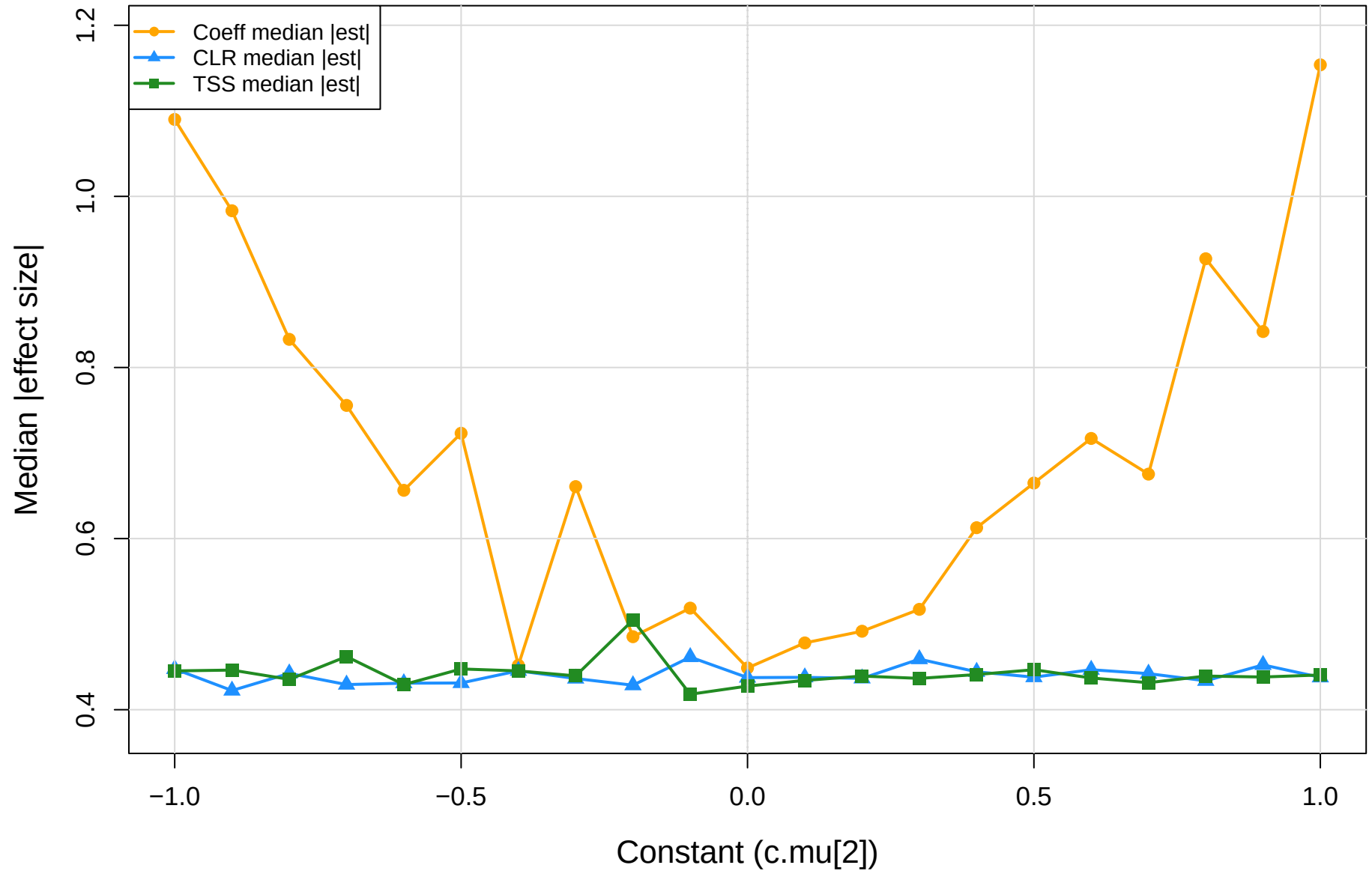
coeff.sm vs CLR vs TSS | eld vs kin | gamma=0.5 Median absolute effect size
