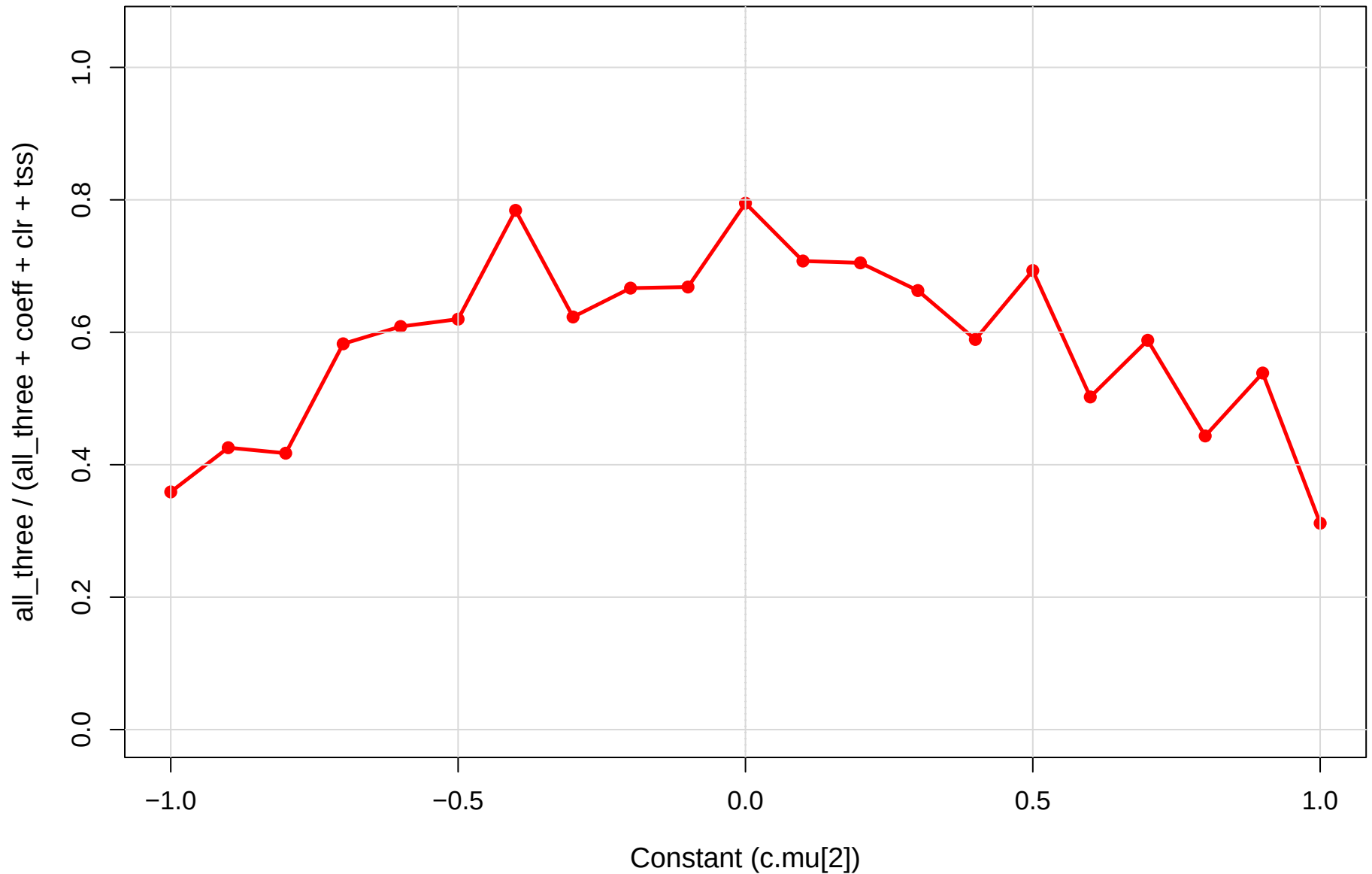
coeff.sm vs CLR vs TSS | eld vs kin | gamma=0.5 Robustness (1 = all agree, 0 = max disagreement)
