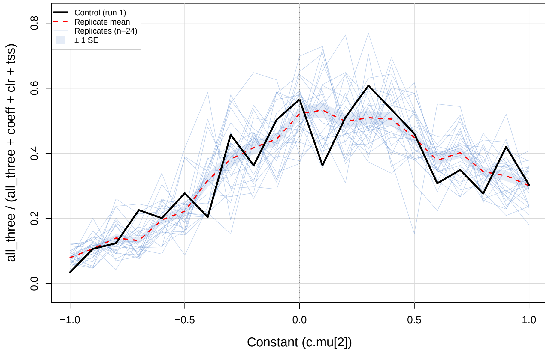
coefficient.sm vs CLR(std) vs TSS – cent_vs_mage (gamma=0.5) Robustness (1 = all agree, 0 = max disagreement)
