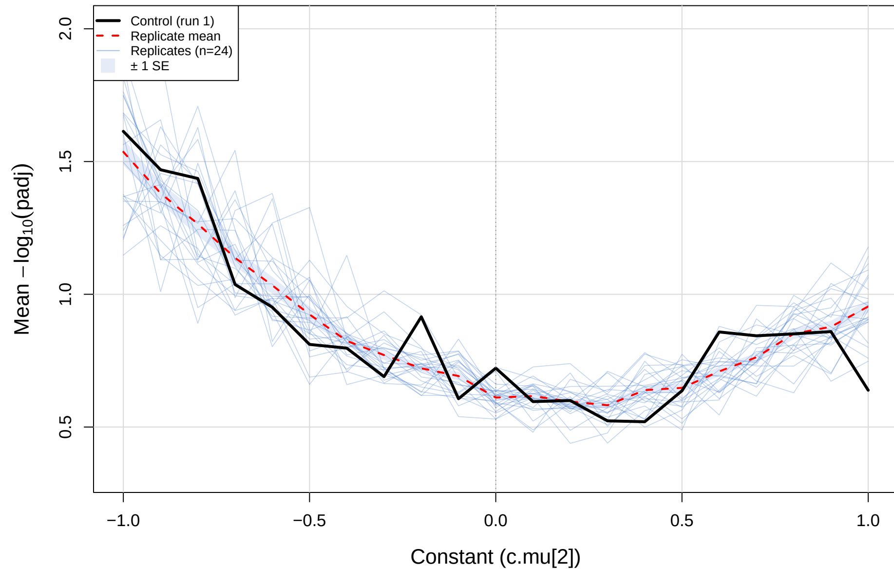
coefficient.sm vs CLR(std) vs TSS – cent_vs_mage (gamma=0.5) Mean -\log_{10}(\text{padj}) coefficient model
