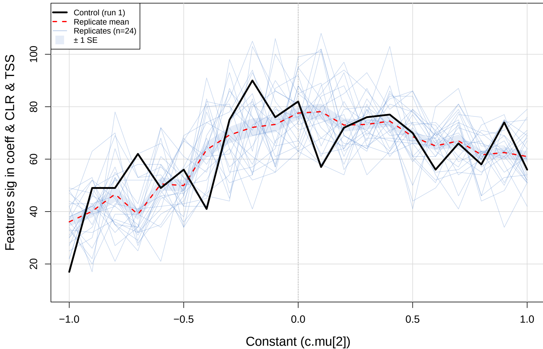
coefficient.sm vs CLR(std) vs TSS – cent_vs_mage (gamma=0.5) Three-way agreement count
