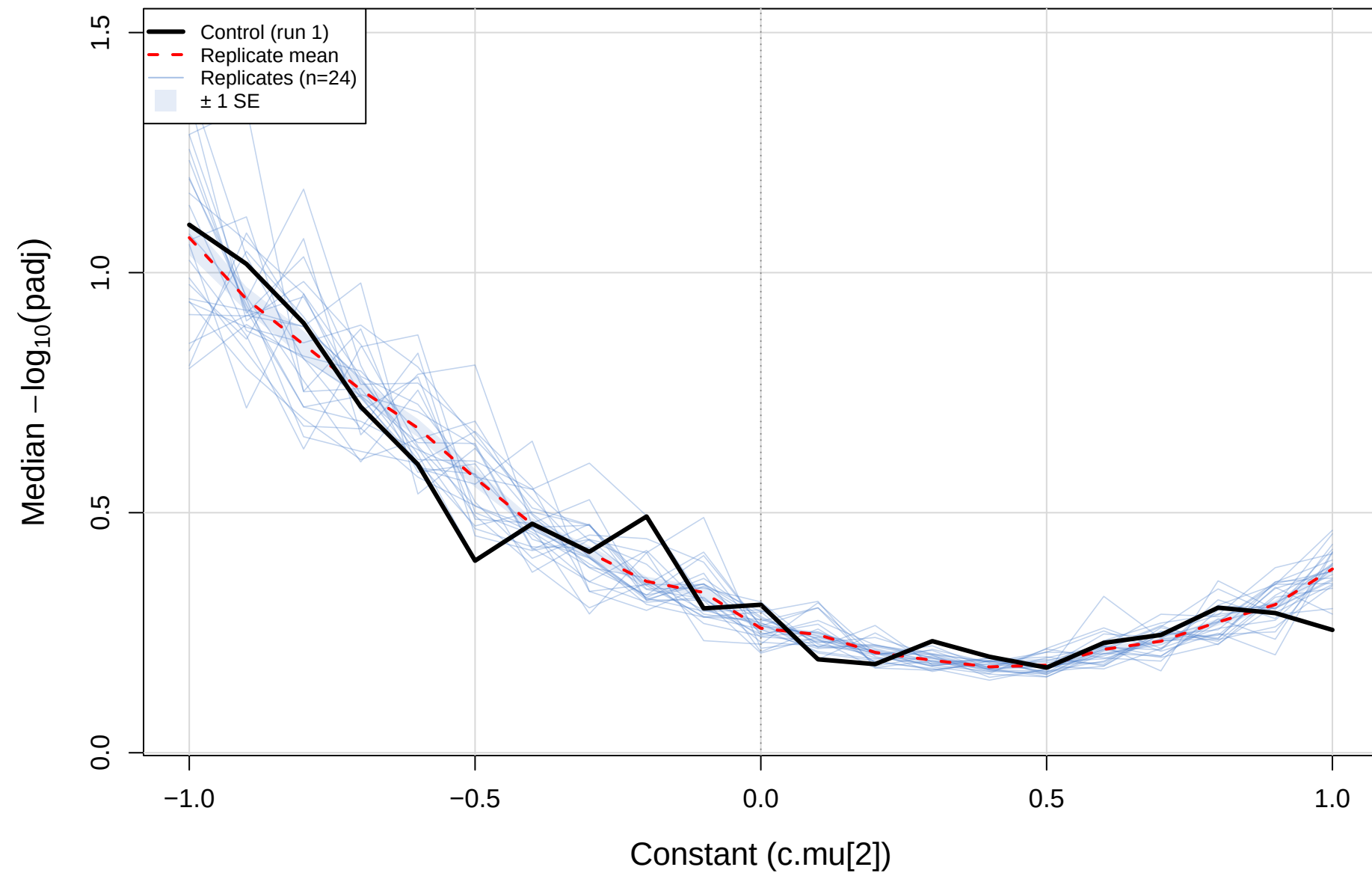
coefficient.sm vs CLR(std) vs TSS – cent_vs_mage (gamma=0.5) Median -\log_{10}(\text{padj}) coefficient model
