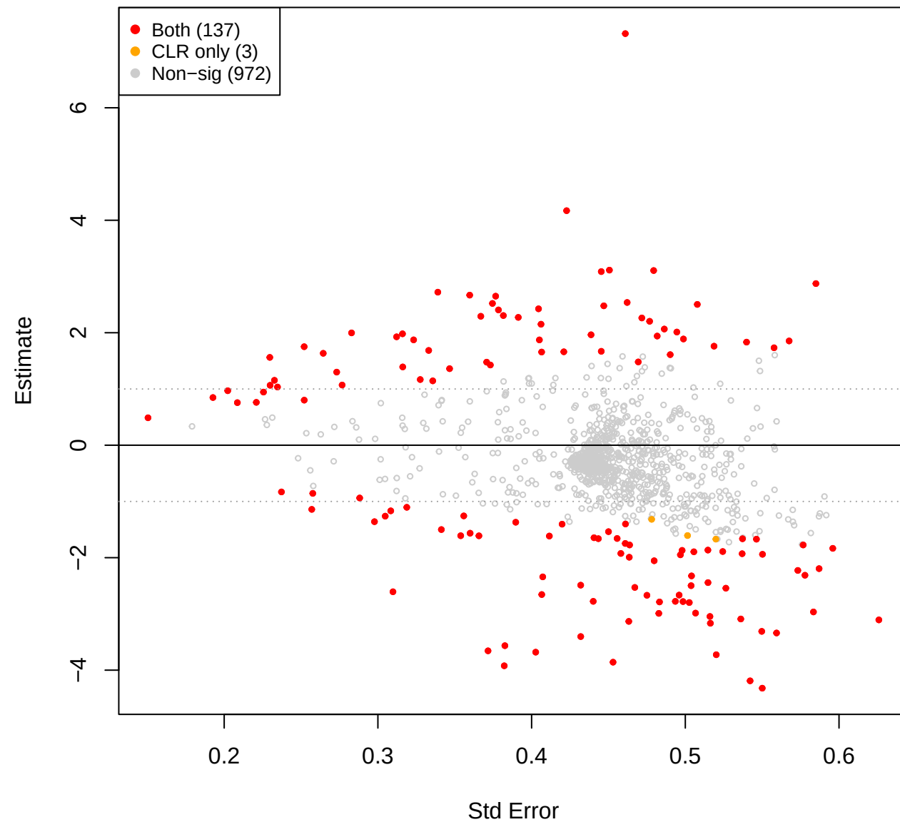
mage vs pup – TSS (CLR(const=0) sig overlay)
