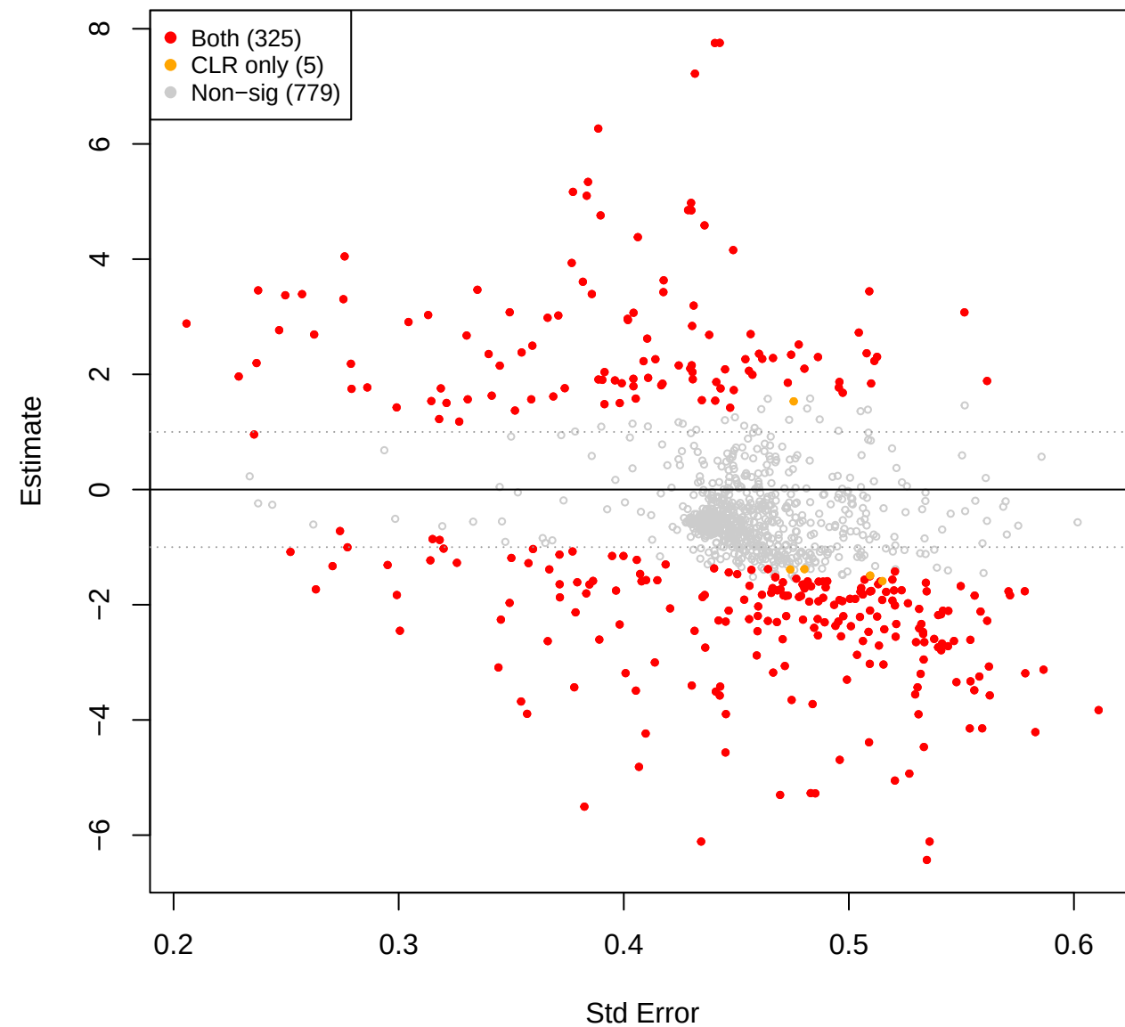
eld vs pup – TSS (CLR(const=0) sig overlay)
