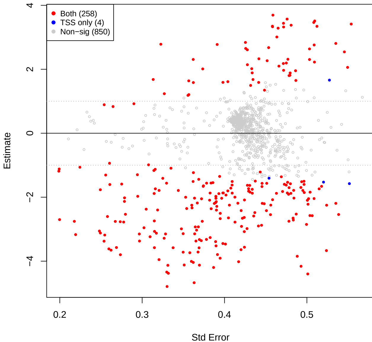
mid vs you – CLR(const=0) (TSS sig overlay)
