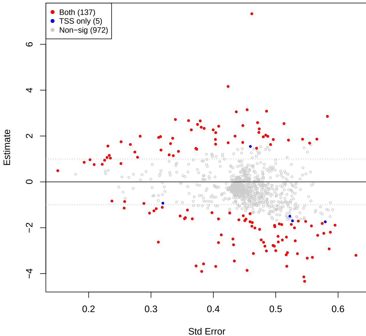
mage vs pup – CLR(const=0) (TSS sig overlay)
