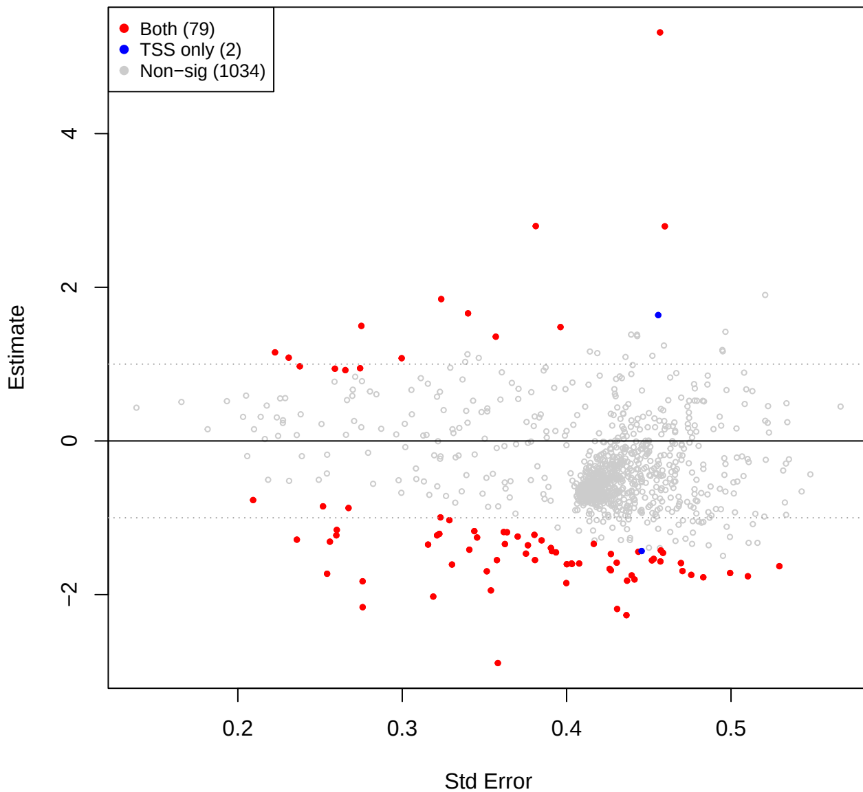
kin vs pup – CLR(const=0) (TSS sig overlay)
