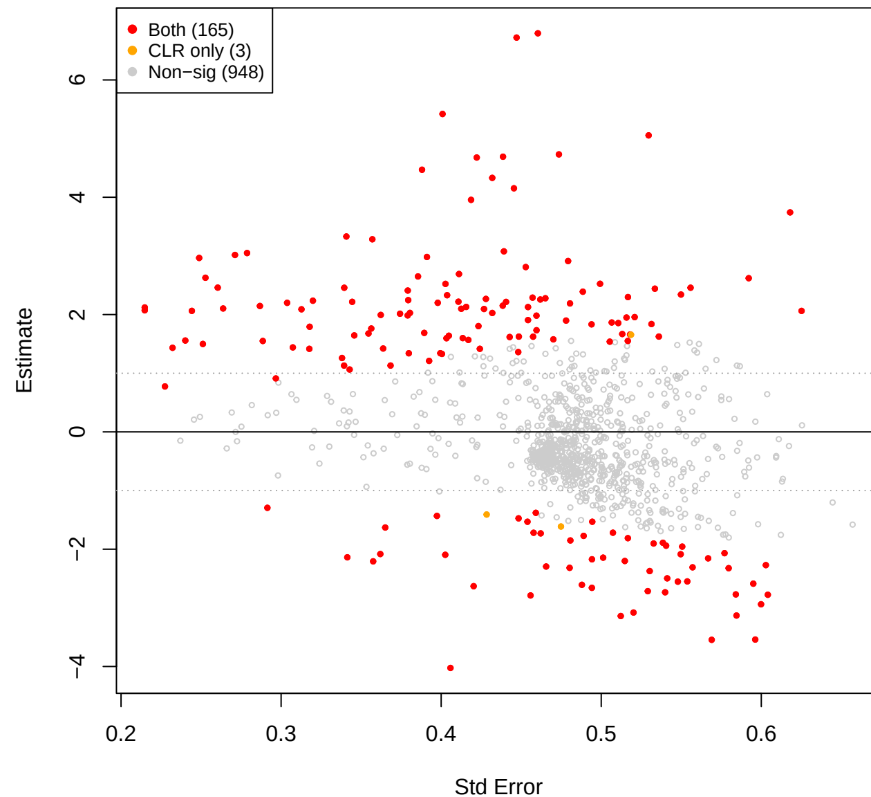
eld vs mid – TSS (CLR(const=0) sig overlay)
