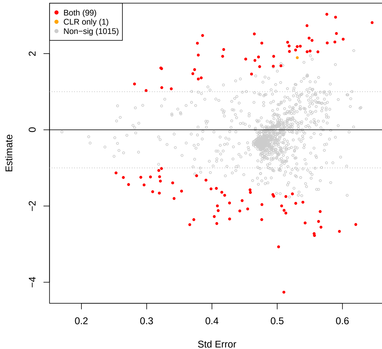
kin vs mage - TSS (CLR(const=0) sig overlay)
