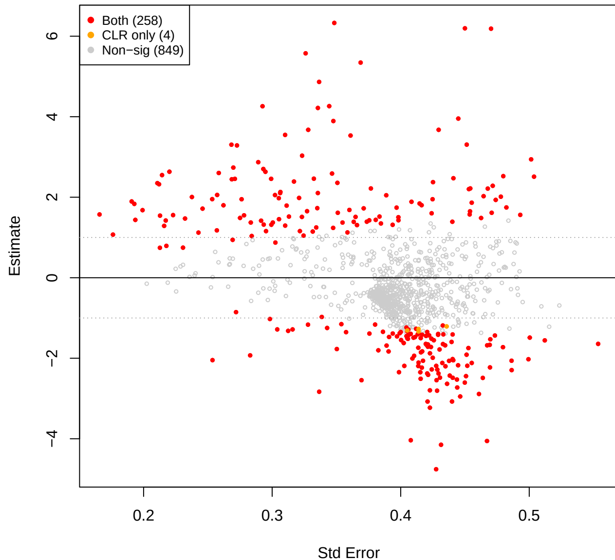
cent vs mid – TSS (CLR(const=0) sig overlay)
