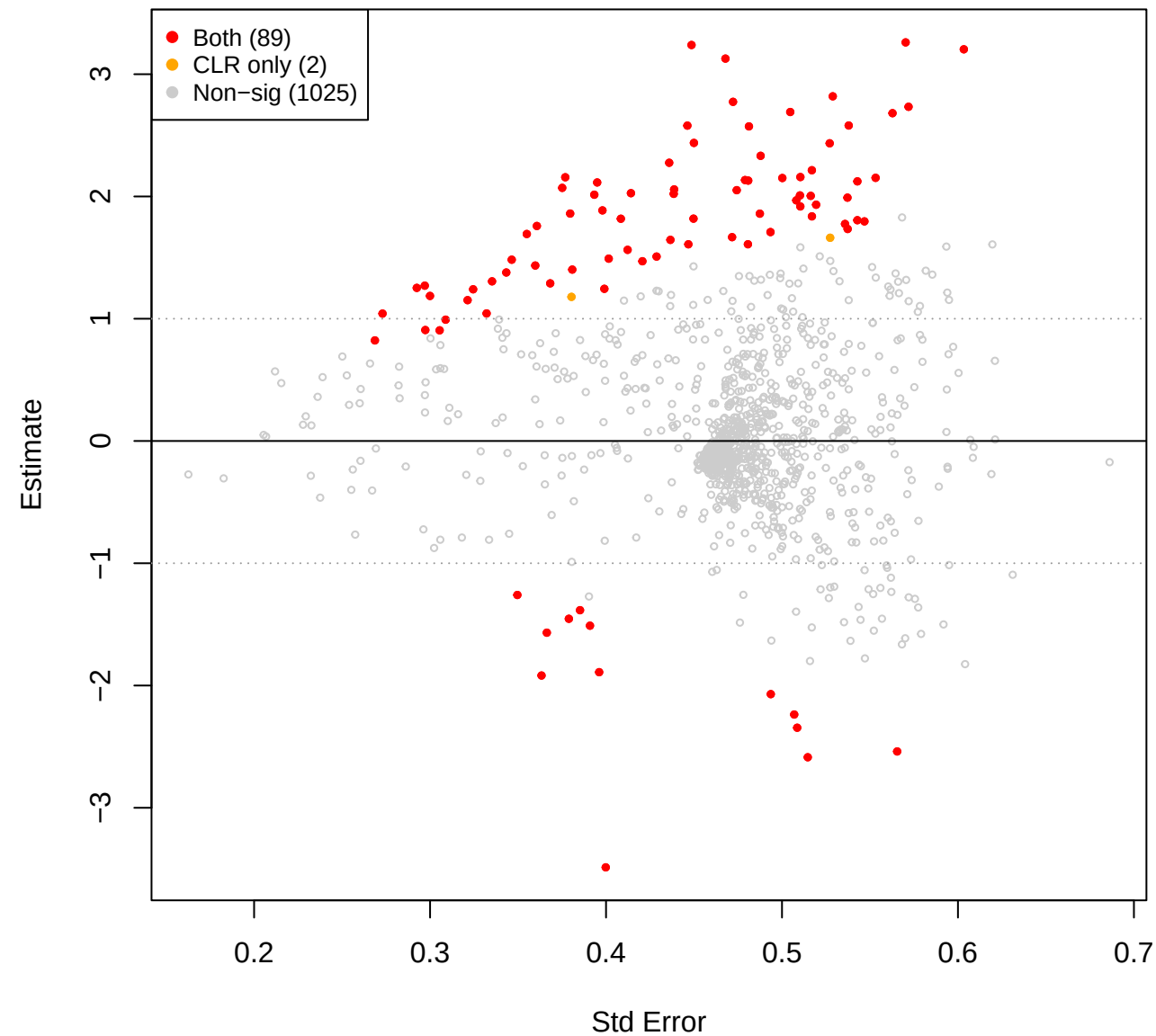
mage vs mid – TSS (CLR(const=0) sig overlay)
