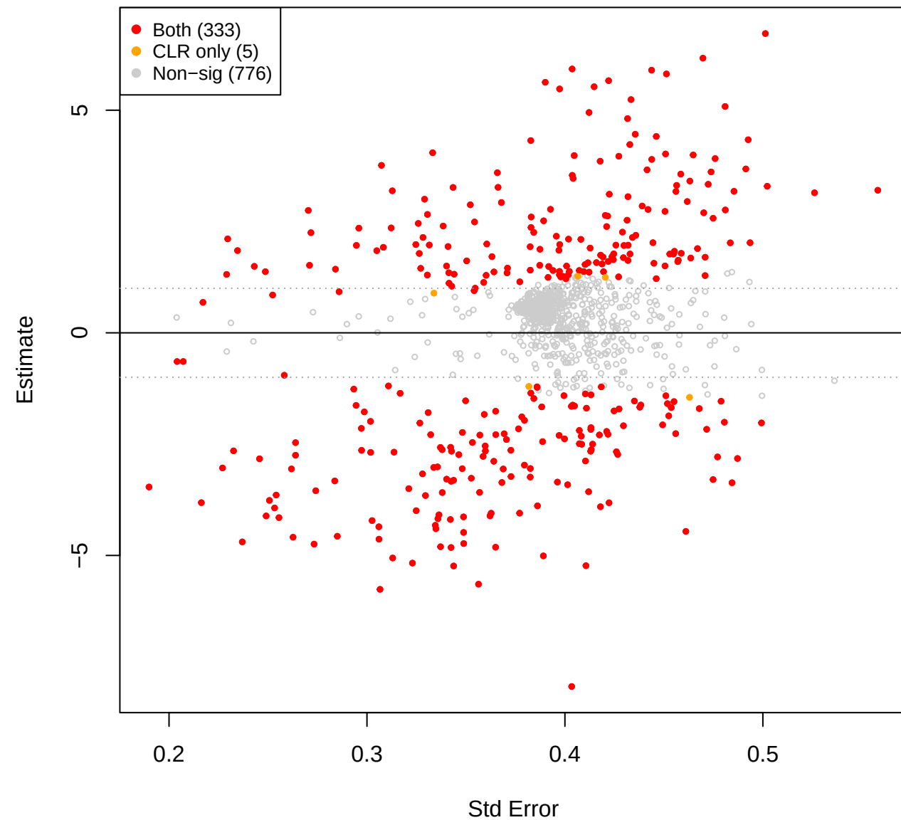
pup vs you – TSS (CLR(const=0) sig overlay)
