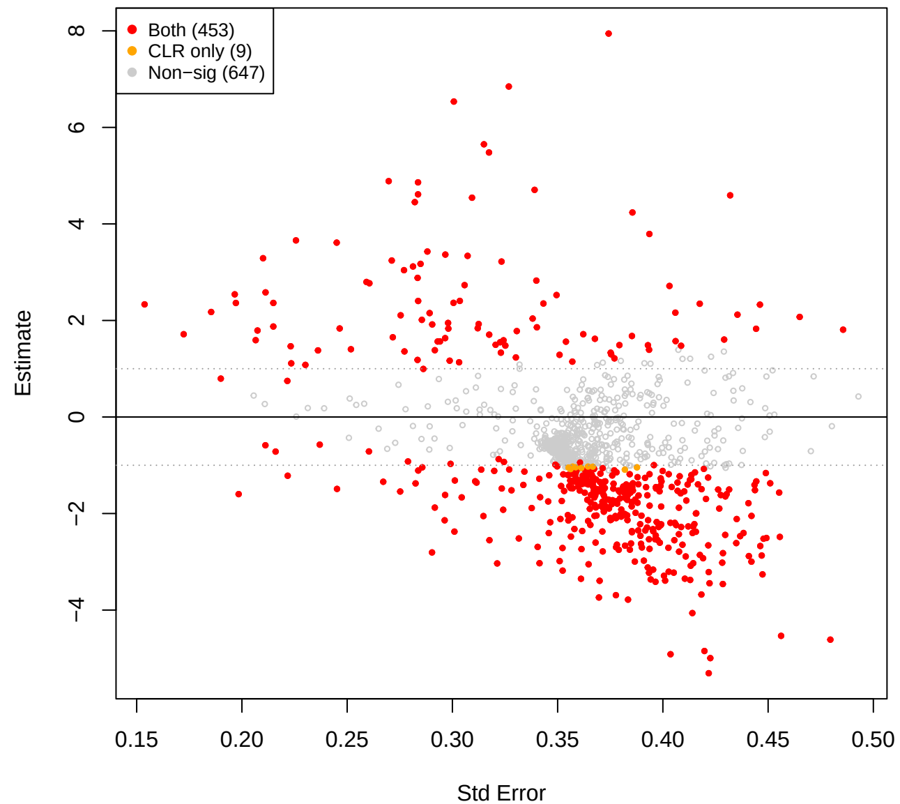
cent vs pup – TSS (CLR(const=0) sig overlay)
