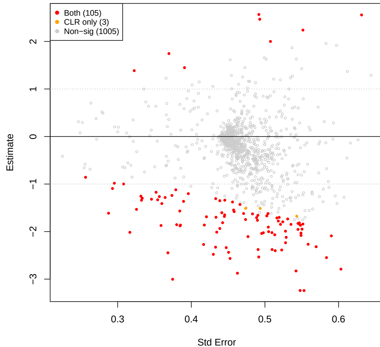
eld vs you - TSS (CLR(const=0) sig overlay)
