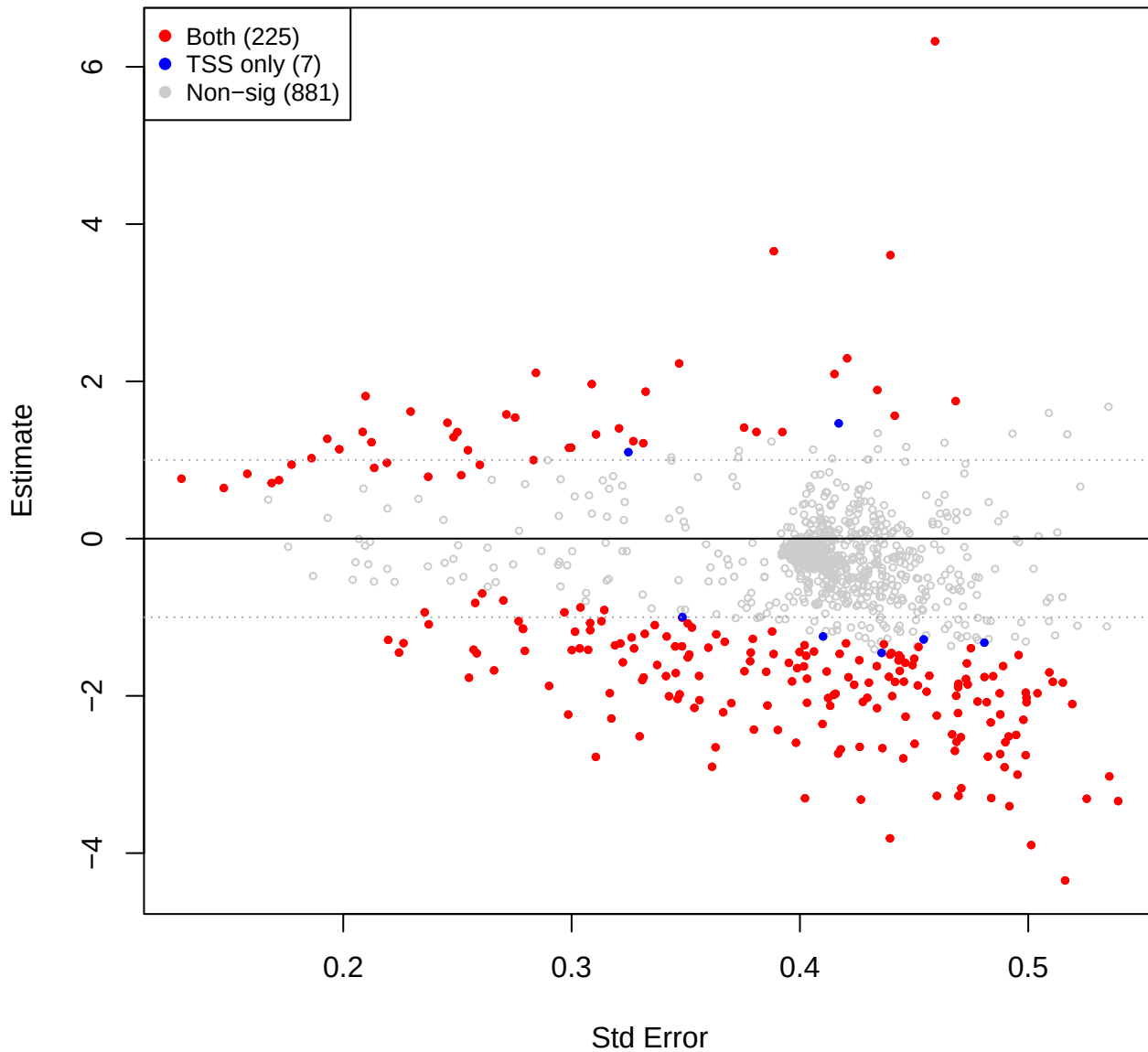
mid vs pup – CLR(const=0) (TSS sig overlay)
