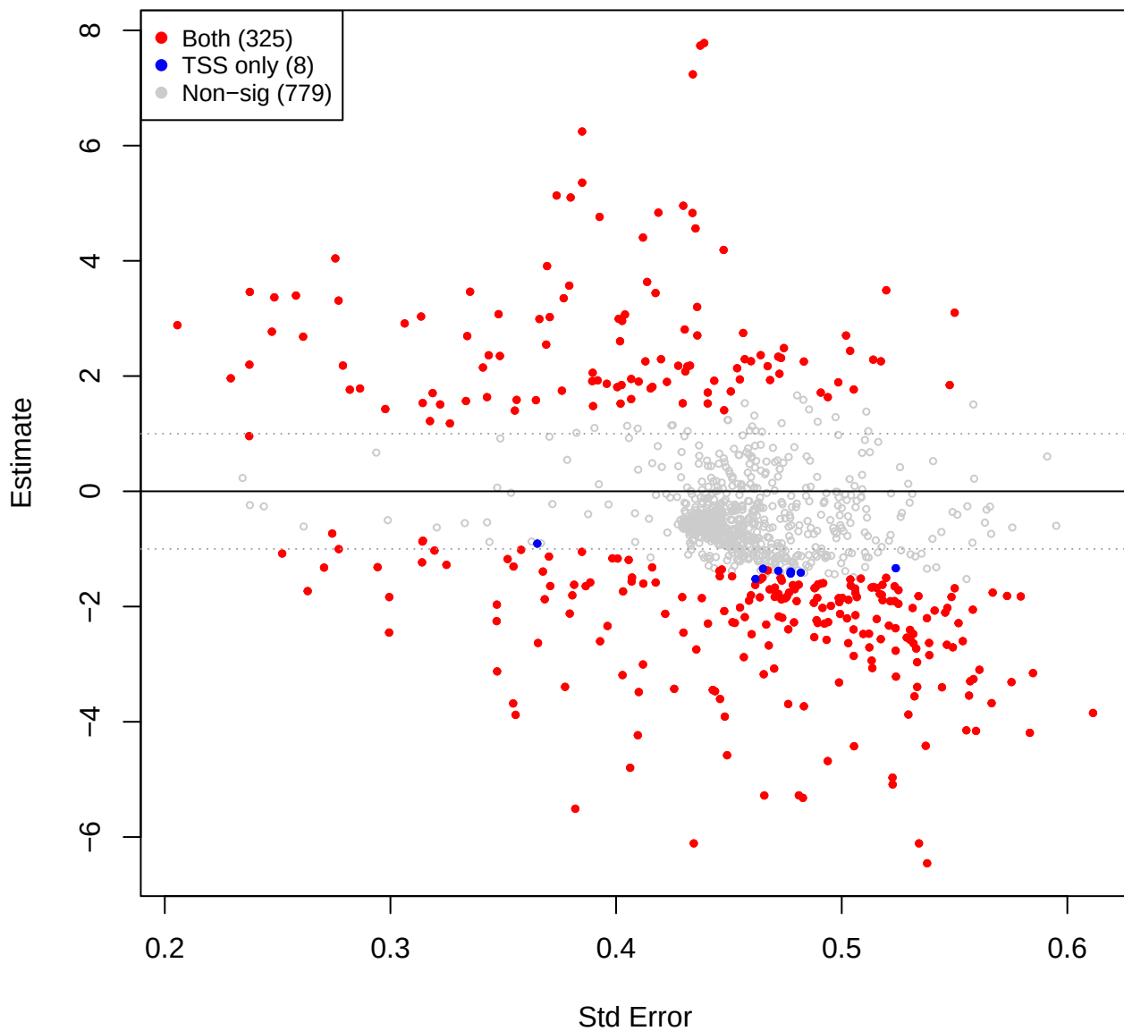
eld vs pup – CLR(const=0) (TSS sig overlay)
