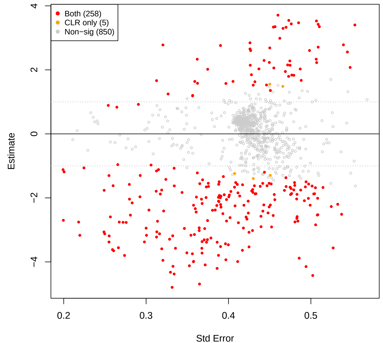
mid vs you – TSS (CLR(const=0) sig overlay)
