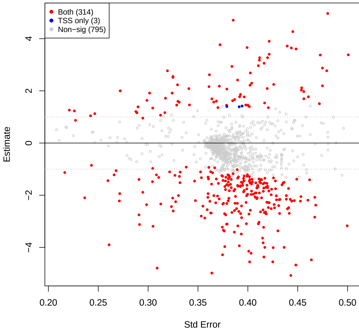
cent vs you – CLR(const=0) (TSS sig overlay)
