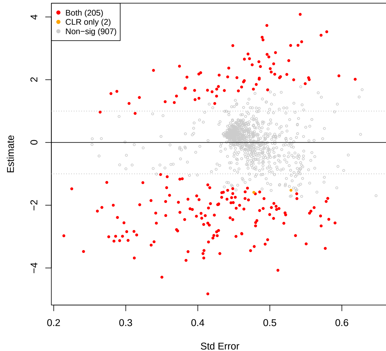
mage vs you – TSS (CLR(const=0) sig overlay)
