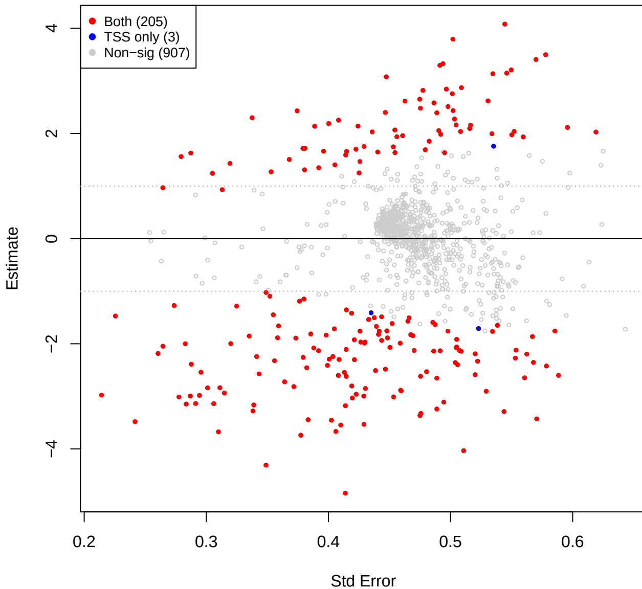
mage vs you – CLR(const=0) (TSS sig overlay)
