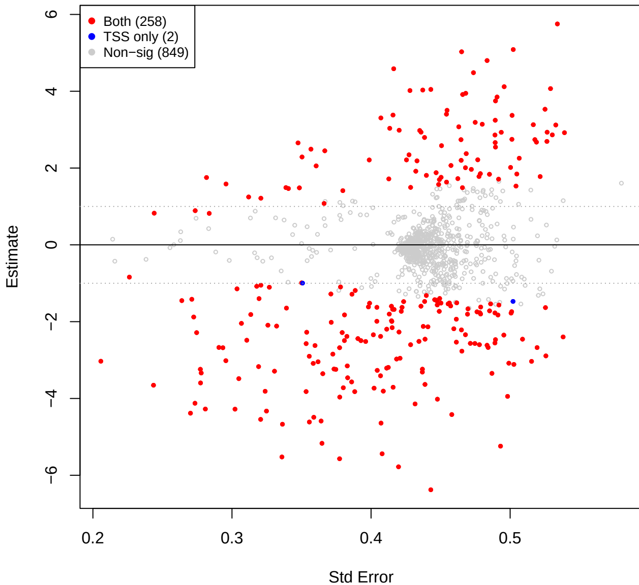
kin vs you – CLR(const=0) (TSS sig overlay)
