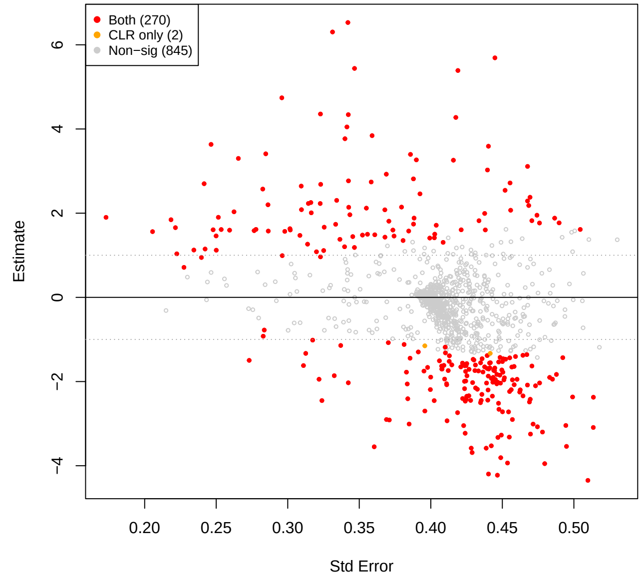
cent vs kin – TSS (CLR(const=0) sig overlay)
