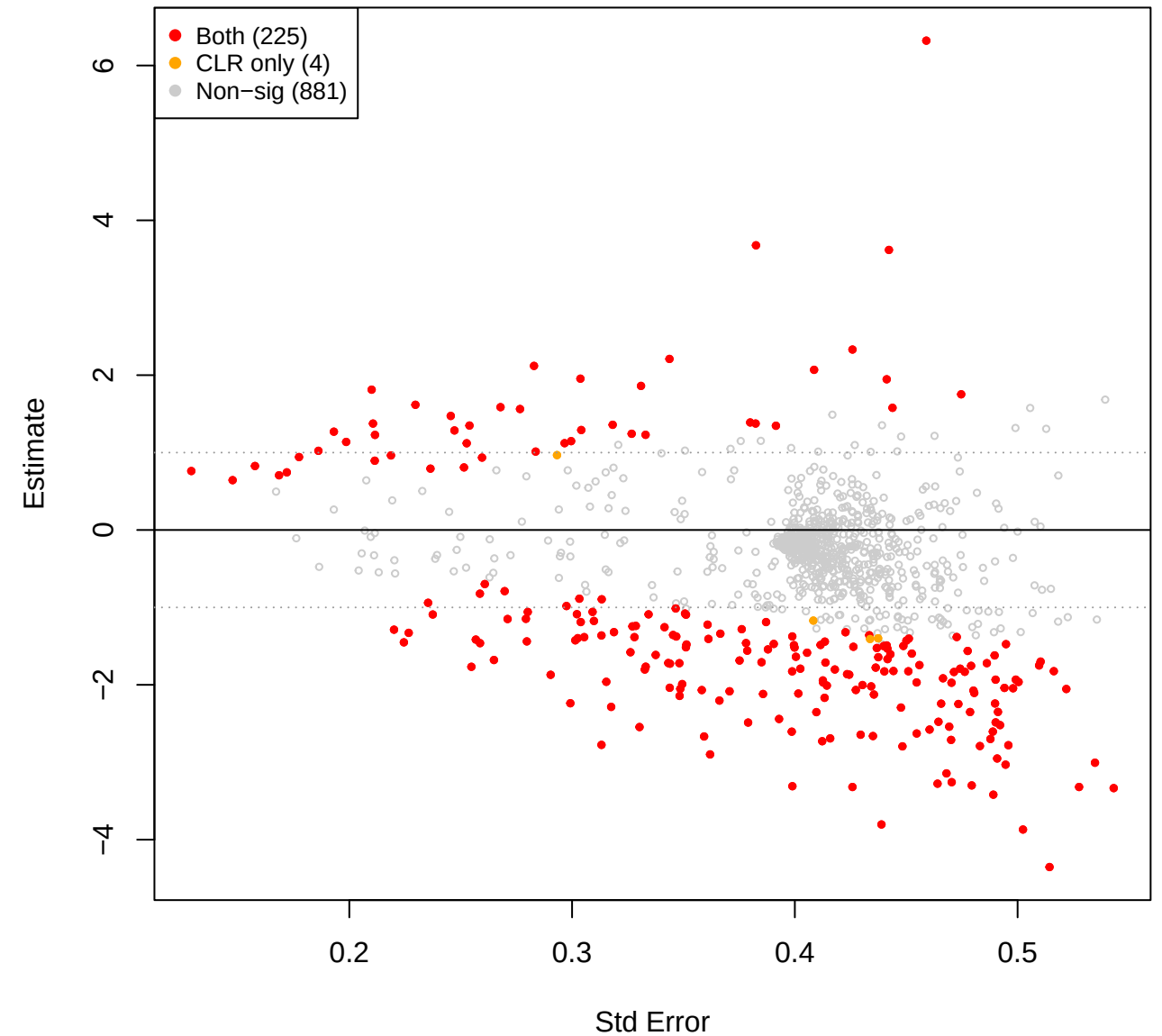
mid vs pup – TSS (CLR(const=0) sig overlay)
