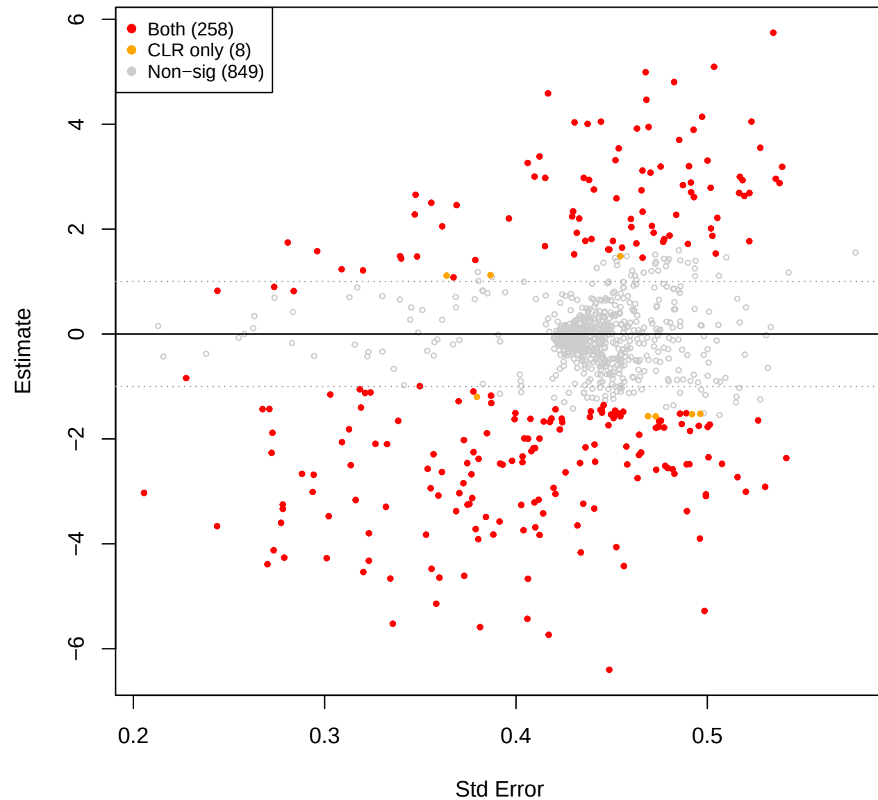
kin vs you – TSS (CLR(const=0) sig overlay)
