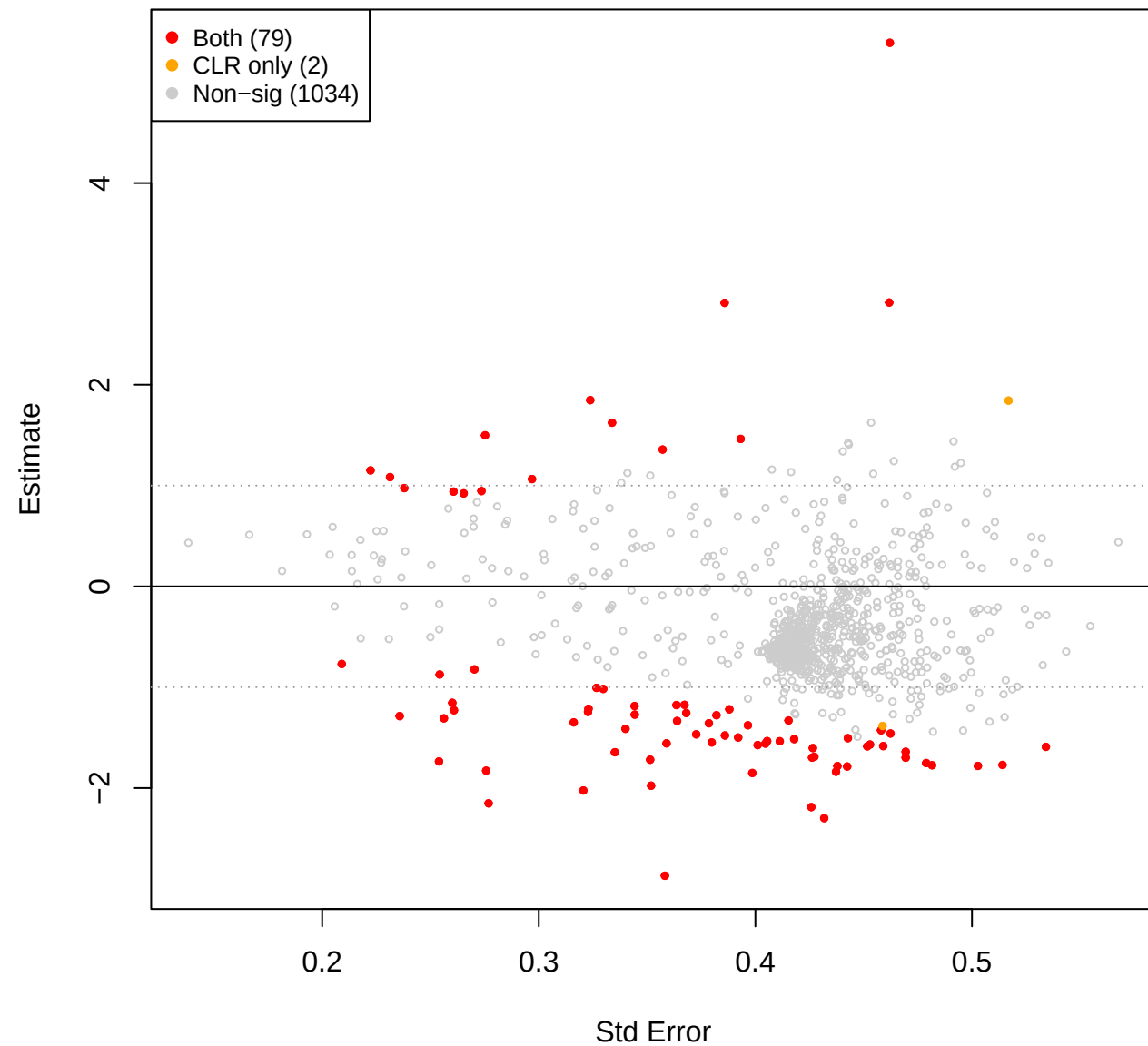
kin vs pup – TSS (CLR(const=0) sig overlay)
