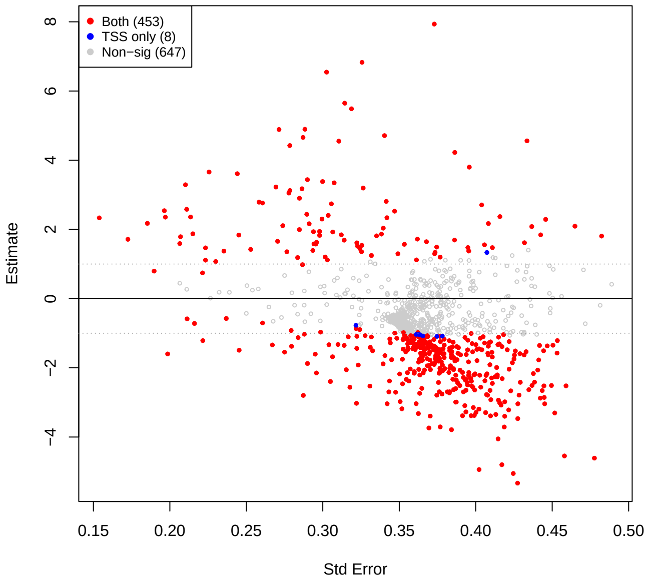
cent vs pup – CLR(const=0) (TSS sig overlay)
