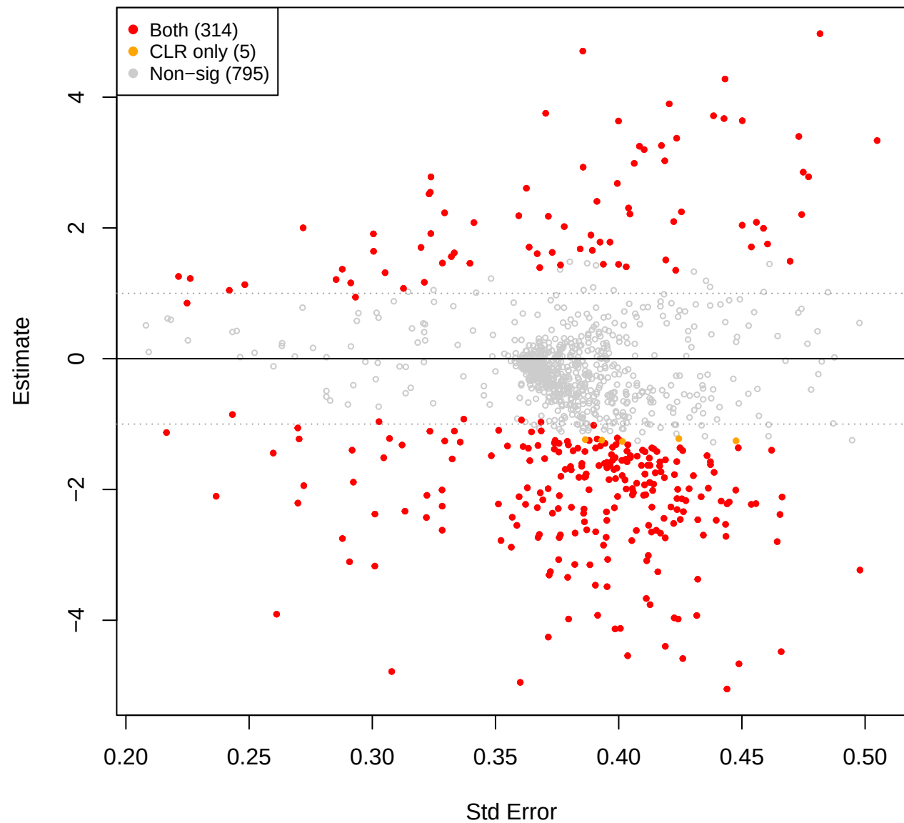
cent vs you – TSS (CLR(const=0) sig overlay)
