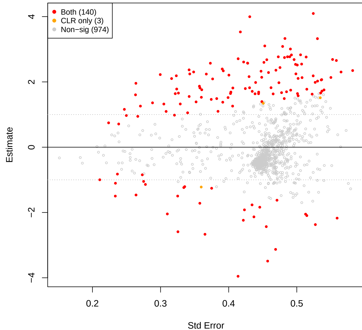
kin vs mid – TSS (CLR(const=0) sig overlay)
