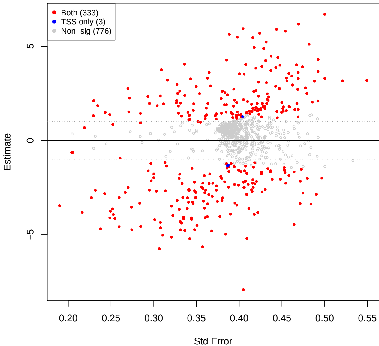
pup vs you – CLR(const=0) (TSS sig overlay)
