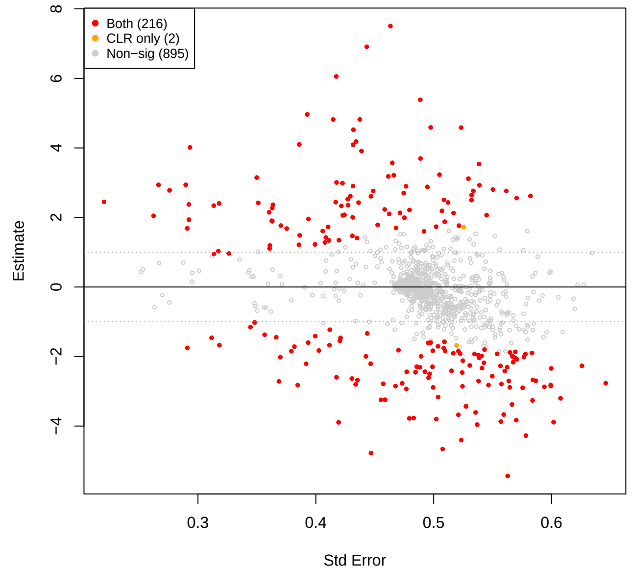
eld vs kin – TSS (CLR(const=0) sig overlay)
