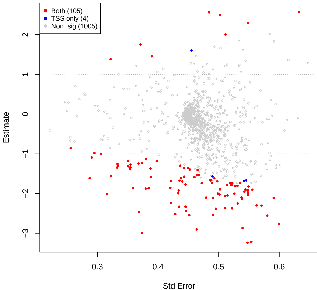
eld vs you - CLR(const=0) (TSS sig overlay)
