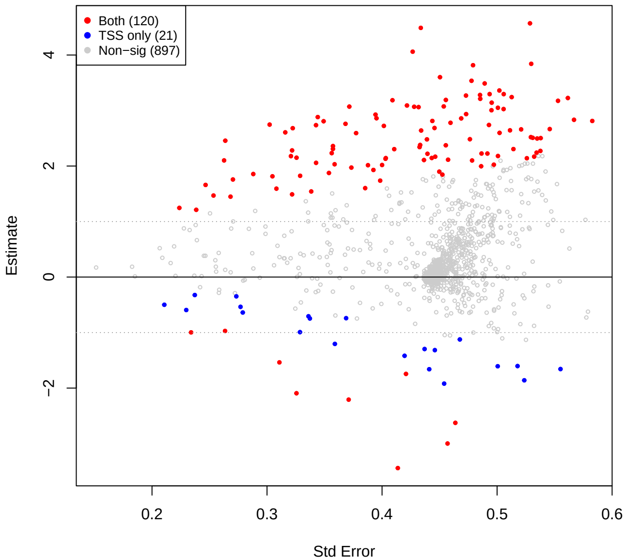
kin vs mid - CLR(const=0.5) (TSS sig overlay)
