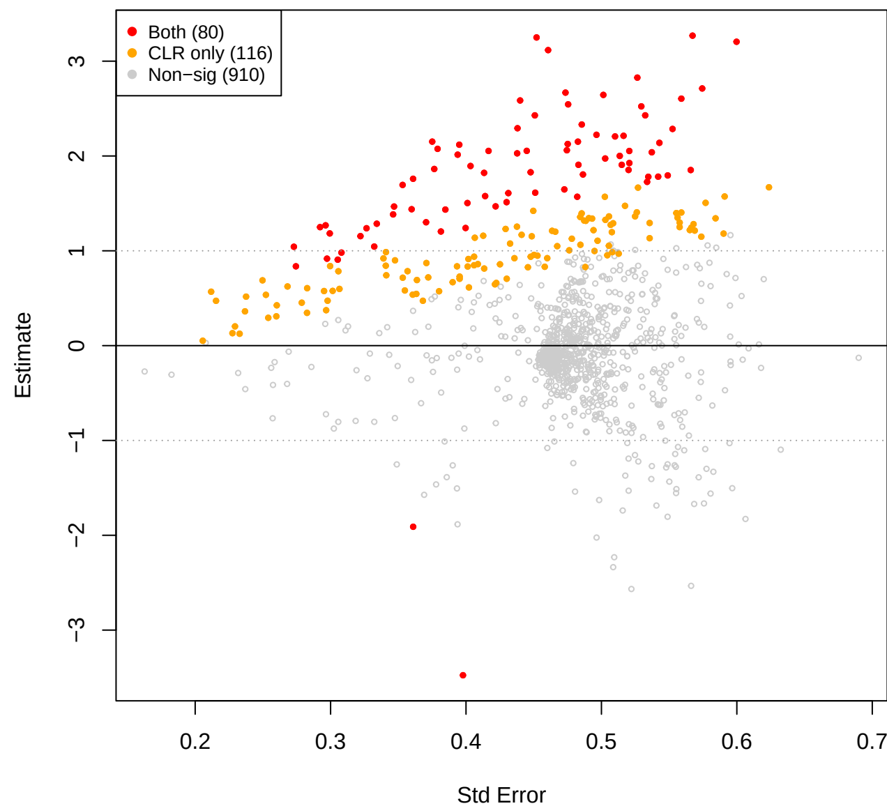
mage vs mid – TSS (CLR(const=0.5) sig overlay)
