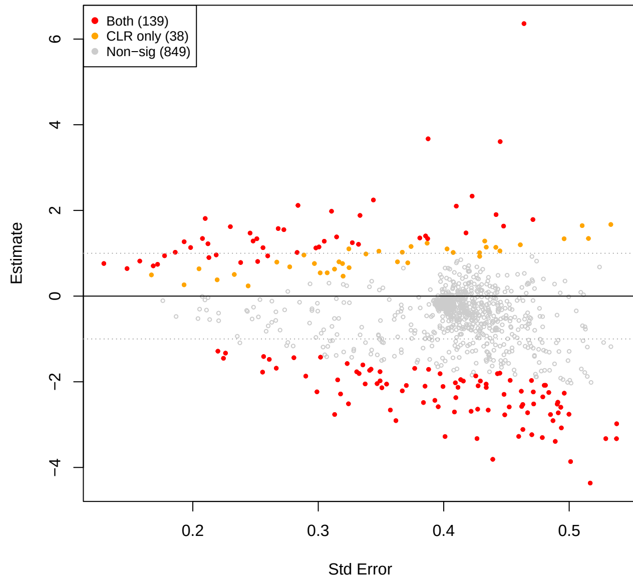
mid vs pup – TSS (CLR(const=0.5) sig overlay)
