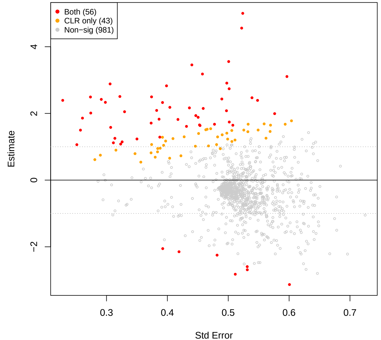
eld vs mage - TSS (CLR(const=0.5) sig overlay)
