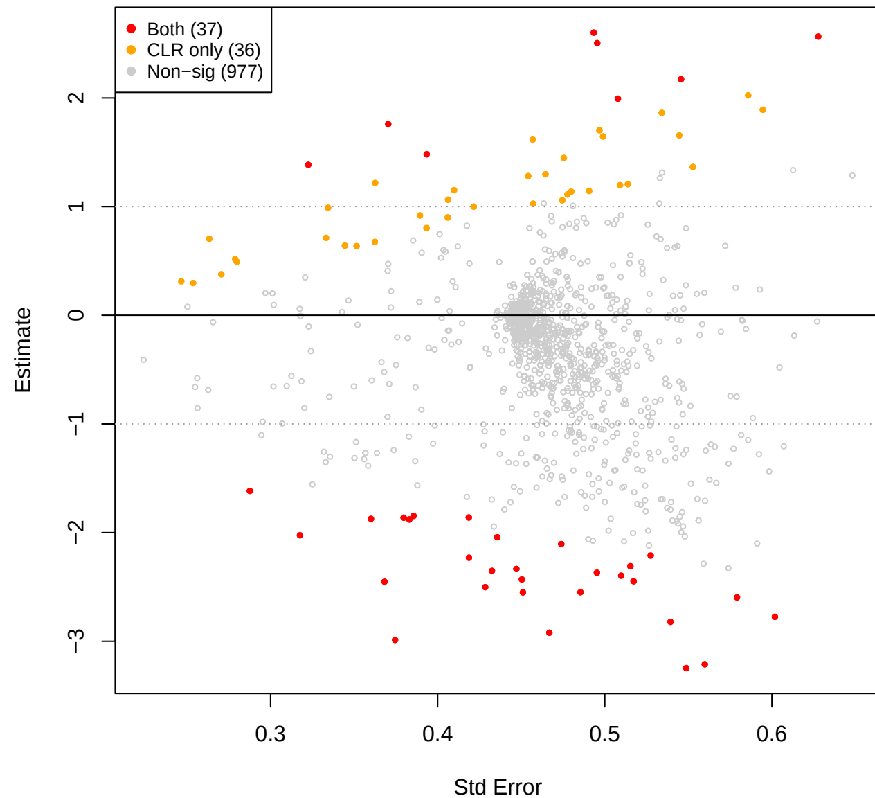
eld vs you – TSS (CLR(const=0.5) sig overlay)
