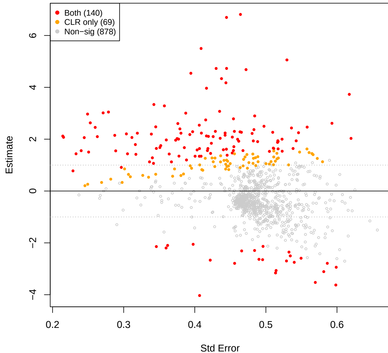
eld vs mid - TSS (CLR(const=0.5) sig overlay)
