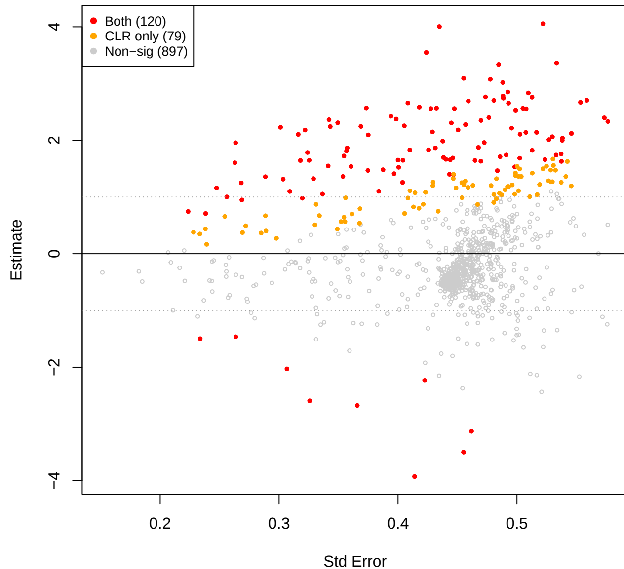
kin vs mid - TSS (CLR(const=0.5) sig overlay)
