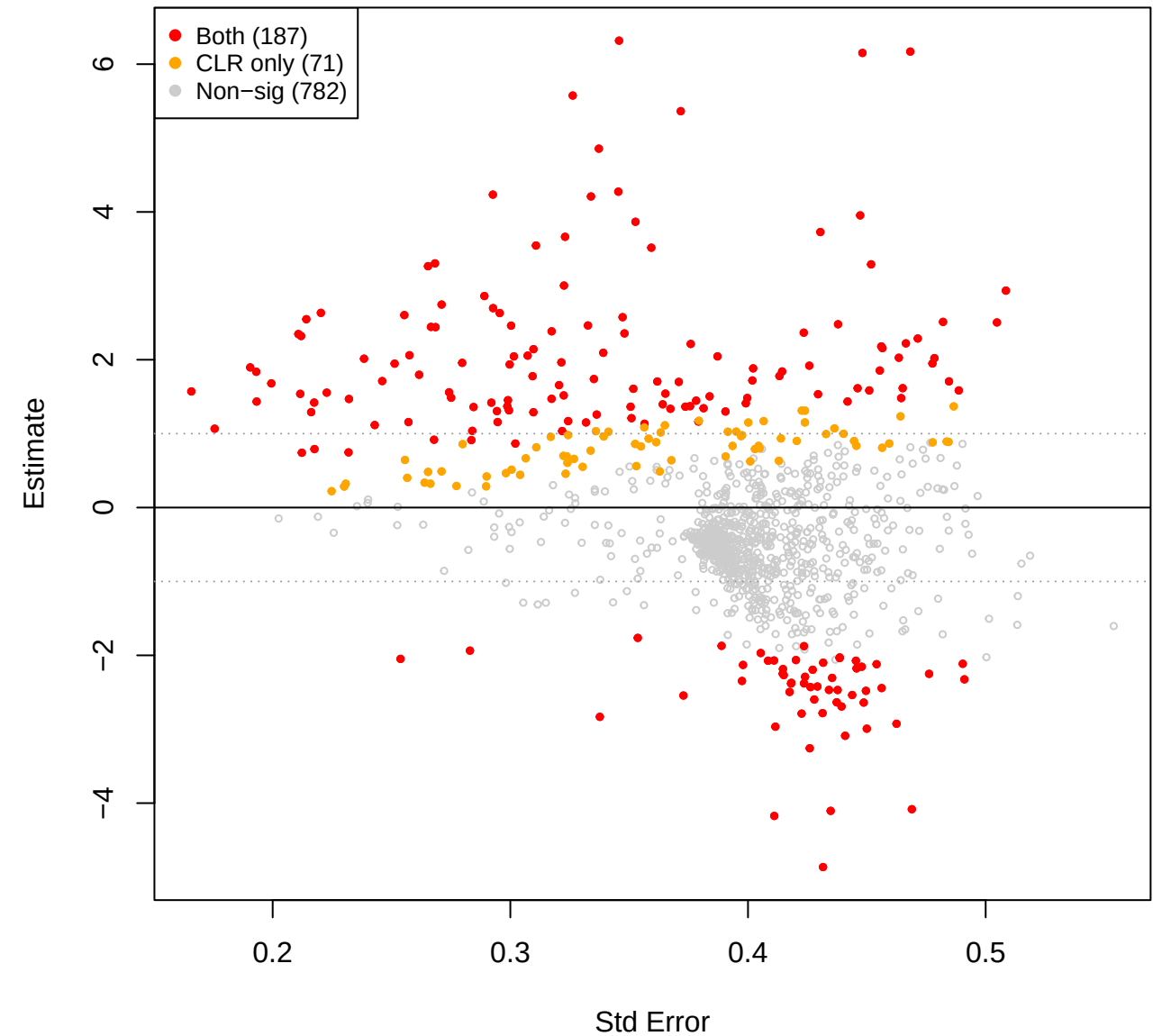
cent vs mid – TSS (CLR(const=0.5) sig overlay)
