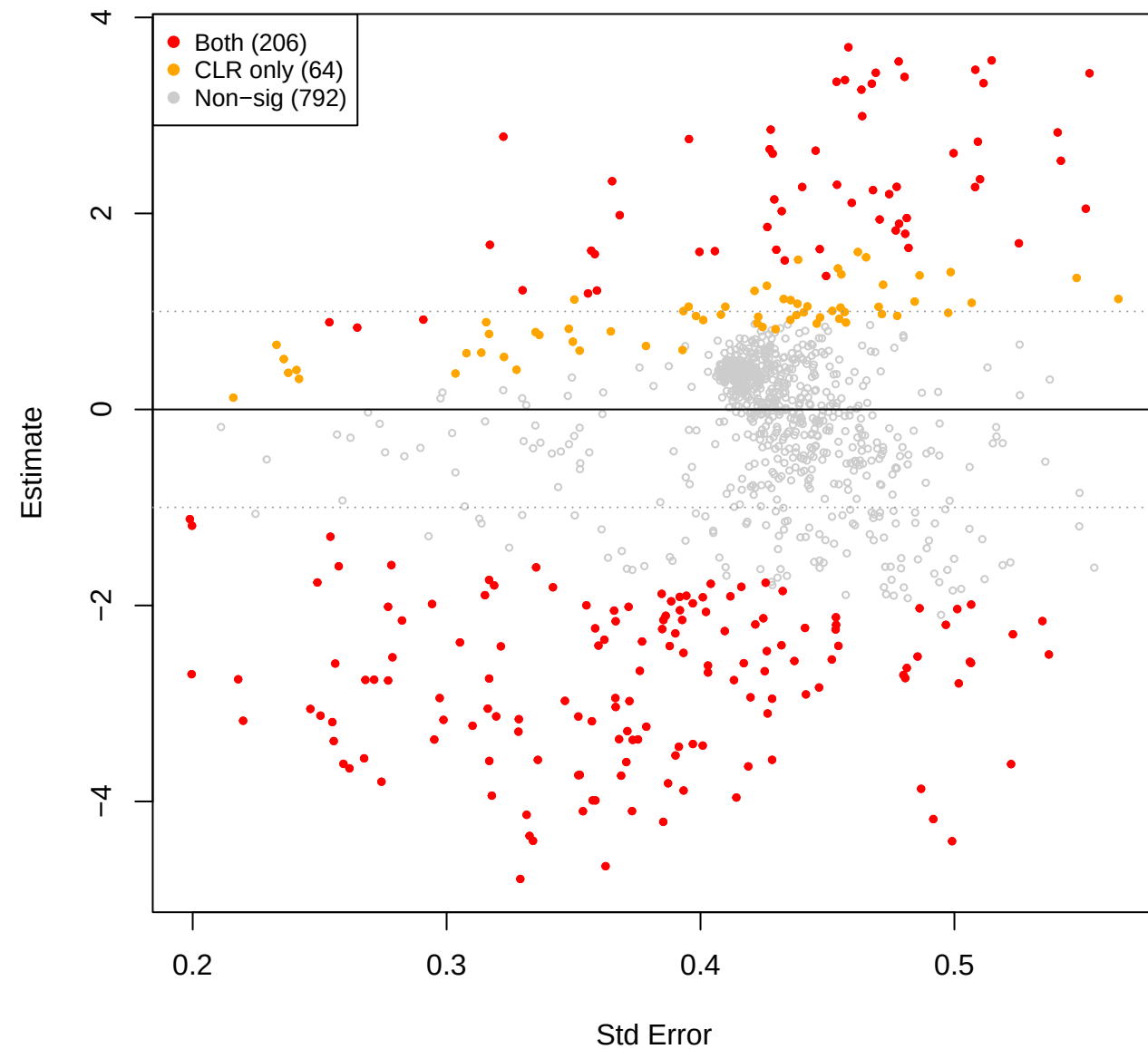
mid vs you – TSS (CLR(const=0.5) sig overlay)
