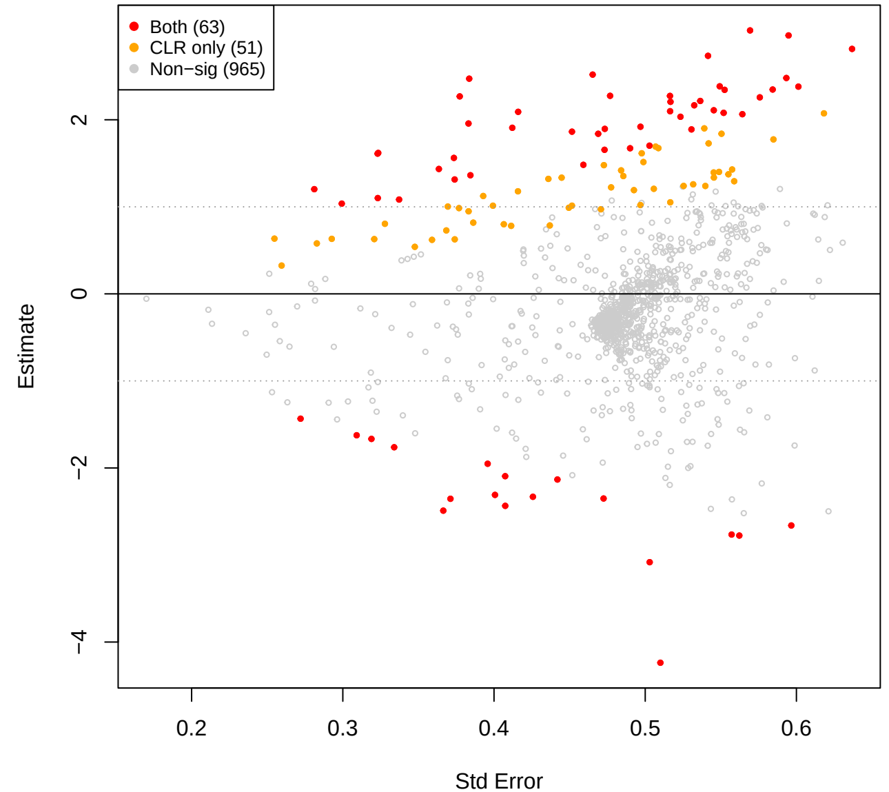
kin vs mage - TSS (CLR(const=0.5) sig overlay)
