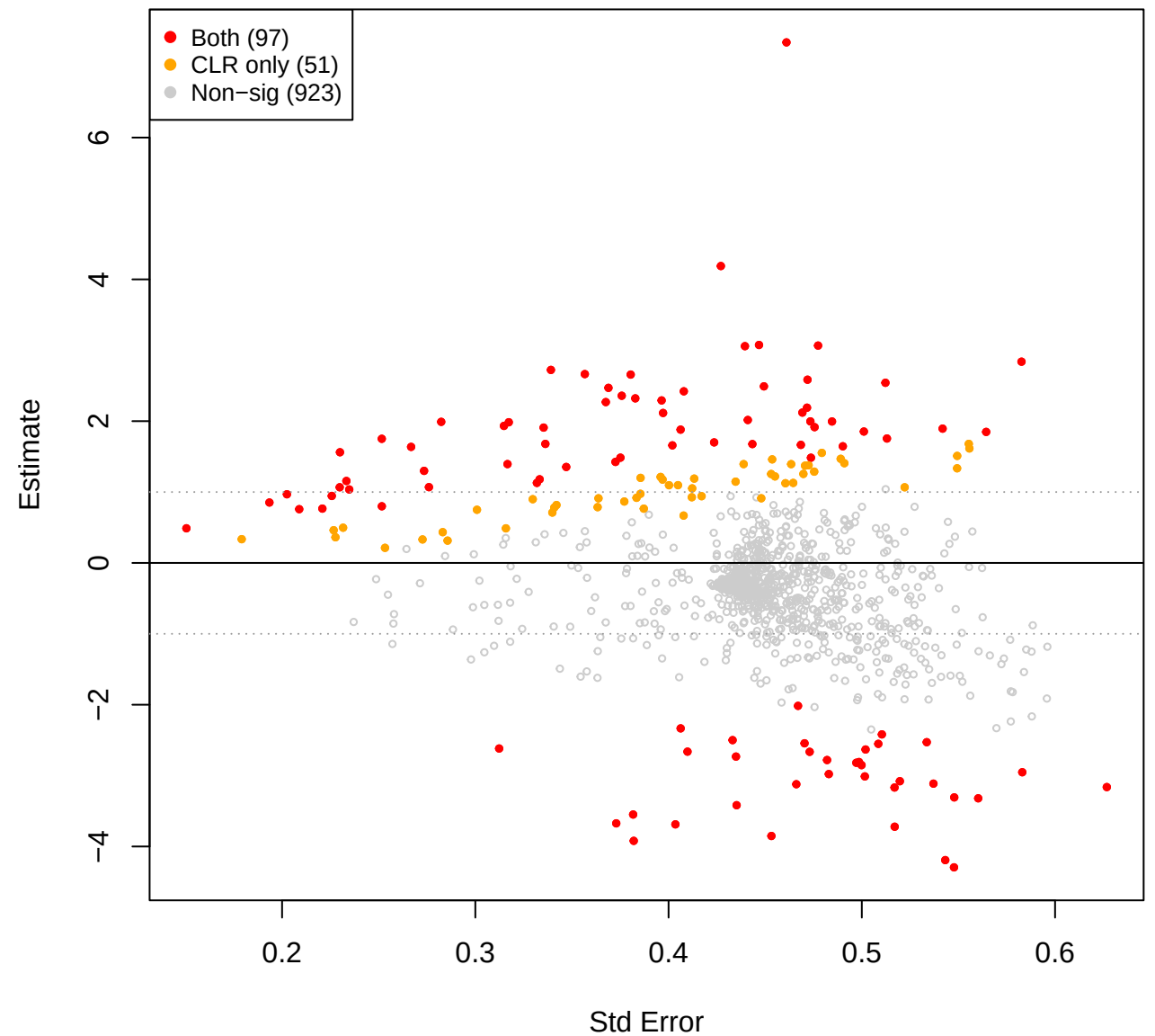
mage vs pup – TSS (CLR(const=0.5) sig overlay)
