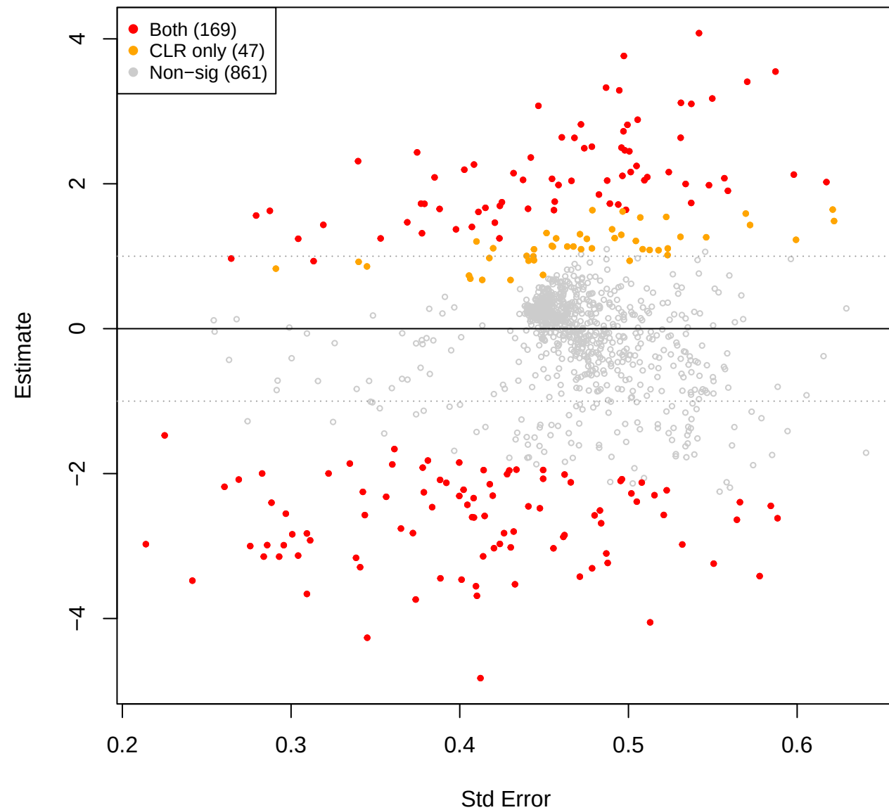
mage vs you – TSS (CLR(const=0.5) sig overlay)
