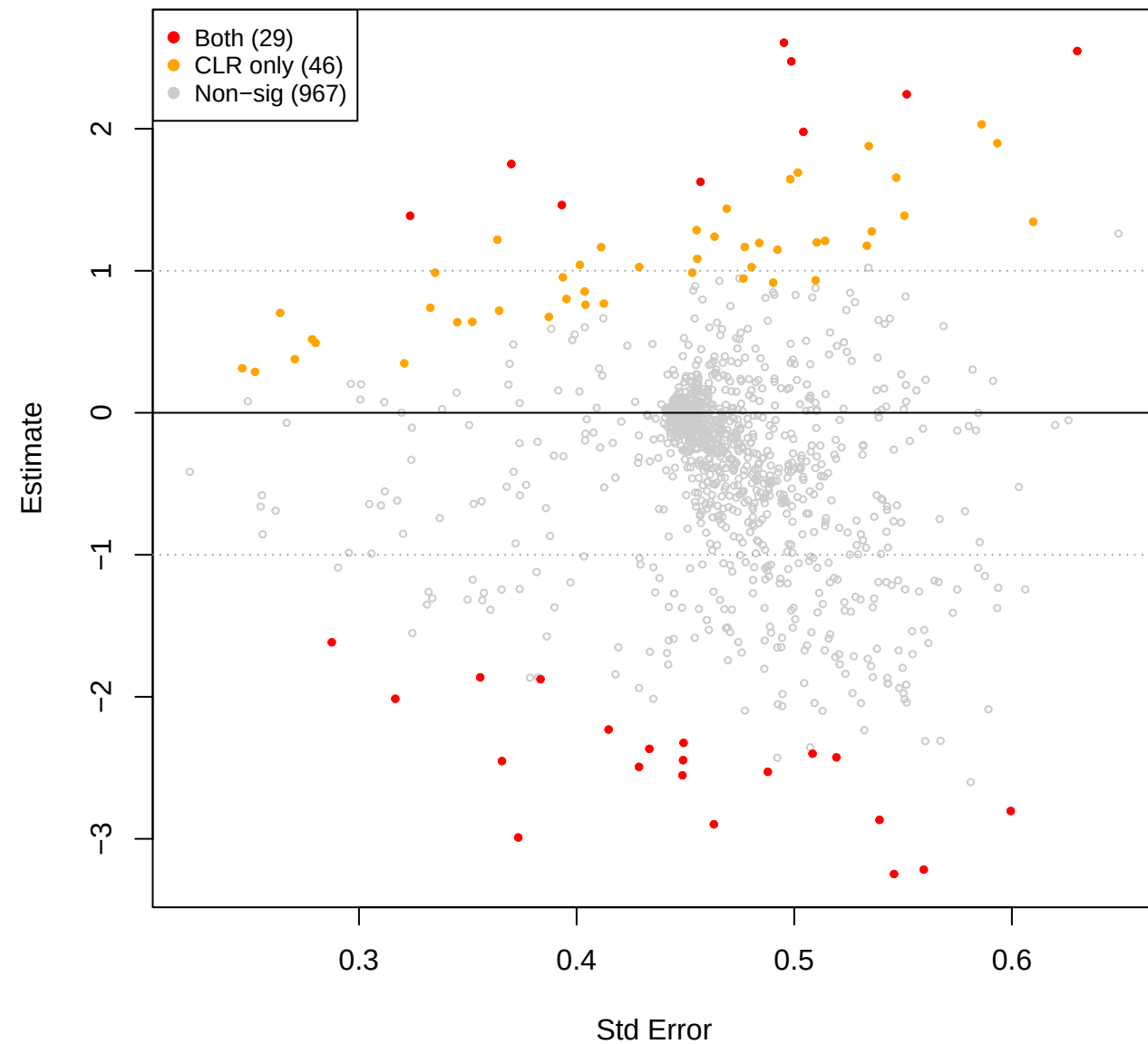
eld vs you – TSS (CLR(const=0.6) sig overlay)
