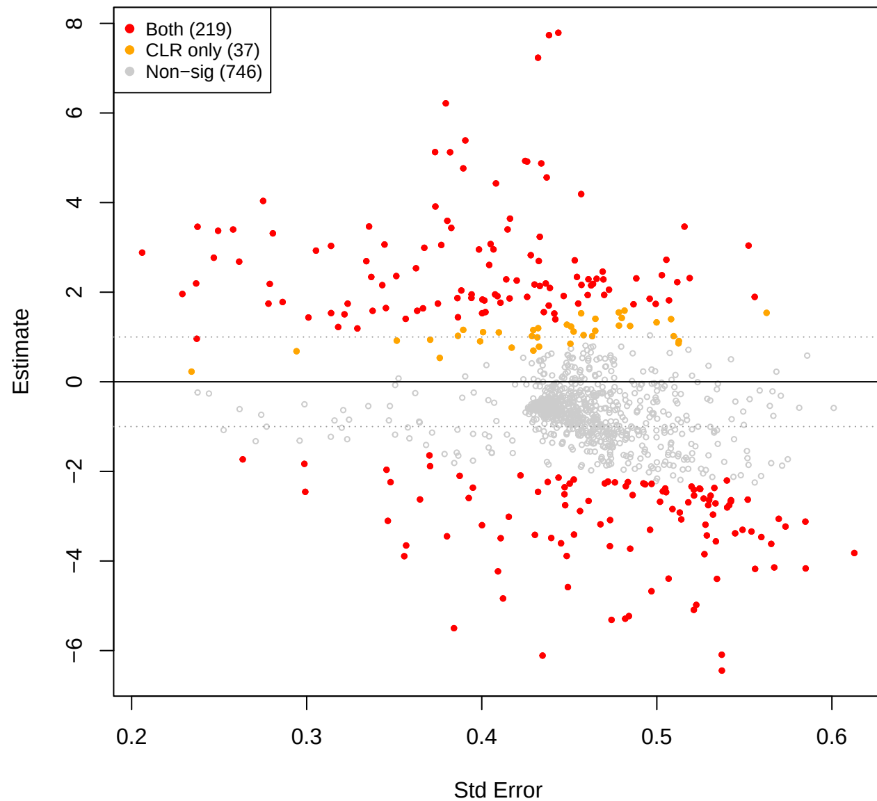
eld vs pup – TSS (CLR(const=0.6) sig overlay)
