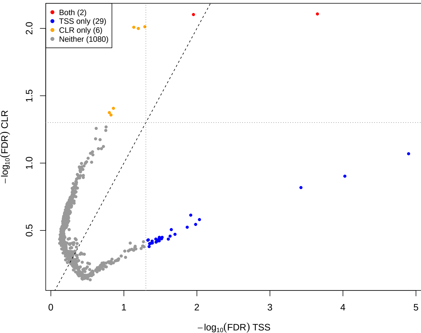
kin vs mid – CLR(const=-1) vs TSS (gamma = 1)
