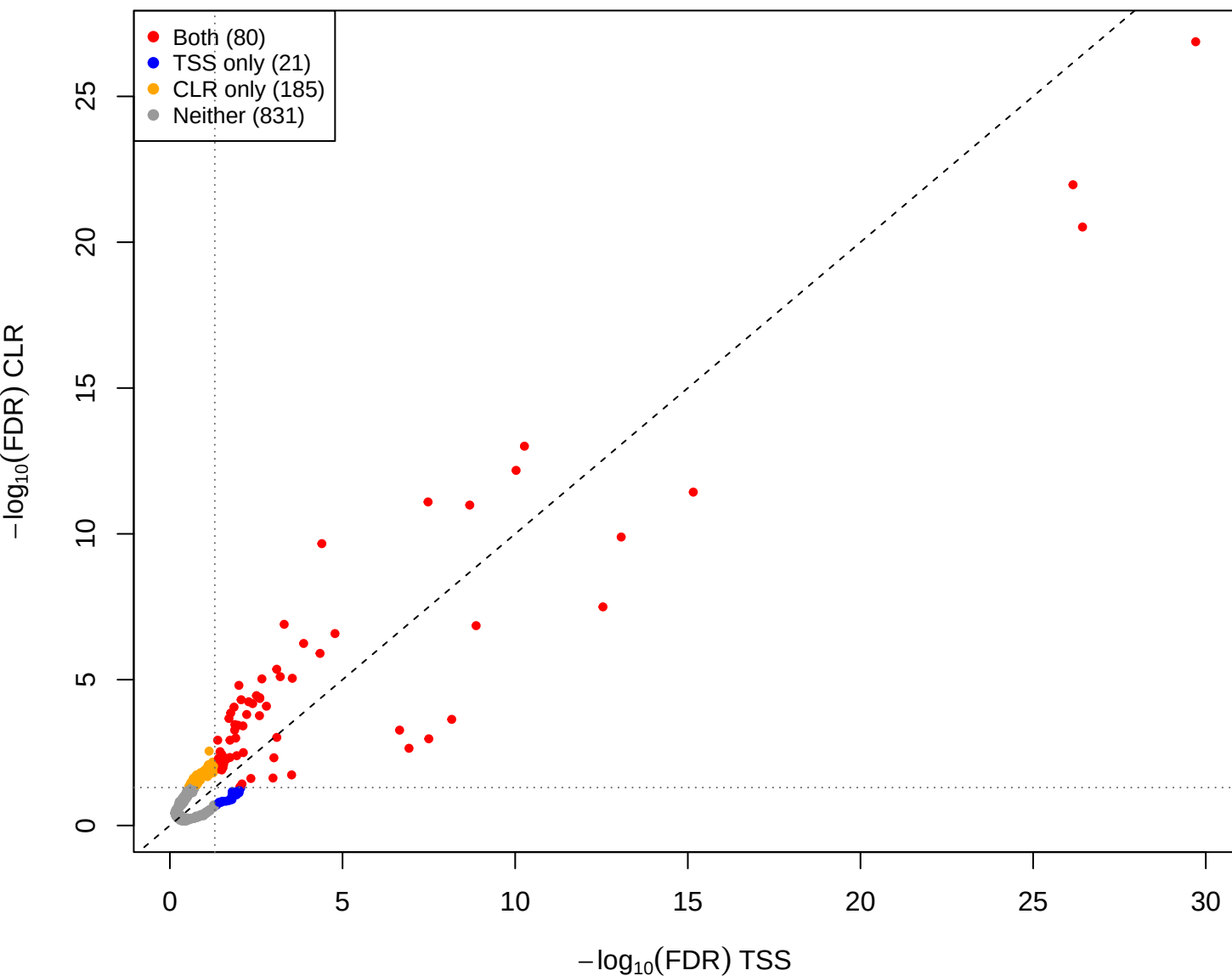
cent vs pup – CLR(const=-1) vs TSS (gamma = 1)
