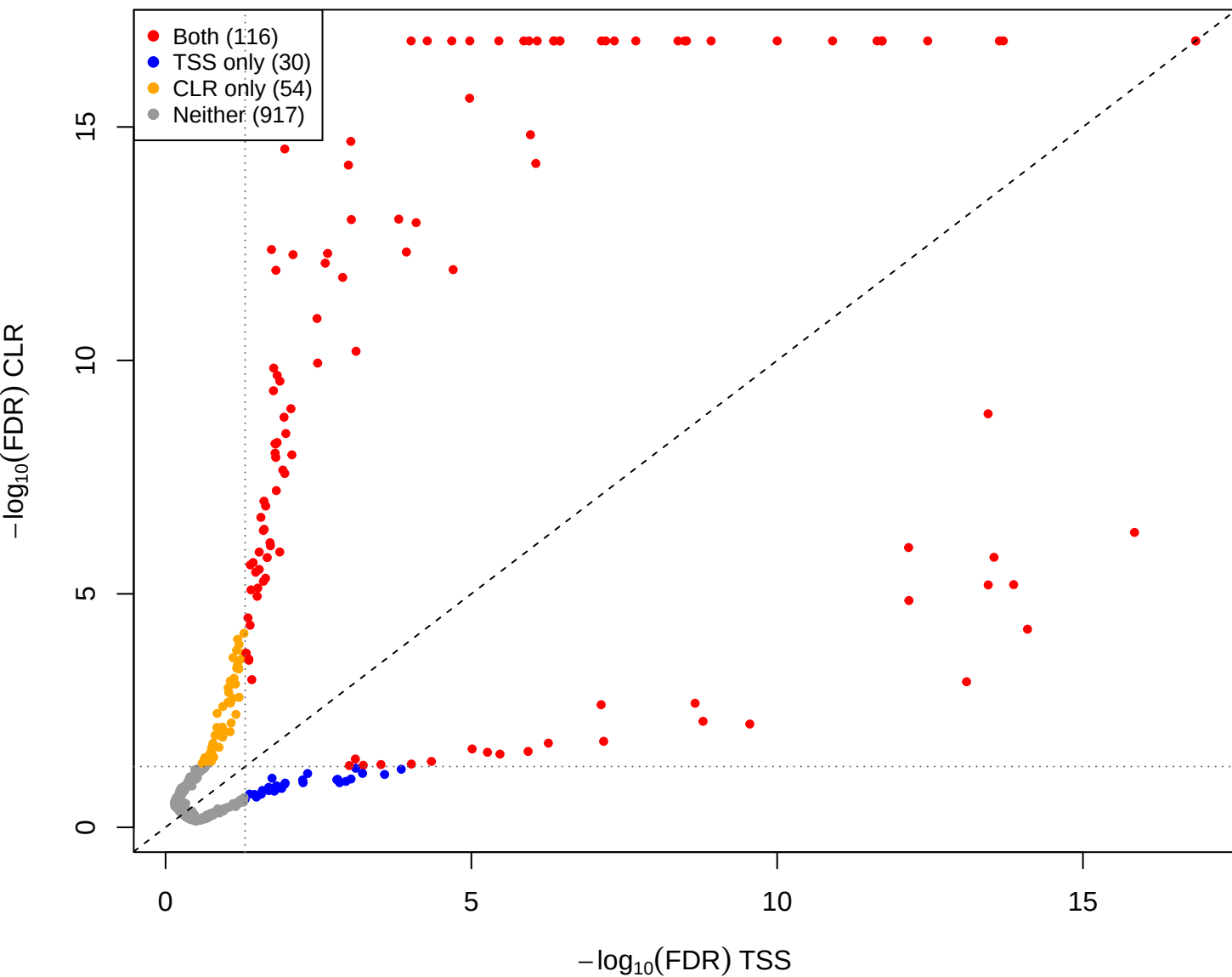
pup vs you - CLR(const=-1) vs TSS (gamma = 1)
