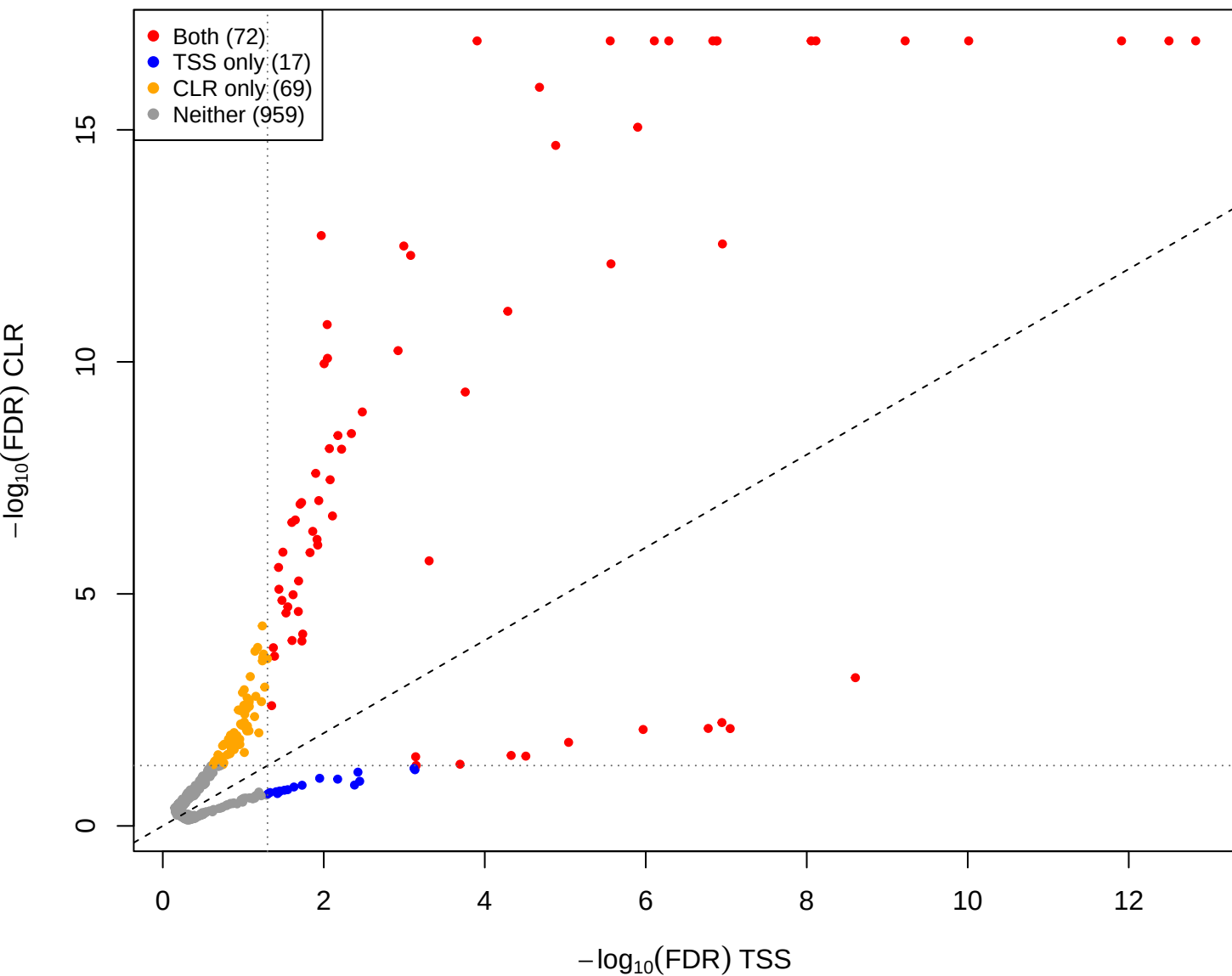
kin vs you – CLR(const=-1) vs TSS (gamma = 1)
