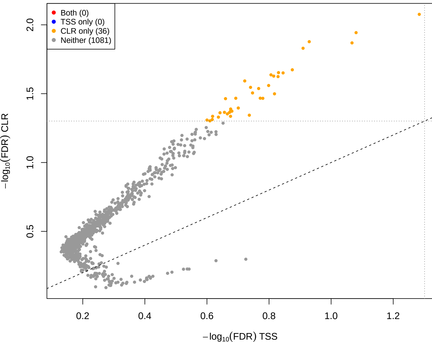
eld vs you - CLR(const=-1) vs TSS (gamma = 1)
