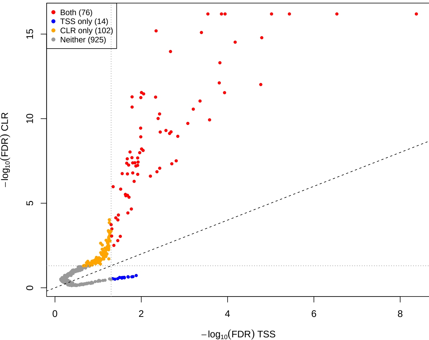
mid vs you - CLR(const=-1) vs TSS (gamma = 1)
