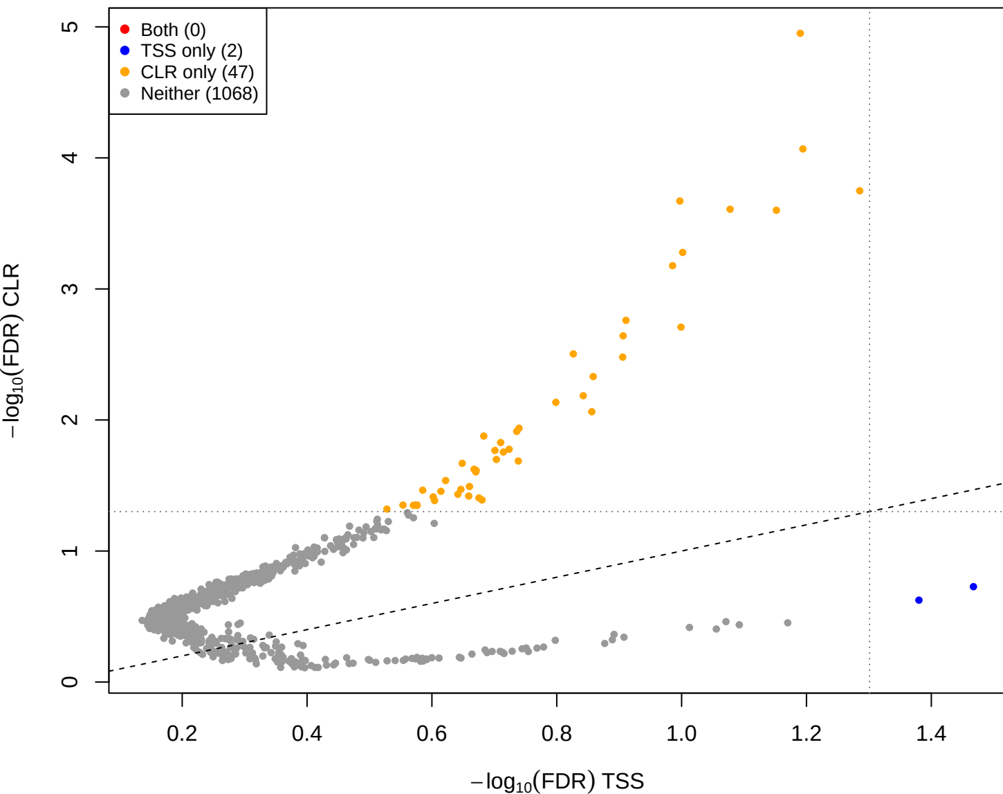
cent vs eld - CLR(const=-1) vs TSS (gamma = 1)
