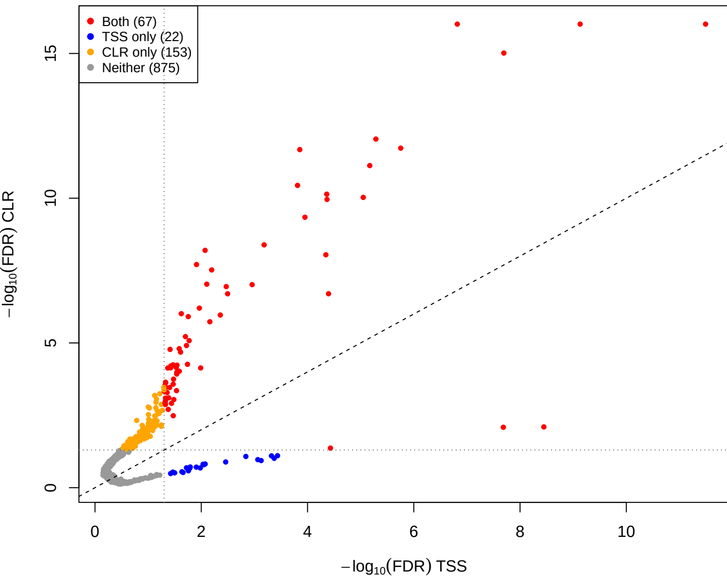
cent vs you – CLR(const=-1) vs TSS (gamma = 1)
