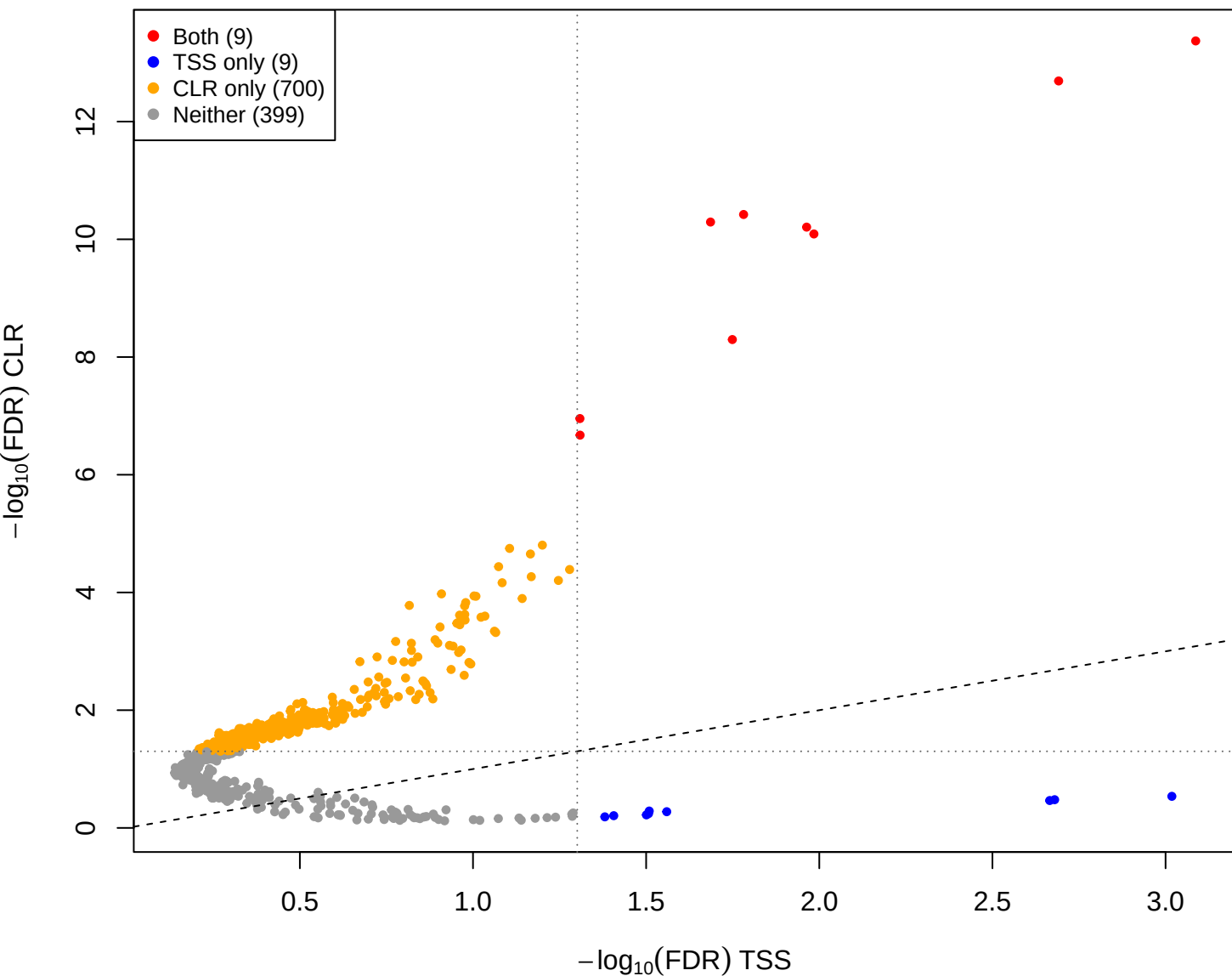
cent vs mage – CLR(const=-2) vs TSS (gamma = 1)
