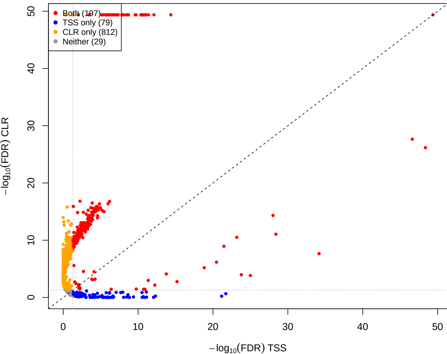
cent vs kin – CLR(const=-2) vs TSS (gamma = 1e-05)
