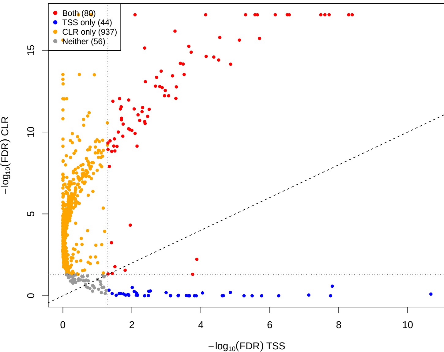
cent vs eld – CLR(const=-2) vs TSS (gamma = 1e-05)
