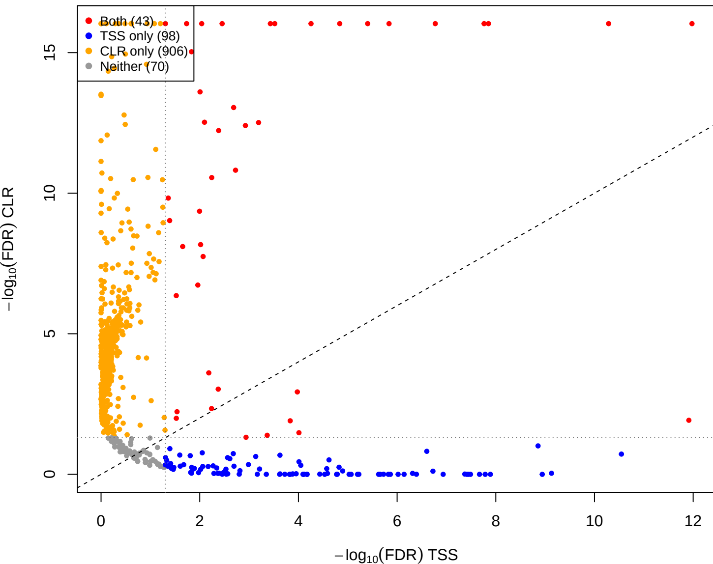
kin vs mid - CLR(const=-2) vs TSS (gamma = 1e-05)
