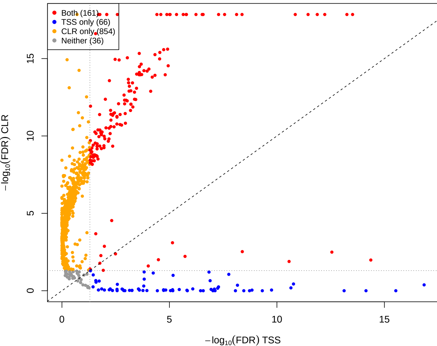
cent vs mage – CLR(const=-2) vs TSS (gamma = 1e-05)
