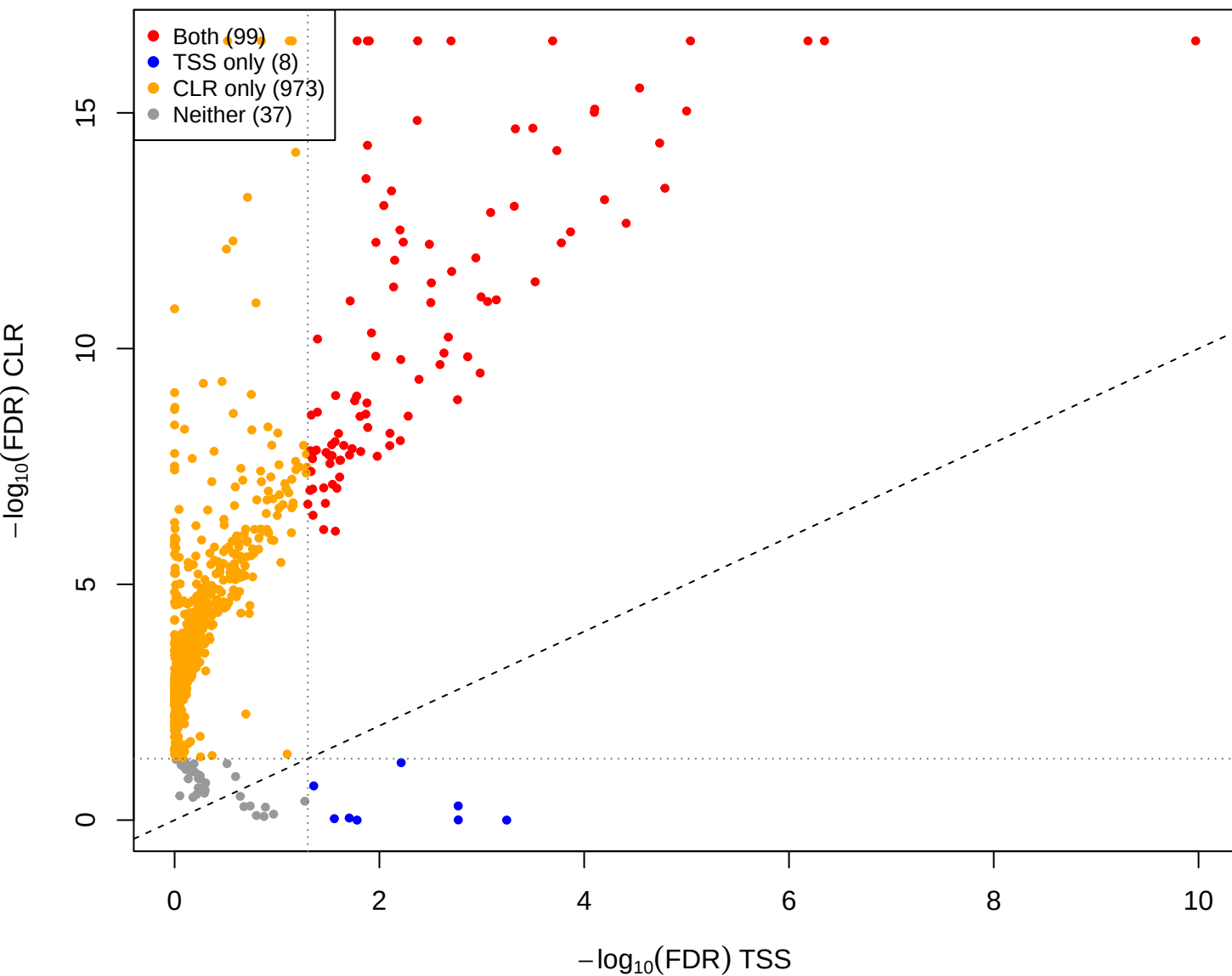
eld vs you - CLR(const=-2) vs TSS (gamma = 1e-05)
