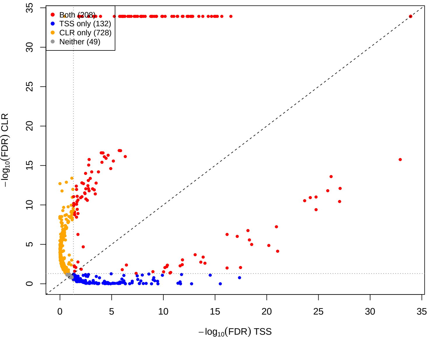
pup vs you – CLR(const=-2) vs TSS (gamma = 1e-05)
