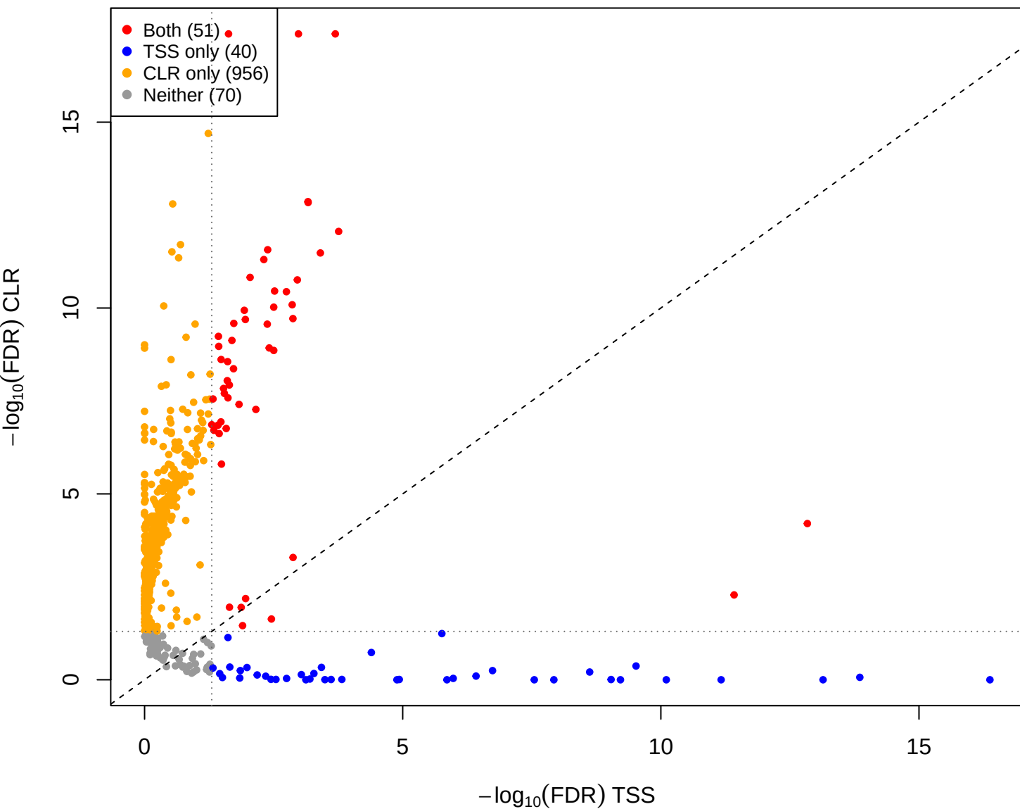
eld vs mage - CLR(const=-2) vs TSS (gamma = 1e-05)
