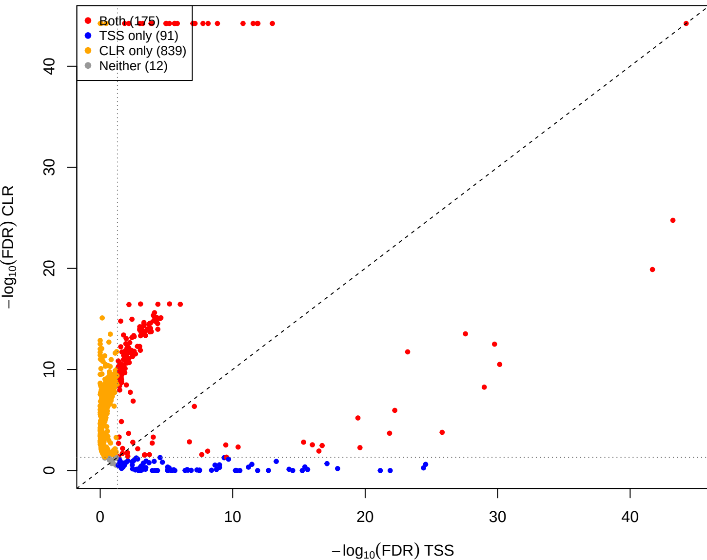
cent vs mid – CLR(const=-2) vs TSS (gamma = 1e-05)
