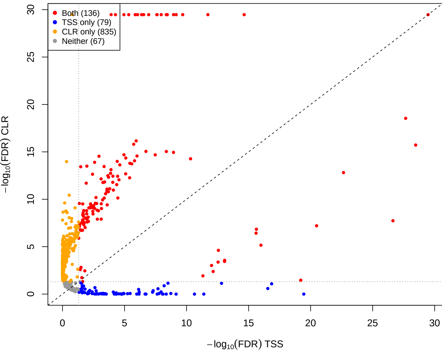
eld vs kin - CLR(const=-2) vs TSS (gamma = 1e-05)
