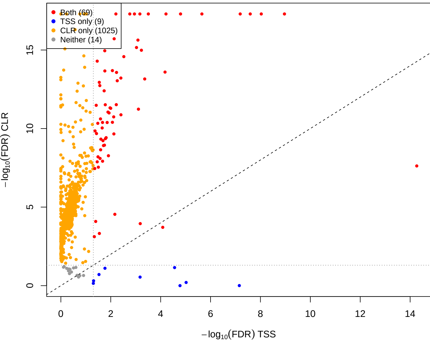
kin vs pup – CLR(const=-2) vs TSS (gamma = 1e-05)
