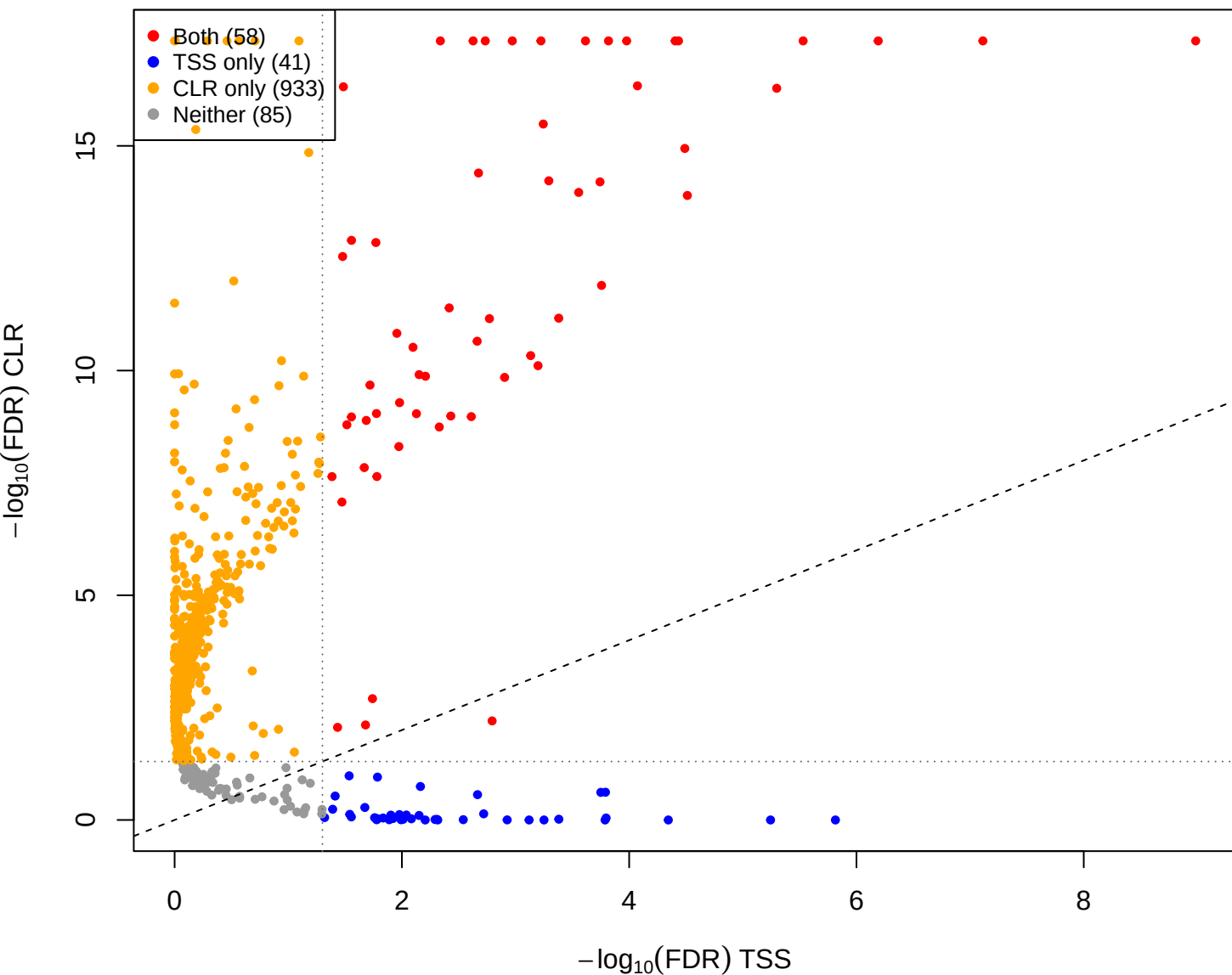
kin vs mage - CLR(const=-2) vs TSS (gamma = 1e-05)
