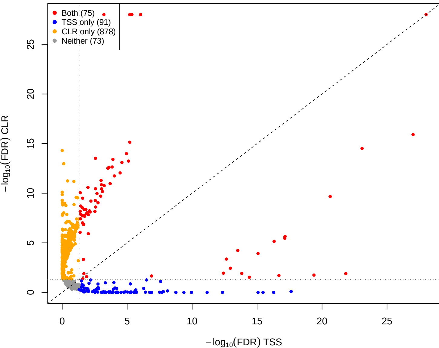
eld vs mid - CLR(const=-2) vs TSS (gamma = 1e-05)
