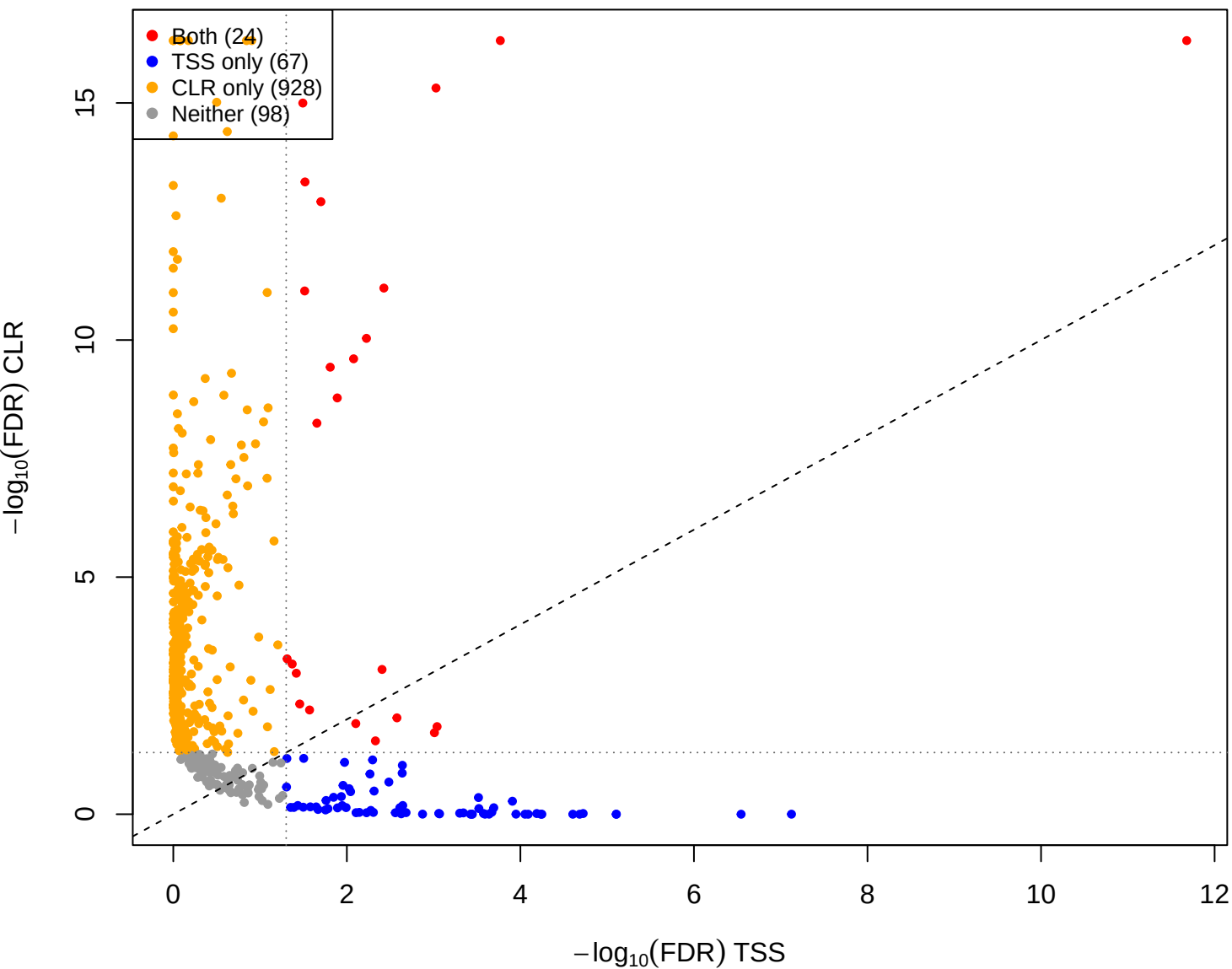
mage vs mid – CLR(const=-2) vs TSS (gamma = 1e-05)
