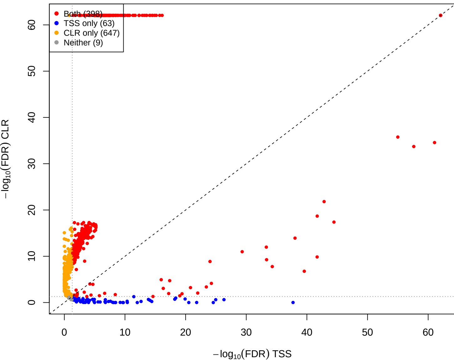
cent vs pup – CLR(const=-2) vs TSS (gamma = 1e-05)
