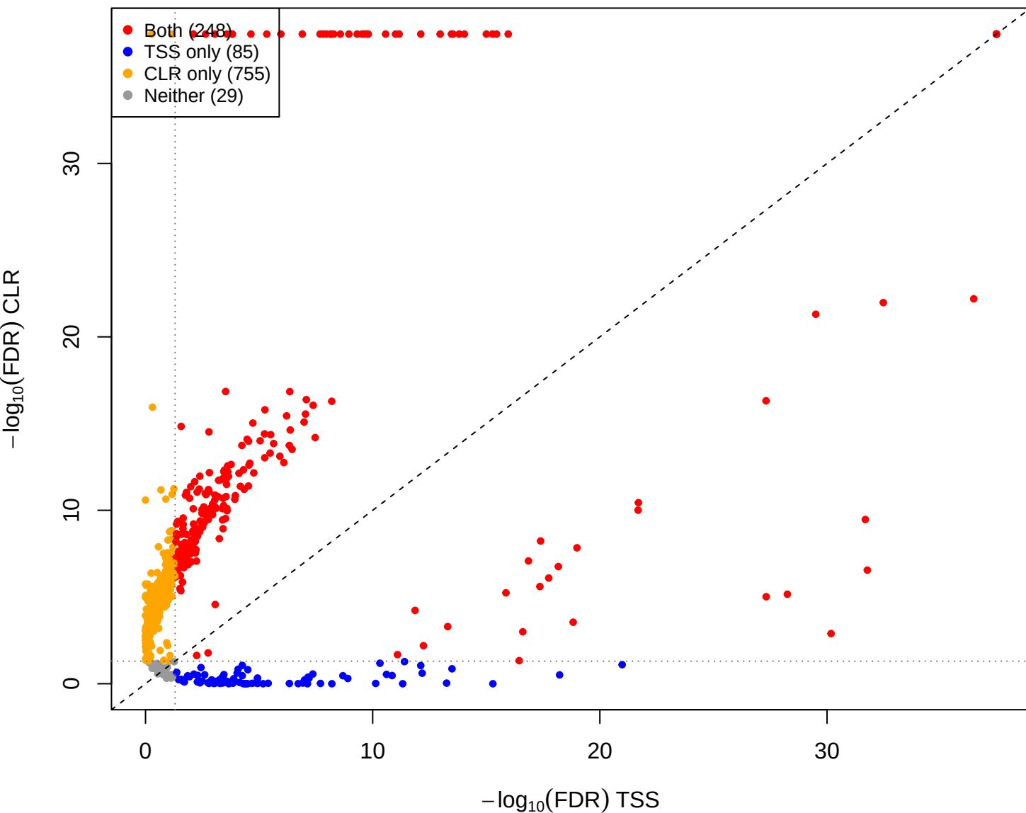
eld vs pup – CLR(const=-2) vs TSS (gamma = 1e-05)
