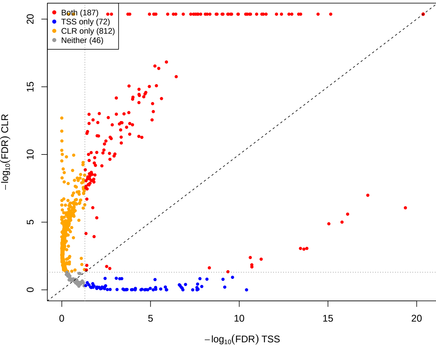
kin vs you - CLR(const=-2) vs TSS (gamma = 1e-05)
