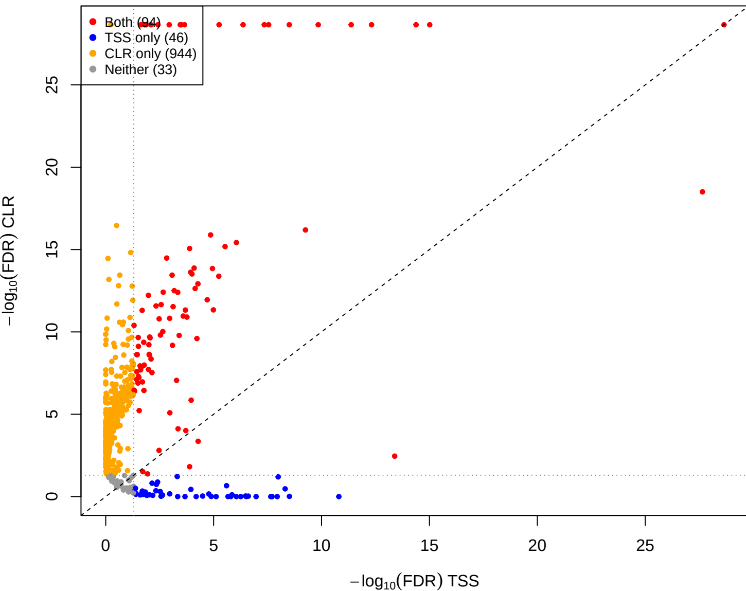
mage vs pup – CLR(const=-2) vs TSS (gamma = 1e-05)
