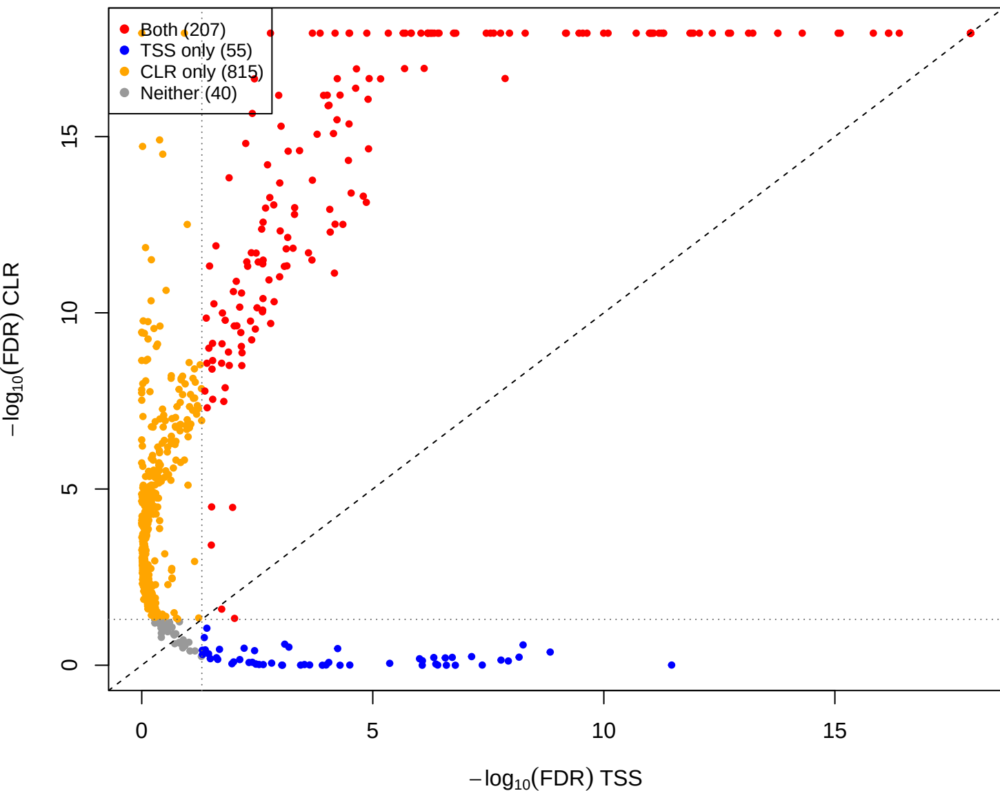
mid vs you – CLR(const=-2) vs TSS (gamma = 1e-05)
