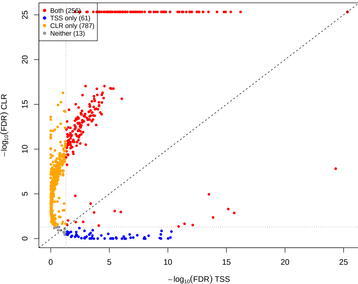
cent vs you – CLR(const=-2) vs TSS (gamma = 1e-05)
