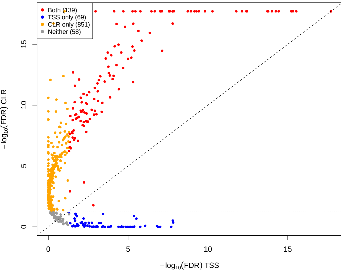
mage vs you – CLR(const=-2) vs TSS (gamma = 1e-05)
