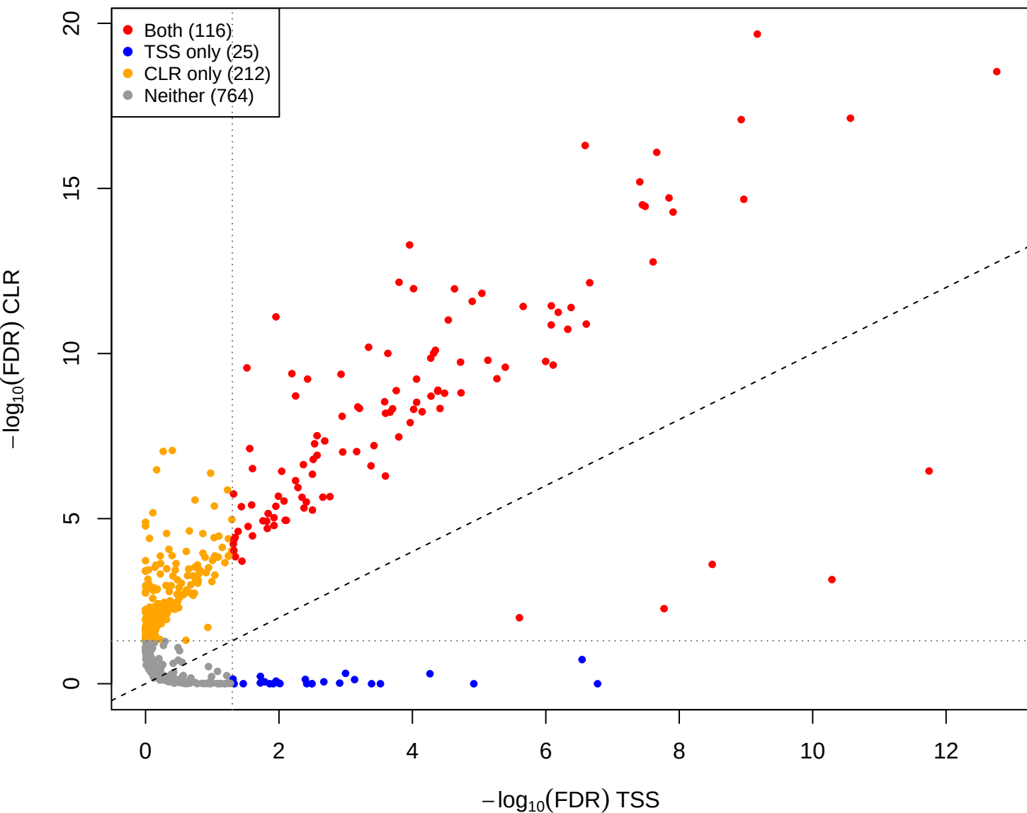
kin vs mid – CLR(const=1) vs TSS (gamma = 1e-05)
