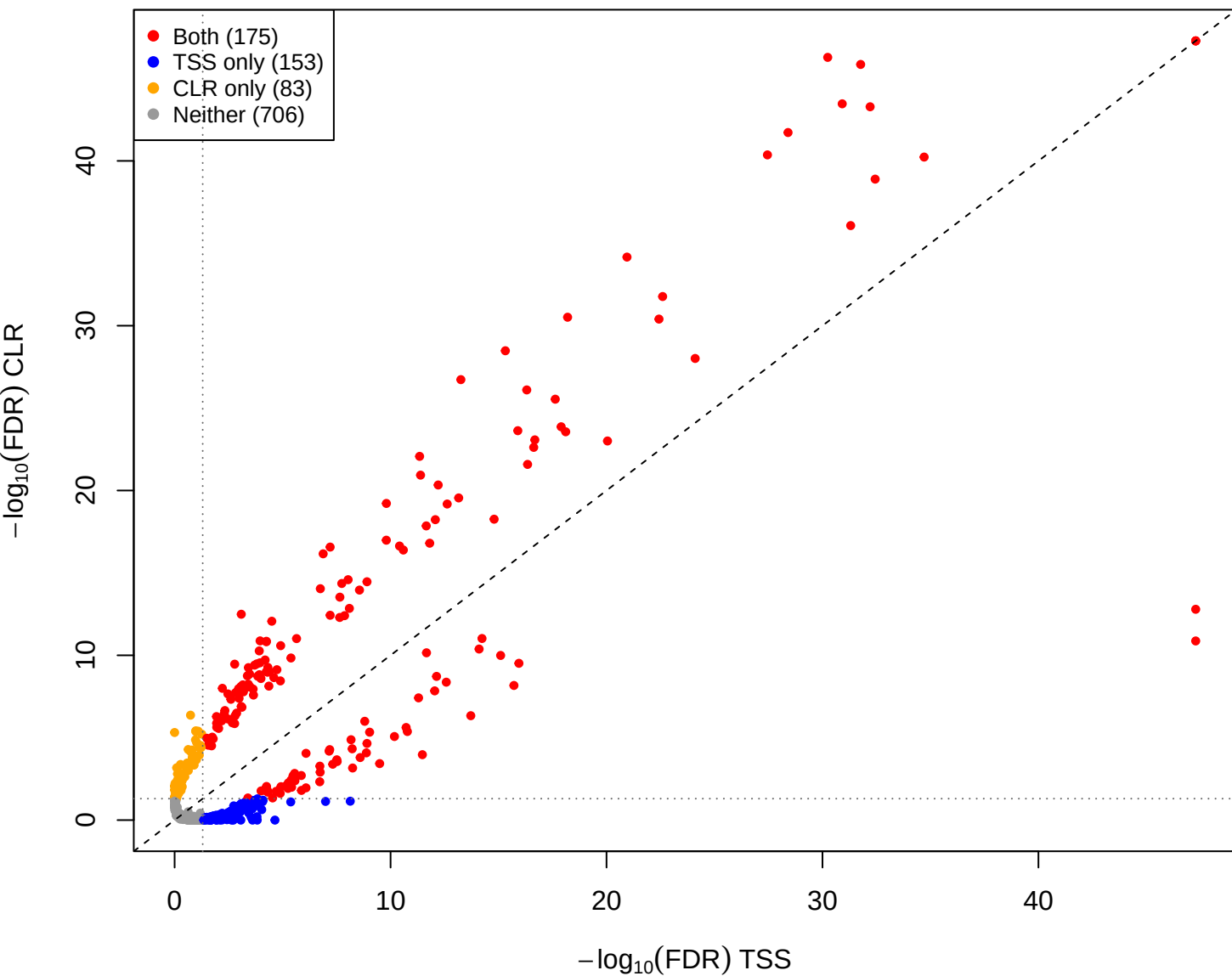
eld vs pup – CLR(const=1) vs TSS (gamma = 1e-05)
