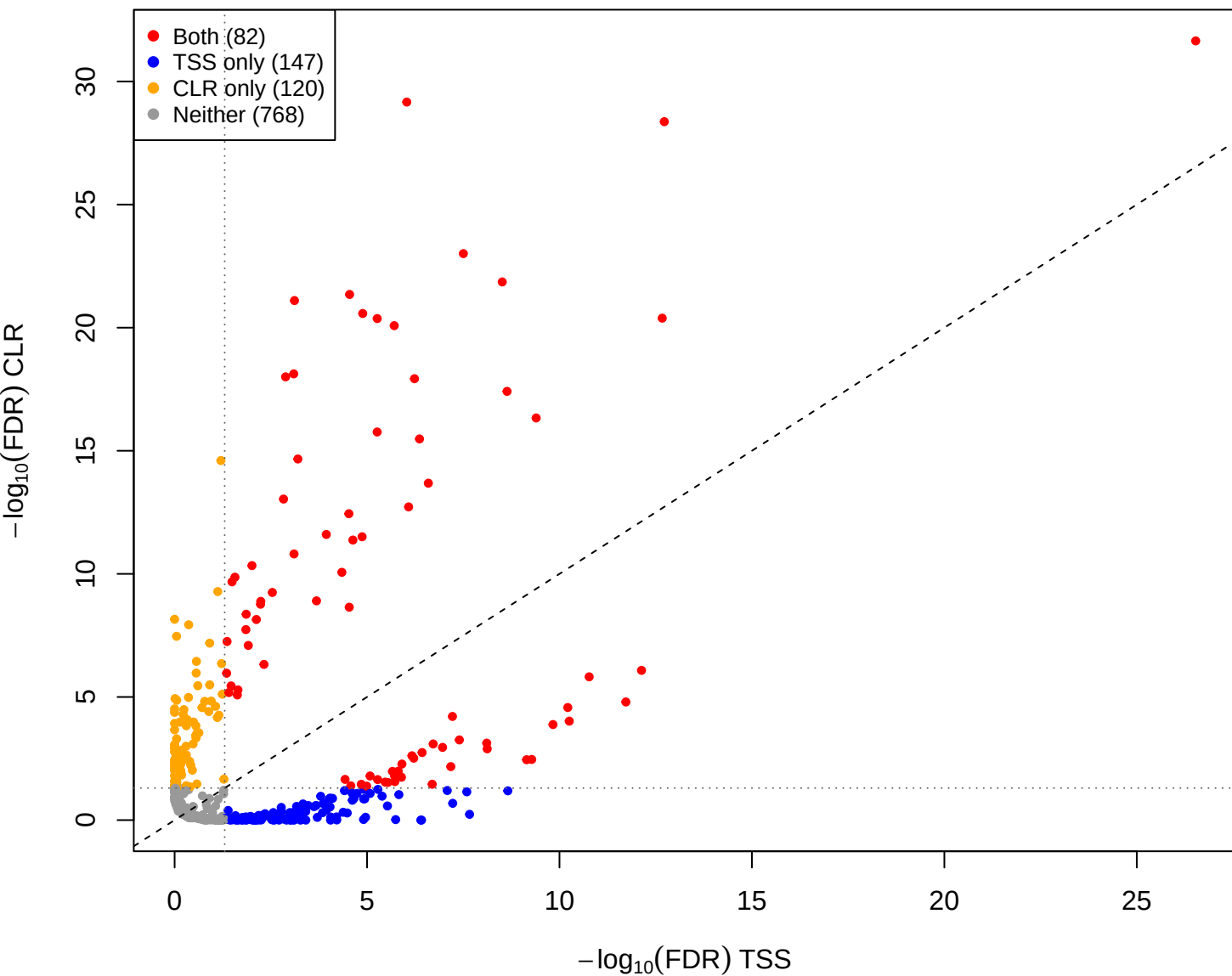
mid vs pup – CLR(const=1) vs TSS (gamma = 1e-05)
