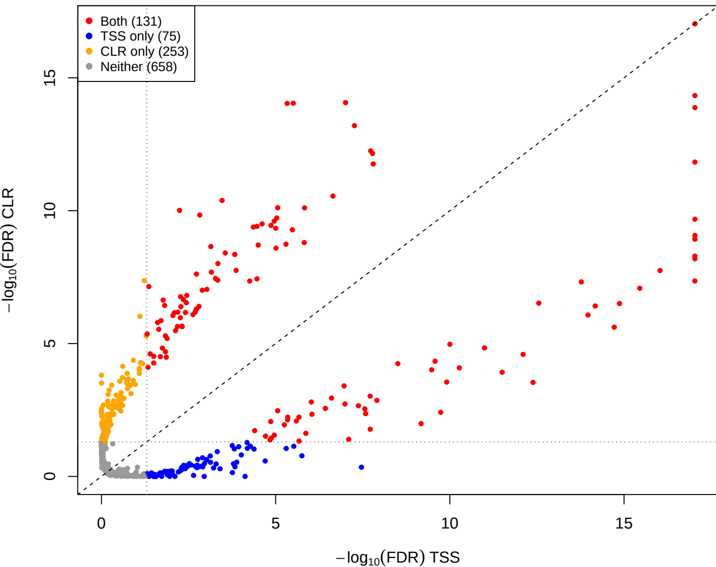
mage vs you - CLR(const=1) vs TSS (gamma = 1e-05)
