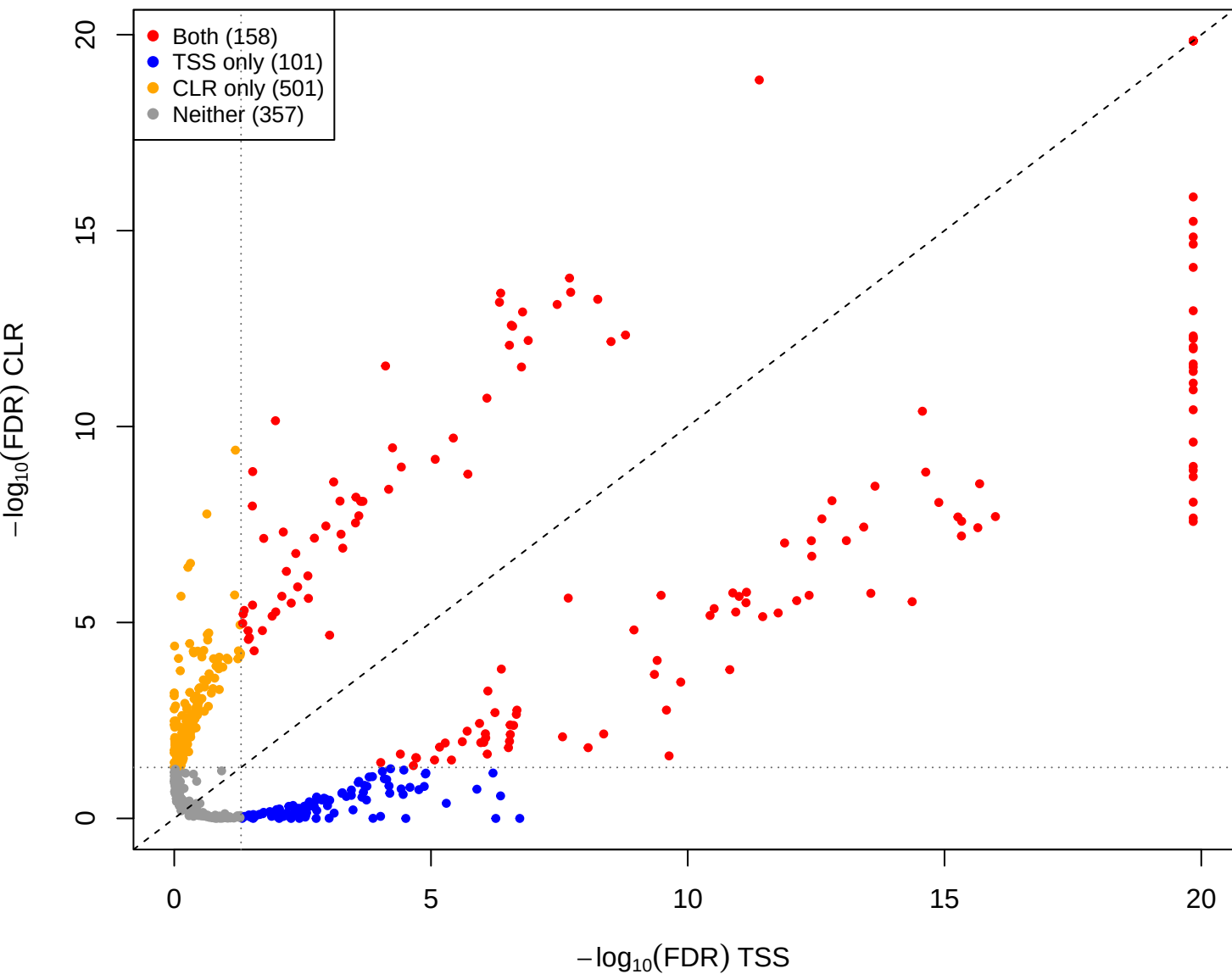
mid vs you - CLR(const=1) vs TSS (gamma = 1e-05)
