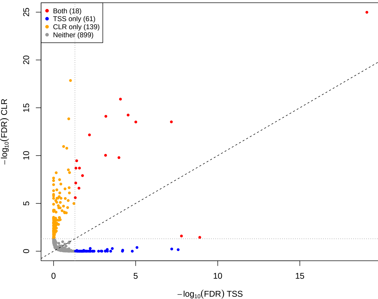
kin vs pup – CLR(const=1) vs TSS (gamma = 1e-05)
