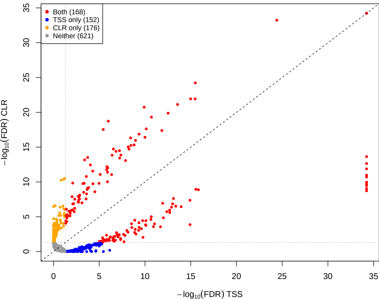
cent vs you – CLR(const=1) vs TSS (gamma = 1e-05)
