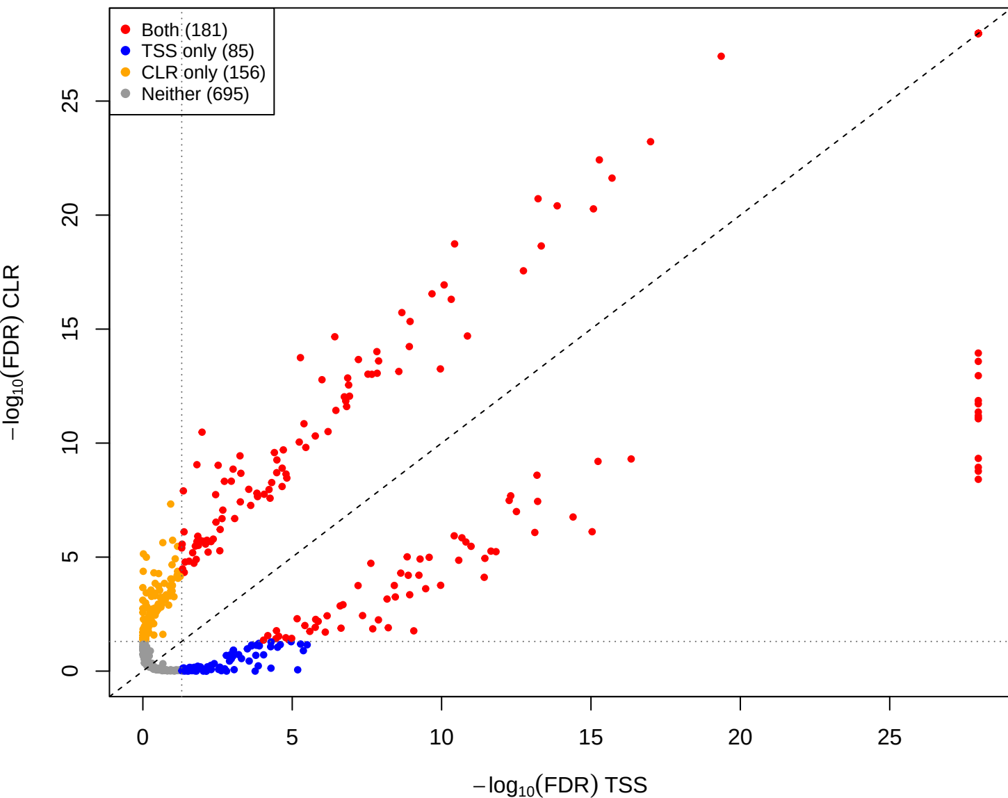
kin vs you – CLR(const=1) vs TSS (gamma = 1e-05)
