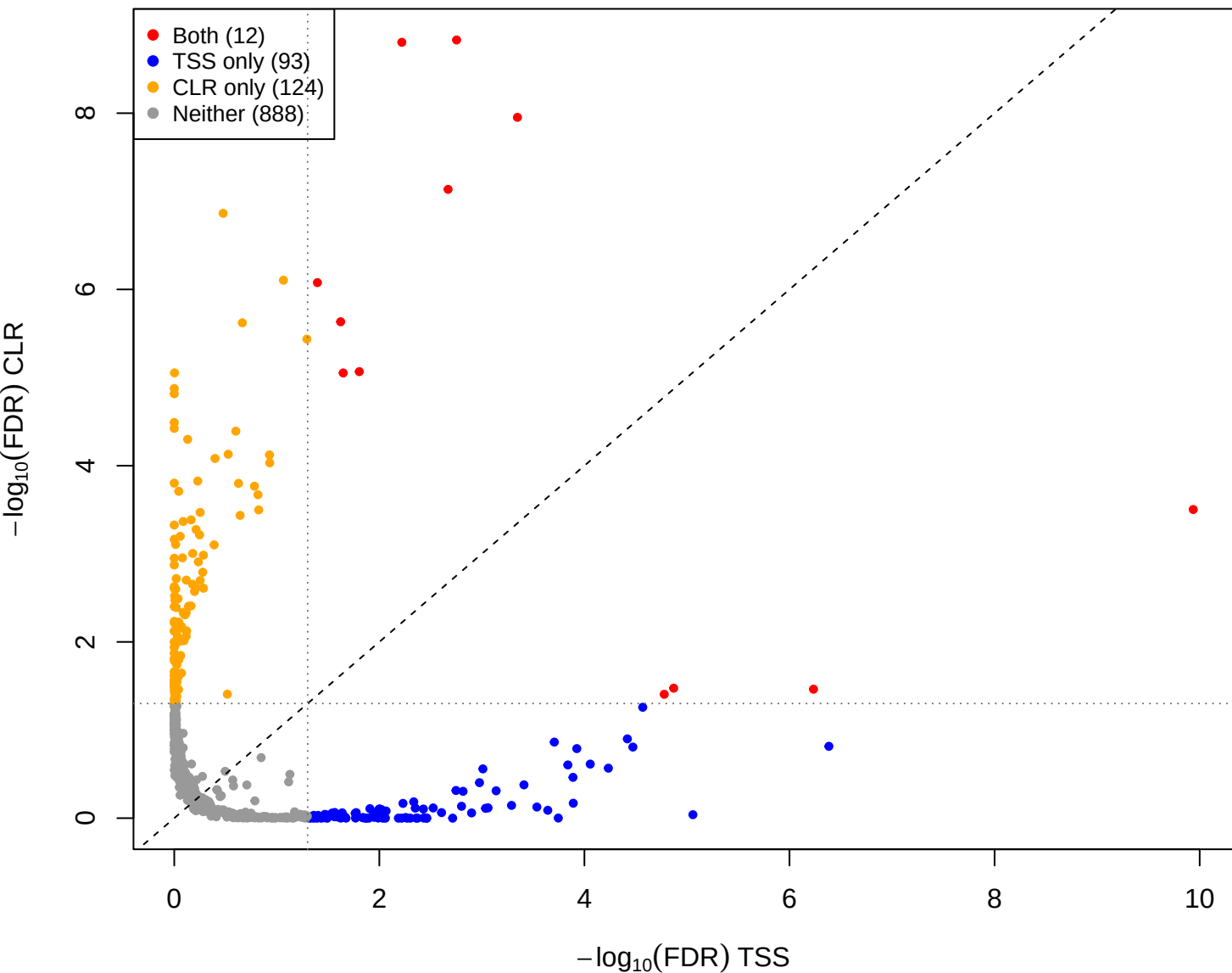
eld vs you – CLR(const=1) vs TSS (gamma = 1e-05)
