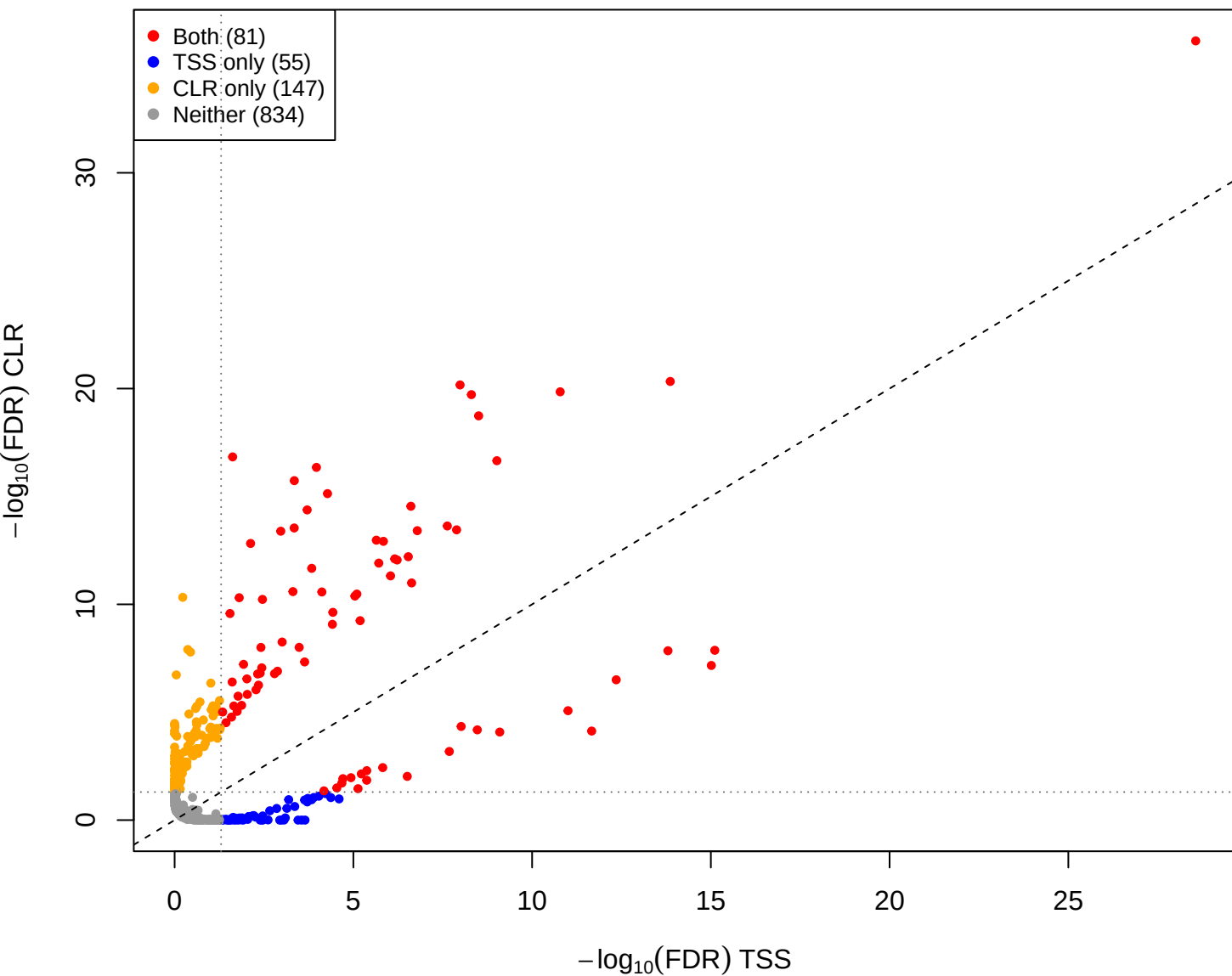
mage vs pup – CLR(const=1) vs TSS (gamma = 1e-05)
