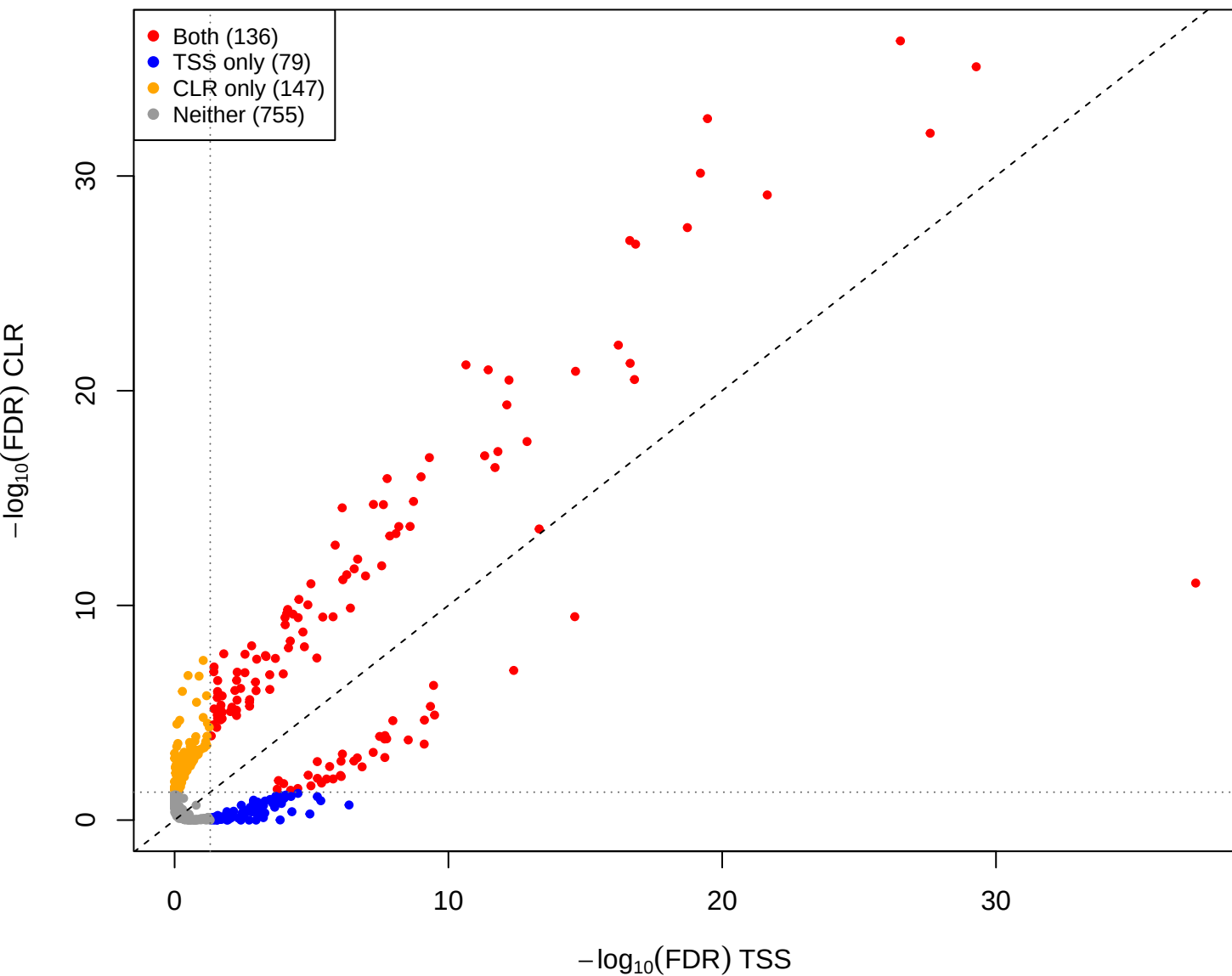
eld vs kin – CLR(const=1) vs TSS (gamma = 1e-05)
