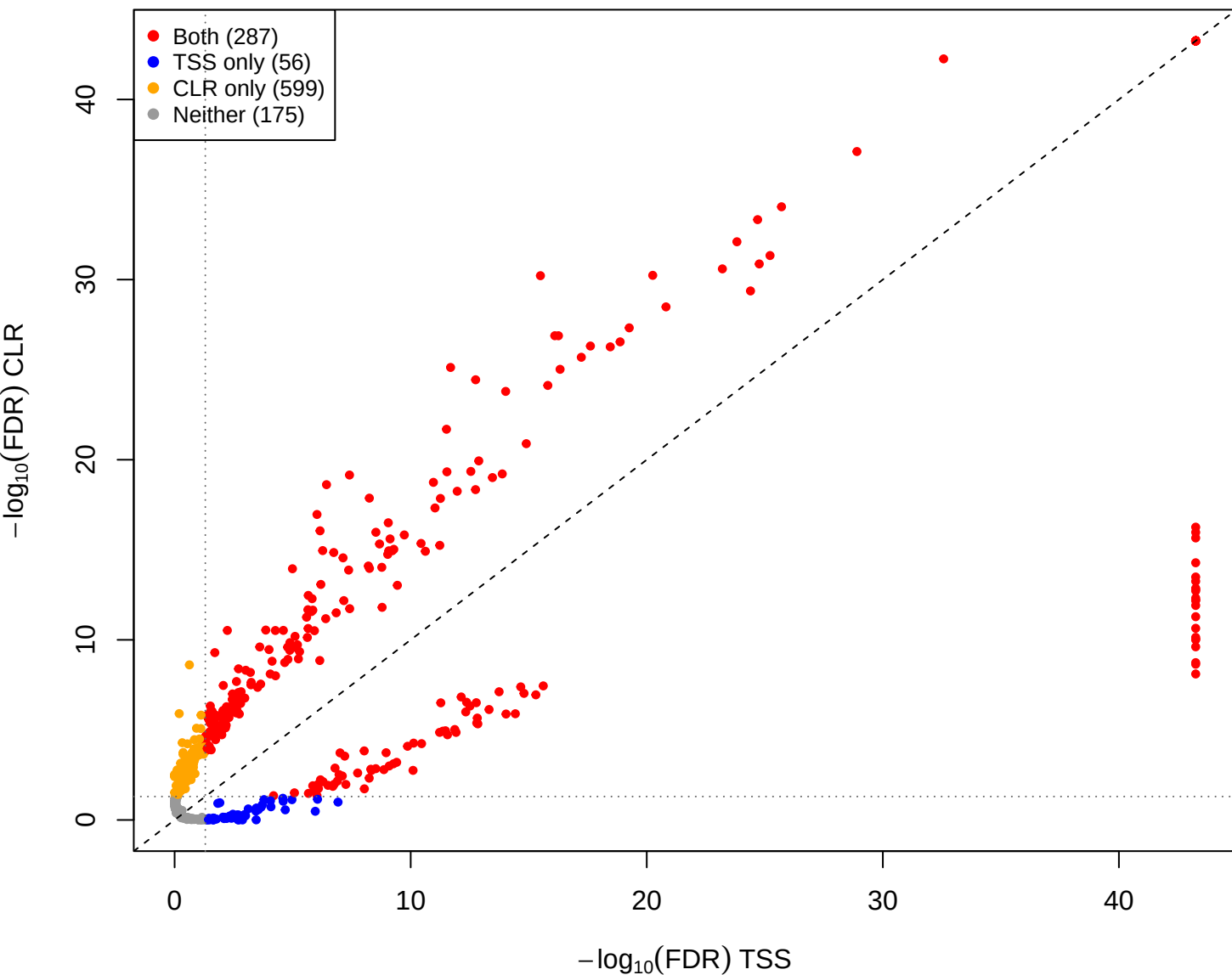
pup vs you – CLR(const=1) vs TSS (gamma = 1e-05)
