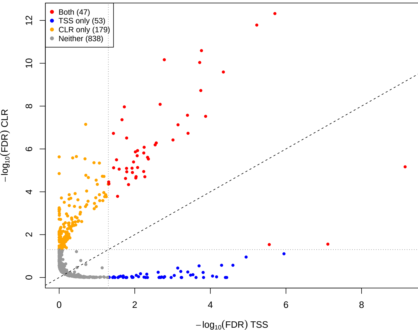
kin vs mage – CLR(const=1) vs TSS (gamma = 1e-05)
