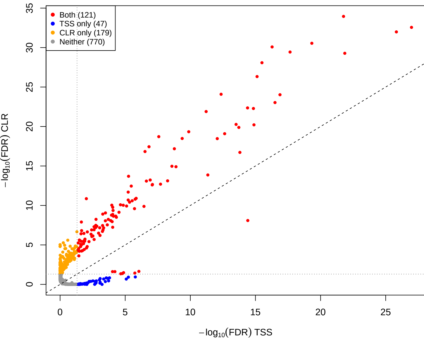
eld vs mid – CLR(const=1) vs TSS (gamma = 1e-05)
