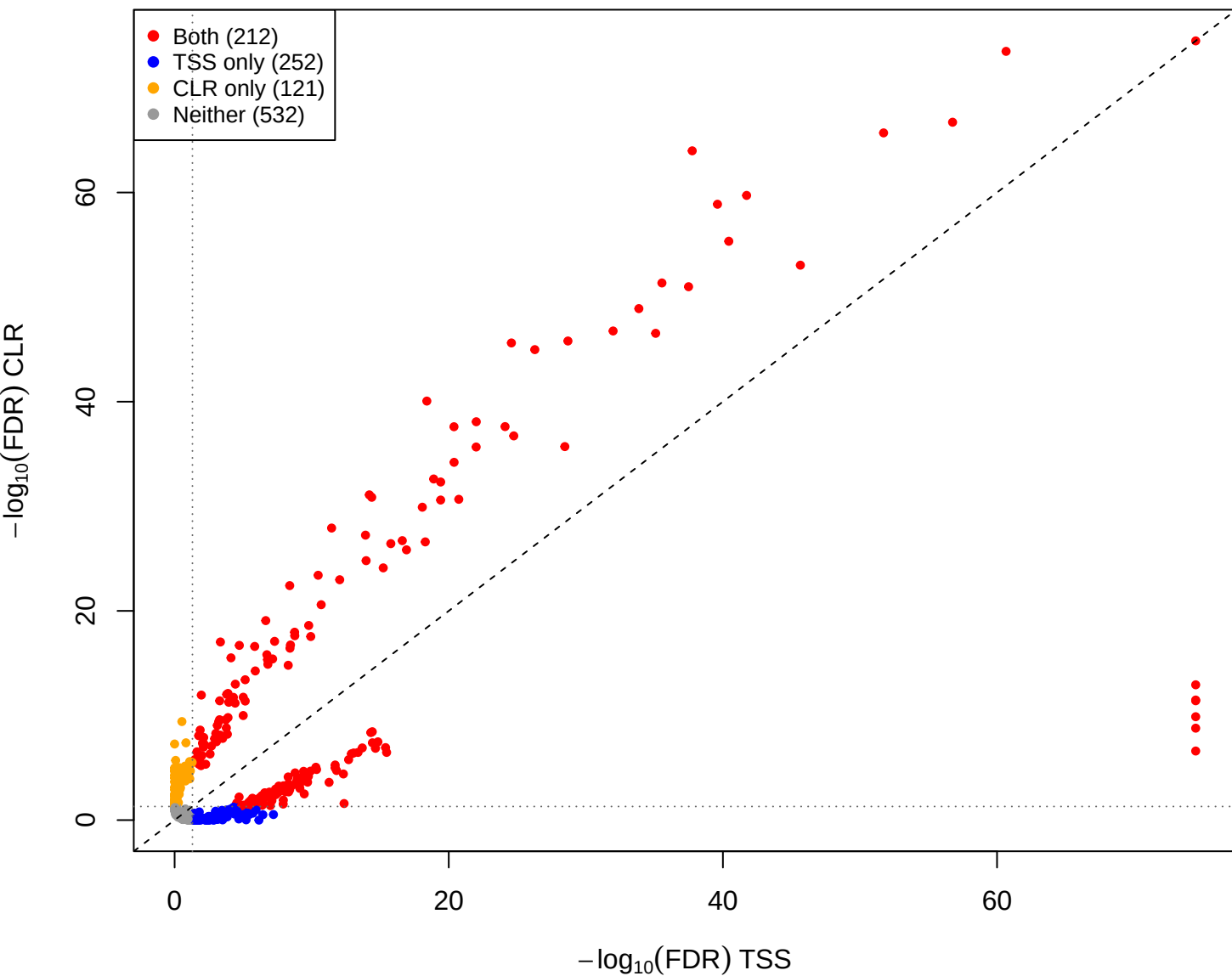
cent vs pup – CLR(const=1) vs TSS (gamma = 1e-05)
