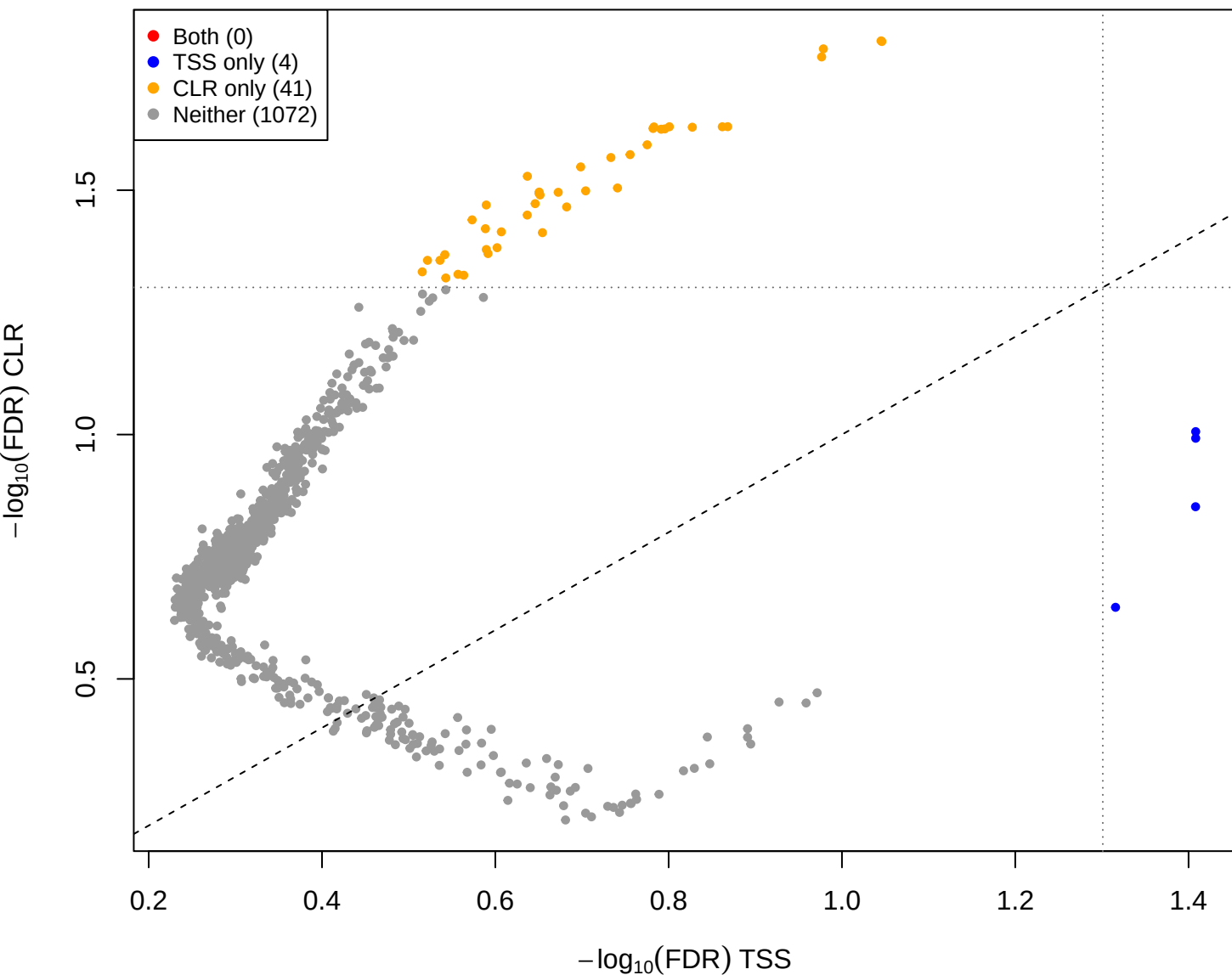
eld vs pup – CLR(const=-3) vs TSS (gamma = 3)
