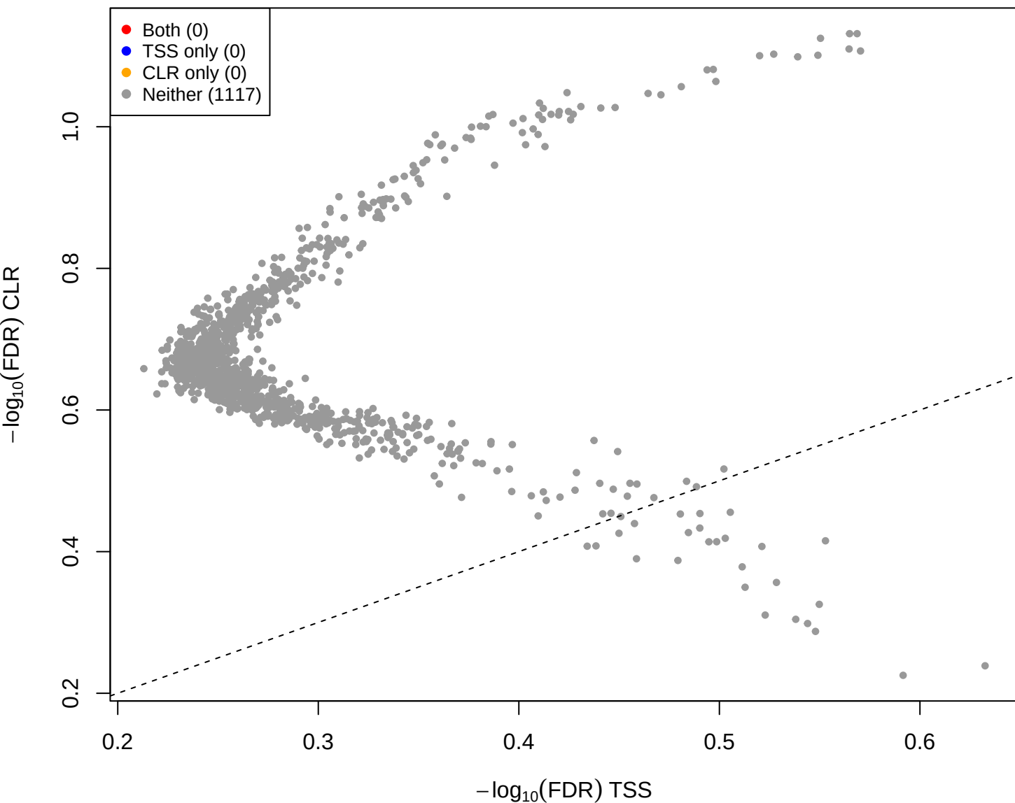
cent vs eld - CLR(const=-3) vs TSS (gamma = 3)
