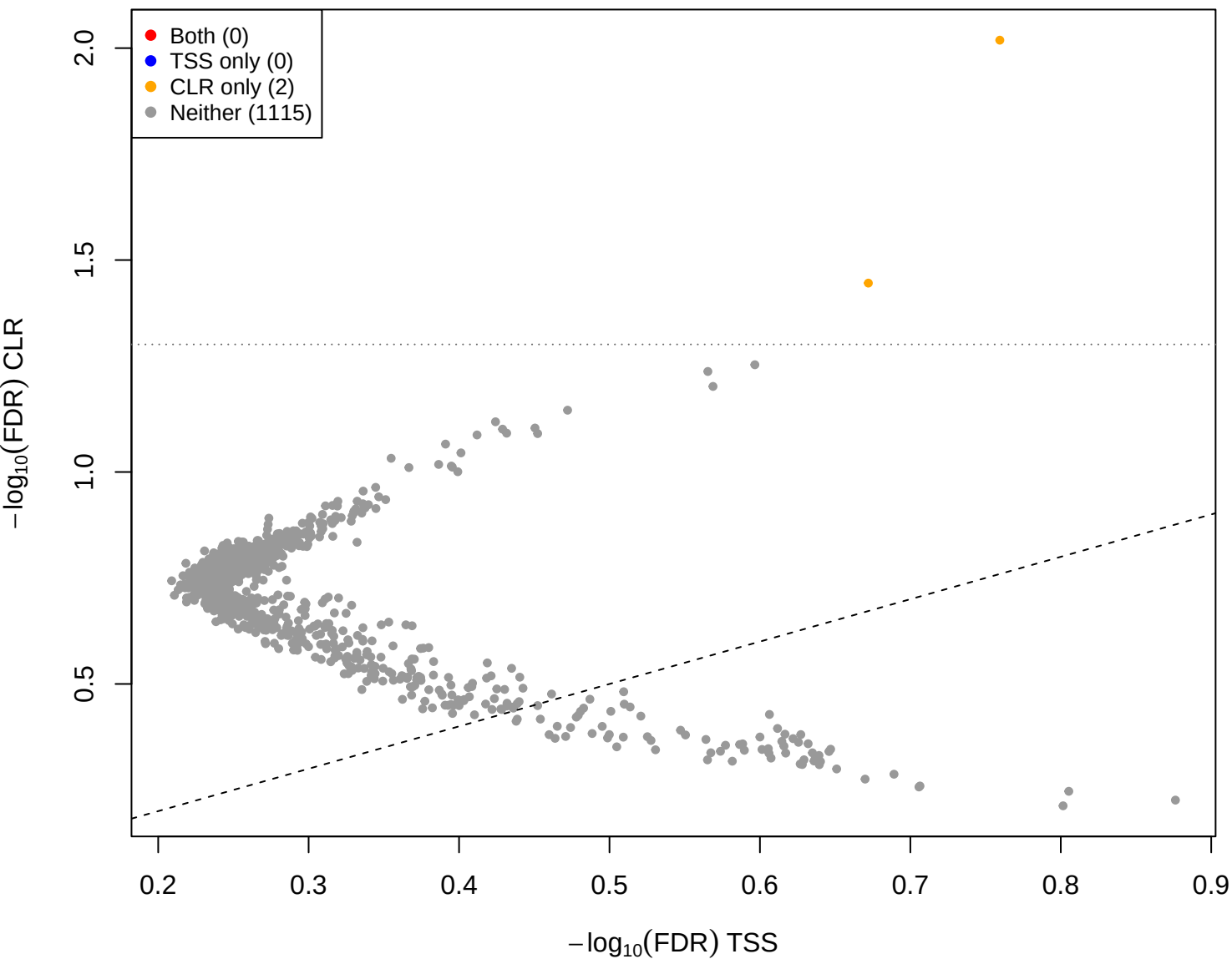
kin vs mid – CLR(const=-3) vs TSS (gamma = 3)
