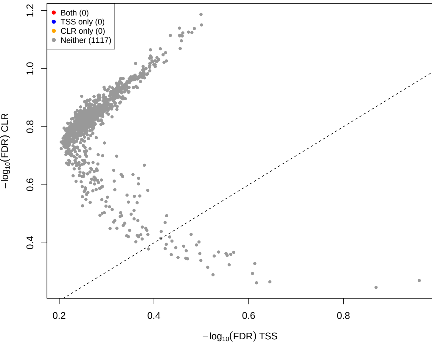
eld vs mage - CLR(const=-3) vs TSS (gamma = 3)
