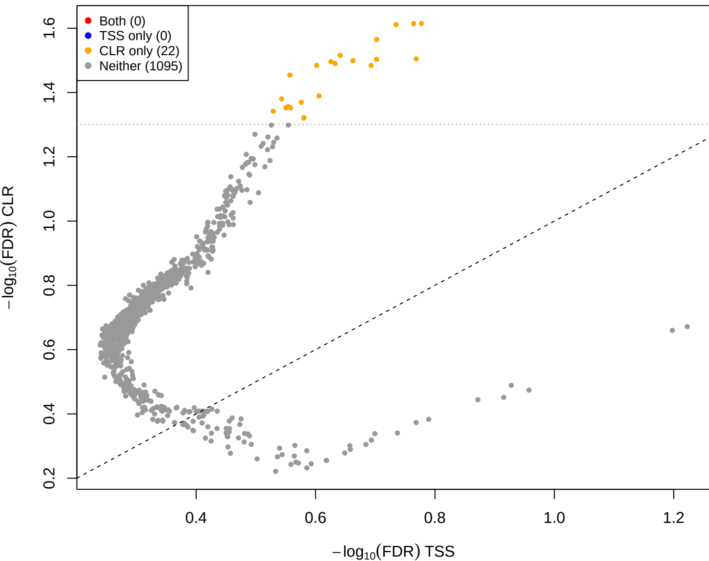
cent vs kin - CLR(const=-3) vs TSS (gamma = 3)
