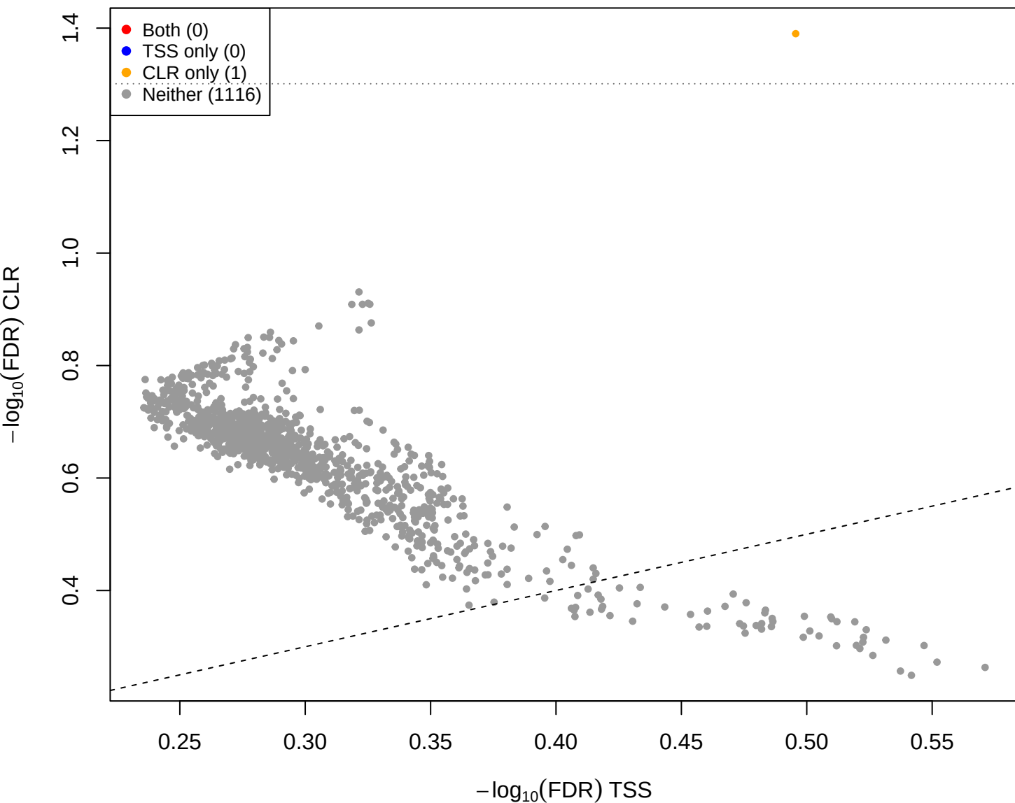
mage vs mid - CLR(const=-3) vs TSS (gamma = 3)
