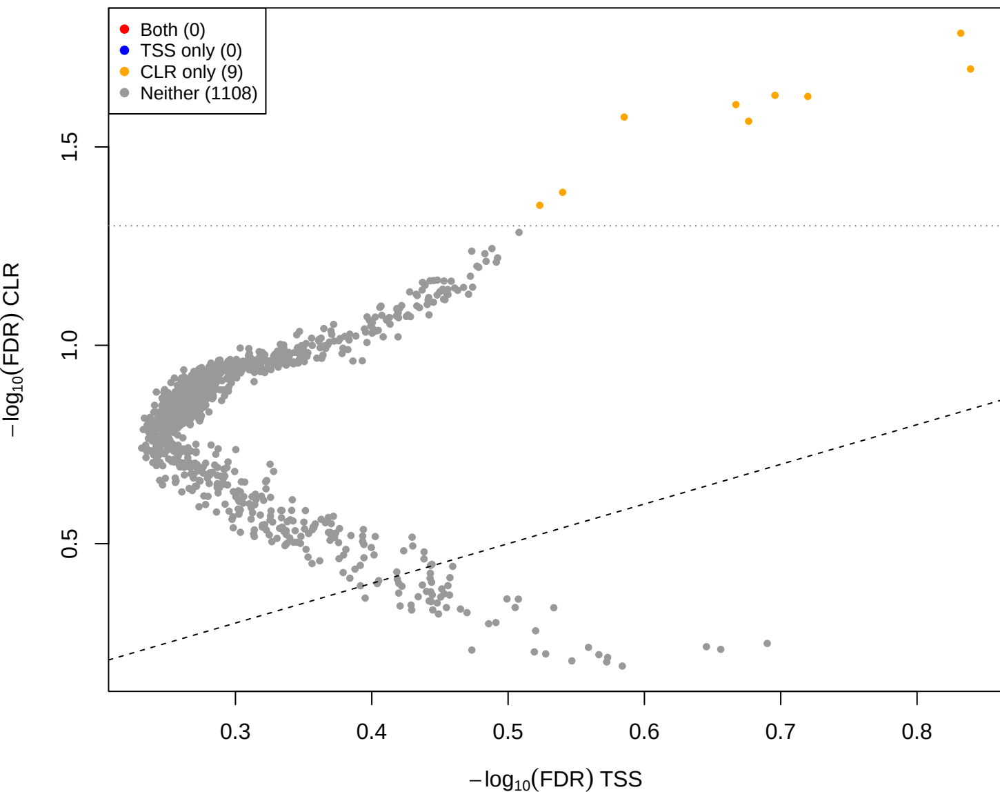
cent vs mage – CLR(const=-3) vs TSS (gamma = 3)
