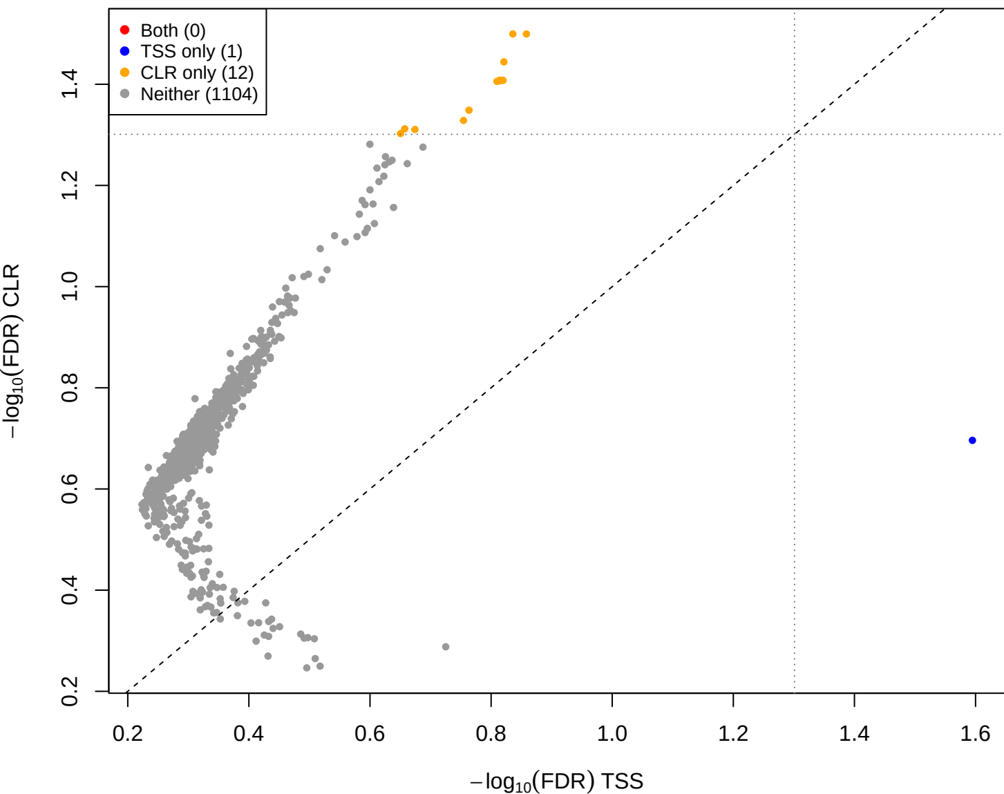
mage vs pup – CLR(const=-3) vs TSS (gamma = 3)
