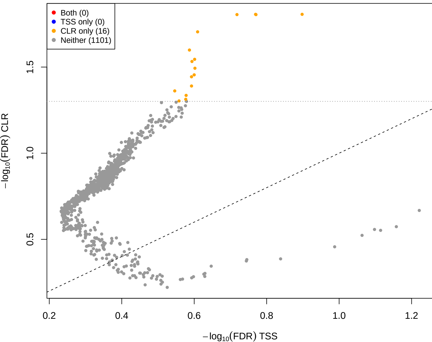
cent vs mid – CLR(const=-3) vs TSS (gamma = 3)
