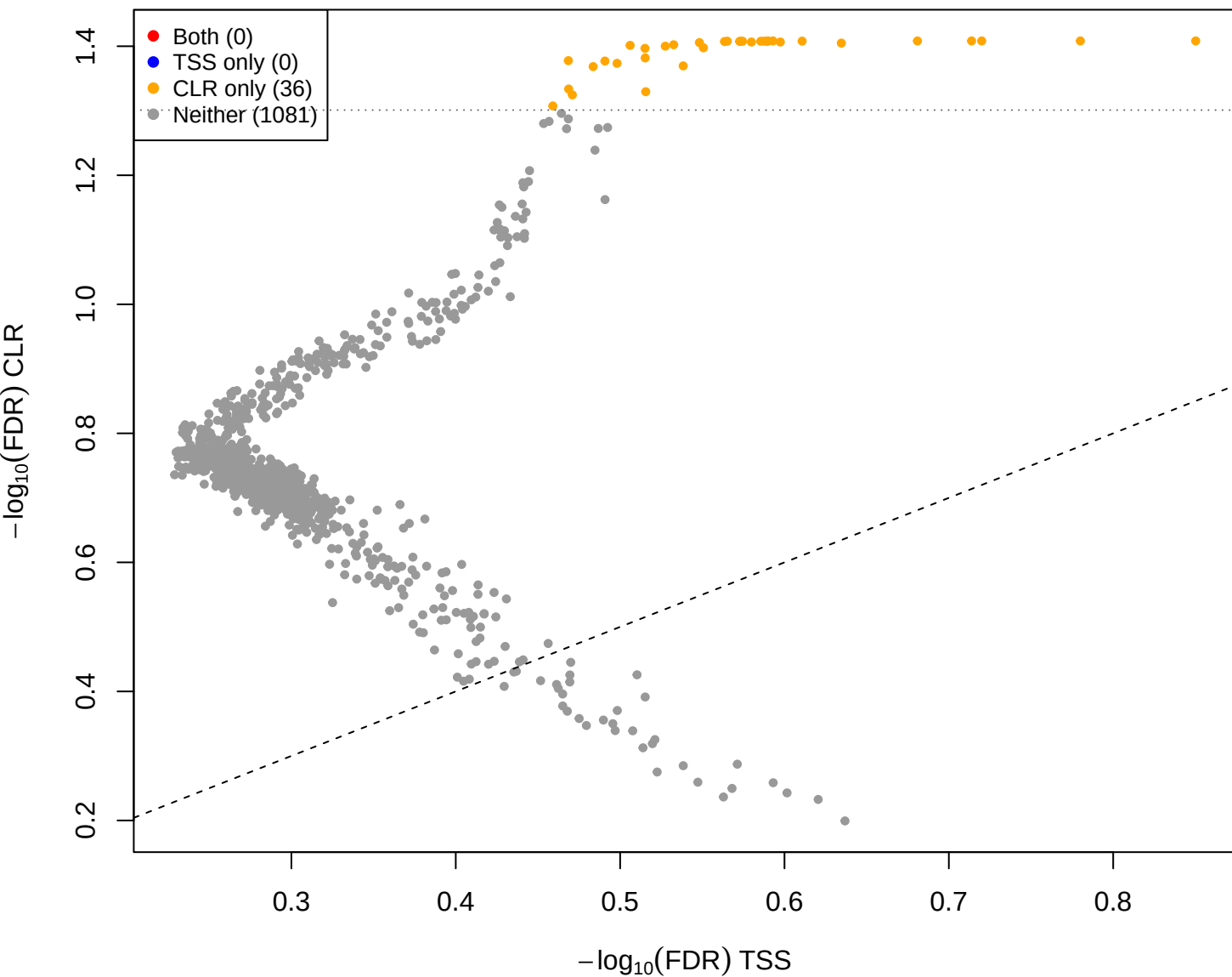
mage vs you - CLR(const=-3) vs TSS (gamma = 3)
