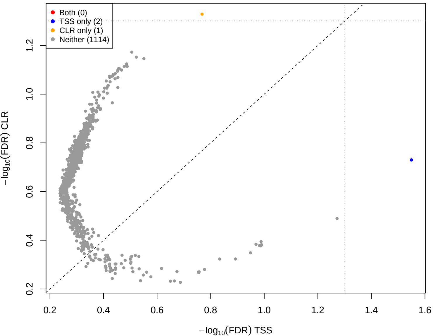
eld vs mid – CLR(const=-3) vs TSS (gamma = 3)
