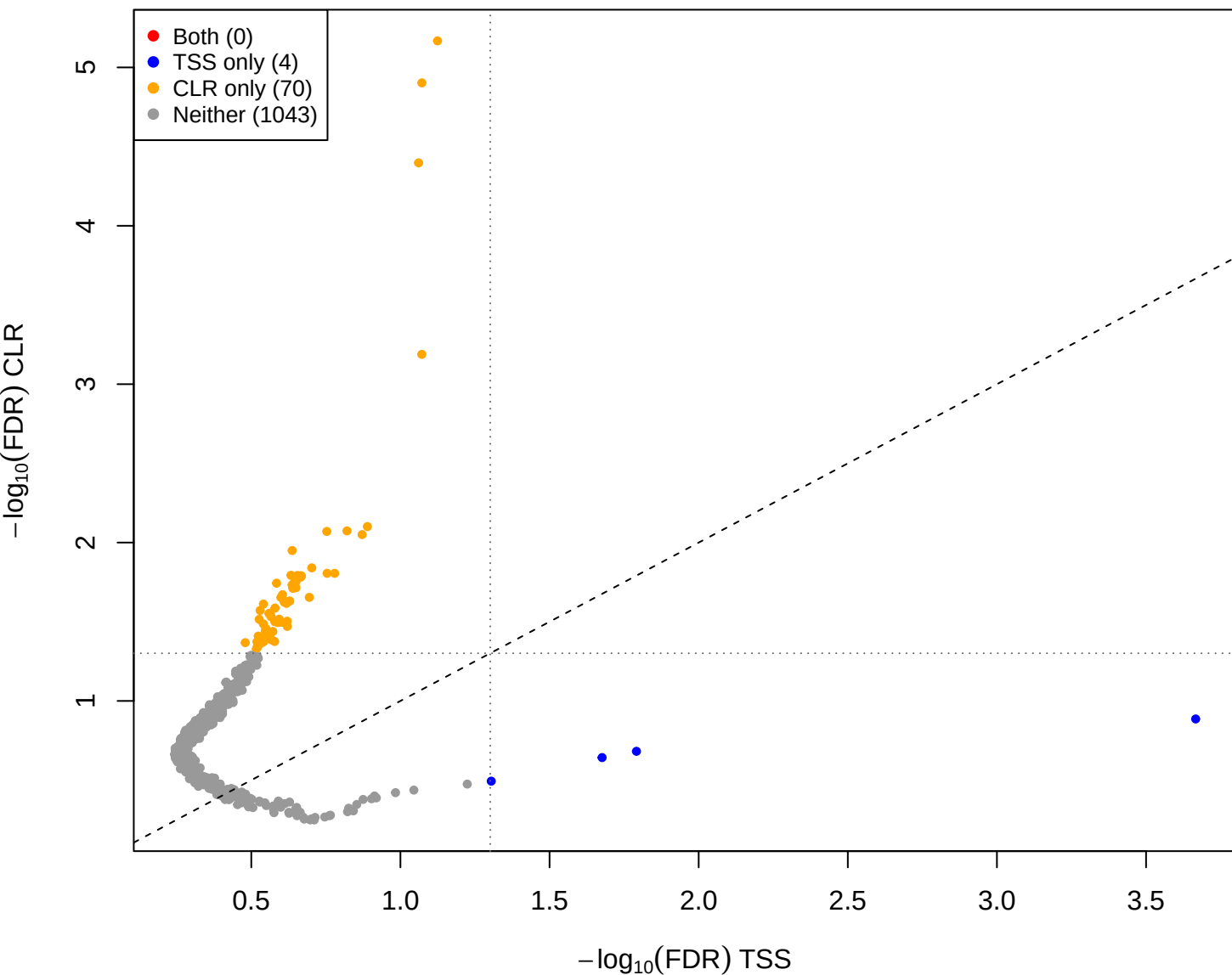
cent vs pup – CLR(const=-3) vs TSS (gamma = 3)
