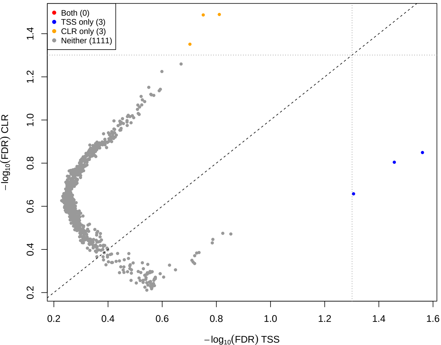
eld vs kin - CLR(const=-3) vs TSS (gamma = 3)
