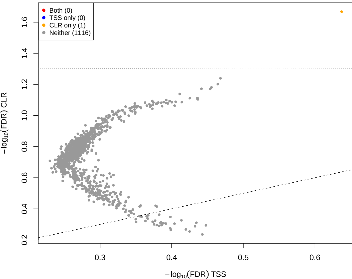
kin vs mage – CLR(const=-3) vs TSS (gamma = 3)
