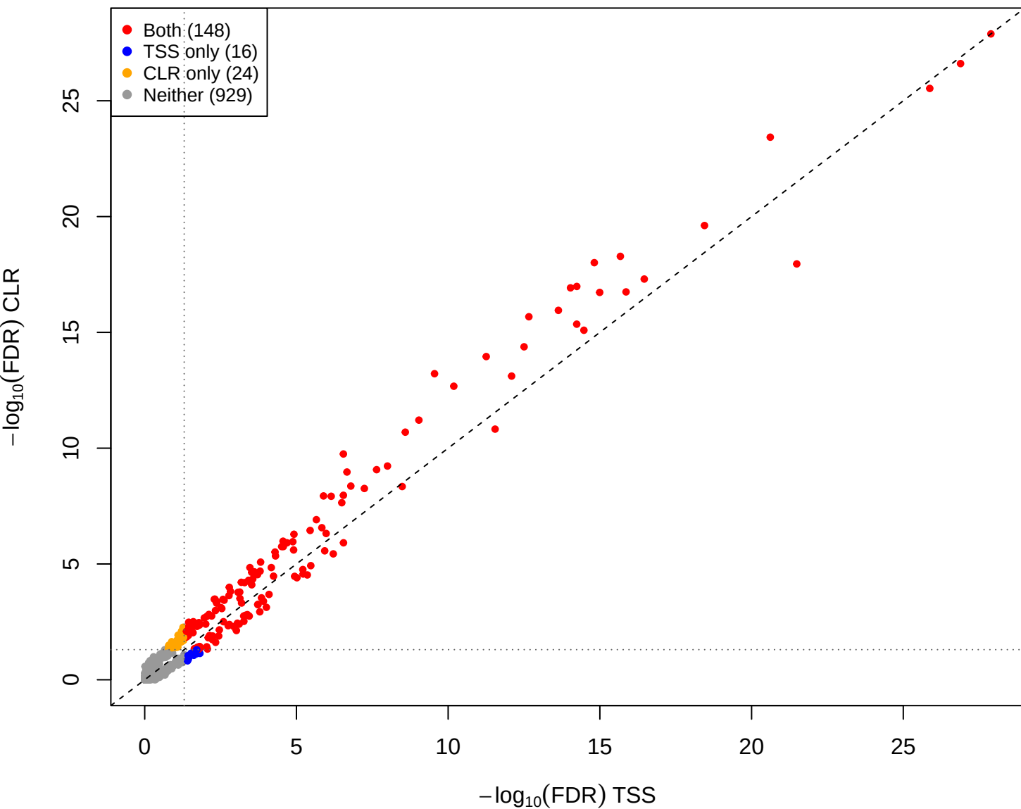
eld vs mid – CLR vs TSS(const=-0.1) (gamma = 0.001)
