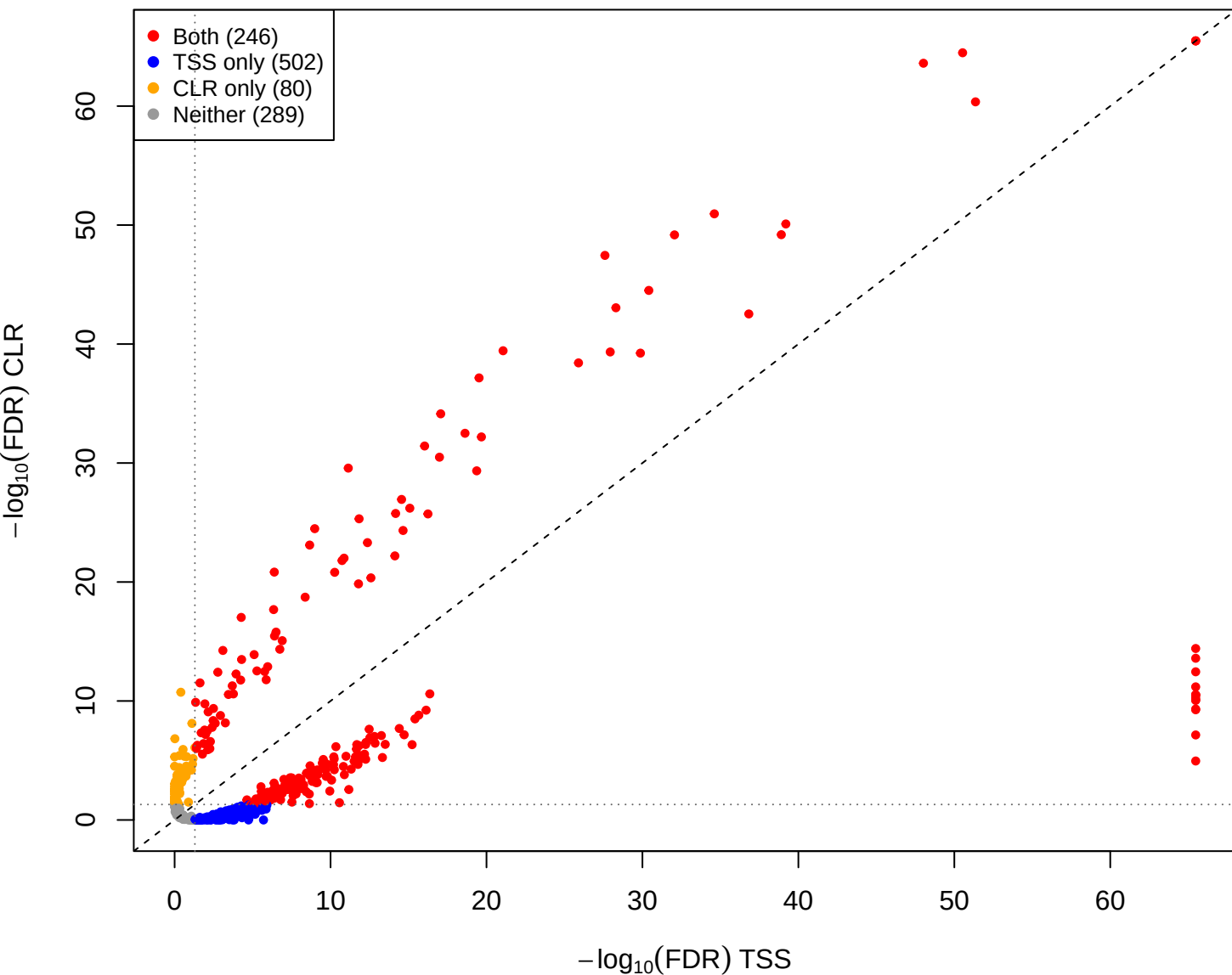
cent vs pup – CLR vs TSS(const=-0.4) (gamma = 0.001)
