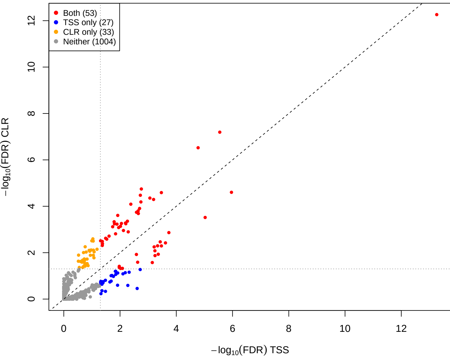
mage vs mid – CLR vs TSS(const=-0.4) (gamma = 0.001)
