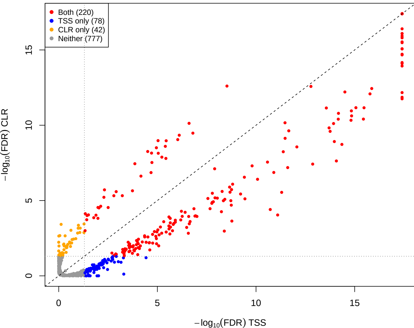
mid vs you – CLR vs TSS(const=-0.4) (gamma = 0.001)
