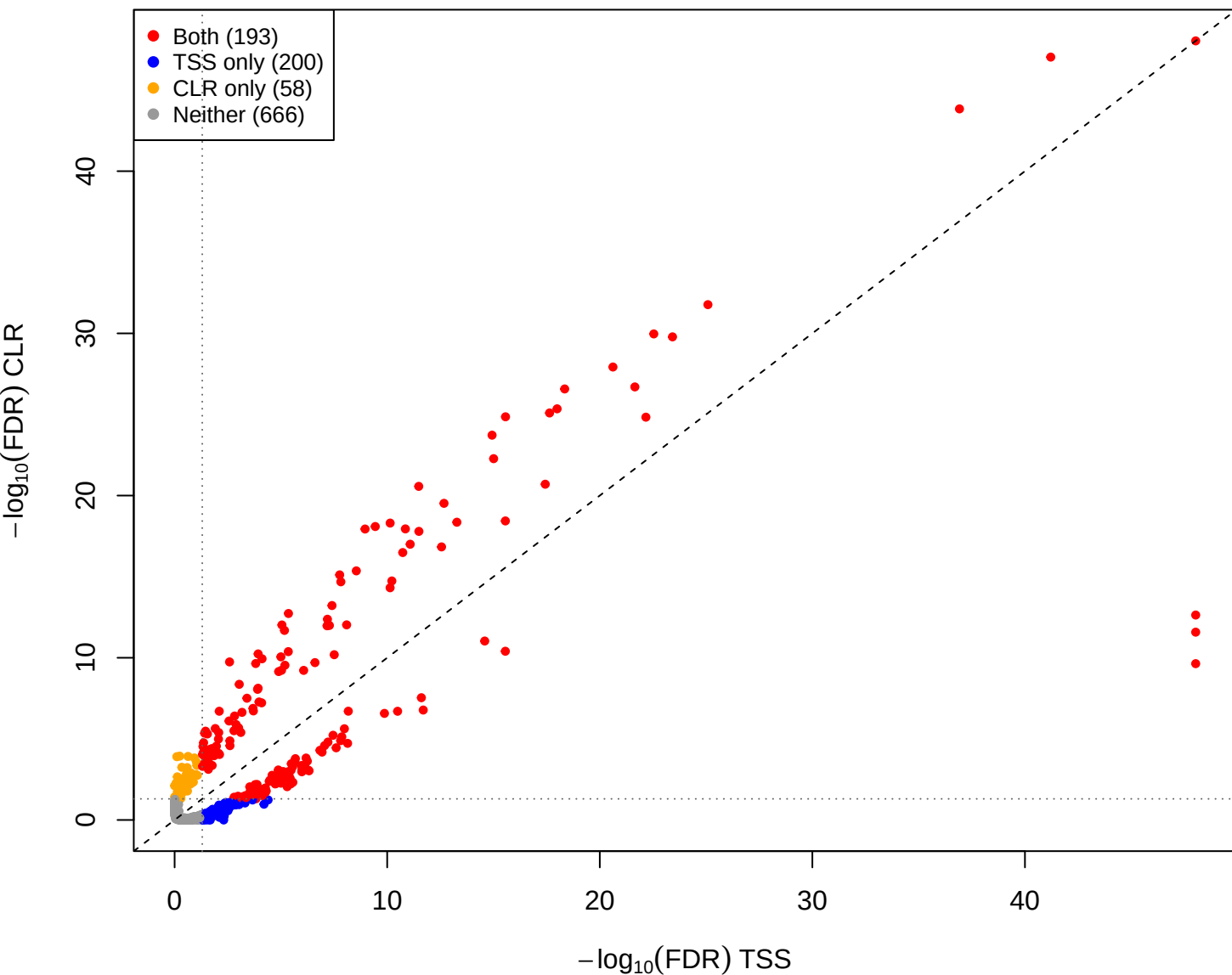
cent vs mid – CLR vs TSS(const=-0.4) (gamma = 0.001)
