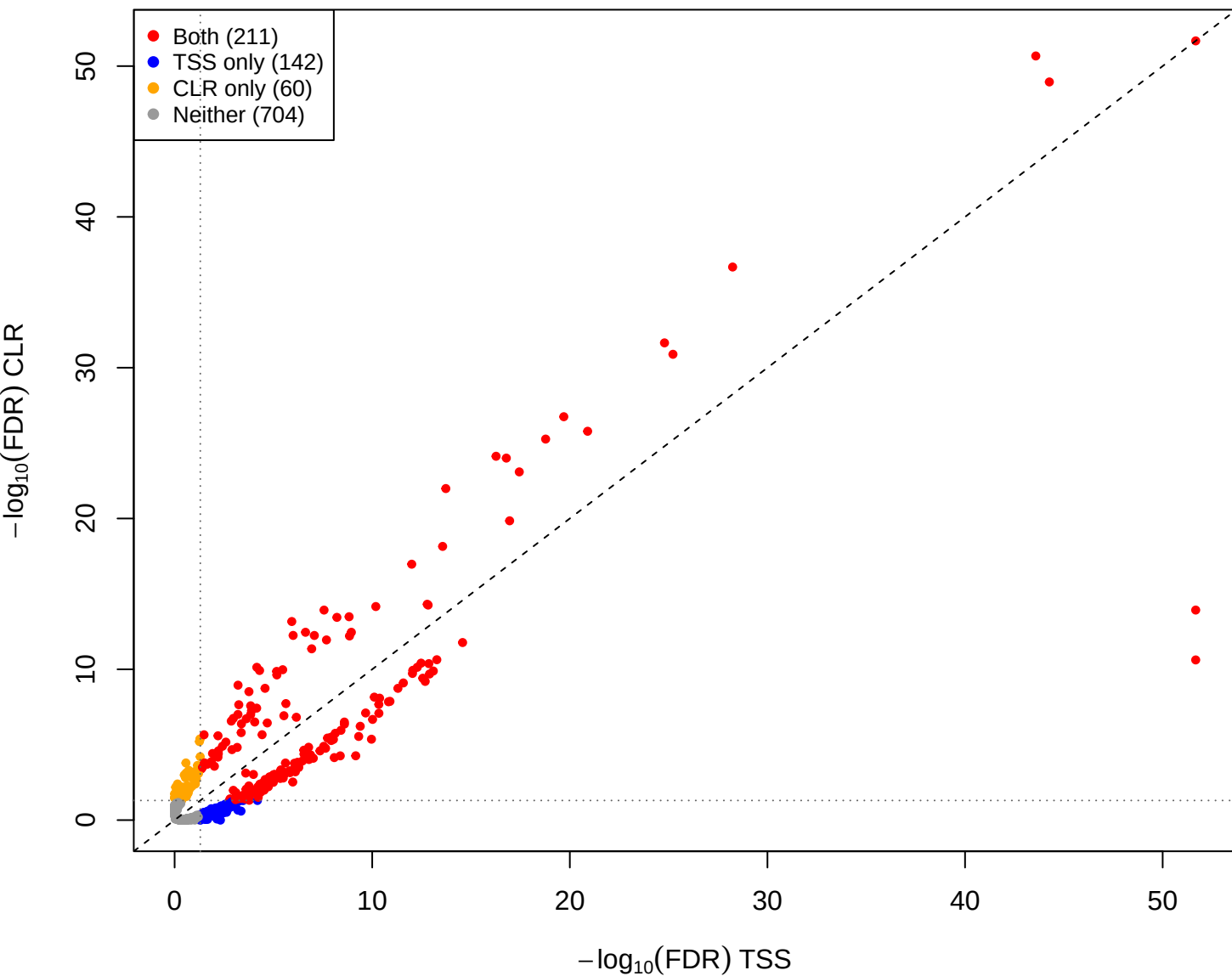
cent vs kin – CLR vs TSS(const=-0.4) (gamma = 0.001)
