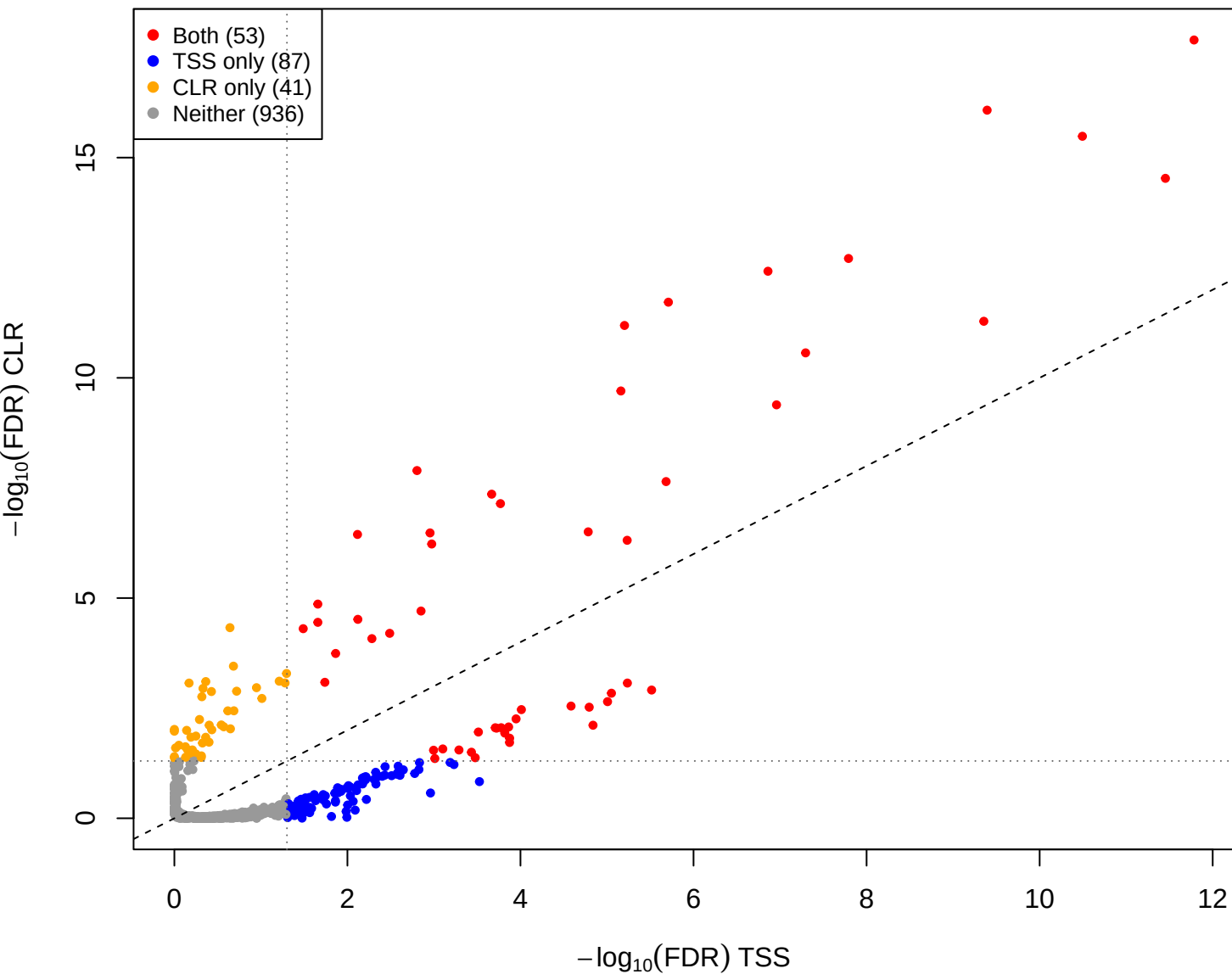
eld vs mage – CLR vs TSS(const=-0.4) (gamma = 0.001)
