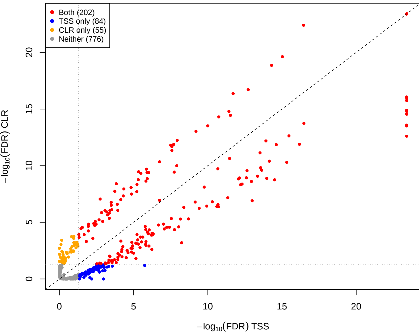
kin vs you – CLR vs TSS(const=-0.4) (gamma = 0.001)
