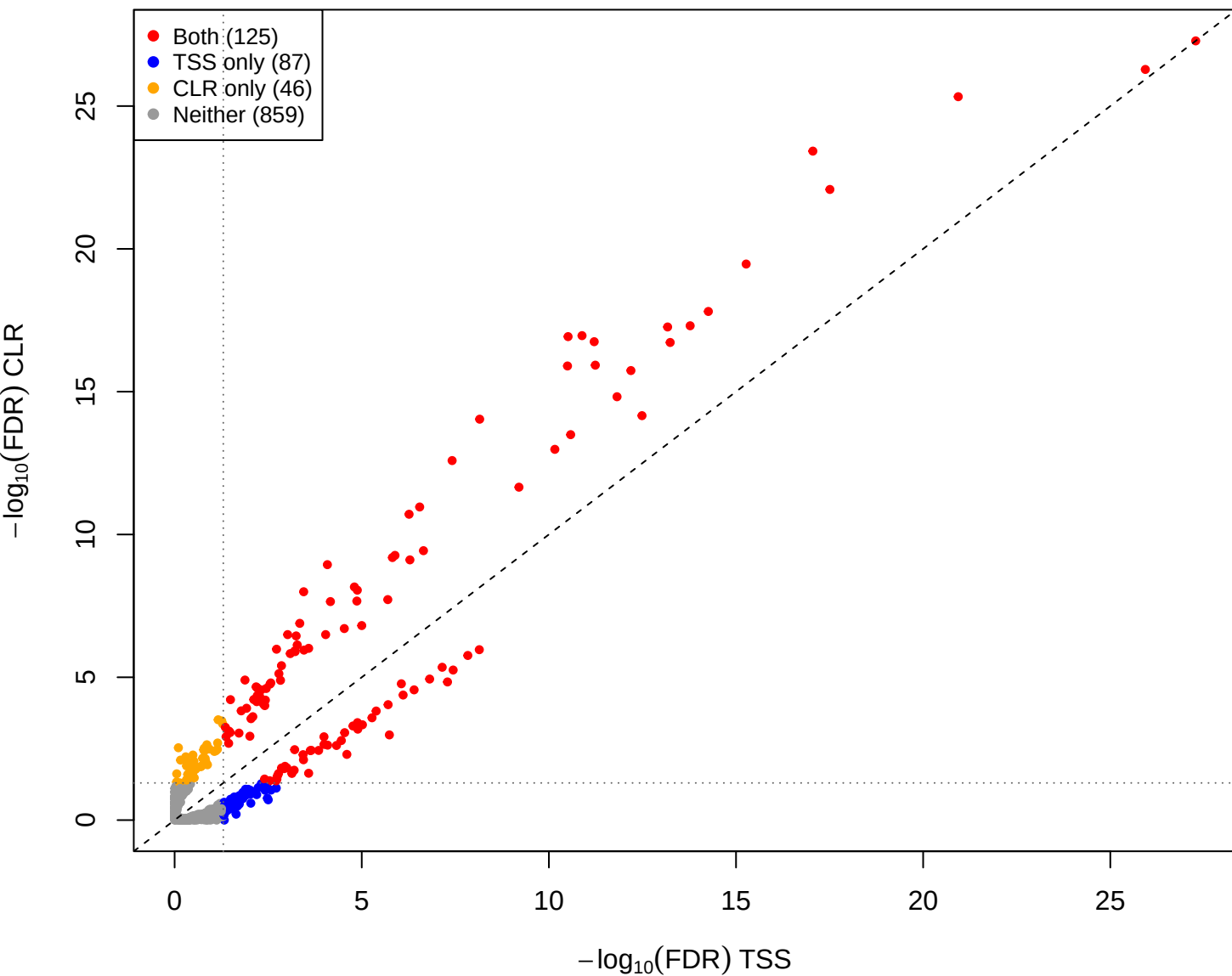
eld vs mid – CLR vs TSS(const=-0.4) (gamma = 0.001)
