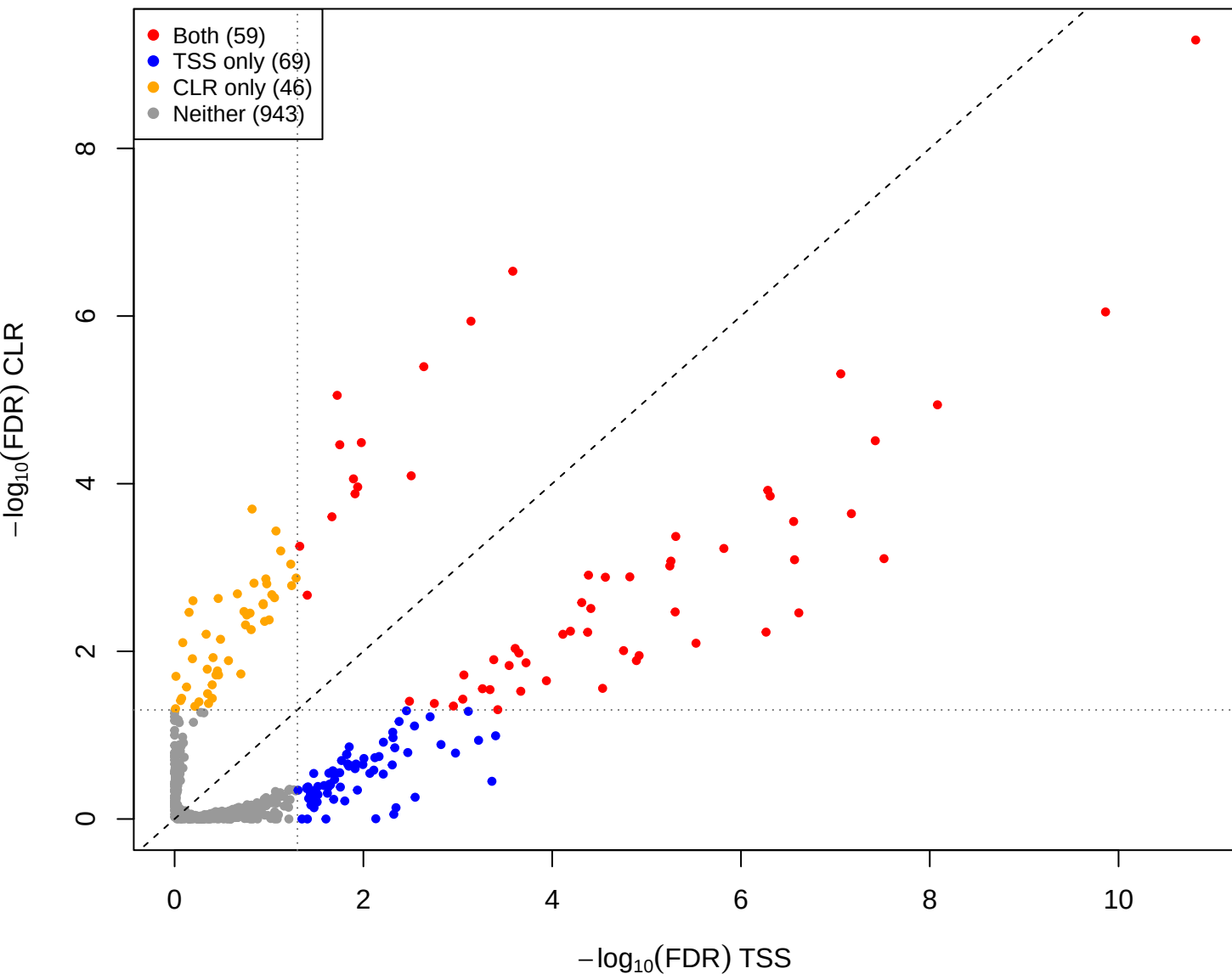
kin vs mage – CLR vs TSS(const=-0.4) (gamma = 0.001)
