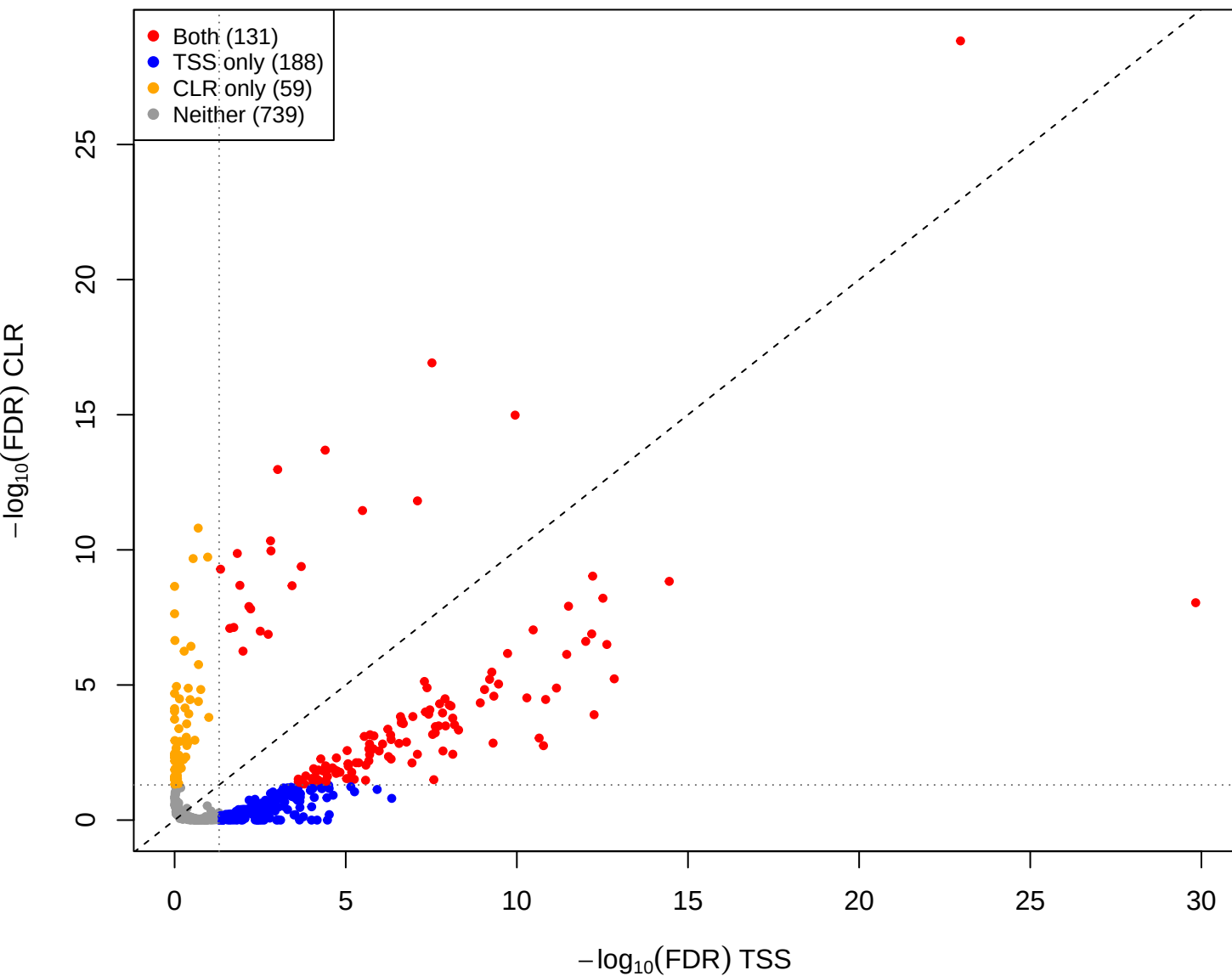
mid vs pup – CLR vs TSS(const=-0.4) (gamma = 0.001)
