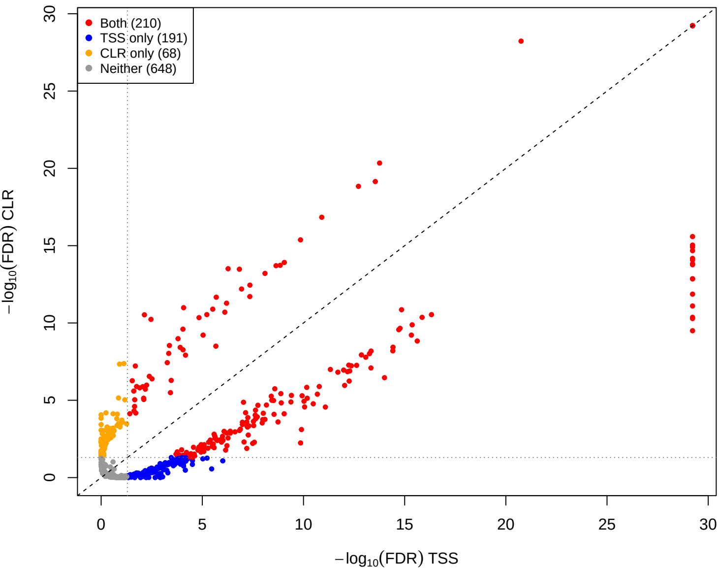
cent vs you – CLR vs TSS(const=-0.4) (gamma = 0.001)
