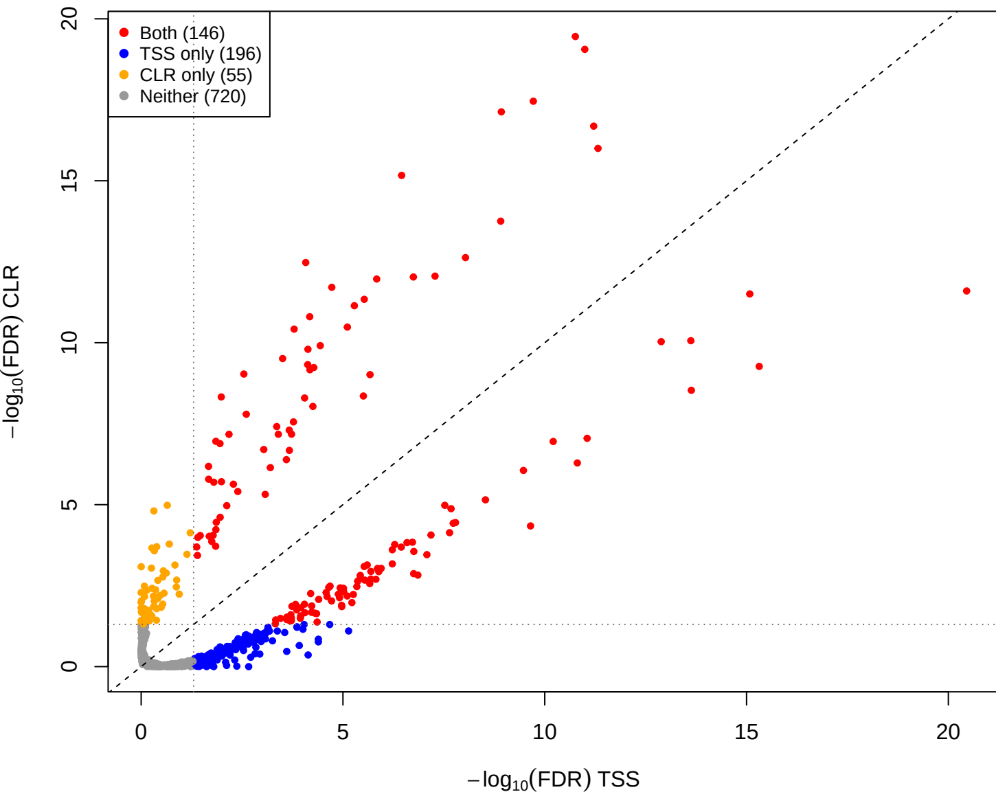
cent vs mage - CLR vs TSS(const=-0.4) (gamma = 0.001)
