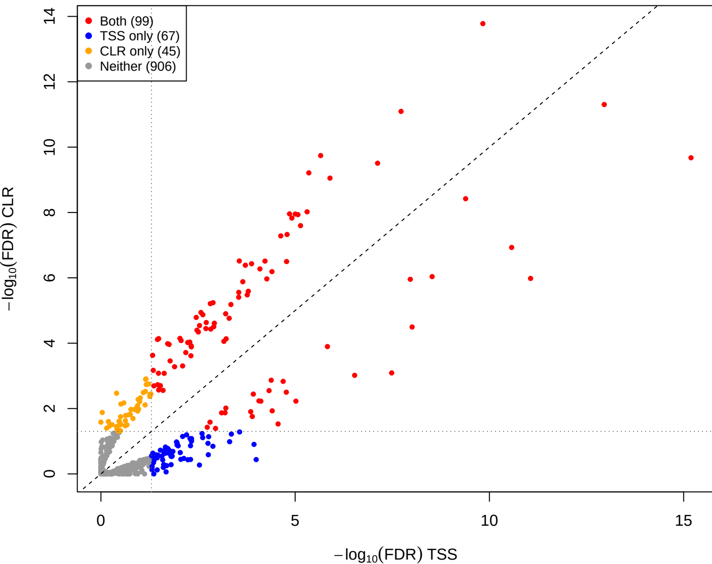
kin vs mid – CLR vs TSS(const=-0.4) (gamma = 0.001)
