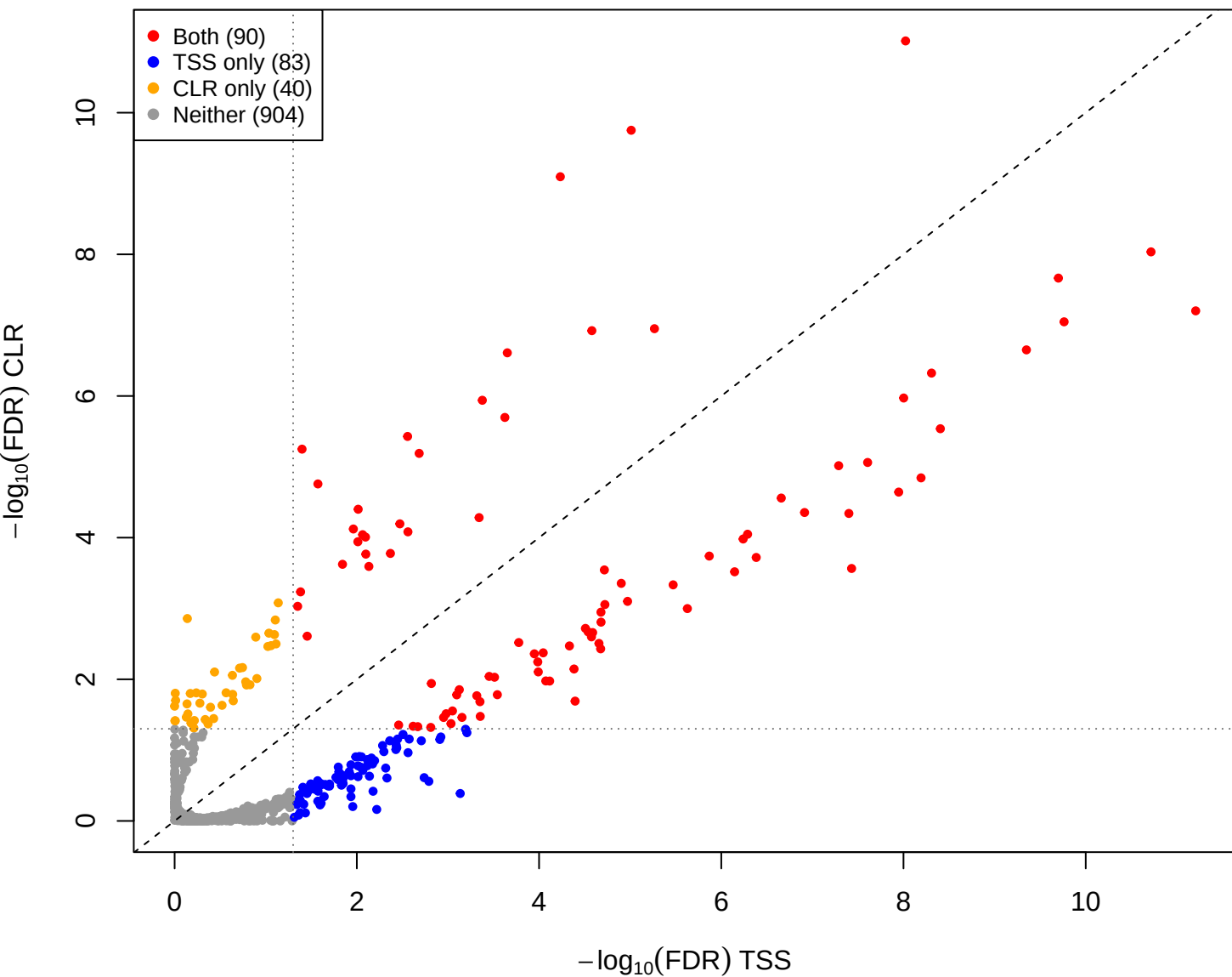
cent vs eld – CLR vs TSS(const=-0.4) (gamma = 0.001)
