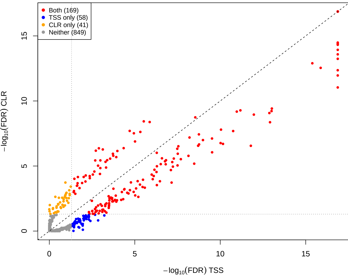
mage vs you – CLR vs TSS(const=-0.4) (gamma = 0.001)
