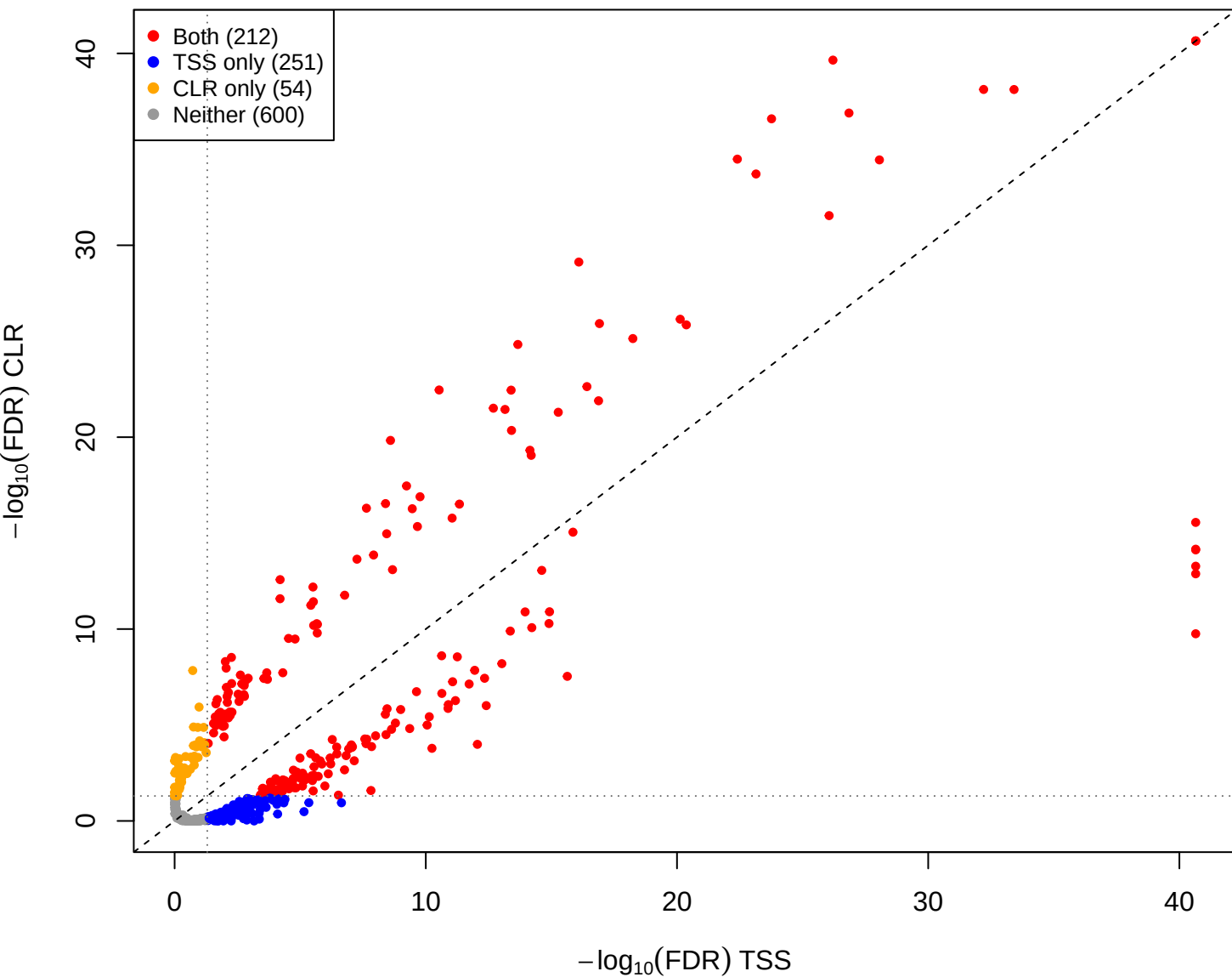
eld vs pup – CLR vs TSS(const=-0.4) (gamma = 0.001)
