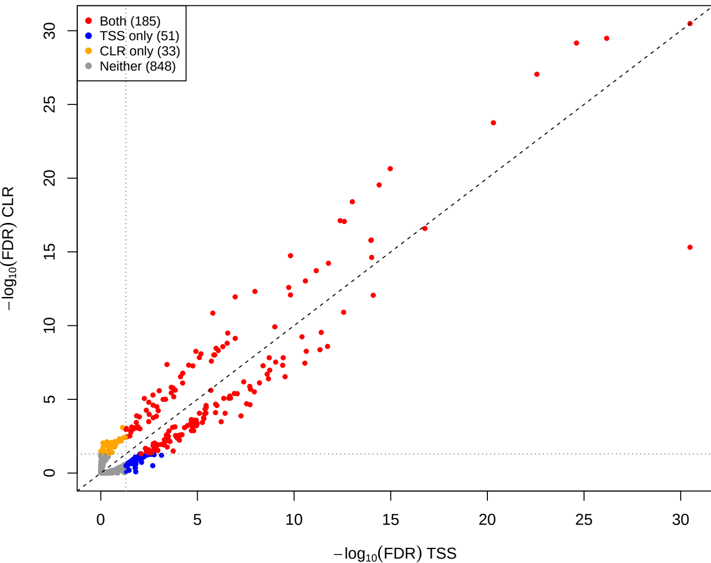
eld vs kin - CLR vs TSS(const=-0.4) (gamma = 0.001)
