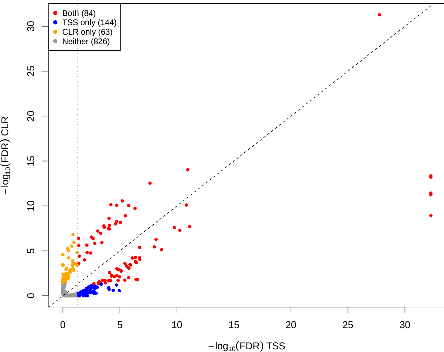
mage vs pup – CLR vs TSS(const=-0.4) (gamma = 0.001)
