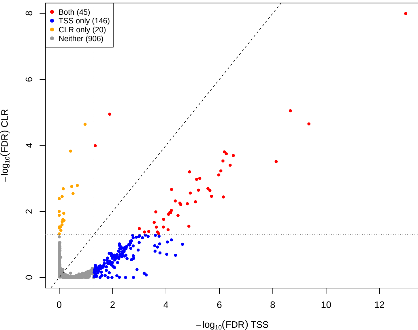
eld vs you – CLR vs TSS(const=-0.4) (gamma = 0.001)
