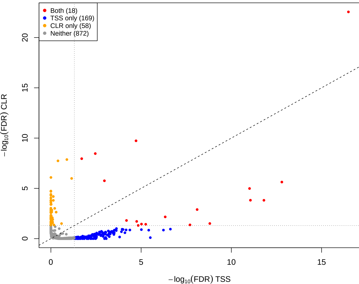
kin vs pup – CLR vs TSS(const=-0.4) (gamma = 0.001)
