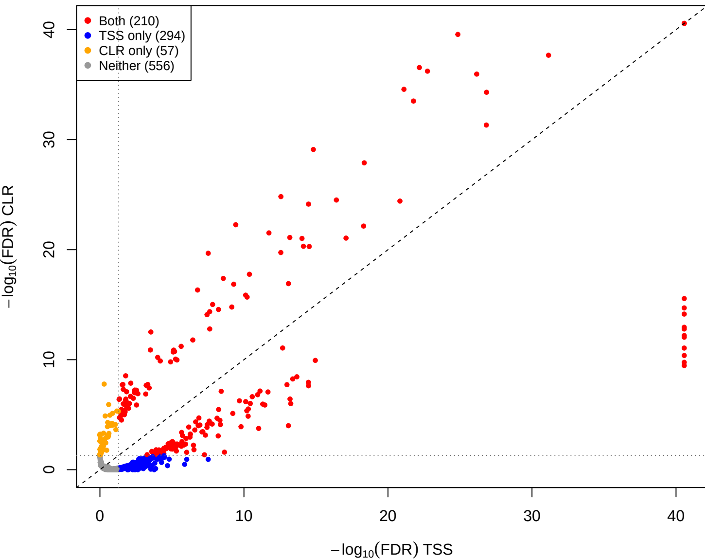
eld vs pup – CLR vs TSS(const=-0.5) (gamma = 0.001)
