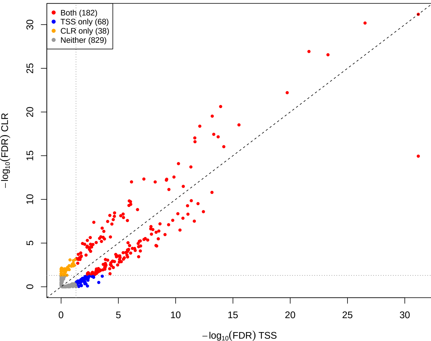
eld vs kin - CLR vs TSS(const=-0.5) (gamma = 0.001)
