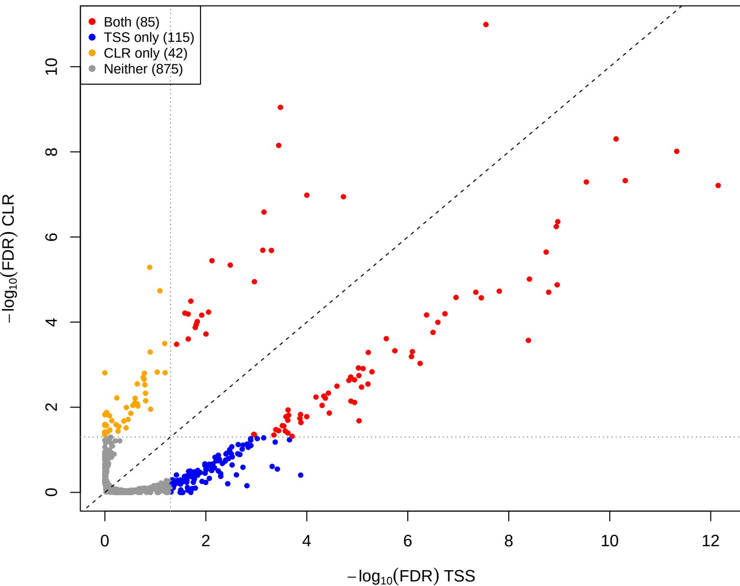
cent vs eld – CLR vs TSS(const=-0.5) (gamma = 0.001)
