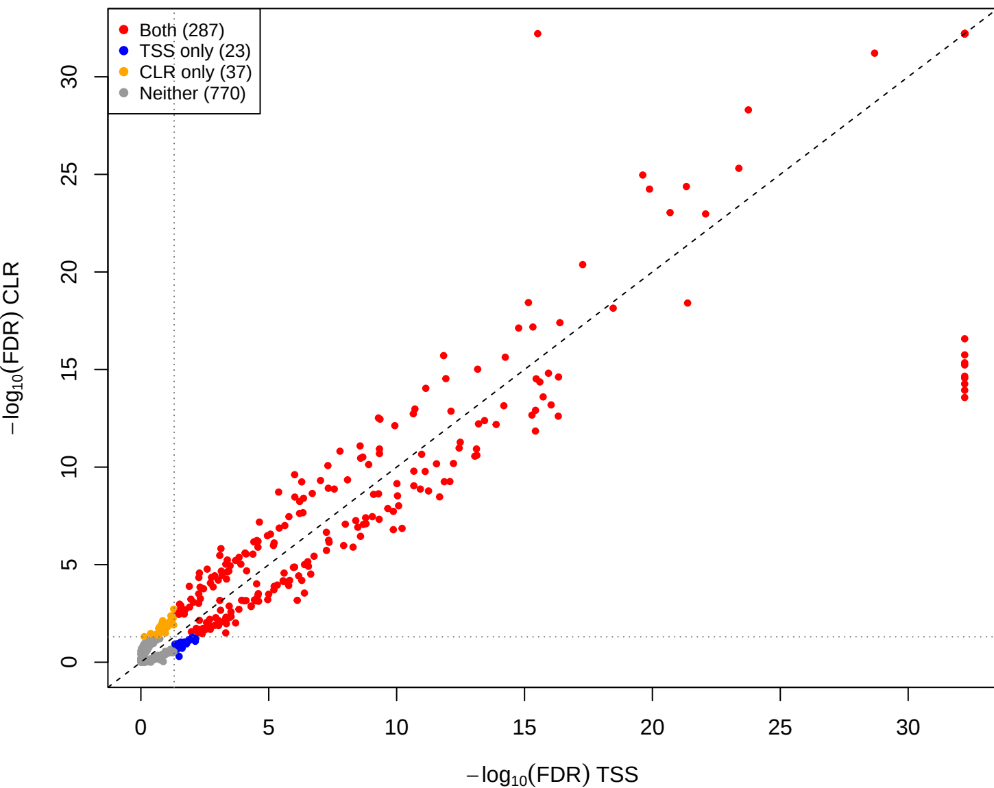
pup vs you – CLR vs TSS(const=-0.5) (gamma = 0.001)
