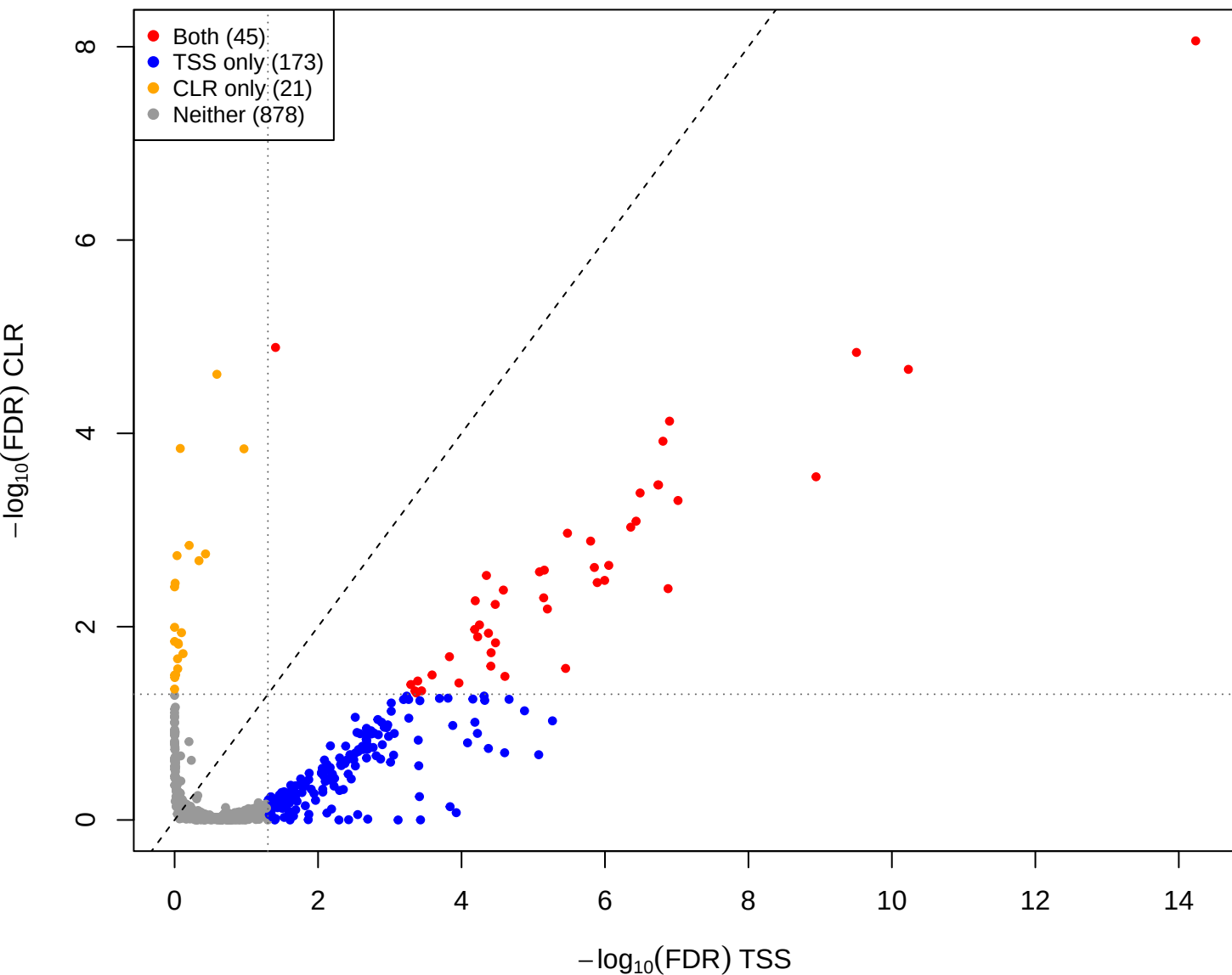
eld vs you – CLR vs TSS(const=-0.5) (gamma = 0.001)
