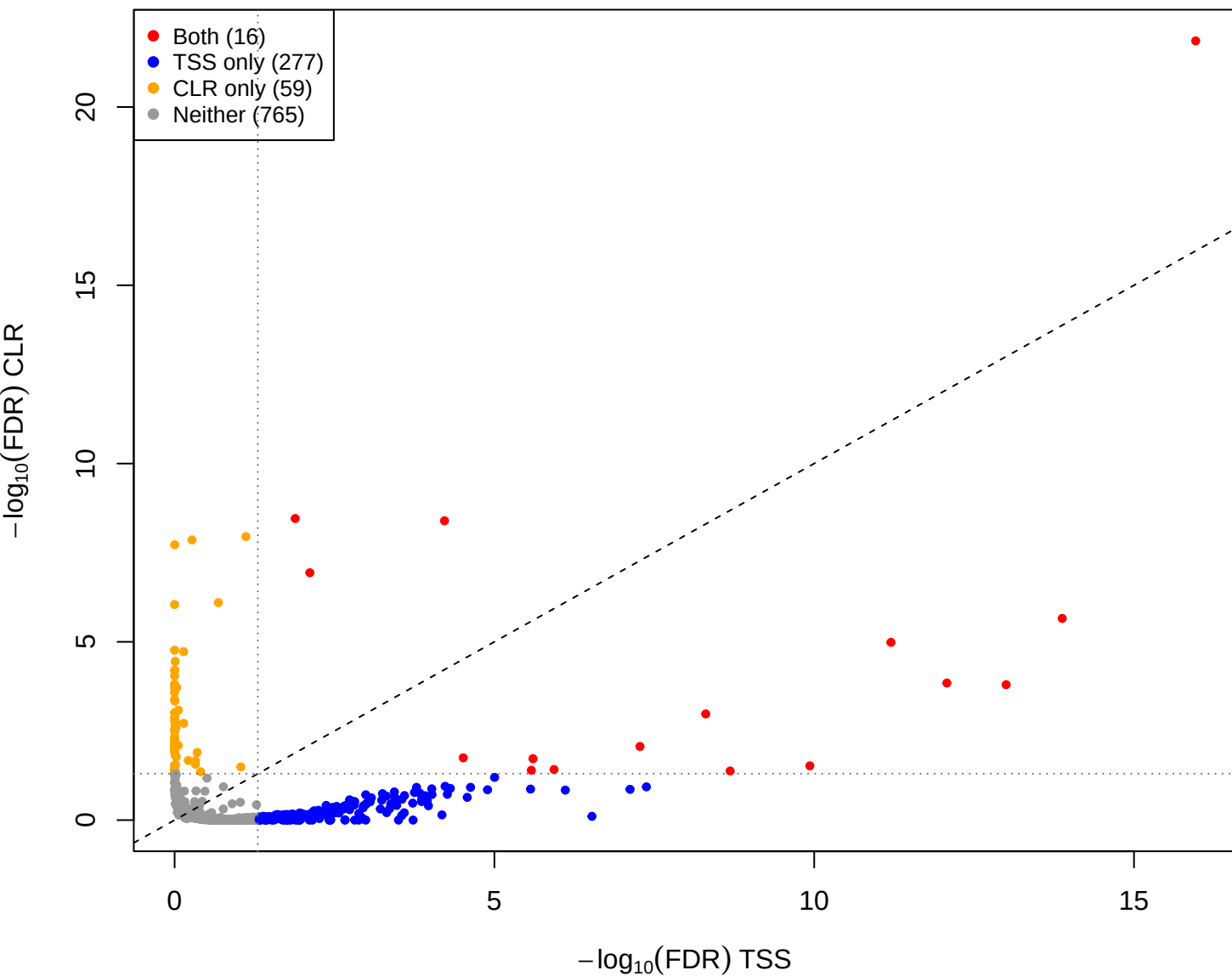
kin vs pup – CLR vs TSS(const=-0.5) (gamma = 0.001)
