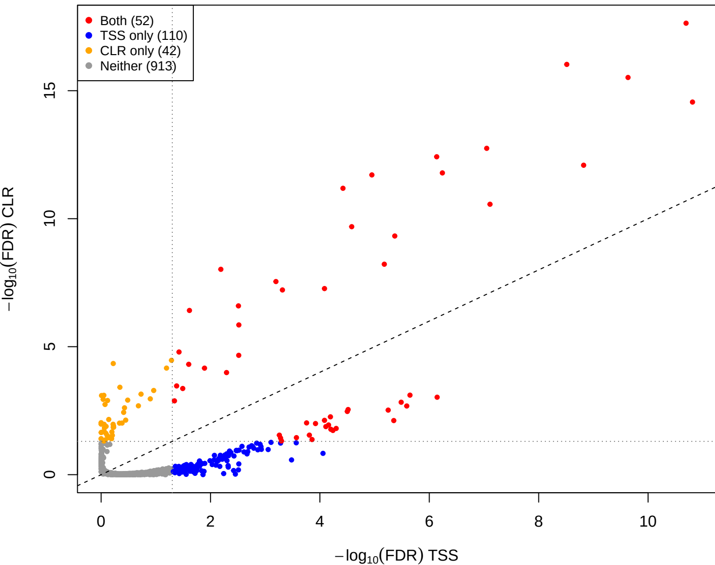
eld vs mage – CLR vs TSS(const=-0.5) (gamma = 0.001)
