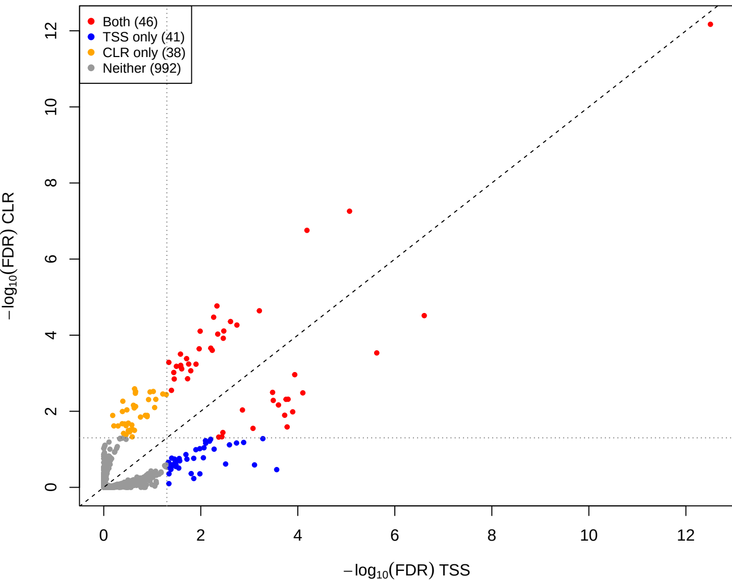
mage vs mid – CLR vs TSS(const=-0.5) (gamma = 0.001)
