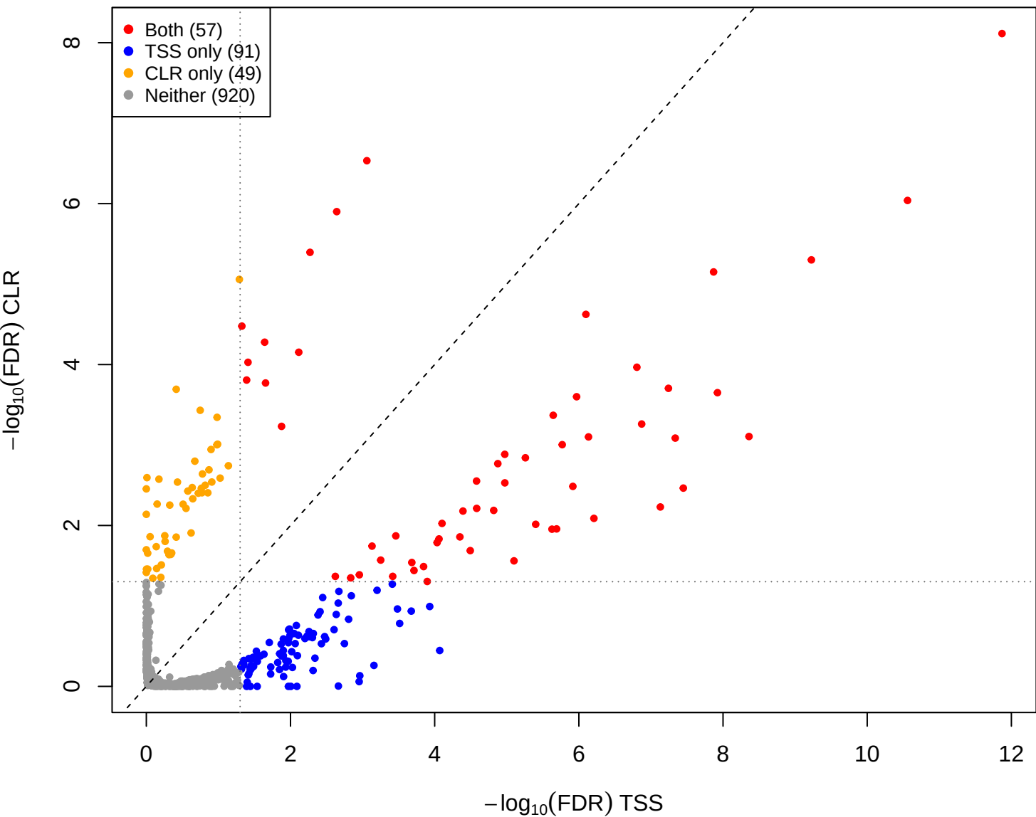
kin vs mage – CLR vs TSS(const=-0.5) (gamma = 0.001)
