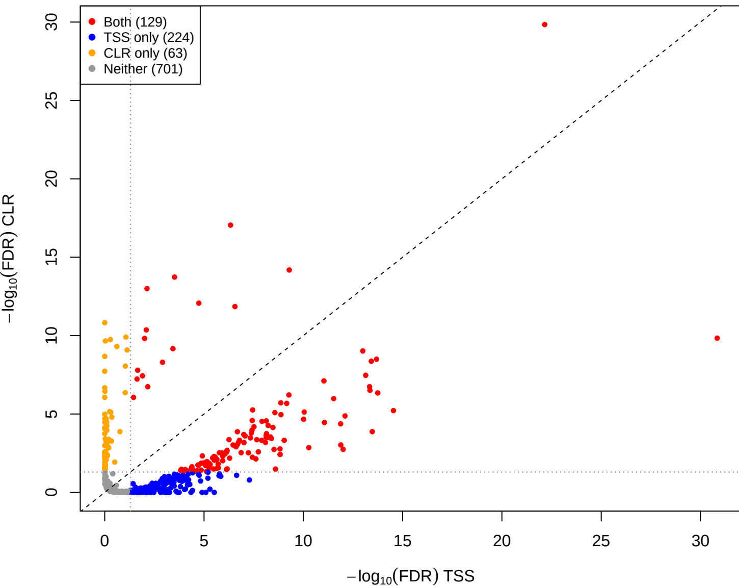
mid vs pup – CLR vs TSS(const=-0.5) (gamma = 0.001)
