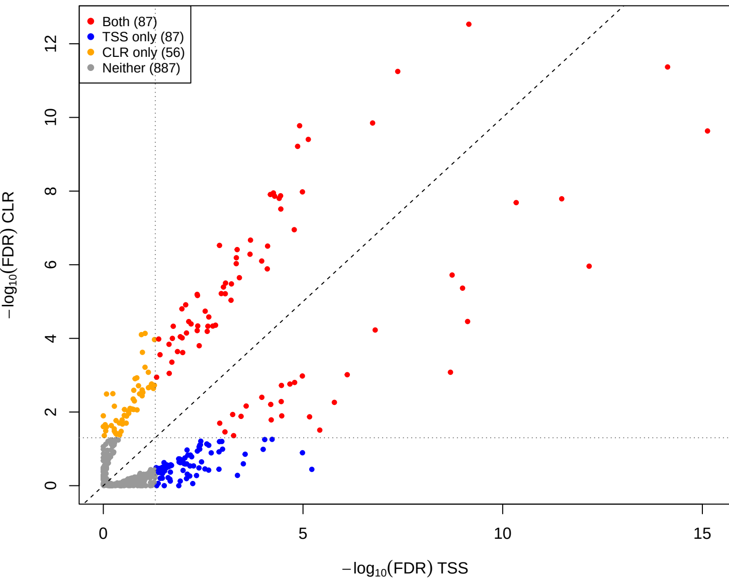
kin vs mid – CLR vs TSS(const=-0.5) (gamma = 0.001)
