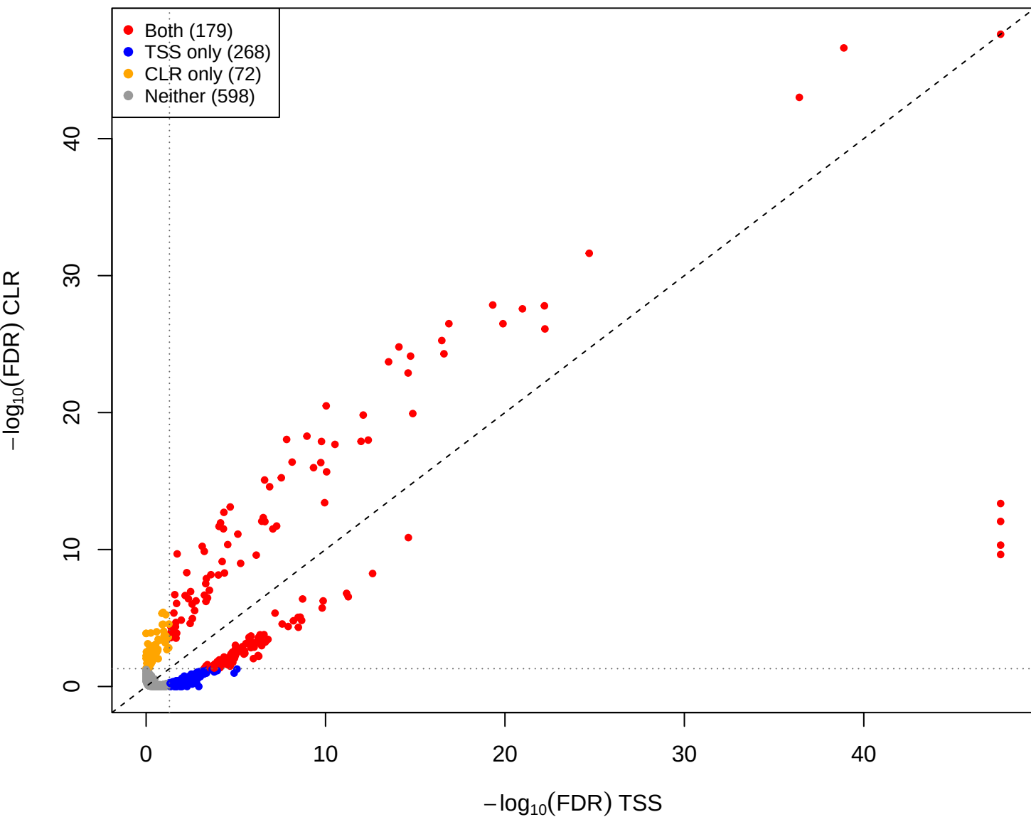
cent vs mid – CLR vs TSS(const=-0.5) (gamma = 0.001)
