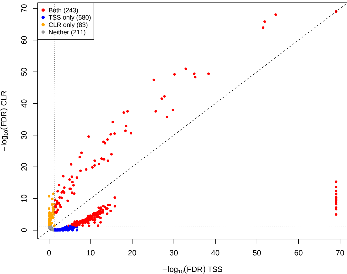
cent vs pup – CLR vs TSS(const=-0.5) (gamma = 0.001)
