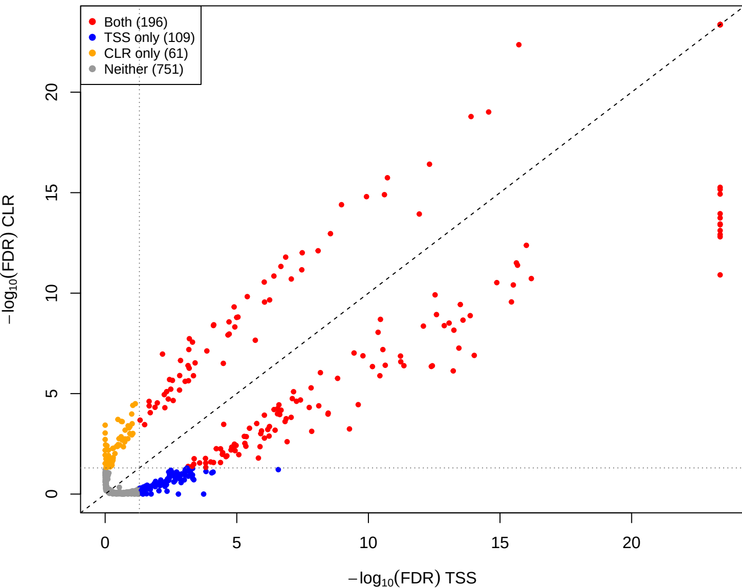
kin vs you – CLR vs TSS(const=-0.5) (gamma = 0.001)
