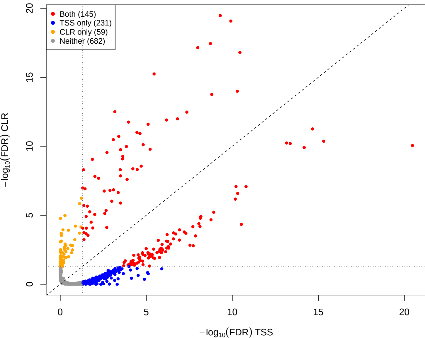
cent vs mage - CLR vs TSS(const=-0.5) (gamma = 0.001)
