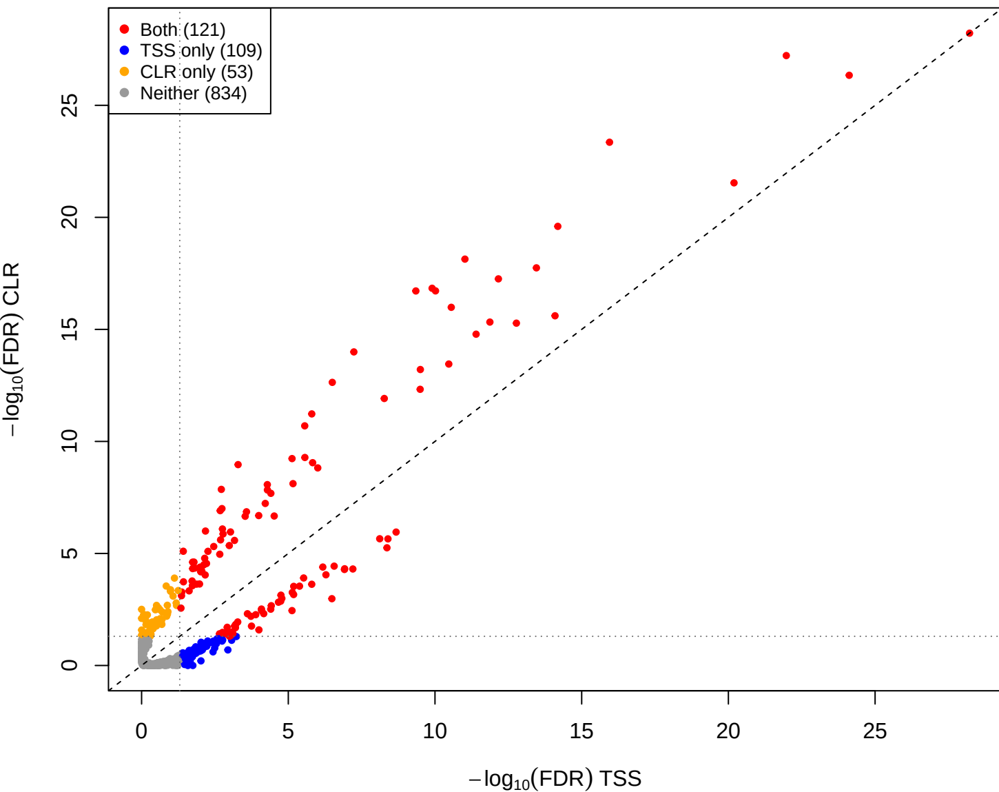
eld vs mid – CLR vs TSS(const=-0.5) (gamma = 0.001)
