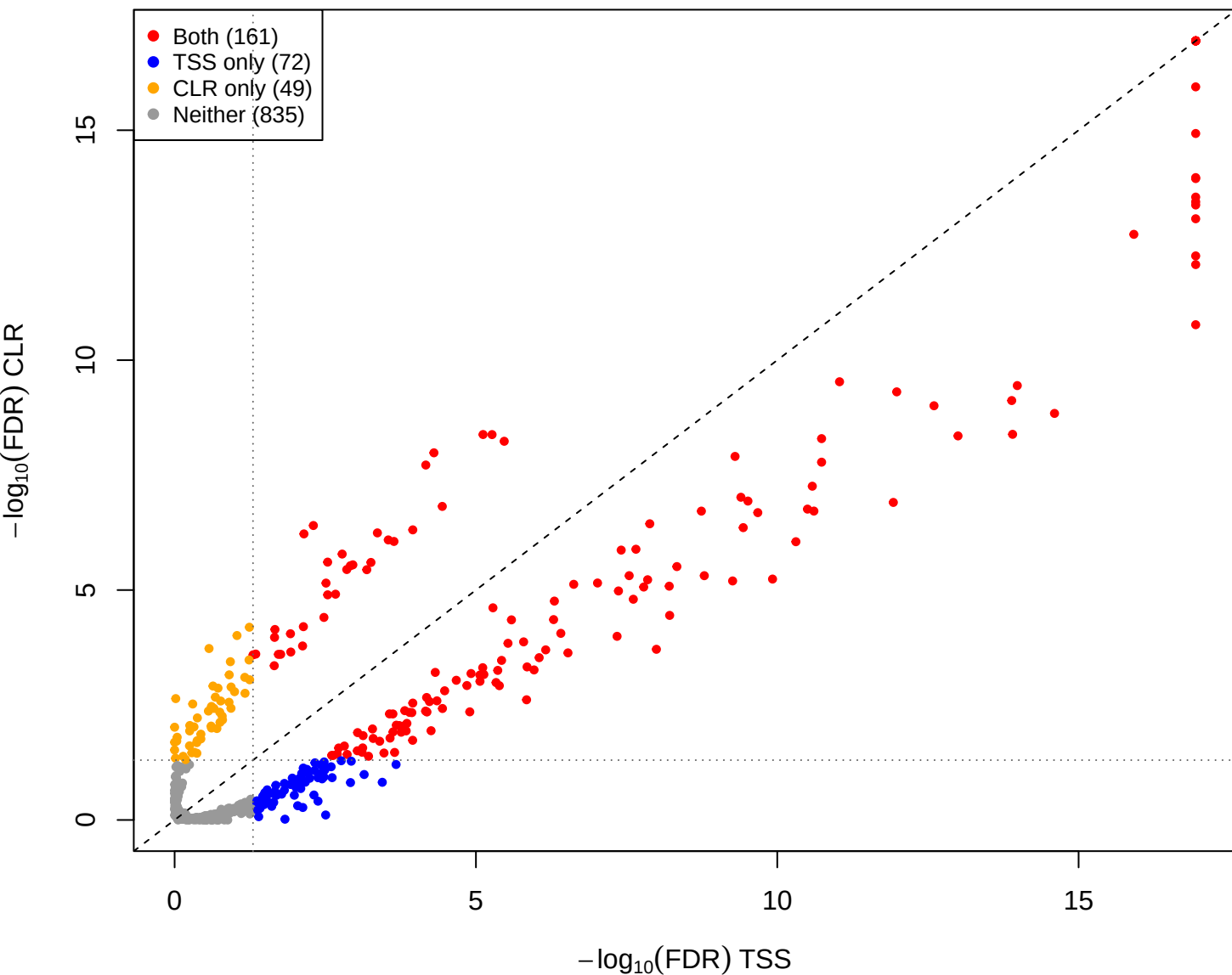
mage vs you – CLR vs TSS(const=-0.5) (gamma = 0.001)
