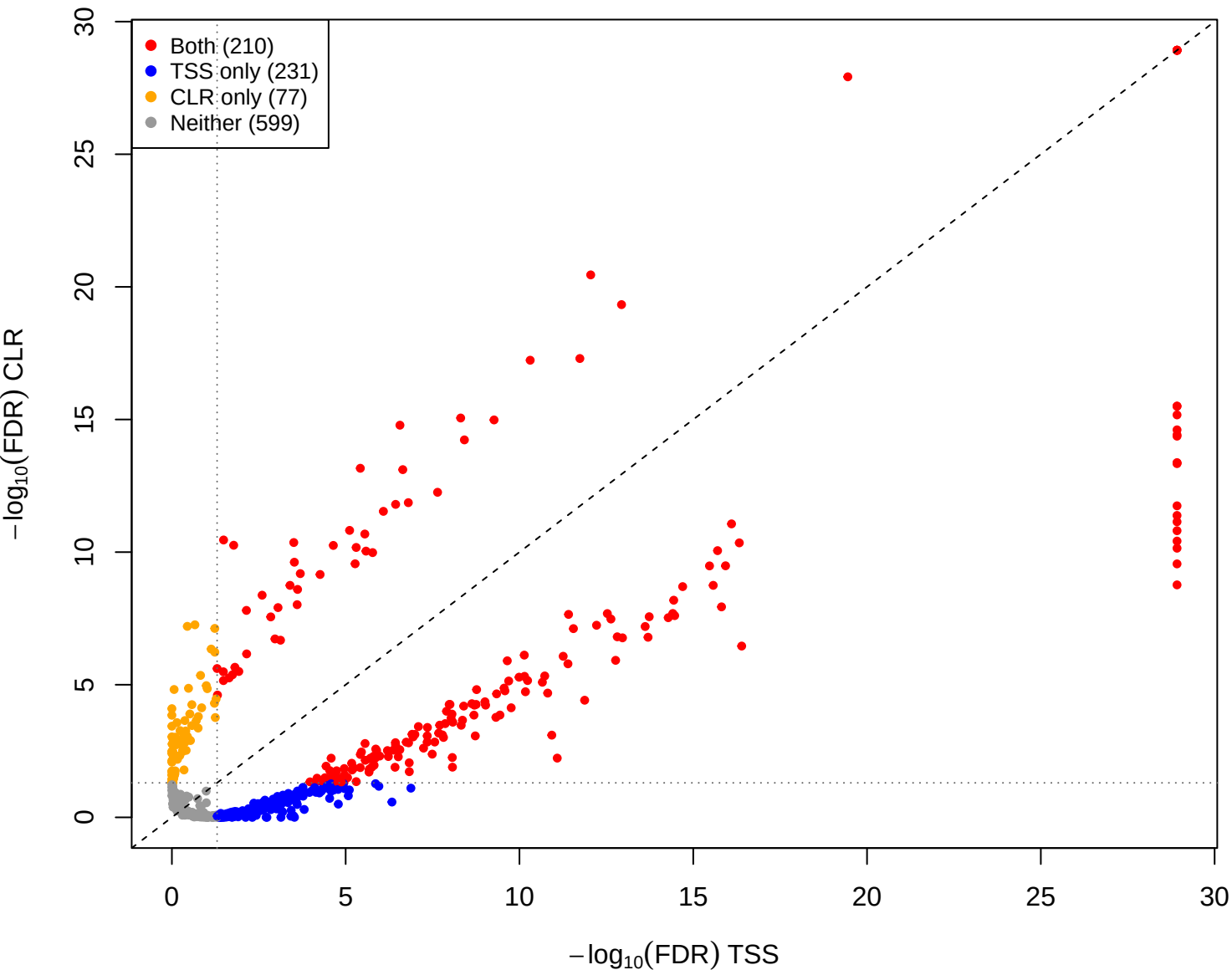
cent vs you – CLR vs TSS(const=-0.5) (gamma = 0.001)
