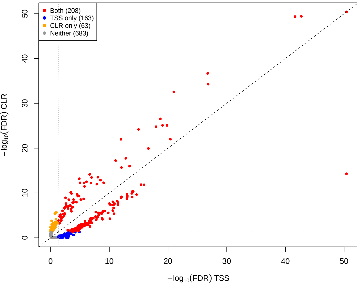
cent vs kin – CLR vs TSS(const=-0.5) (gamma = 0.001)
