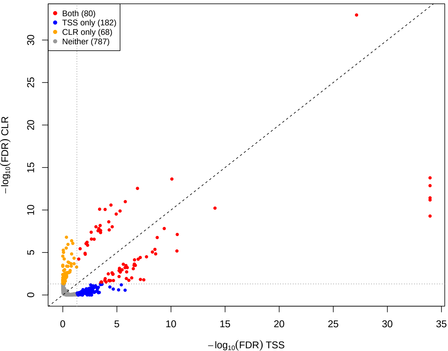
mage vs pup – CLR vs TSS(const=-0.5) (gamma = 0.001)
