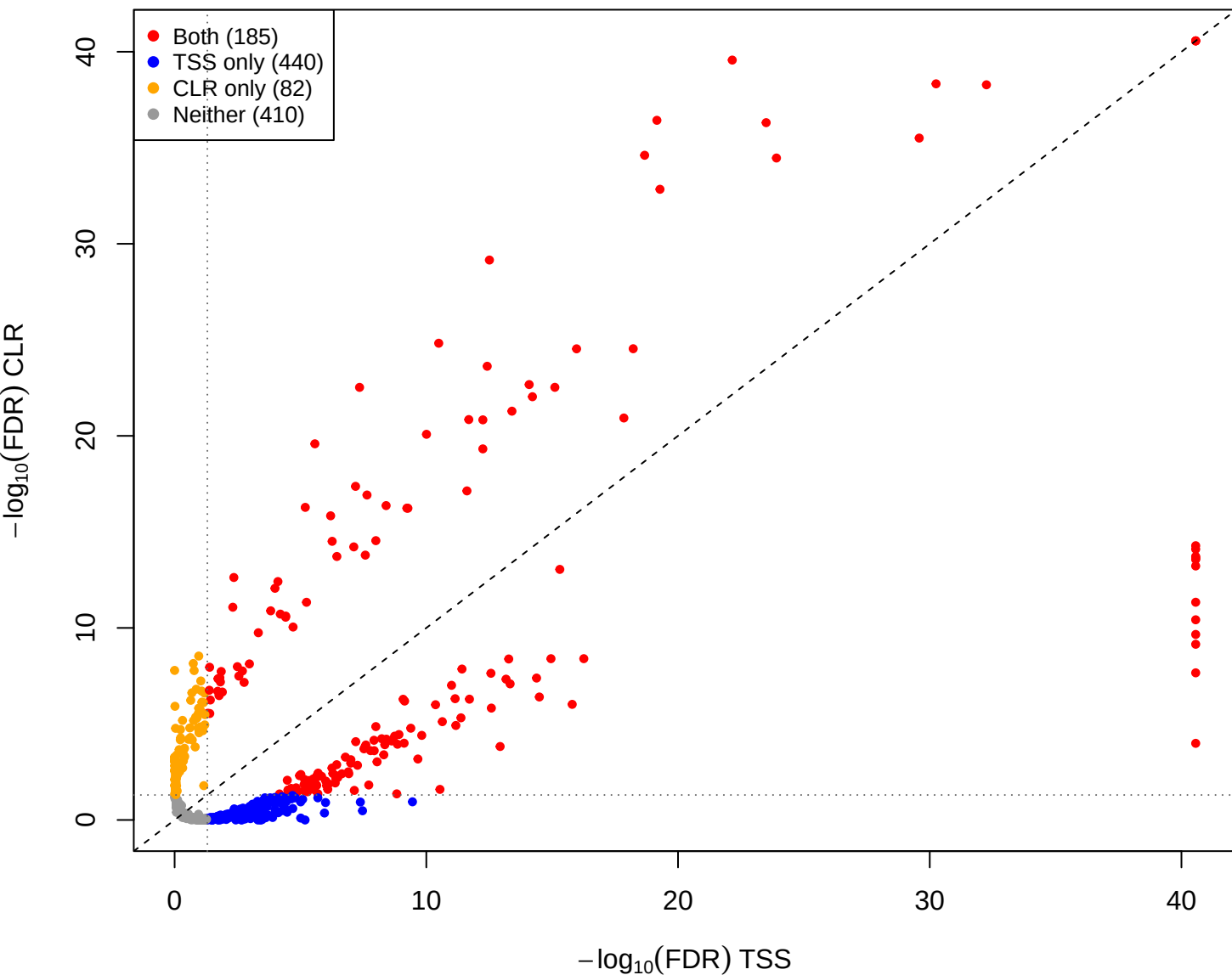
eld vs pup – CLR vs TSS(const=-0.7) (gamma = 0.001)
