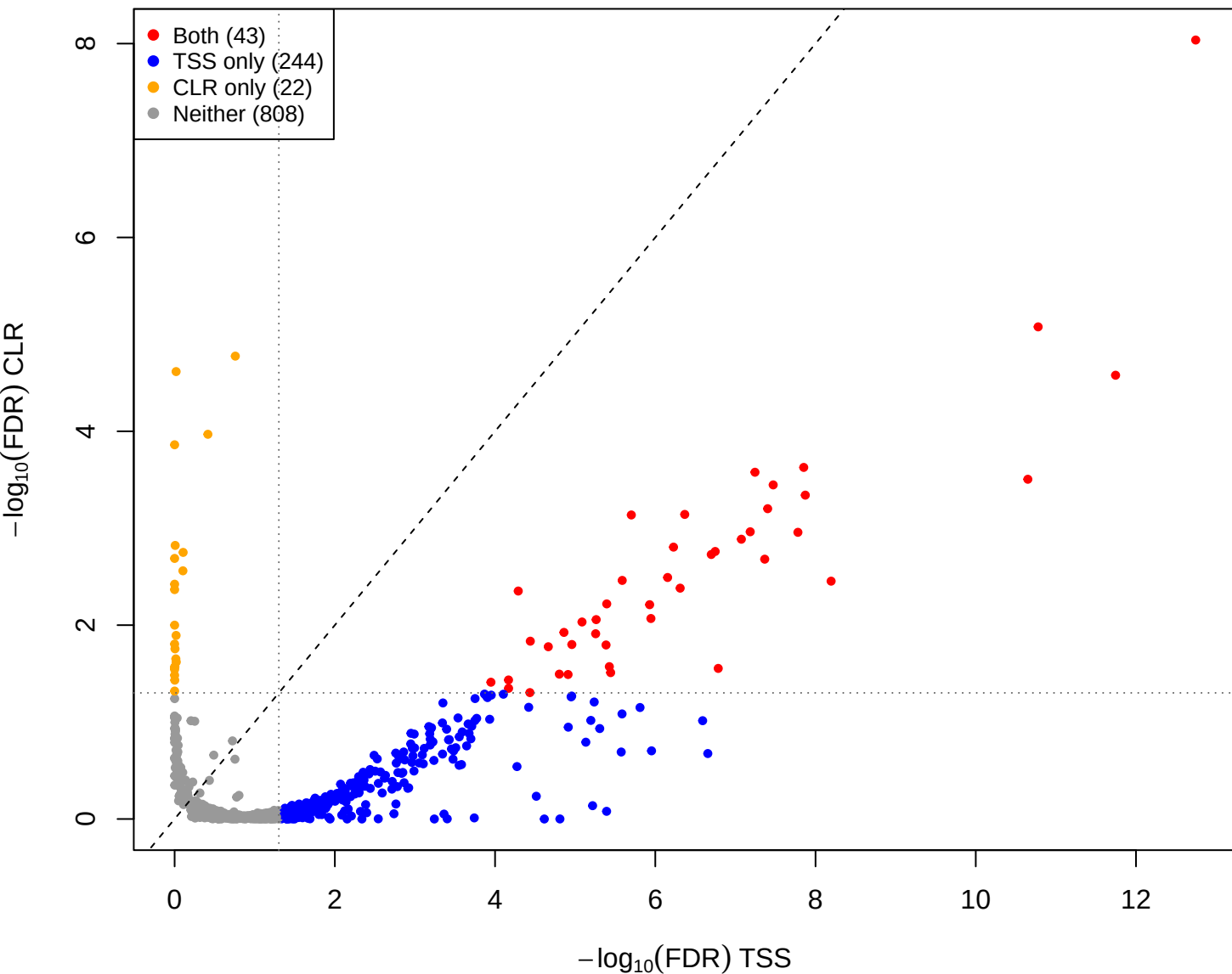
eld vs you – CLR vs TSS(const=-0.7) (gamma = 0.001)
