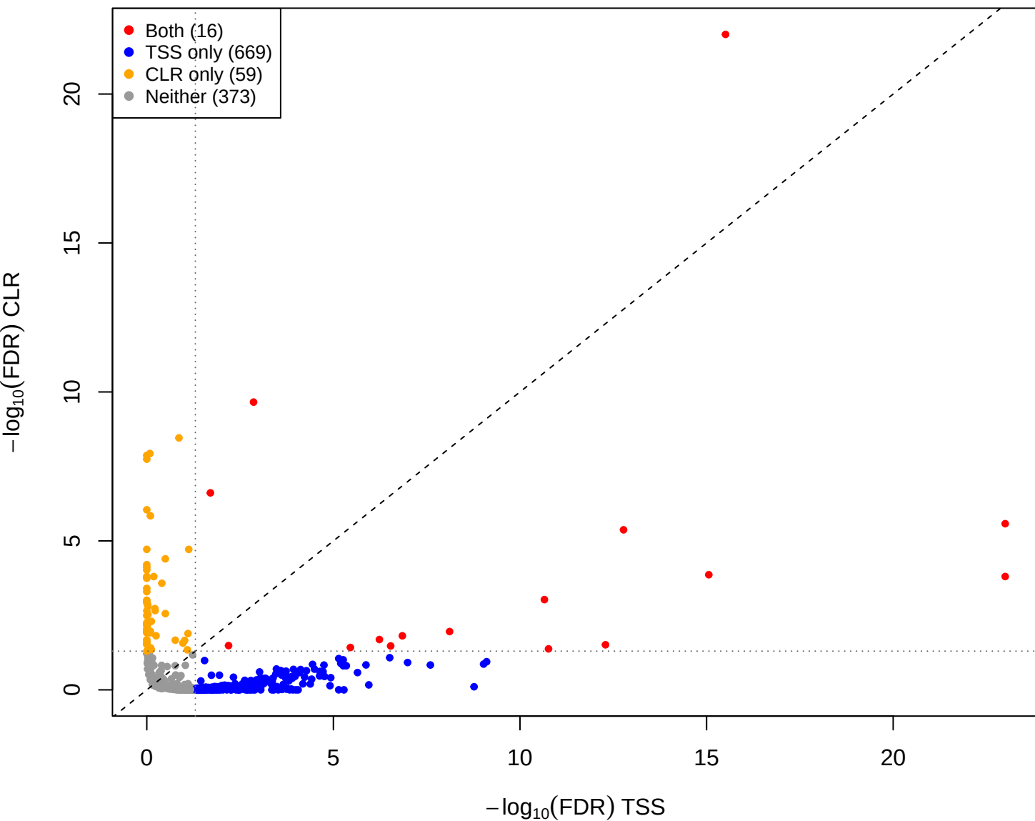
kin vs pup – CLR vs TSS(const=-0.7) (gamma = 0.001)
