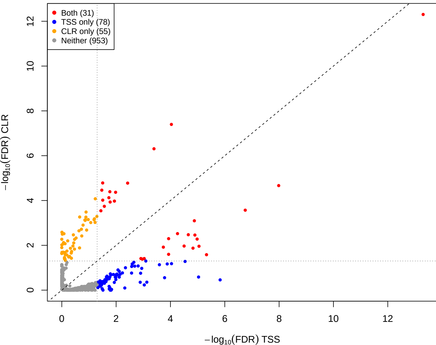
mage vs mid – CLR vs TSS(const=-0.7) (gamma = 0.001)
