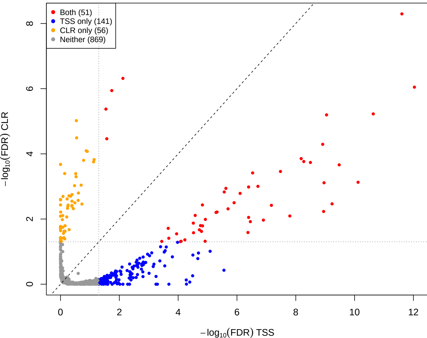
kin vs mage – CLR vs TSS(const=-0.7) (gamma = 0.001)
