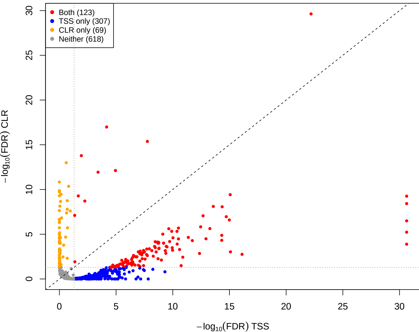
mid vs pup – CLR vs TSS(const=-0.7) (gamma = 0.001)
