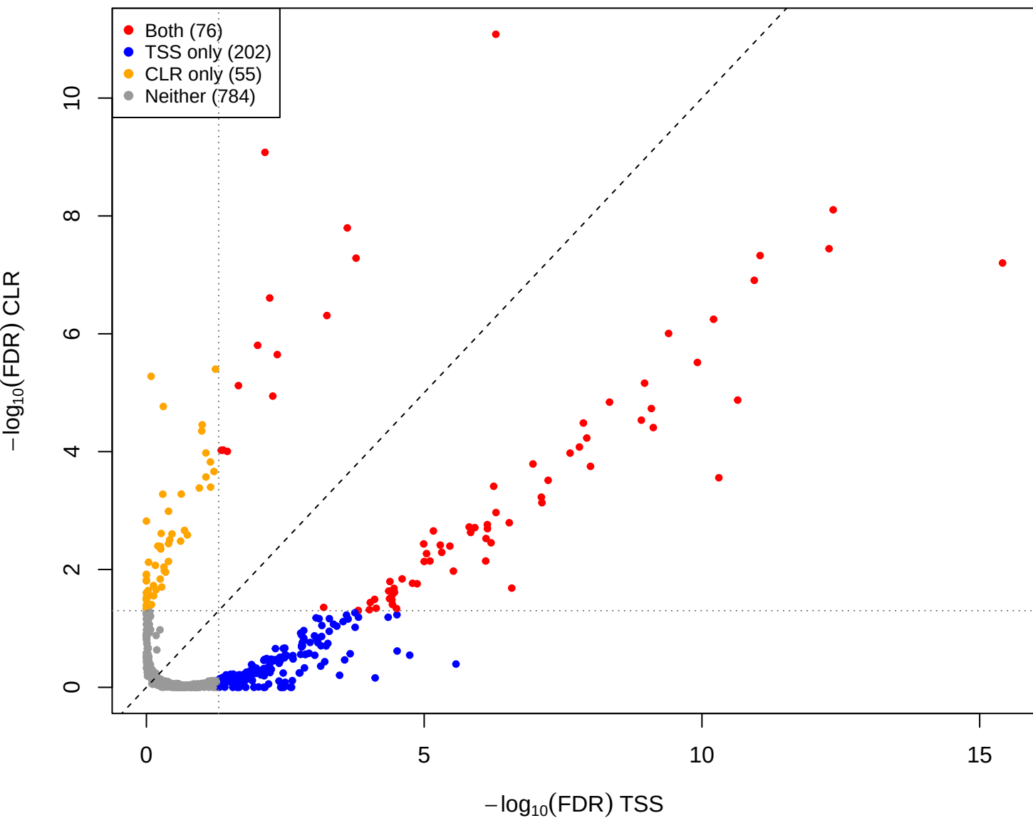
cent vs eld – CLR vs TSS(const=-0.7) (gamma = 0.001)
