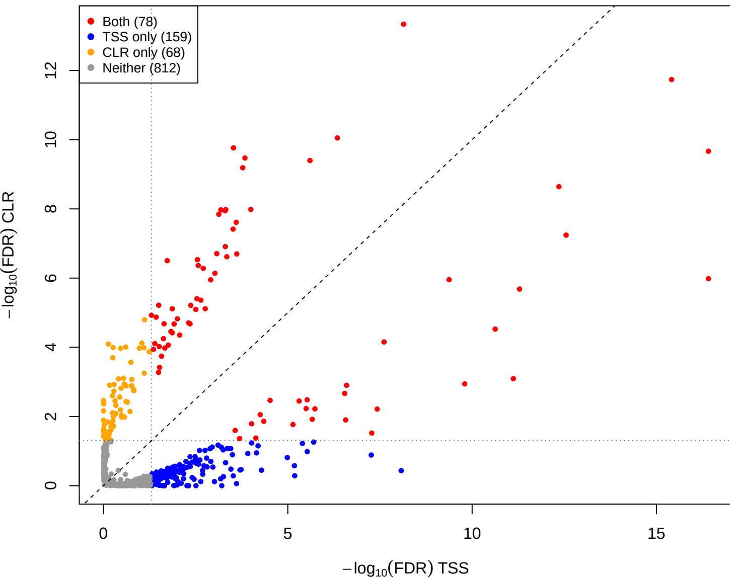
kin vs mid – CLR vs TSS(const=-0.7) (gamma = 0.001)
