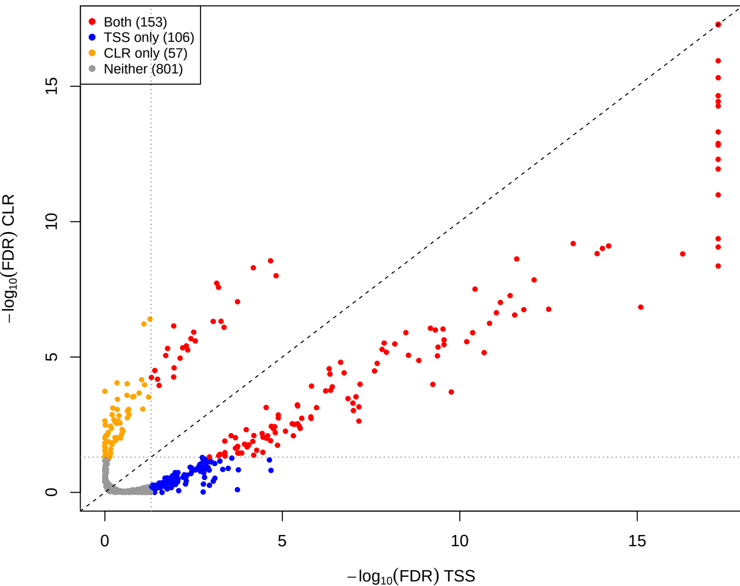
mage vs you – CLR vs TSS(const=-0.7) (gamma = 0.001)
