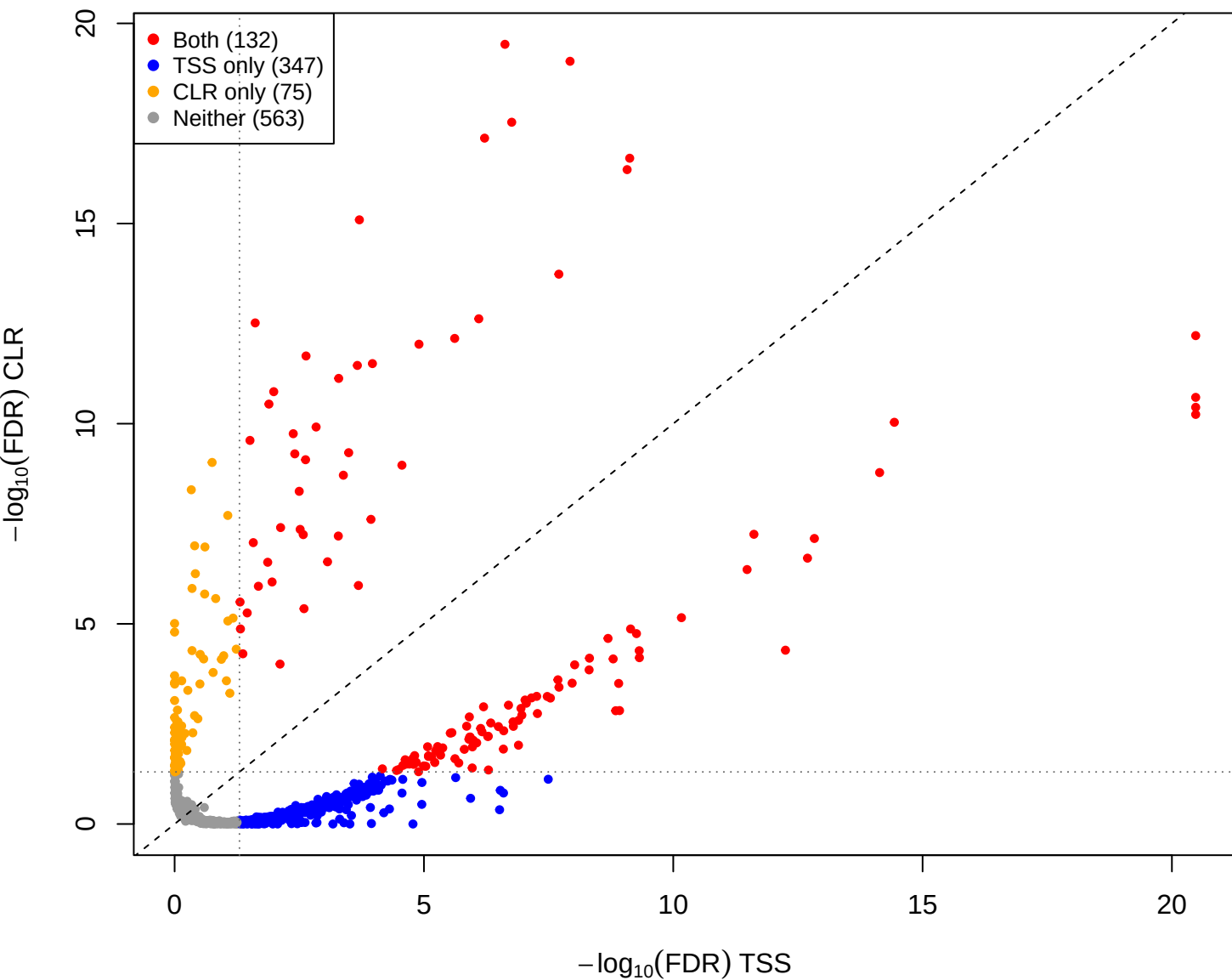
cent vs mage – CLR vs TSS(const=-0.7) (gamma = 0.001)
