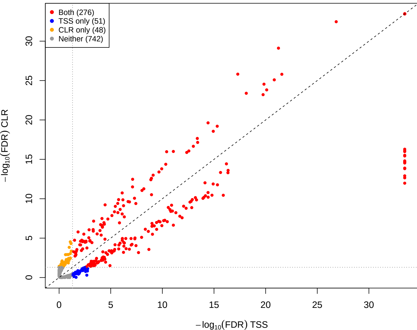
pup vs you – CLR vs TSS(const=-0.7) (gamma = 0.001)
