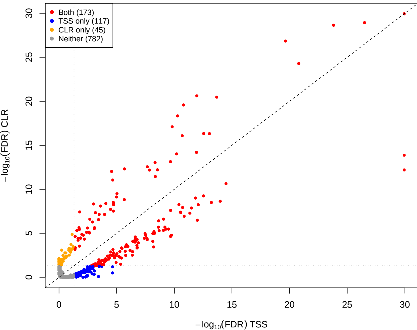
eld vs kin - CLR vs TSS(const=-0.7) (gamma = 0.001)
