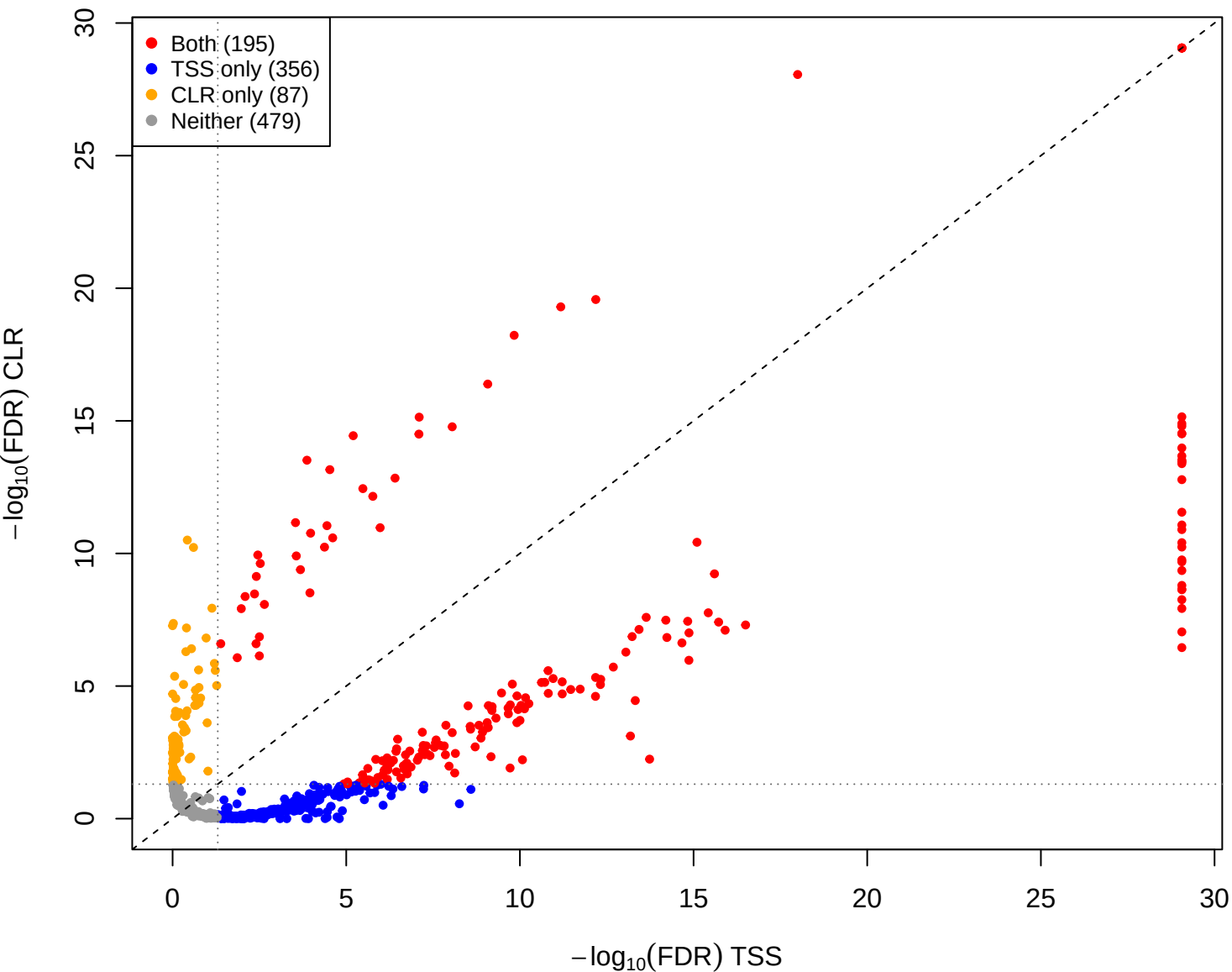
cent vs you – CLR vs TSS(const=-0.7) (gamma = 0.001)
