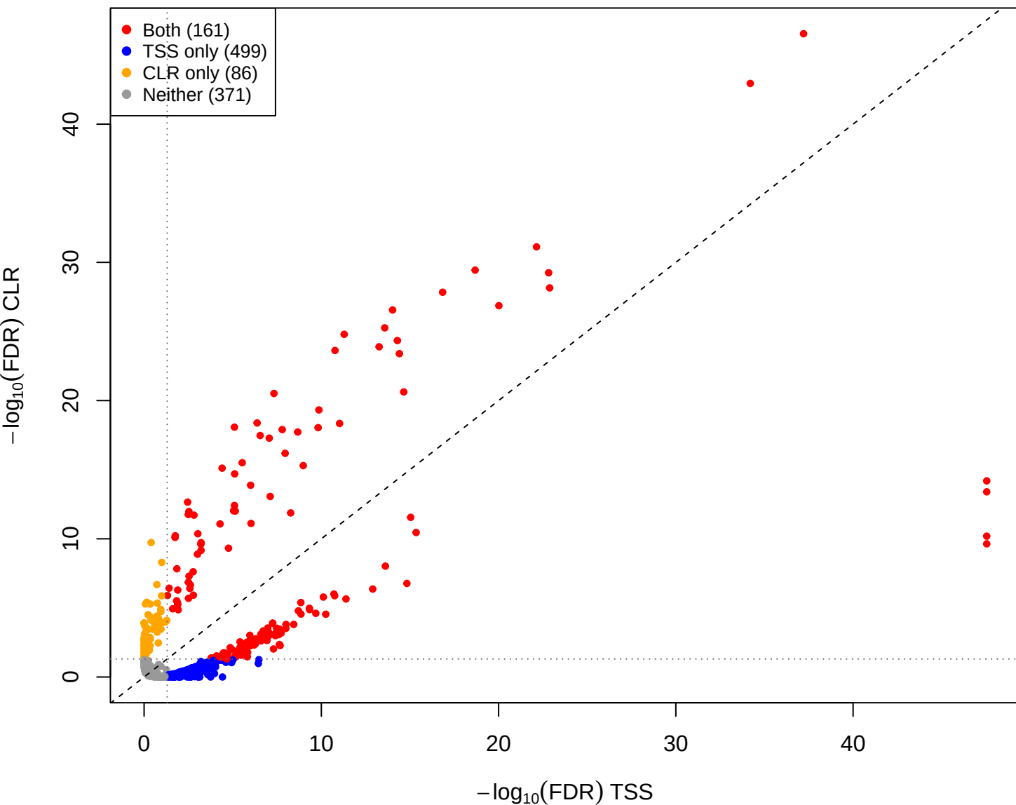
cent vs mid – CLR vs TSS(const=-0.7) (gamma = 0.001)
