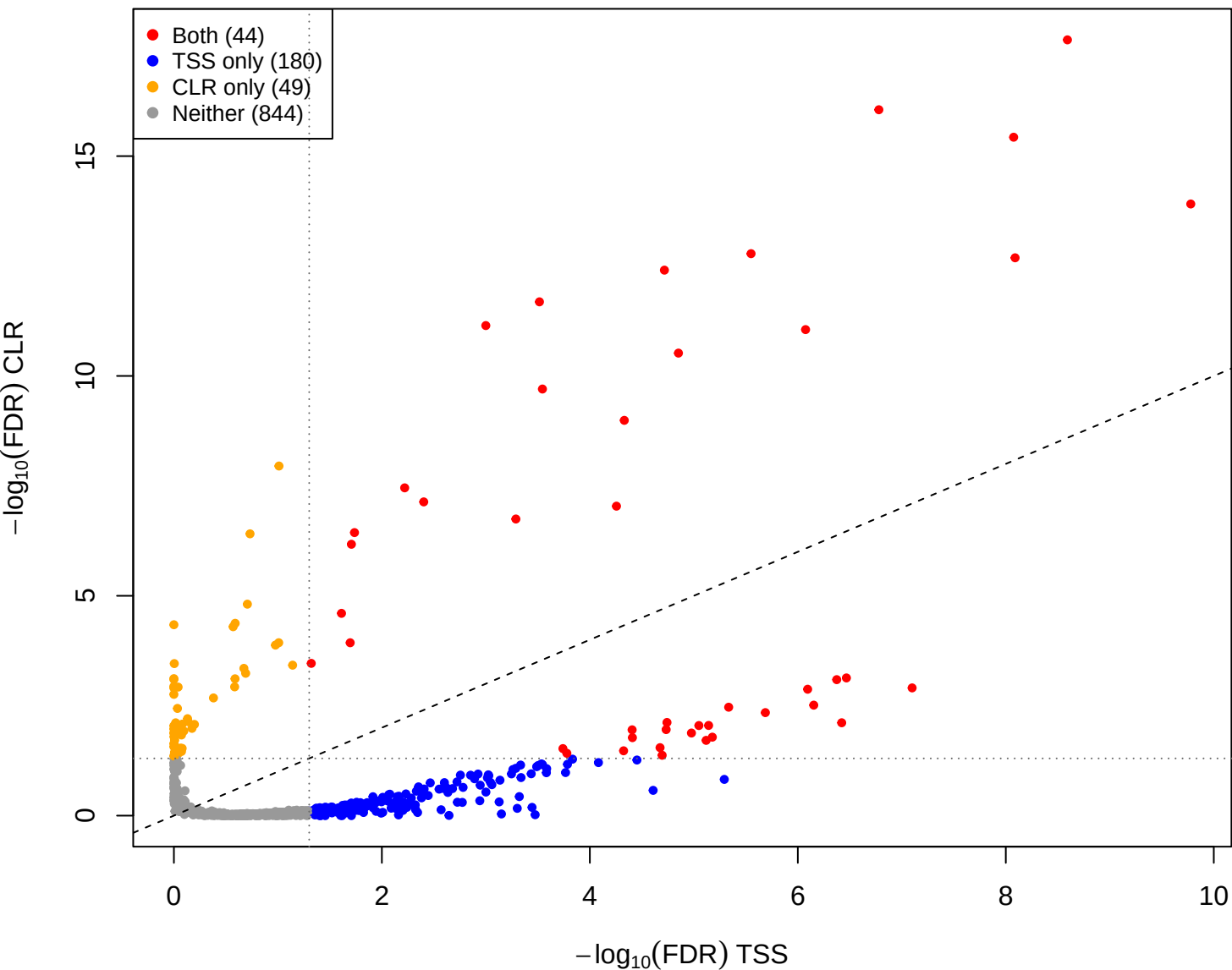
eld vs mage – CLR vs TSS(const=-0.7) (gamma = 0.001)
