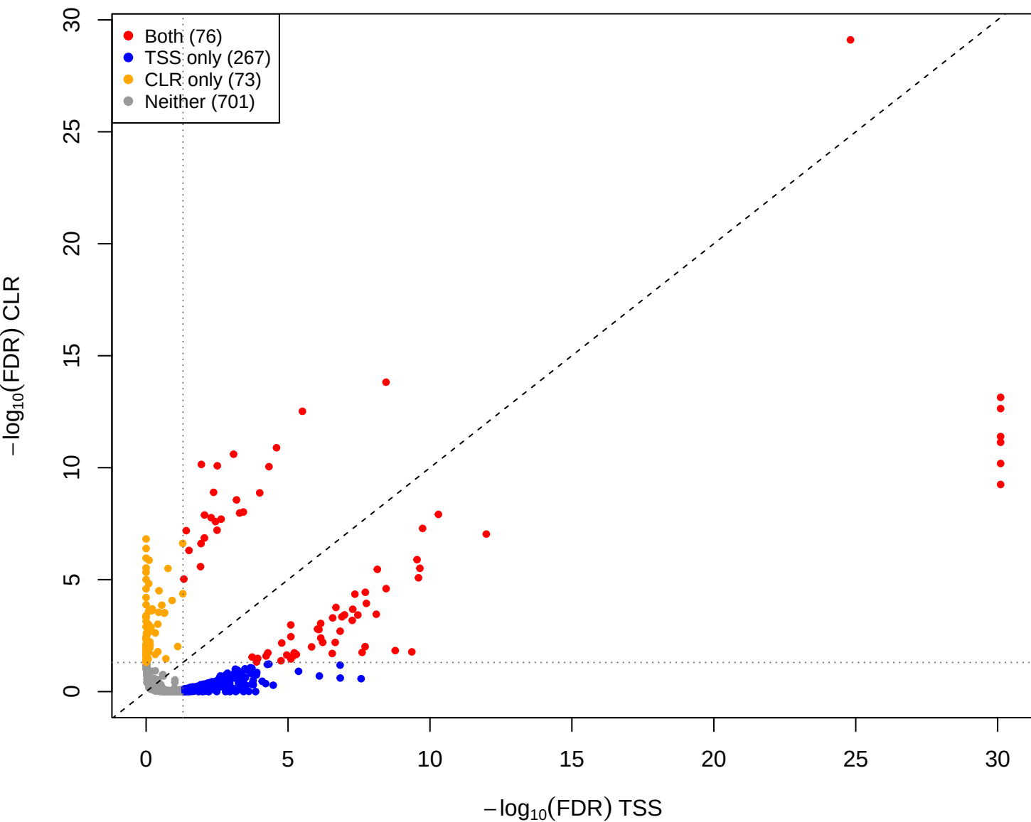
mage vs pup – CLR vs TSS(const=-0.7) (gamma = 0.001)
