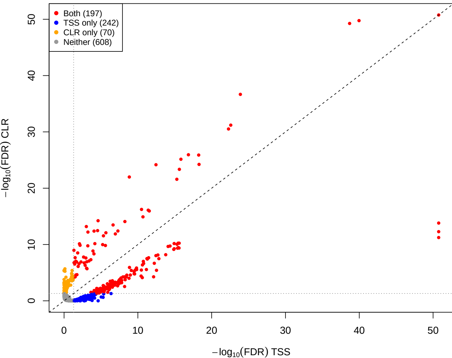
cent vs kin – CLR vs TSS(const=-0.7) (gamma = 0.001)
