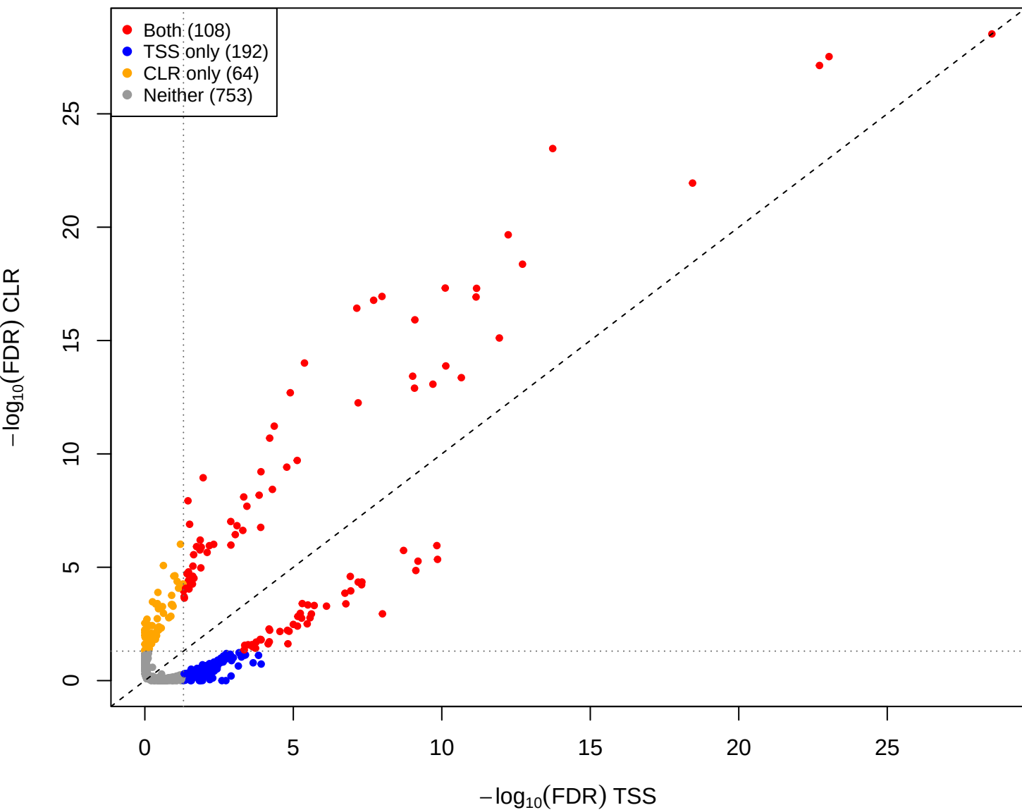
eld vs mid – CLR vs TSS(const=-0.7) (gamma = 0.001)
