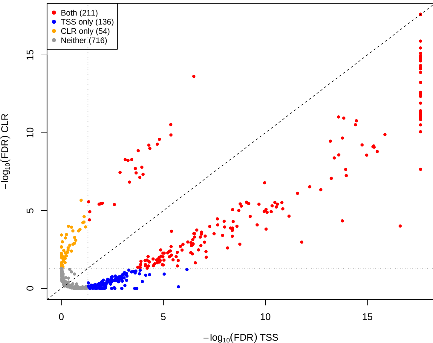
mid vs you – CLR vs TSS(const=-0.7) (gamma = 0.001)
