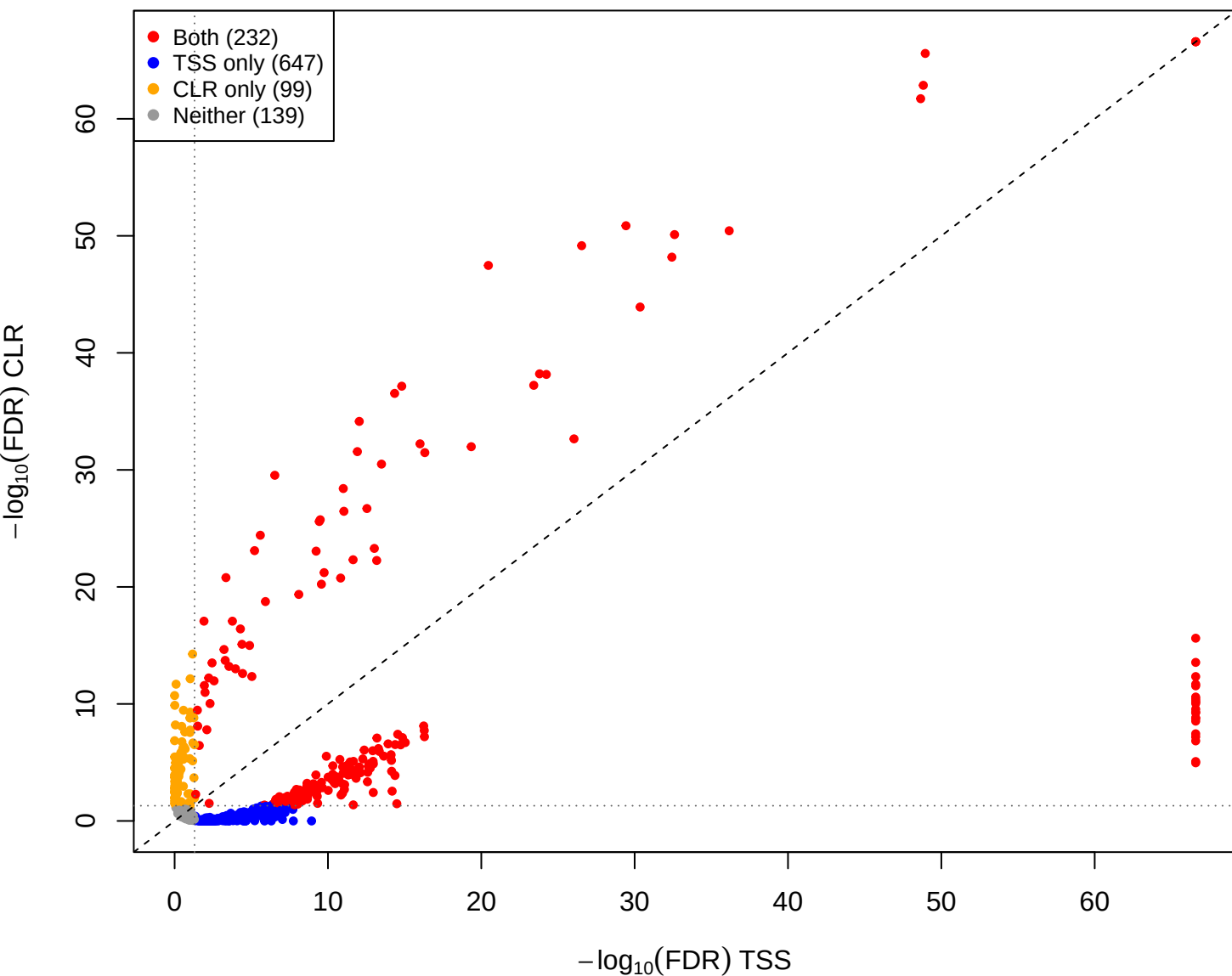
cent vs pup – CLR vs TSS(const=-0.7) (gamma = 0.001)
