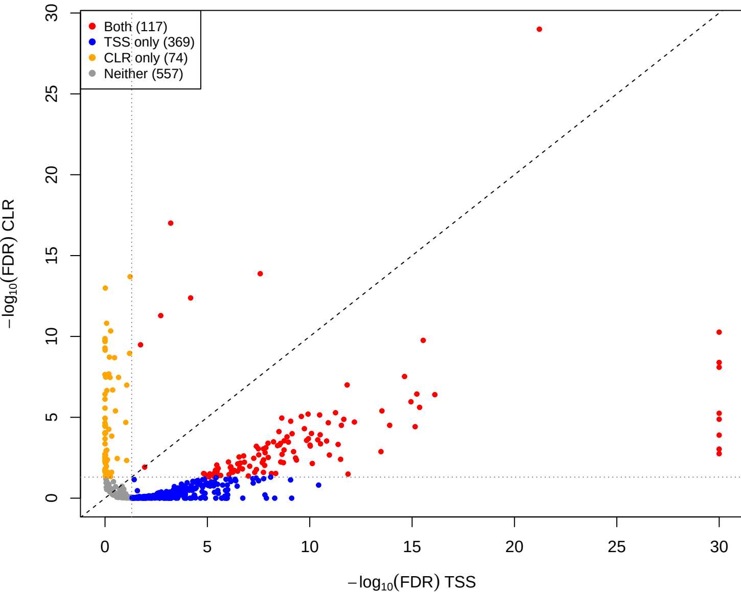
mid vs pup – CLR vs TSS(const=-0.8) (gamma = 0.001)
