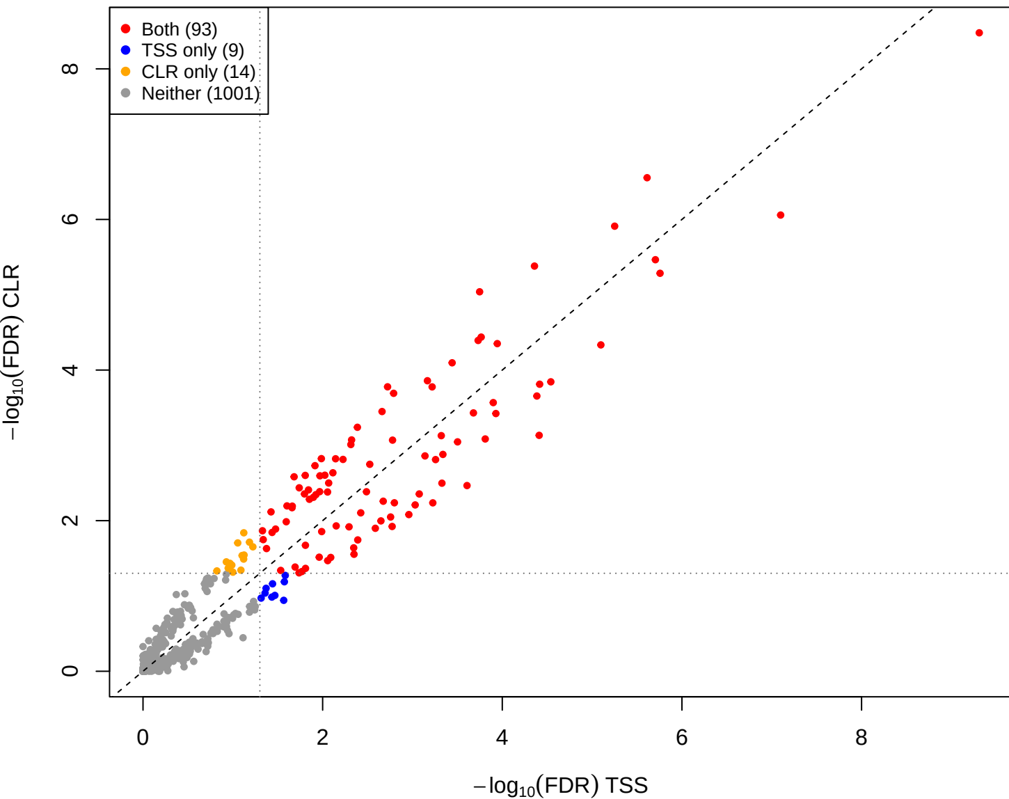
kin vs mage – CLR vs TSS(const=0) (gamma = 0.001)
