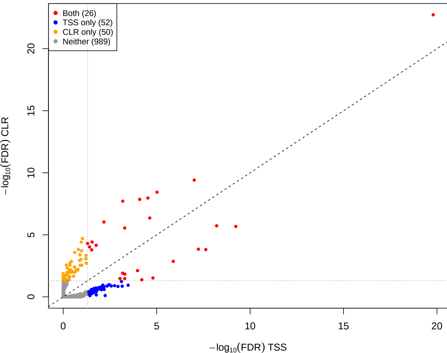
kin vs pup – CLR vs TSS(const=0) (gamma = 0.001)
