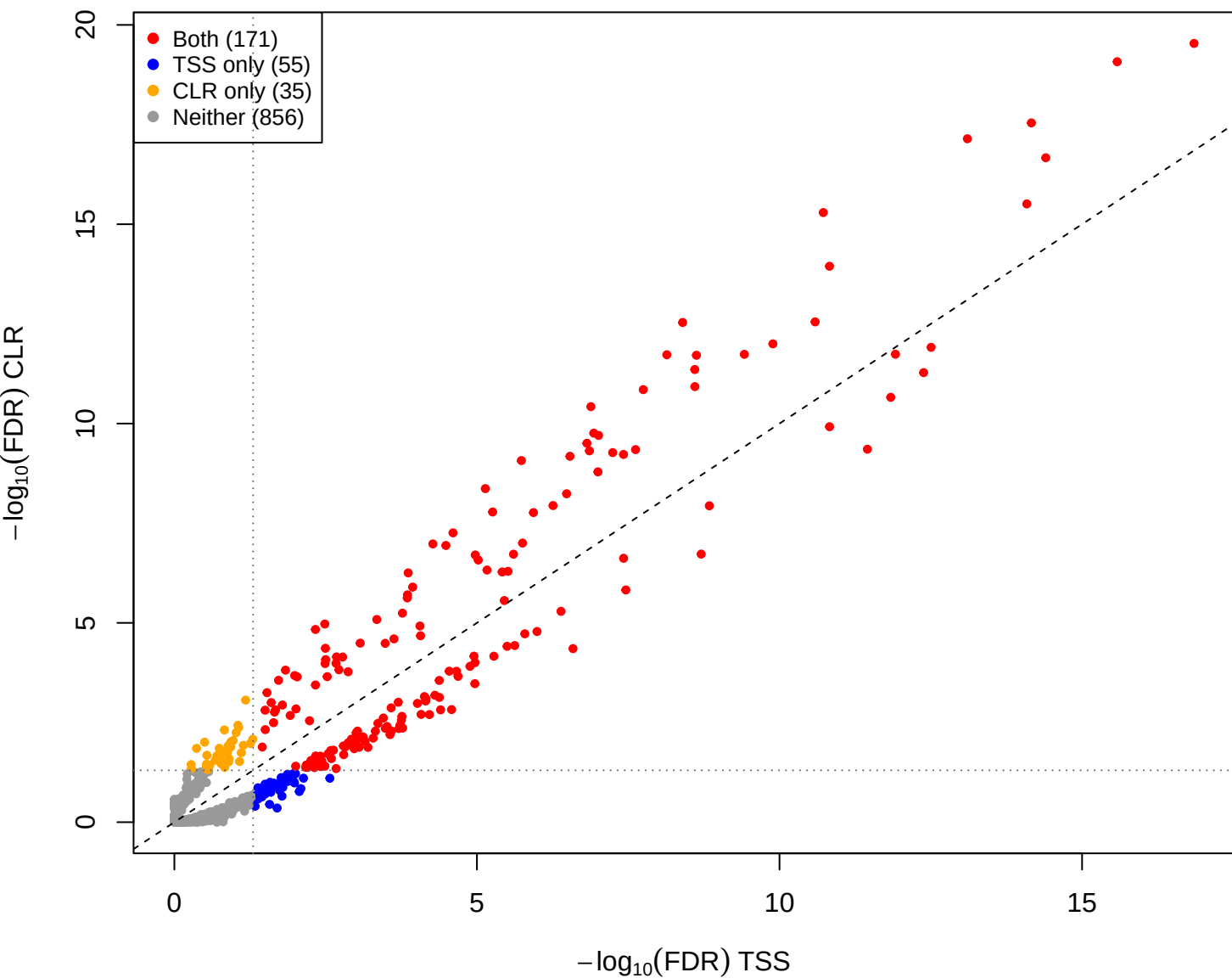
cent vs mage – CLR vs TSS(const=0) (gamma = 0.001)
