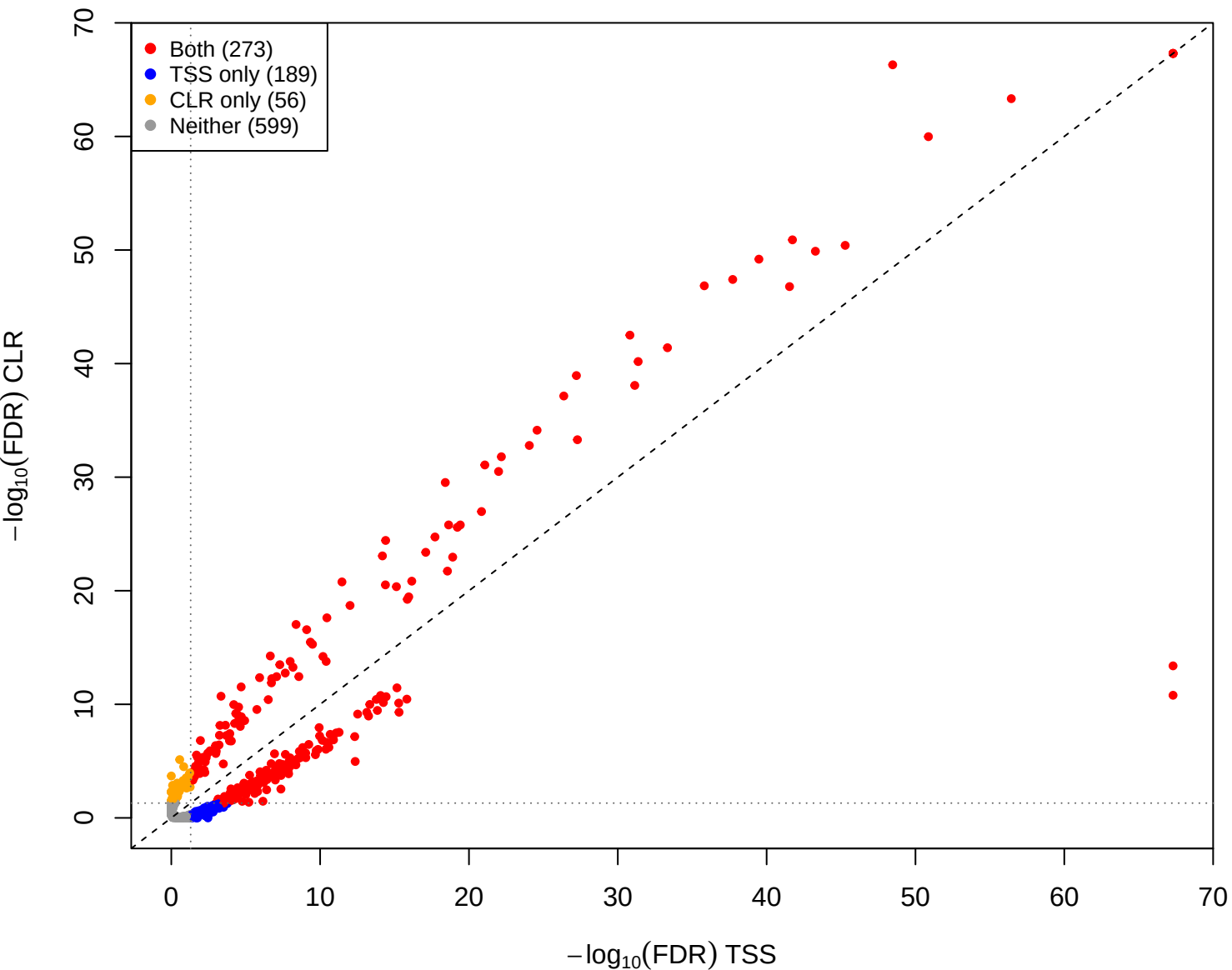
cent vs pup – CLR vs TSS(const=0) (gamma = 0.001)
