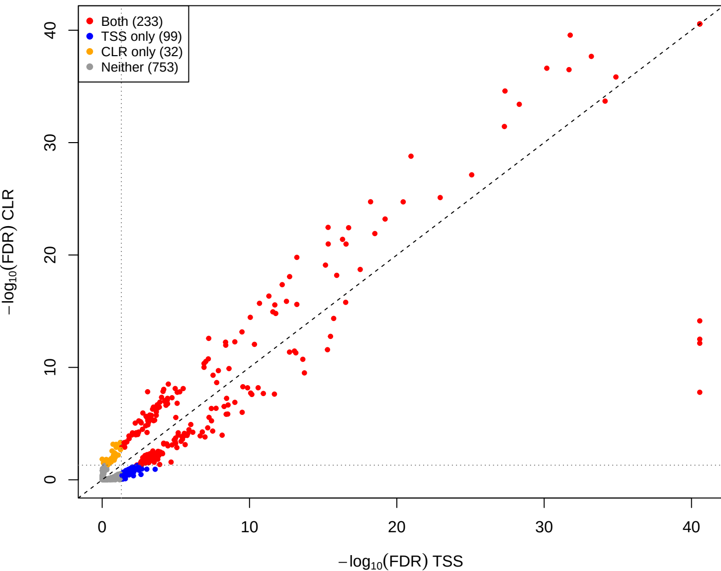
eld vs pup – CLR vs TSS(const=0) (gamma = 0.001)
