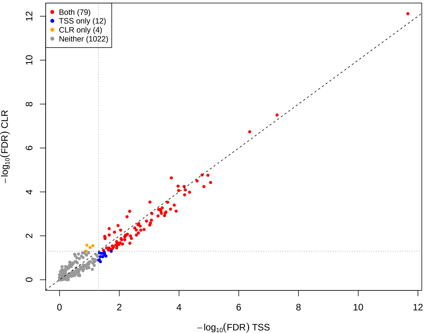
mage vs mid – CLR vs TSS(const=0) (gamma = 0.001)
