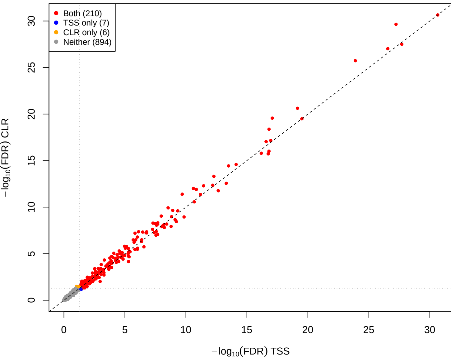
eld vs kin – CLR vs TSS(const=0) (gamma = 0.001)
