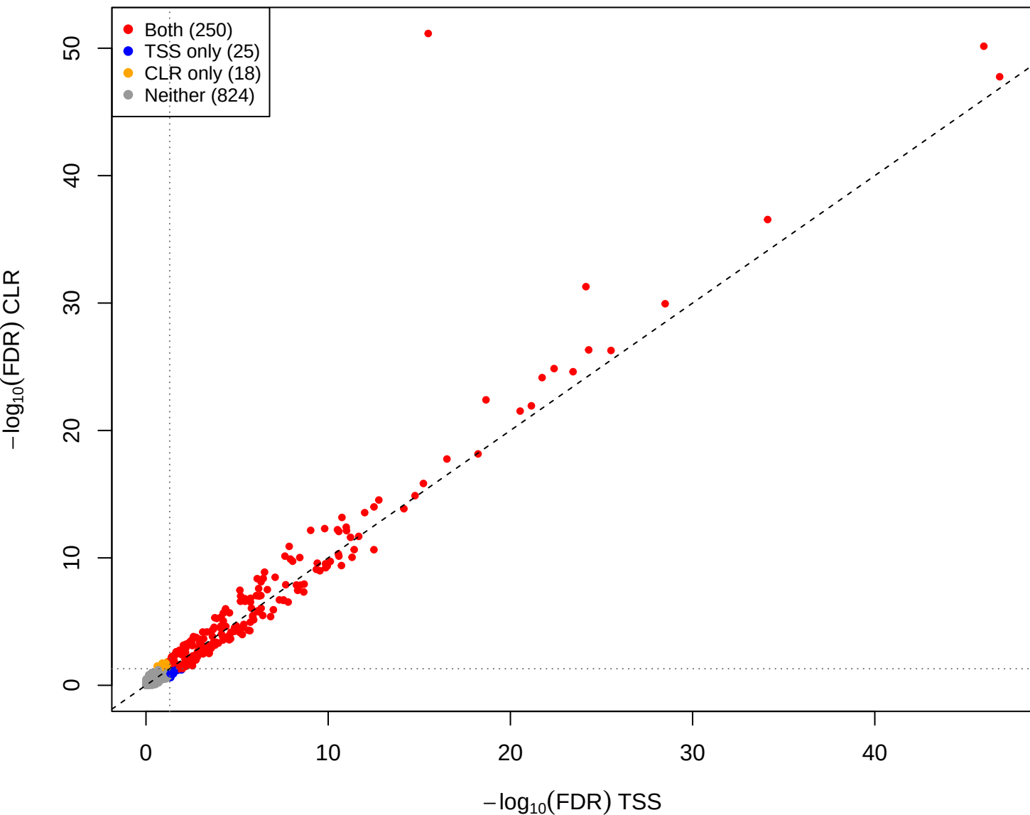
cent vs kin – CLR vs TSS(const=0) (gamma = 0.001)
