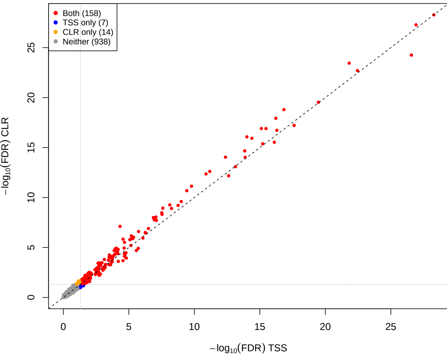
eld vs mid – CLR vs TSS(const=0) (gamma = 0.001)
