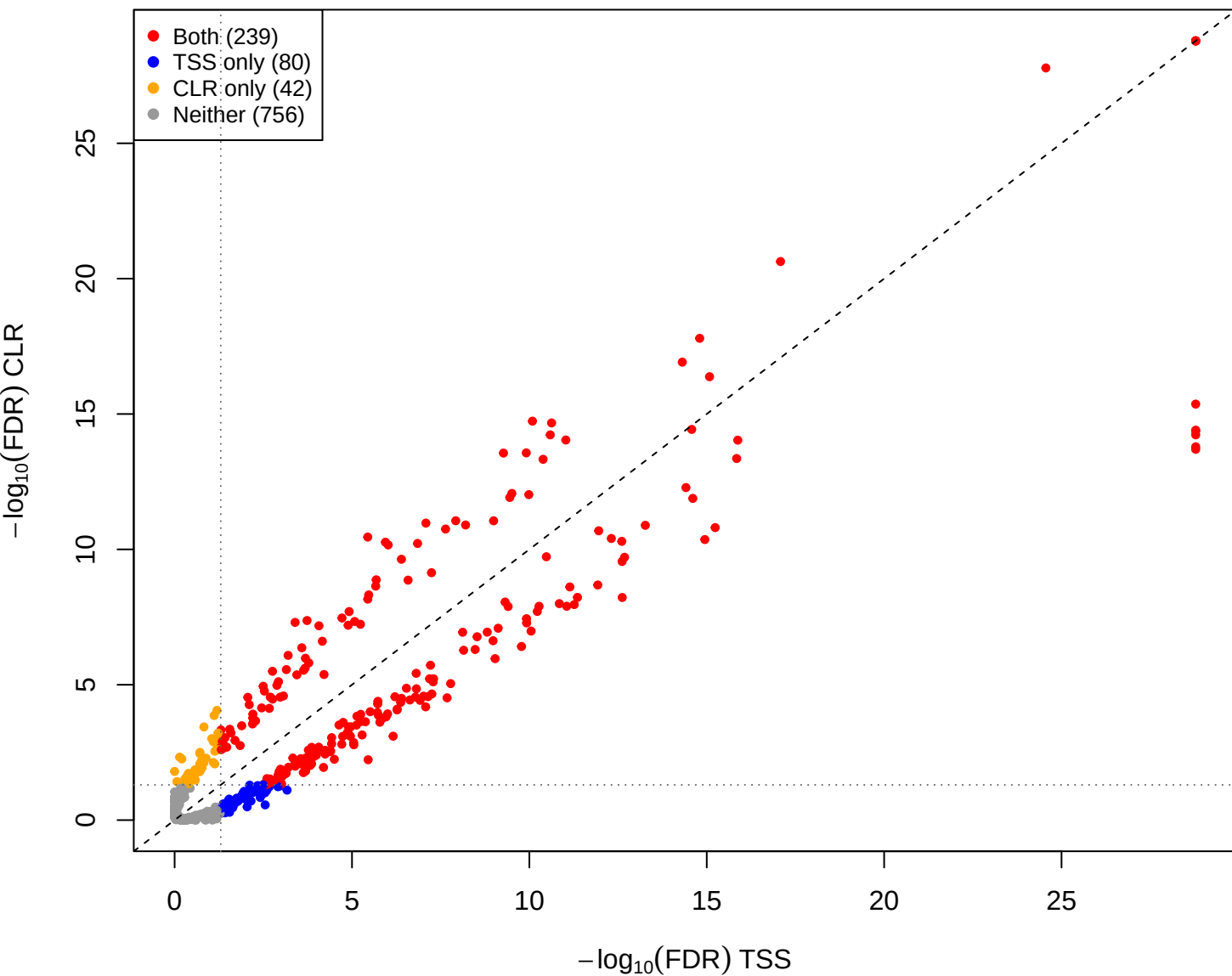
cent vs you – CLR vs TSS(const=0) (gamma = 0.001)
