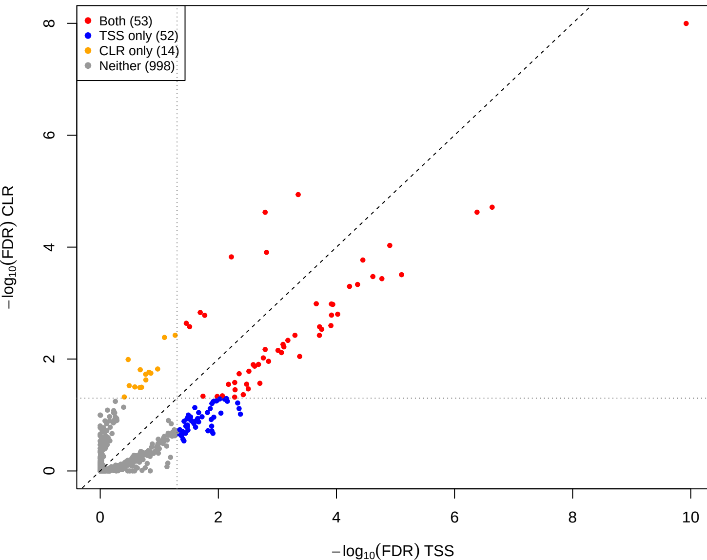
eld vs you - CLR vs TSS(const=0) (gamma = 0.001)
