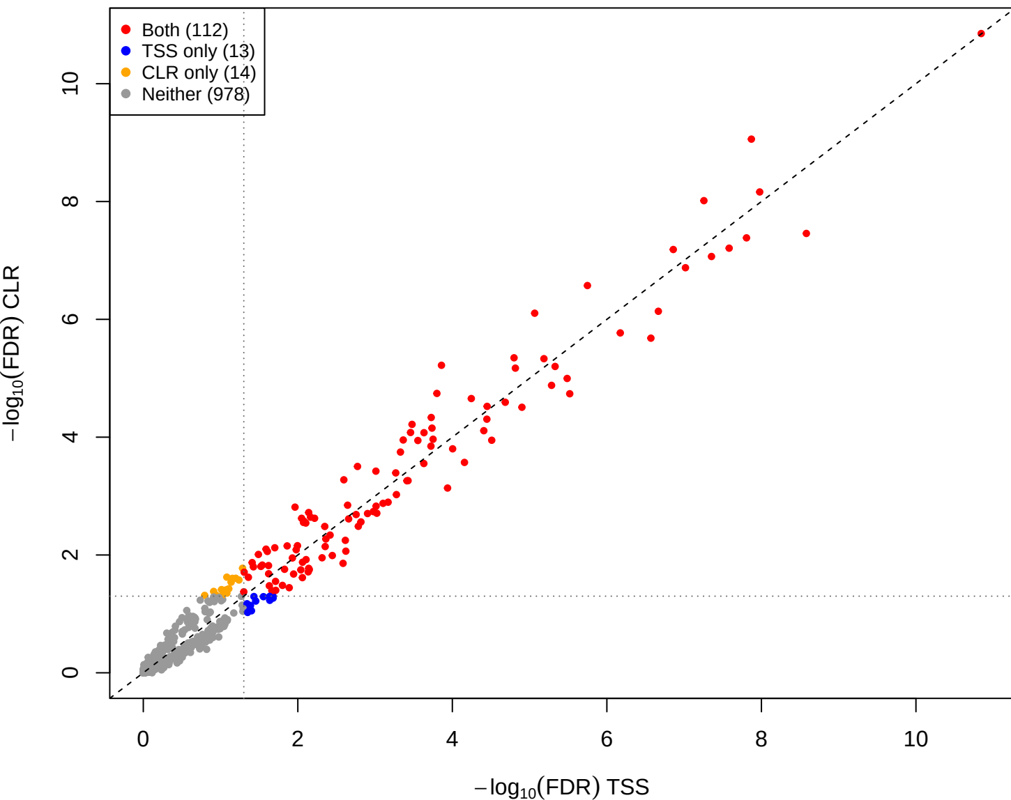
cent vs eld – CLR vs TSS(const=0) (gamma = 0.001)
