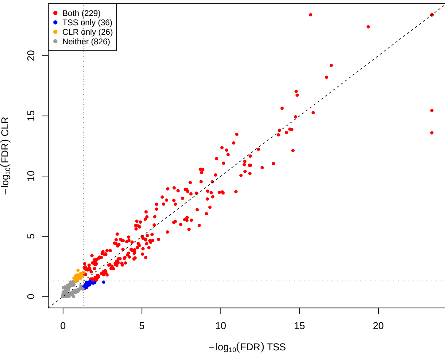
kin vs you – CLR vs TSS(const=0) (gamma = 0.001)
