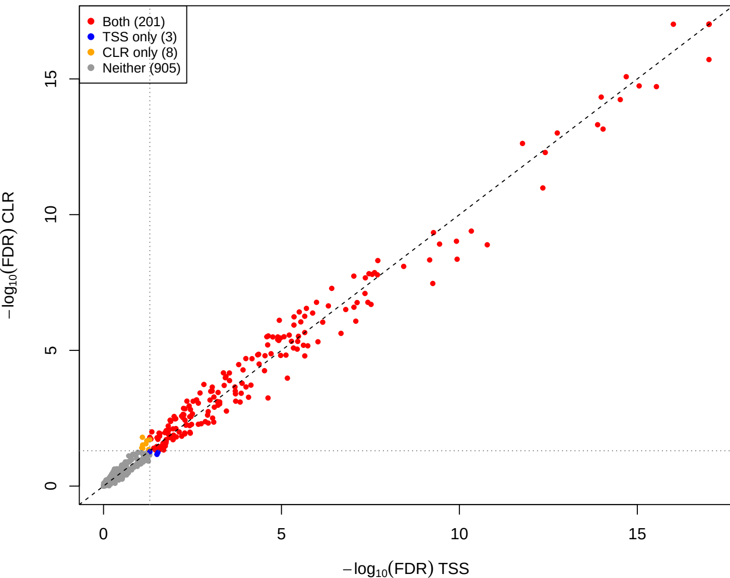
mage vs you – CLR vs TSS(const=0) (gamma = 0.001)
