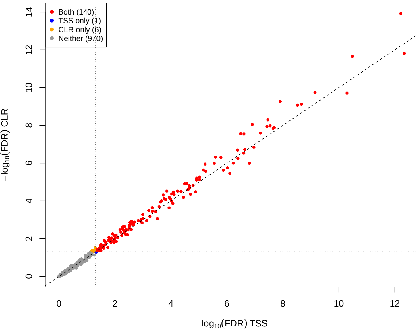
kin vs mid – CLR vs TSS(const=0) (gamma = 0.001)
