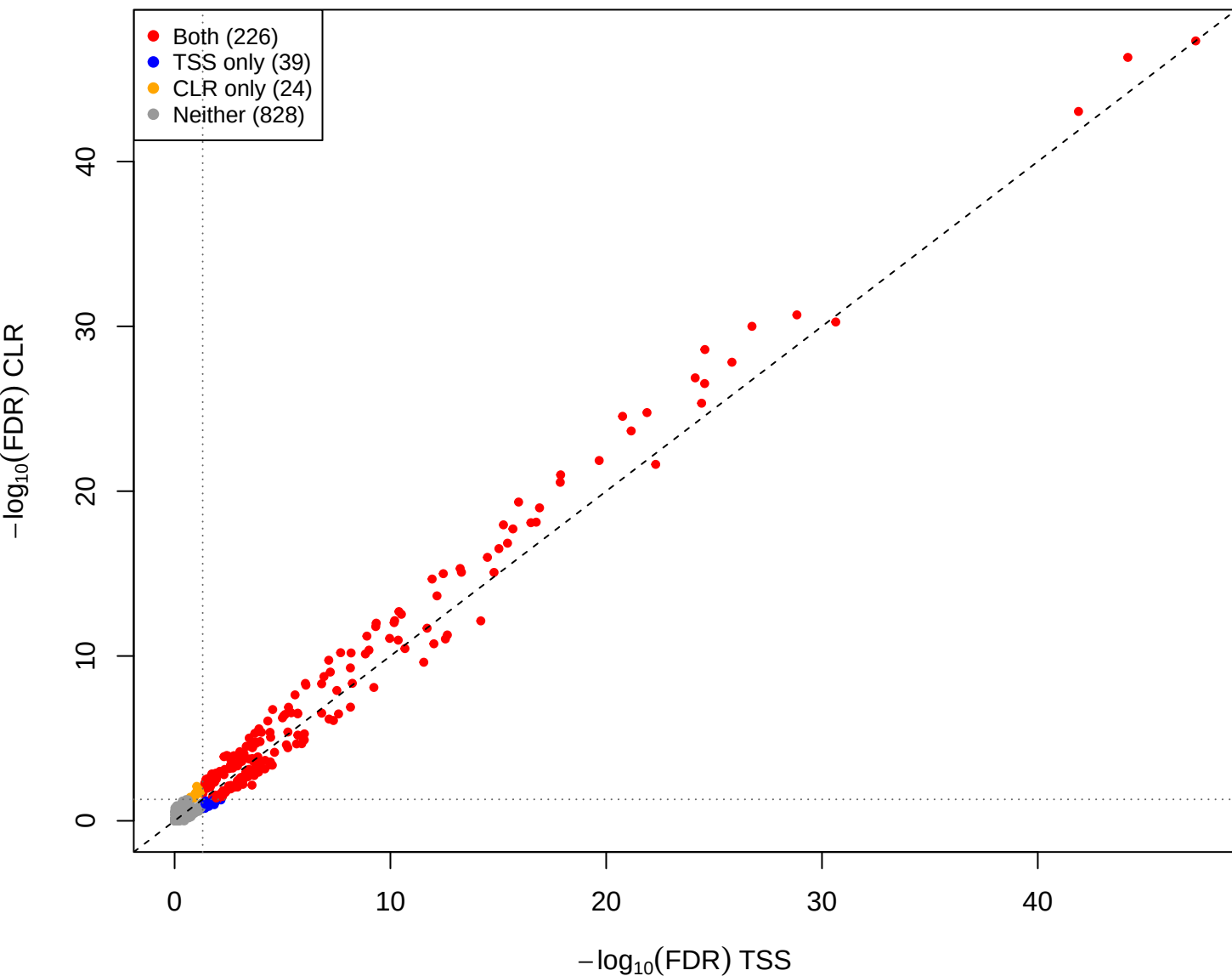
cent vs mid – CLR vs TSS(const=0) (gamma = 0.001)
