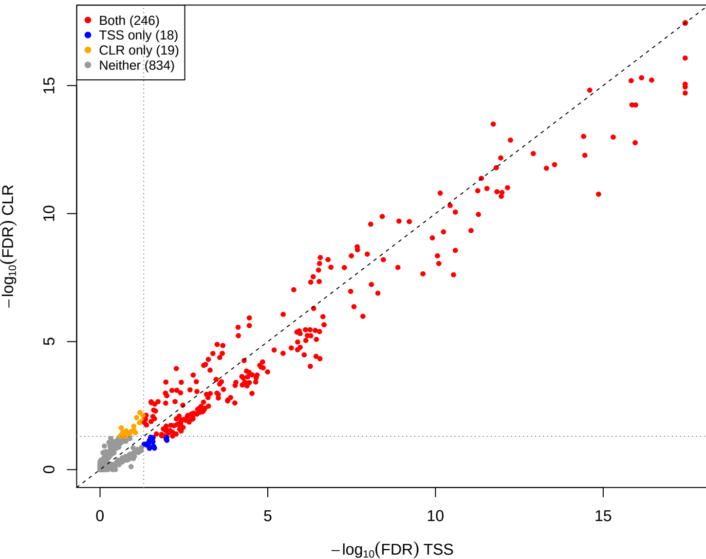
mid vs you – CLR vs TSS(const=0) (gamma = 0.001)
