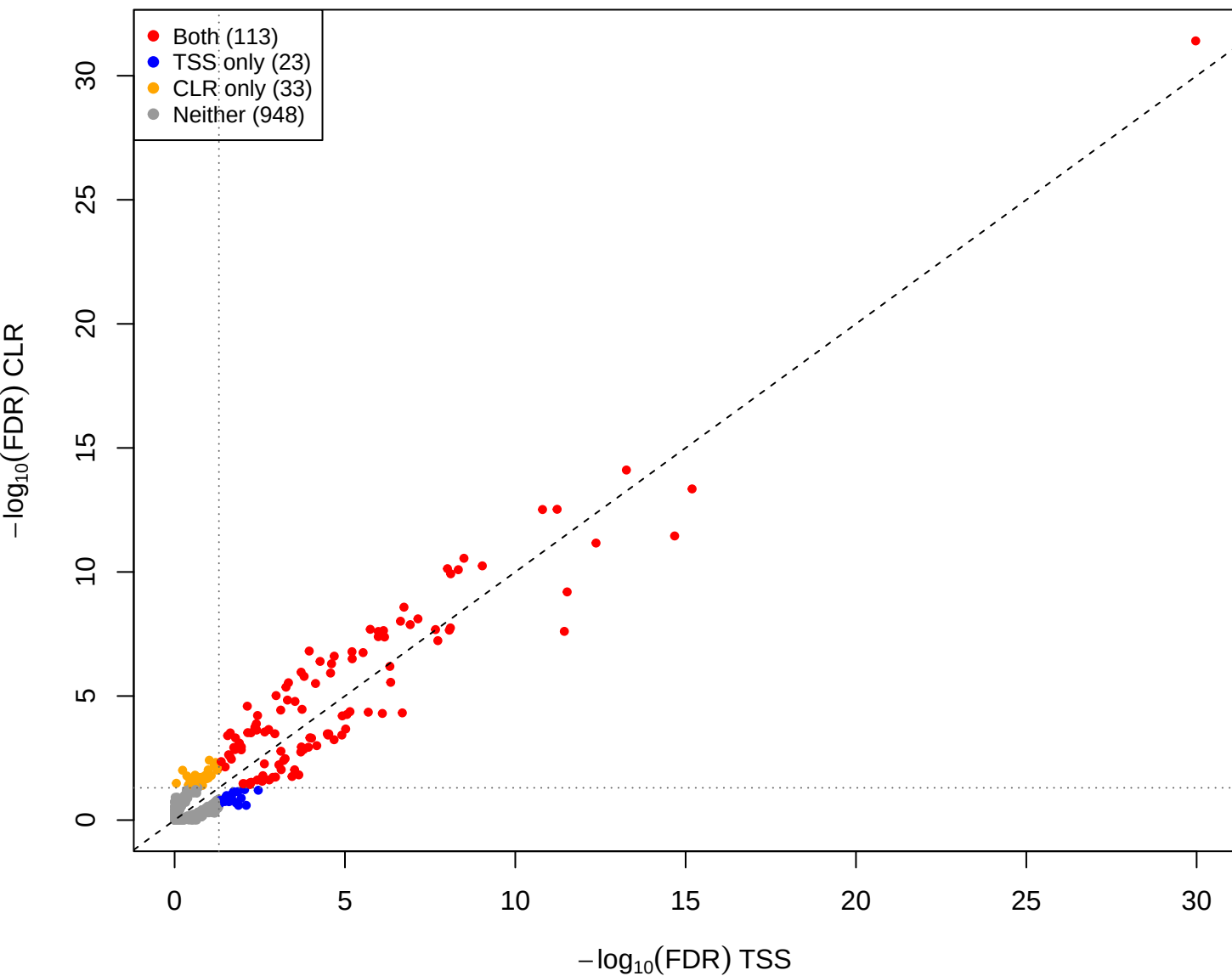
mage vs pup – CLR vs TSS(const=0) (gamma = 0.001)
