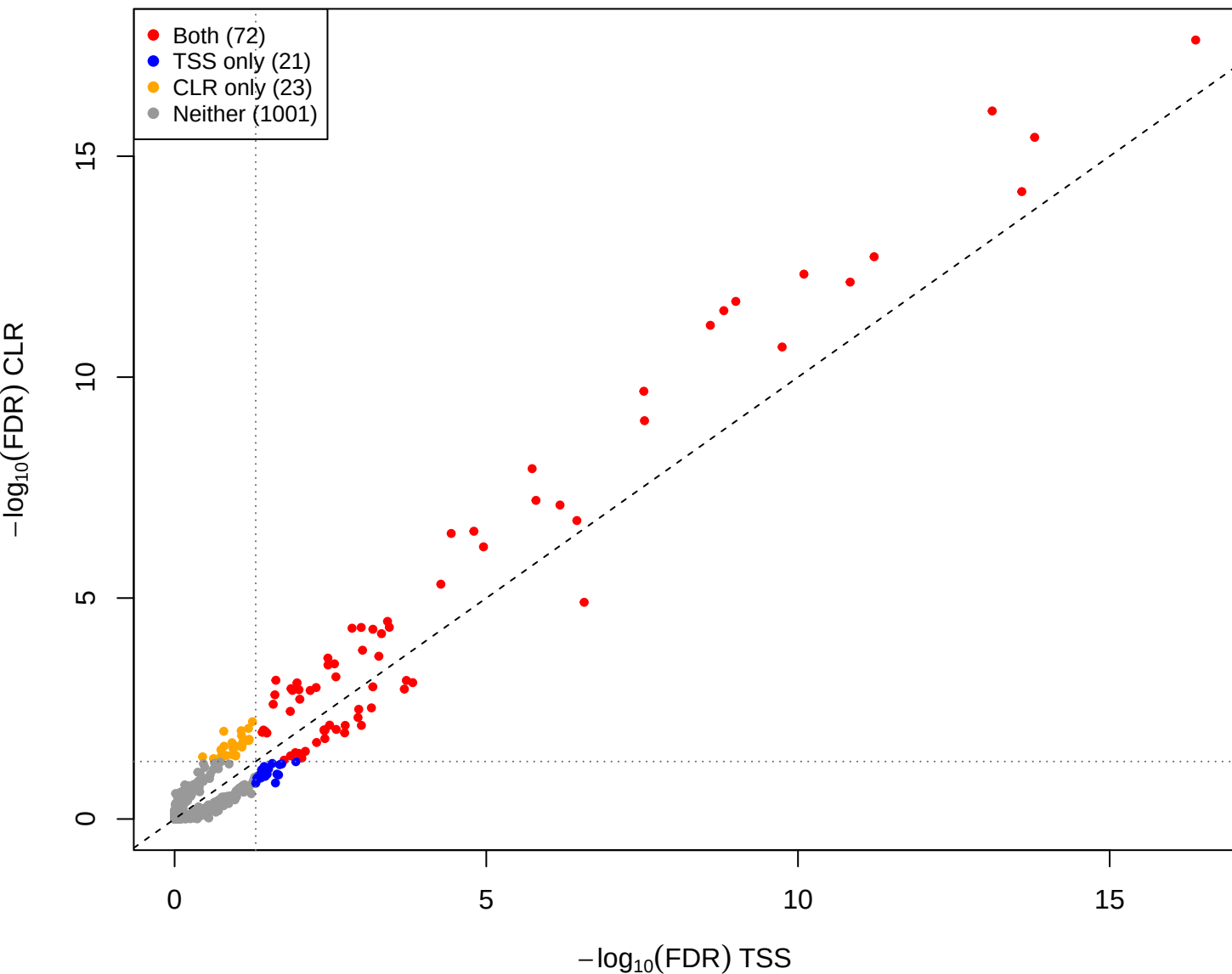
eld vs mage - CLR vs TSS(const=0) (gamma = 0.001)
