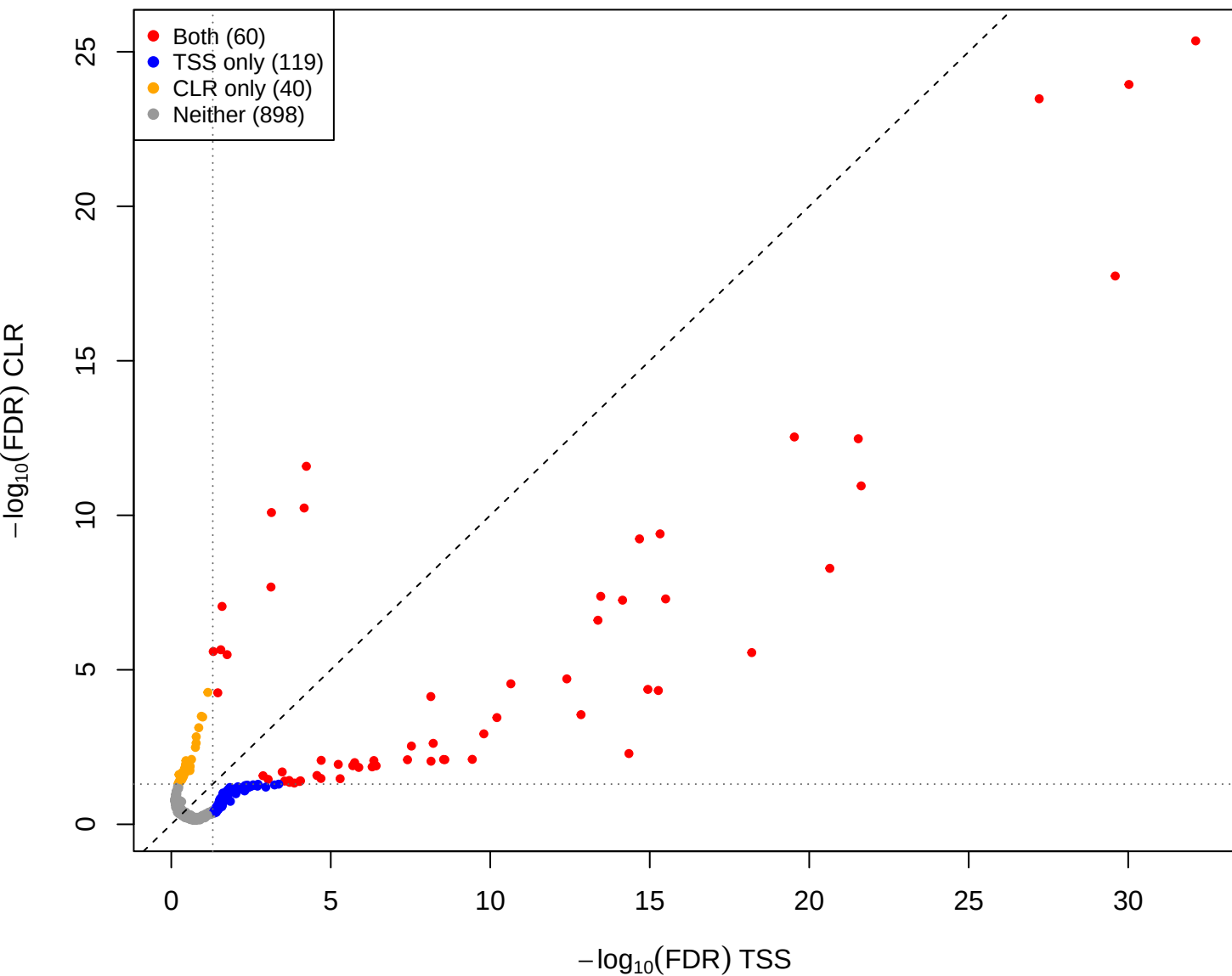
eld vs pup – CLR vs TSS(const=2) (gamma = 1)
