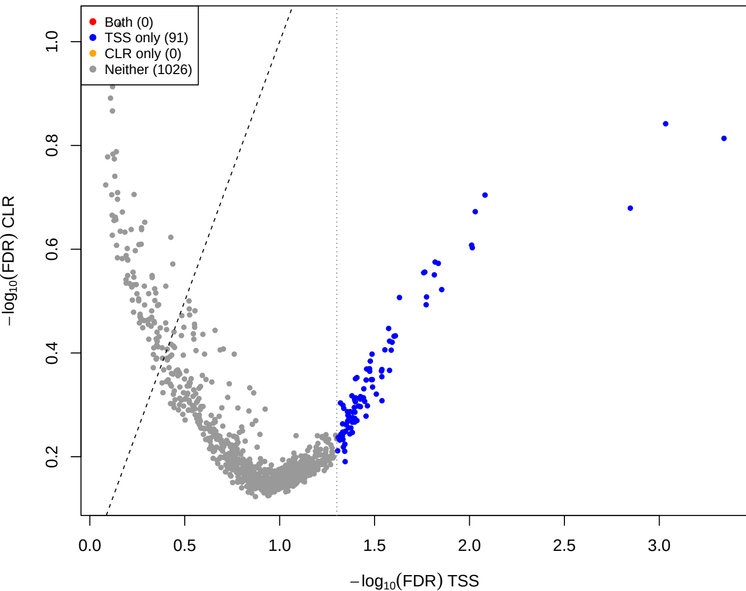
eld vs you – CLR vs TSS(const=2) (gamma = 1)
