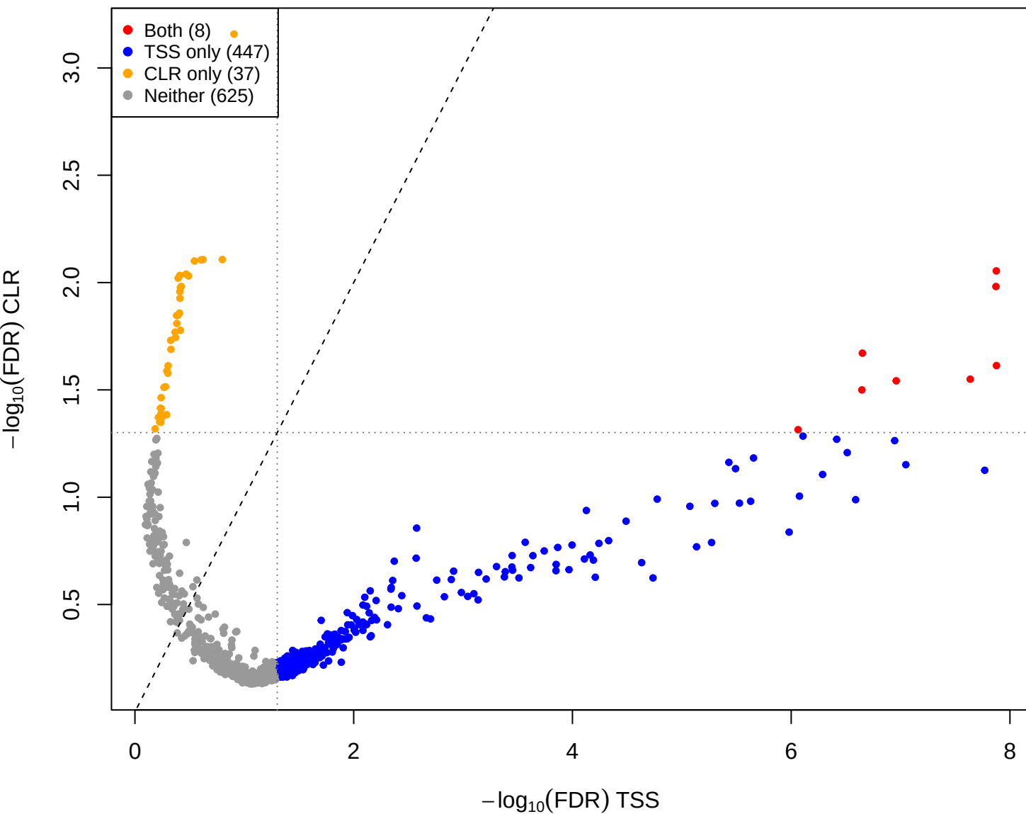
mage vs you – CLR vs TSS(const=2) (gamma = 1)
