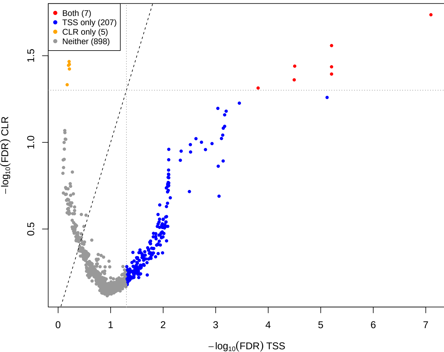
cent vs eld – CLR vs TSS(const=2) (gamma = 1)
