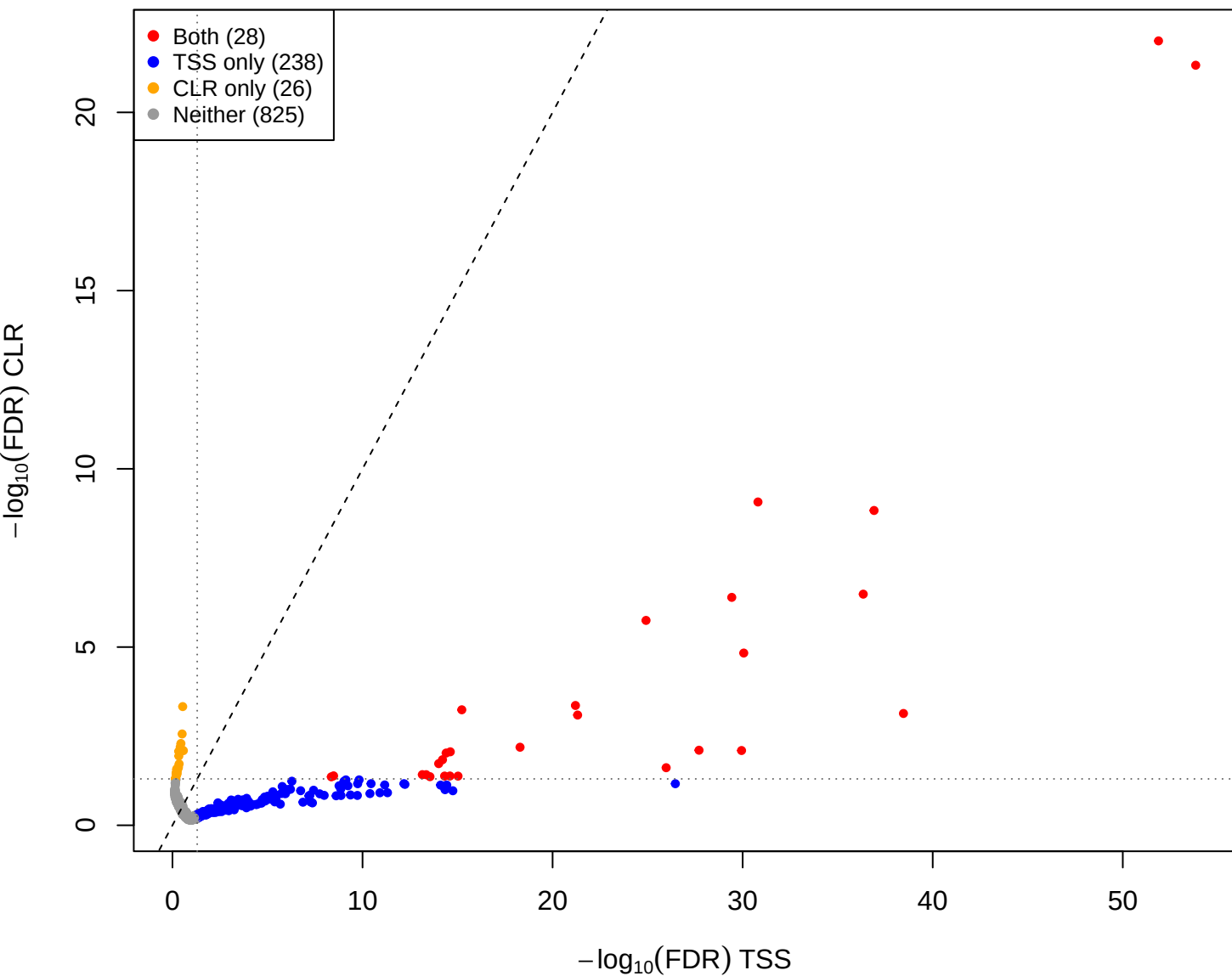
cent vs kin – CLR vs TSS(const=2) (gamma = 1)
