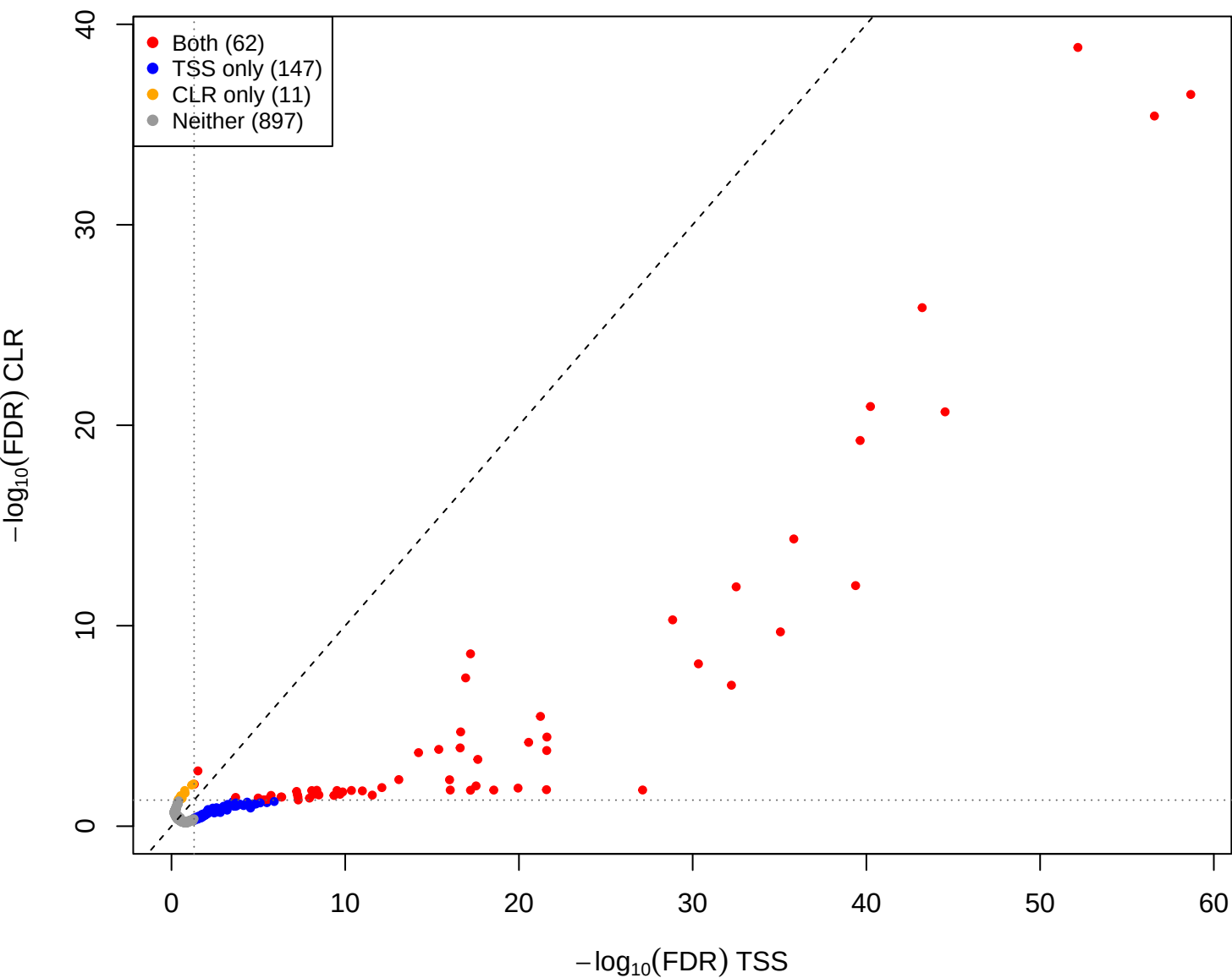
cent vs pup – CLR vs TSS(const=2) (gamma = 1)
