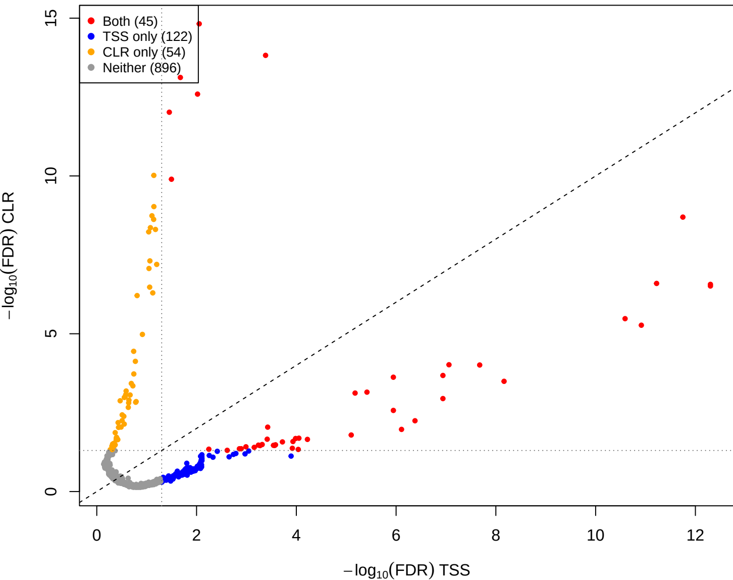
kin vs you – CLR vs TSS(const=2) (gamma = 1)
