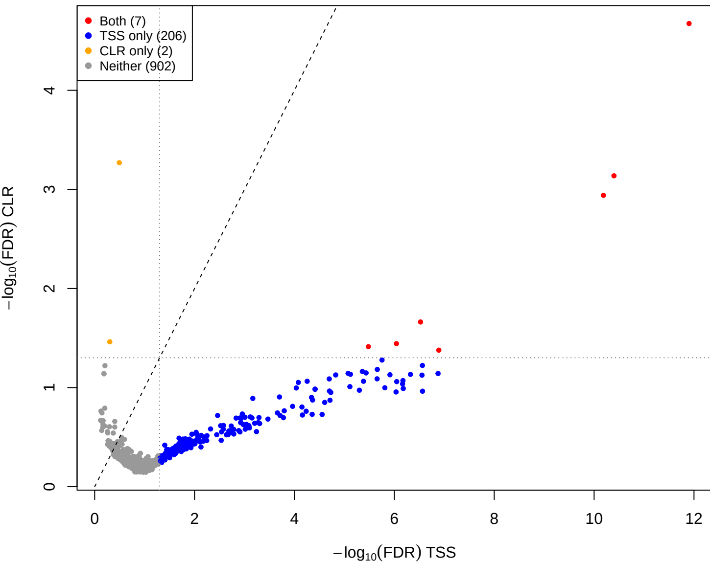
kin vs mid – CLR vs TSS(const=2) (gamma = 1)
