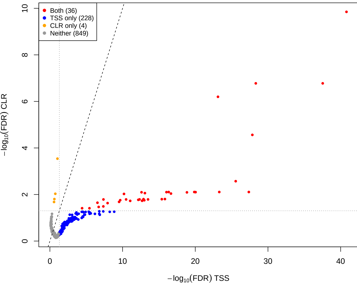
cent vs mid – CLR vs TSS(const=2) (gamma = 1)
