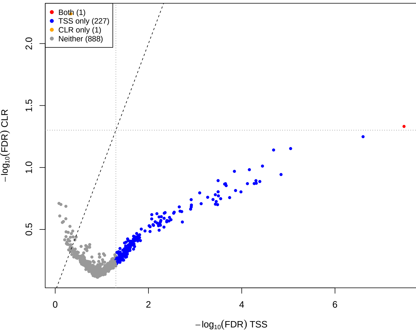
mage vs mid – CLR vs TSS(const=2) (gamma = 1)
