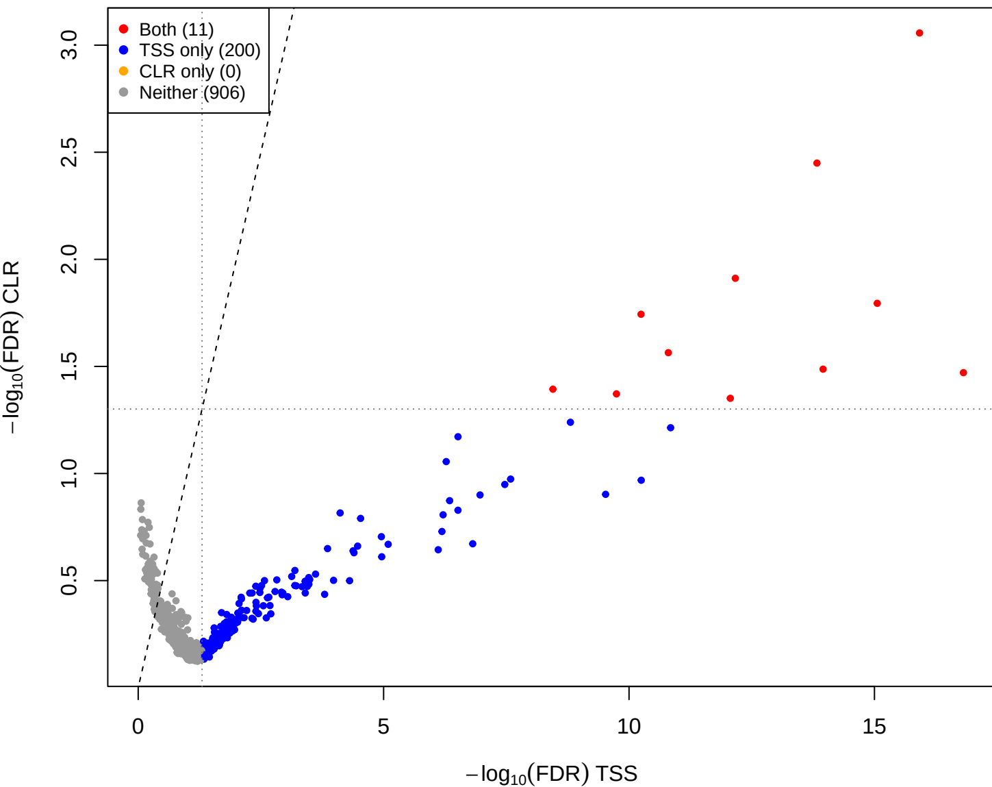
eld vs mage – CLR vs TSS(const=2) (gamma = 1)
