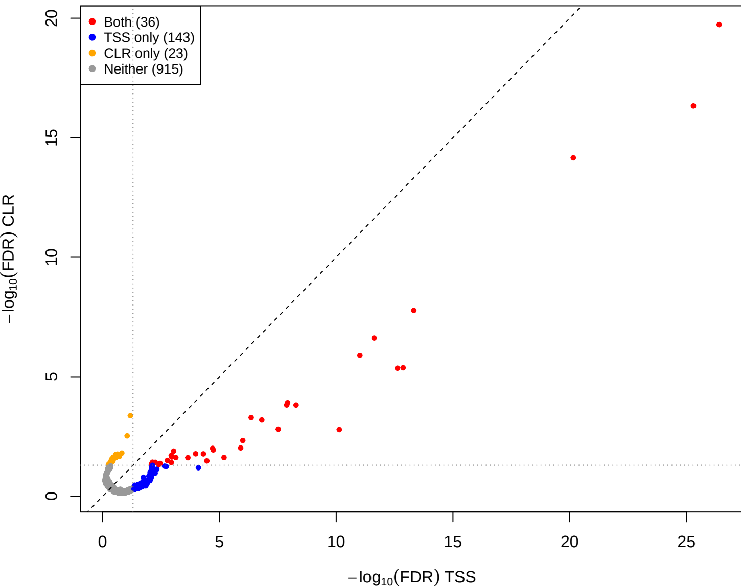
eld vs kin - CLR vs TSS(const=2) (gamma = 1)
