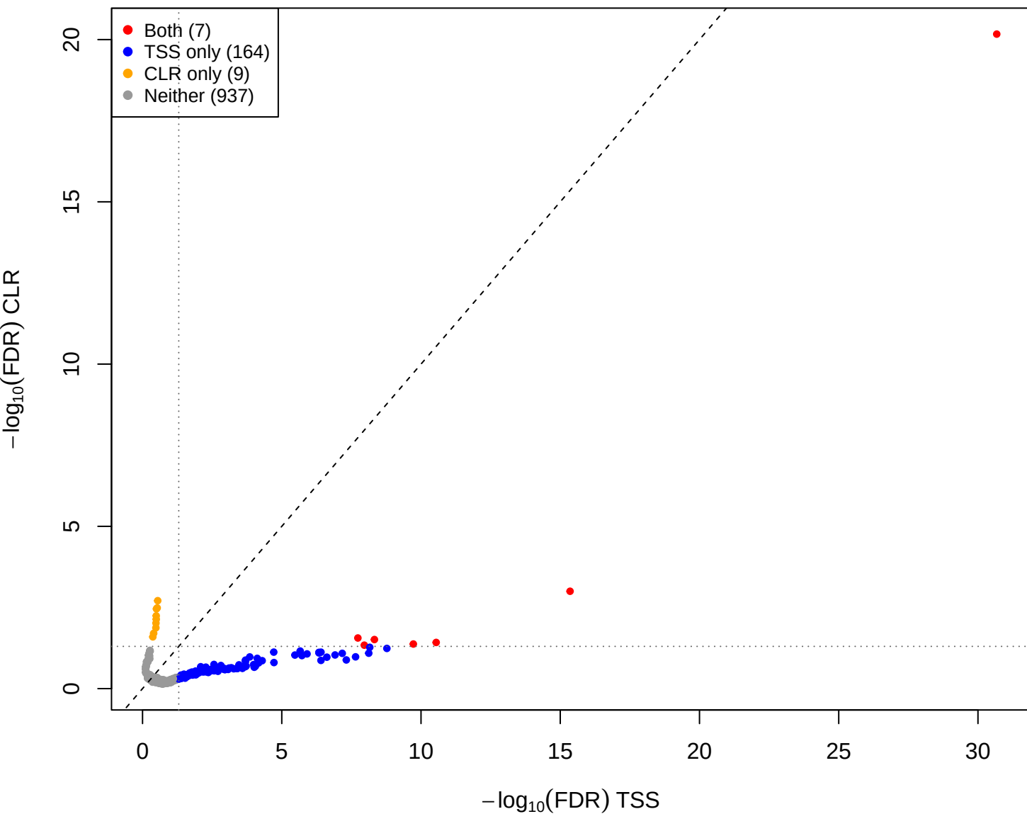
mage vs pup – CLR vs TSS(const=2) (gamma = 1)
