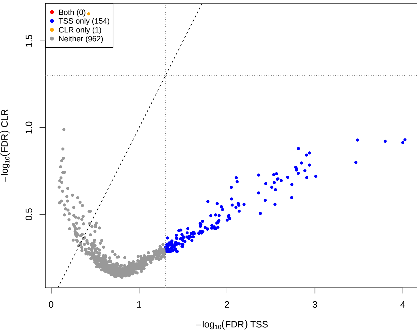
kin vs mage – CLR vs TSS(const=2) (gamma = 1)
