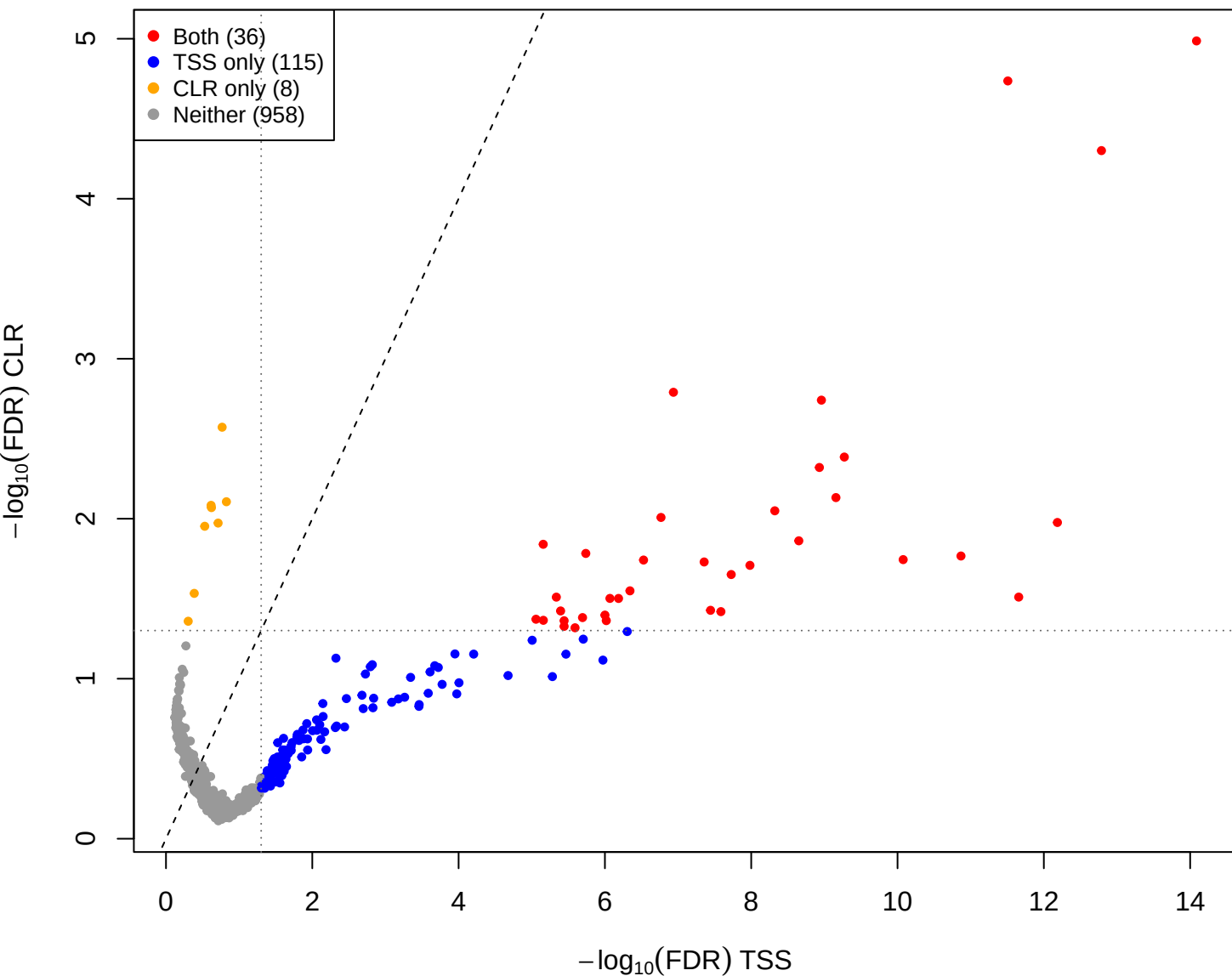
cent vs mage - CLR vs TSS(const=2) (gamma = 1)
