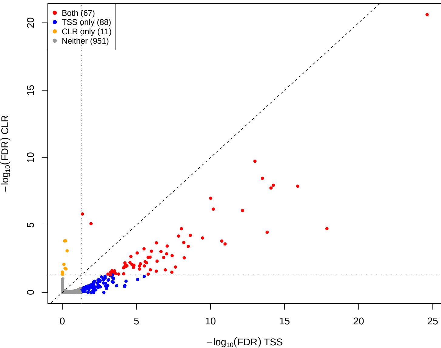
kin vs pup – CLR vs TSS(const=1) (gamma = 1e-05)
