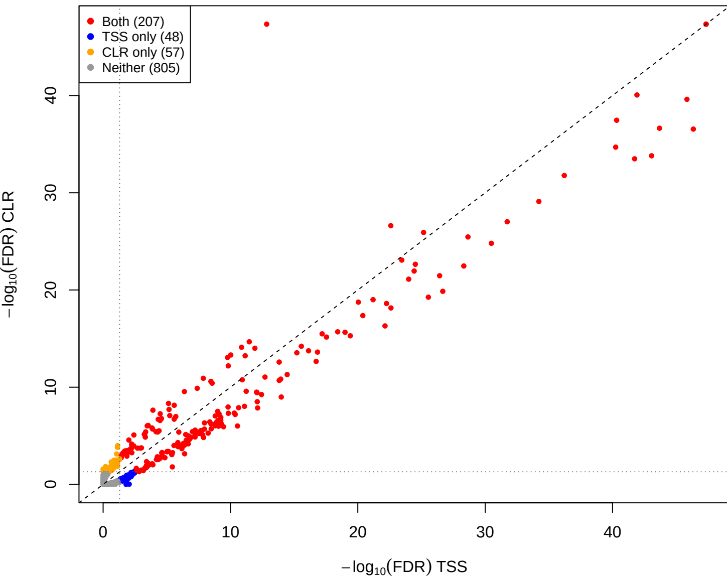
eld vs pup – CLR vs TSS(const=1) (gamma = 1e-05)
