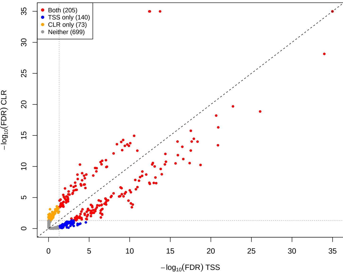
cent vs you – CLR vs TSS(const=1) (gamma = 1e-05)
