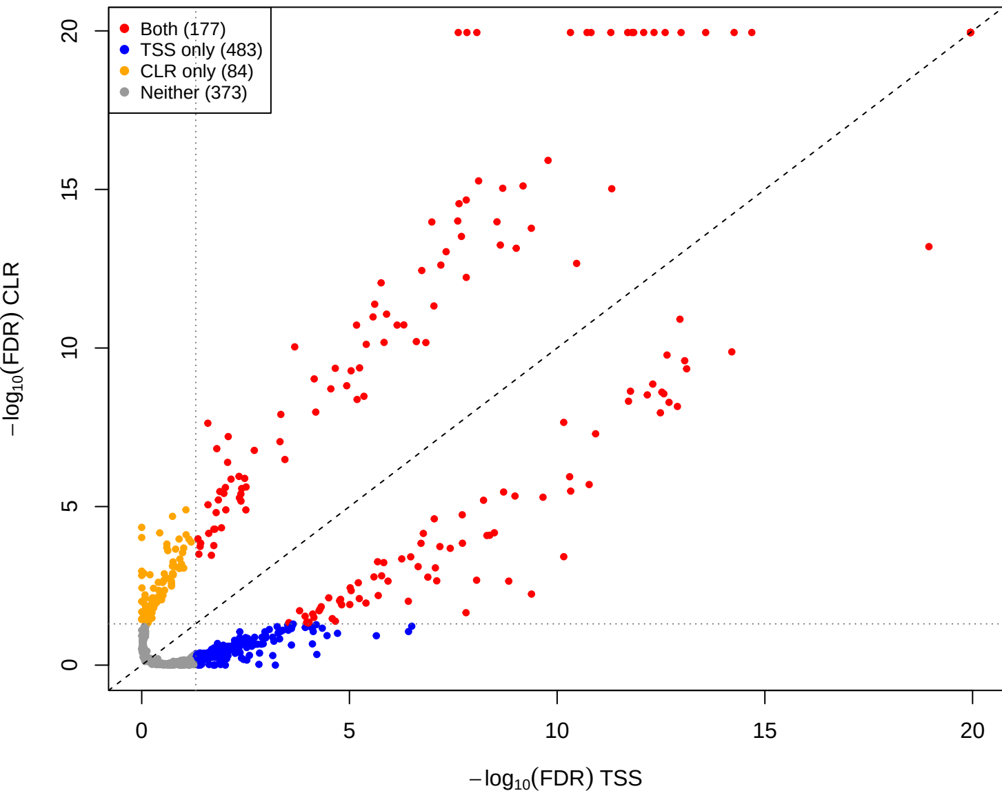
mid vs you - CLR vs TSS(const=1) (gamma = 1e-05)
