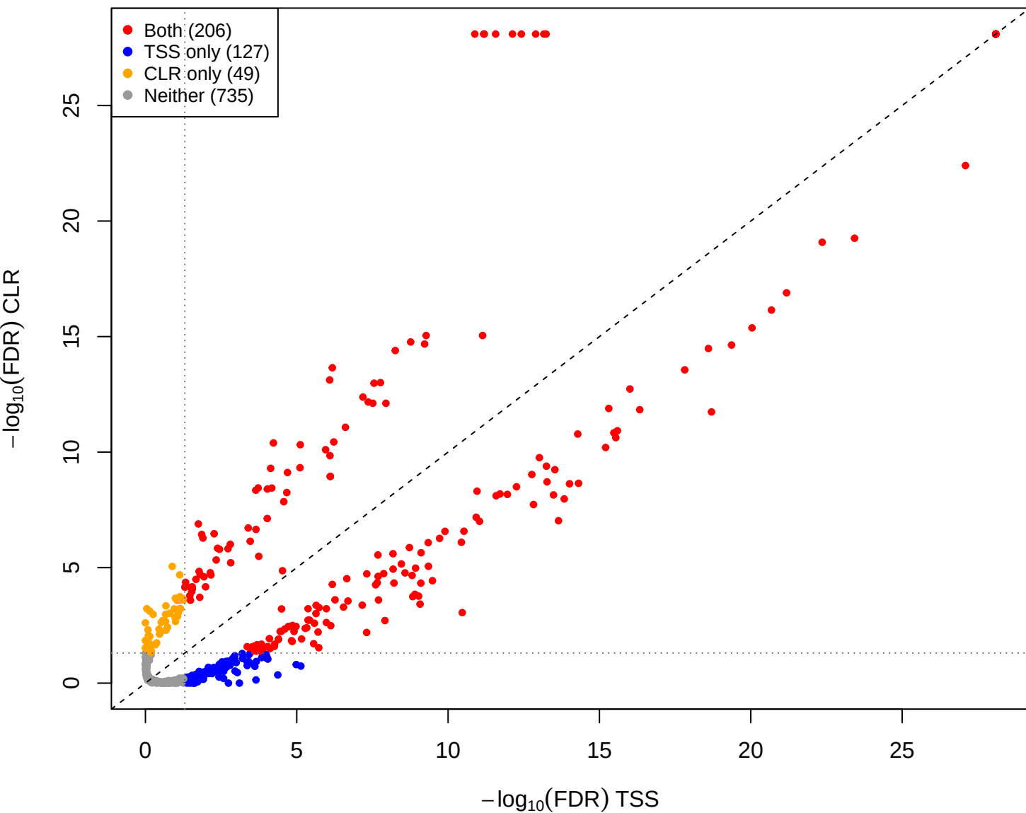
kin vs you – CLR vs TSS(const=1) (gamma = 1e-05)
