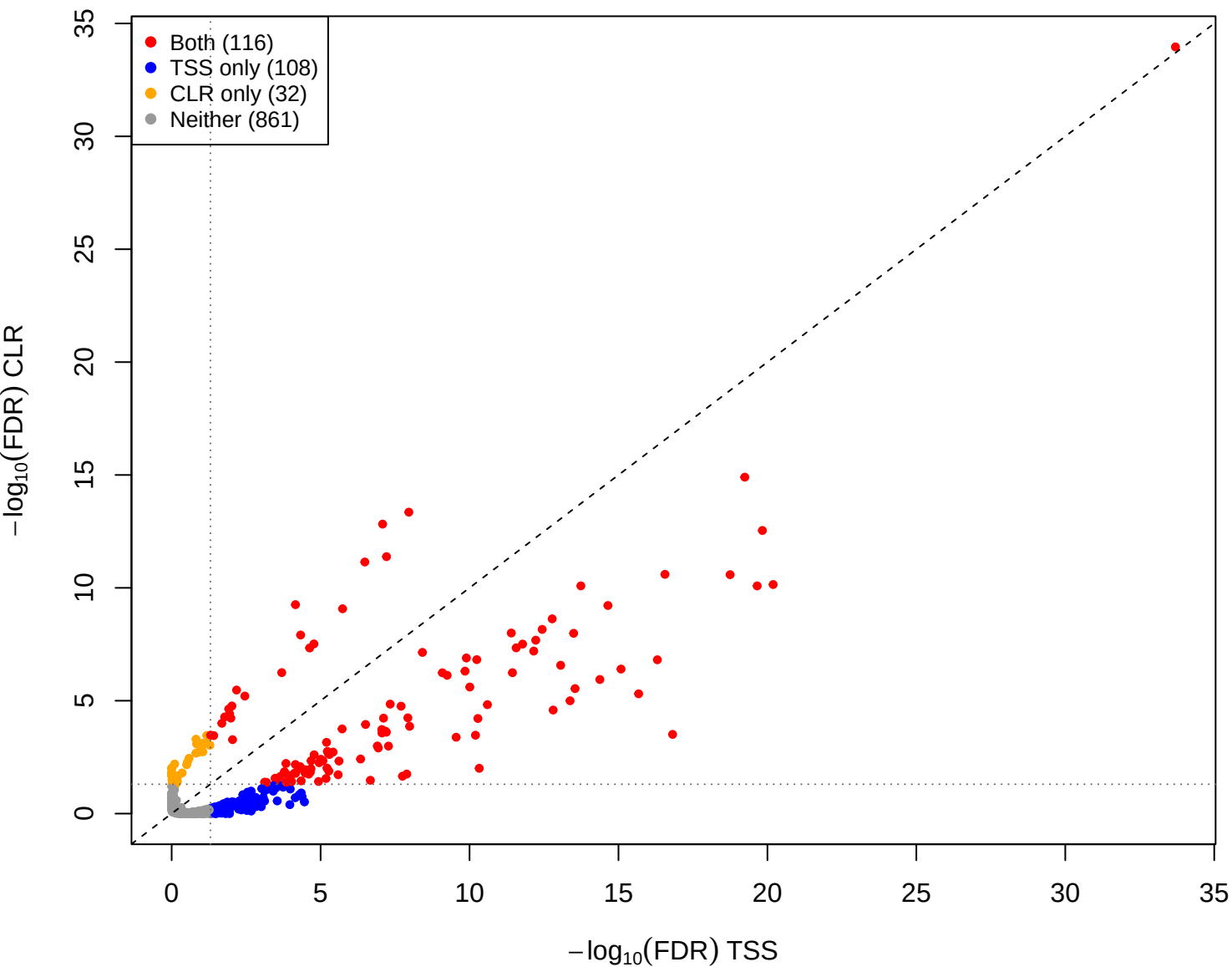
mage vs pup – CLR vs TSS(const=1) (gamma = 1e-05)
