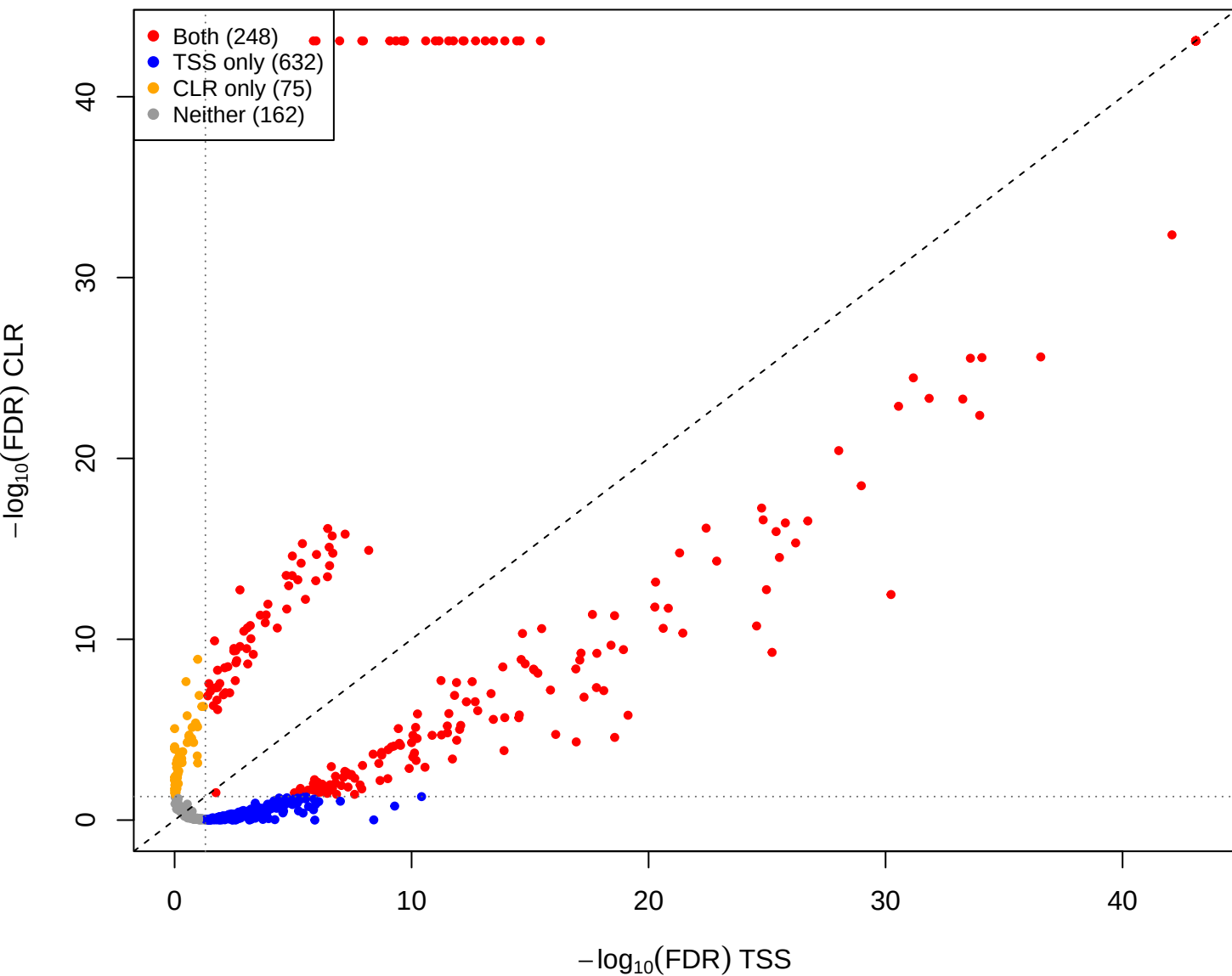
pup vs you – CLR vs TSS(const=1) (gamma = 1e-05)
