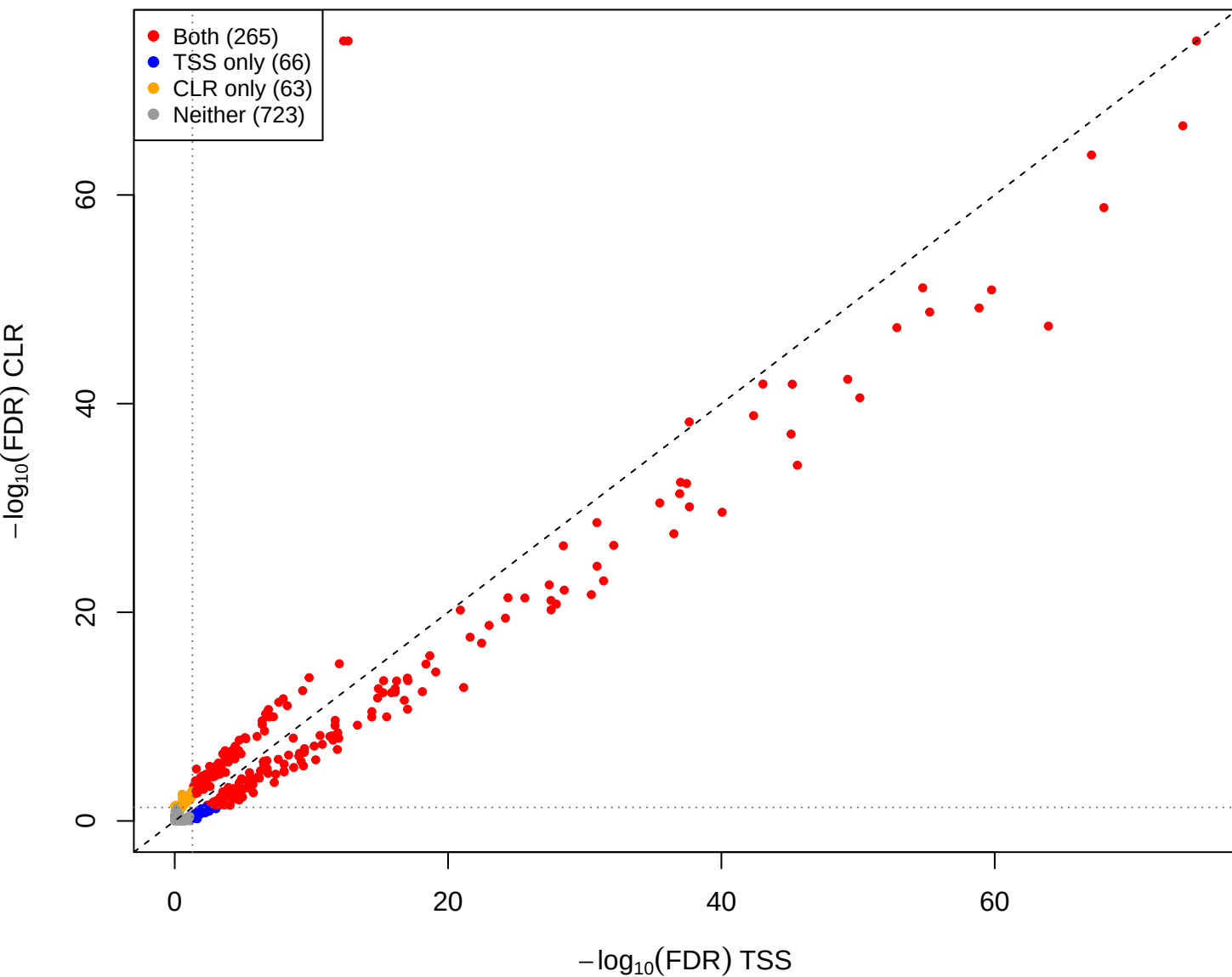
cent vs pup – CLR vs TSS(const=1) (gamma = 1e-05)
