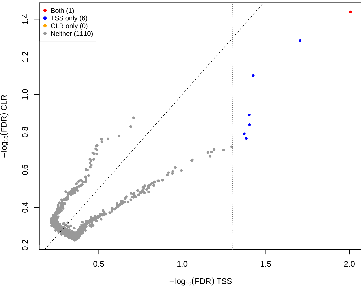
eld vs kin - CLR vs TSS(const=1) (gamma = 3)
