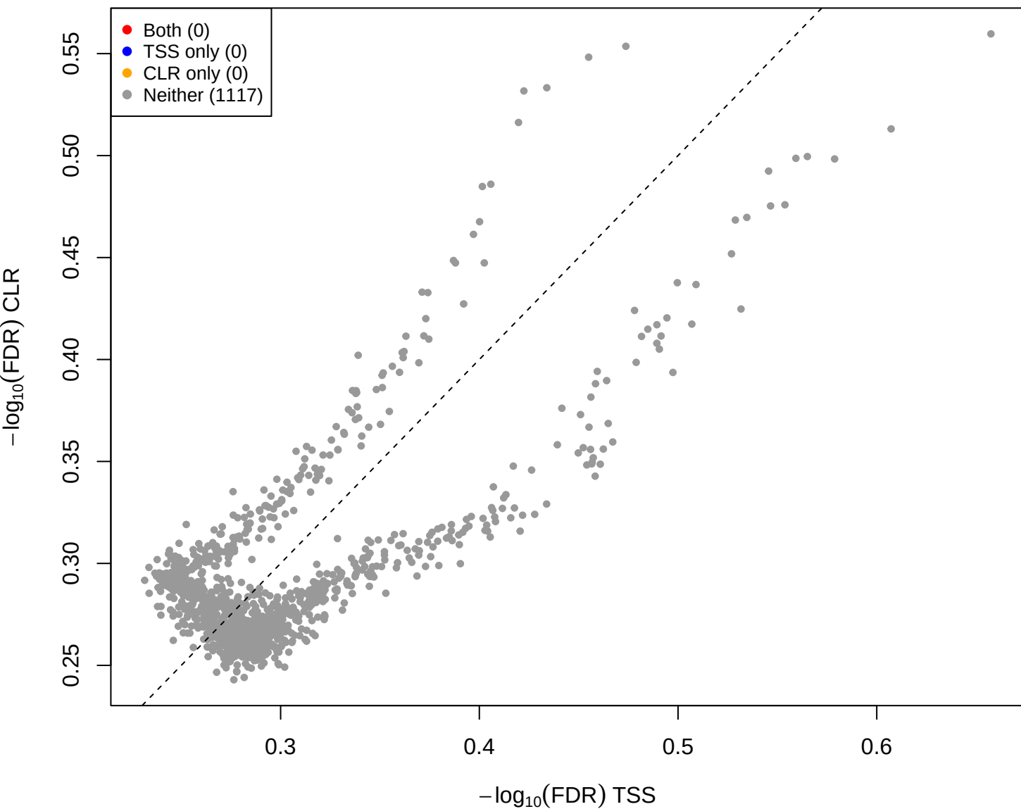
cent vs eld – CLR vs TSS(const=1) (gamma = 3)
