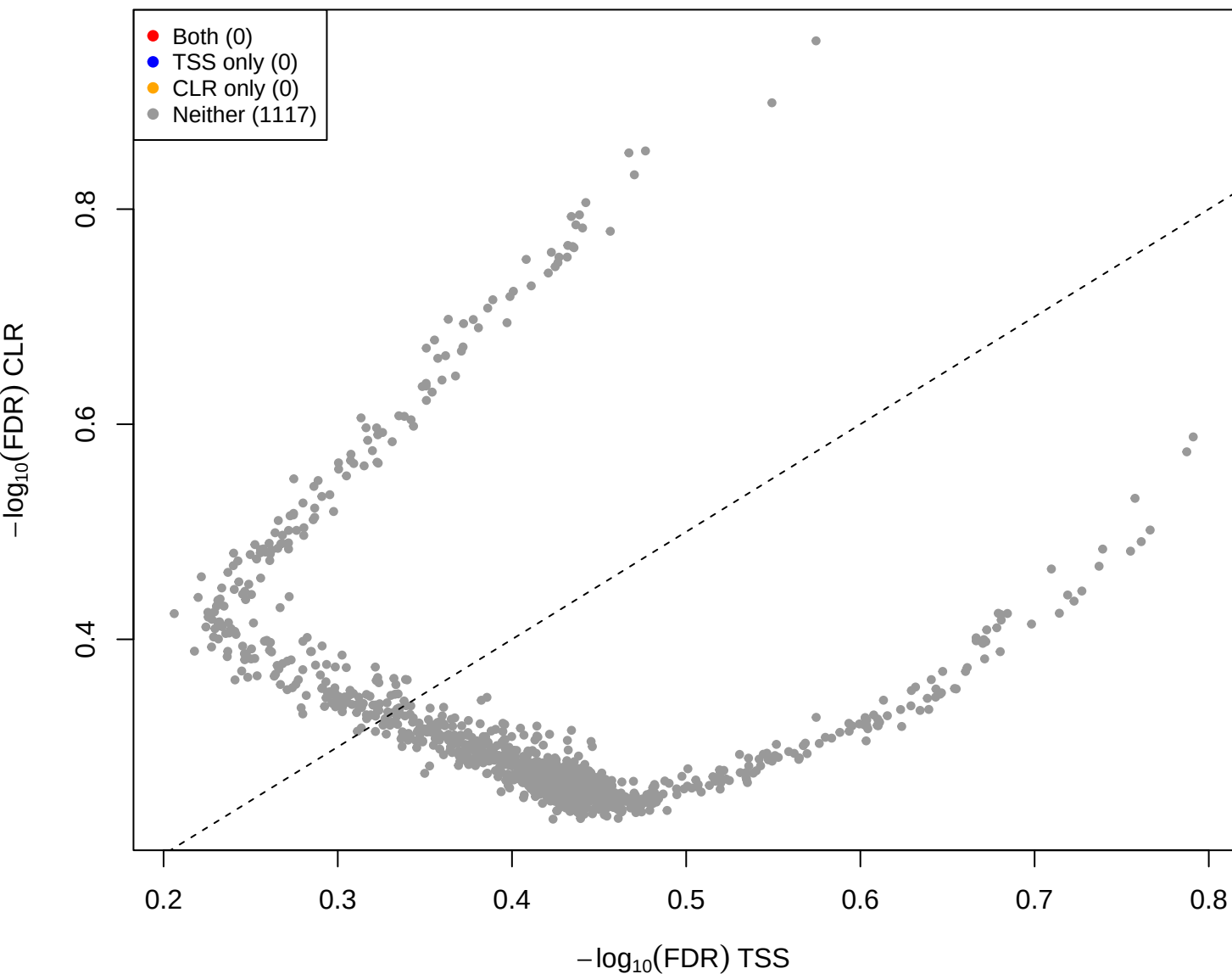
mage vs you – CLR vs TSS(const=1) (gamma = 3)
