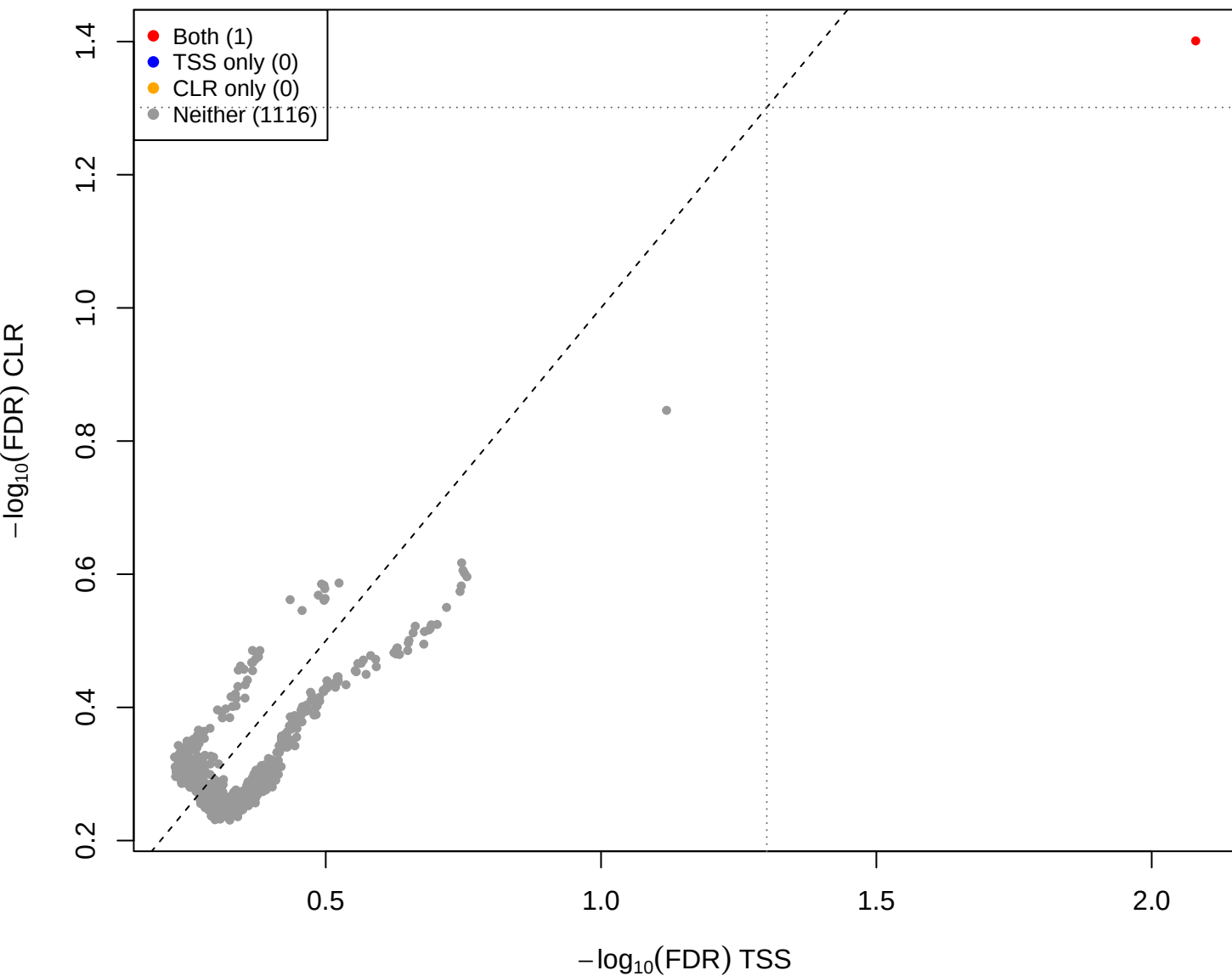
mage vs pup – CLR vs TSS(const=1) (gamma = 3)
