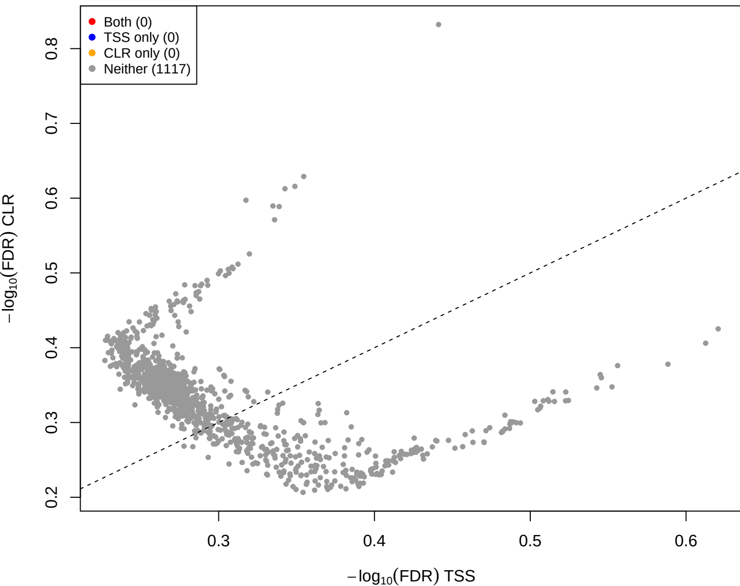
mage vs mid – CLR vs TSS(const=1) (gamma = 3)
