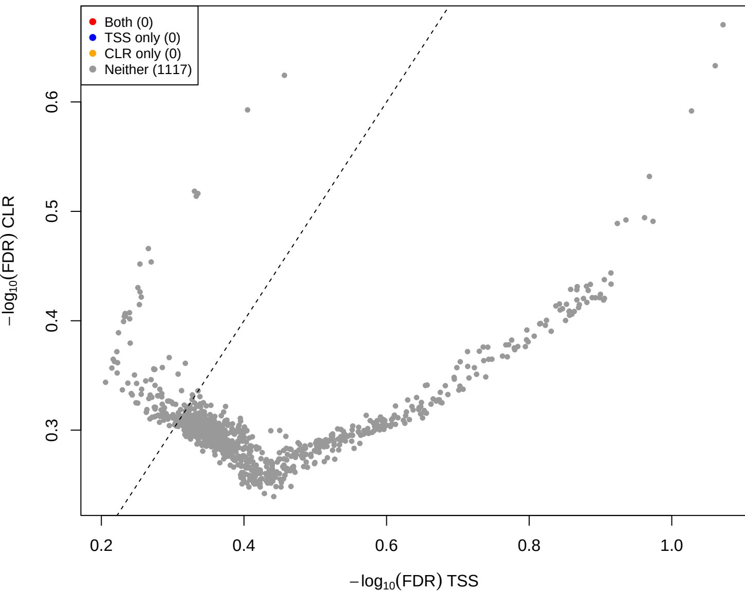
kin vs mid – CLR vs TSS(const=1) (gamma = 3)
