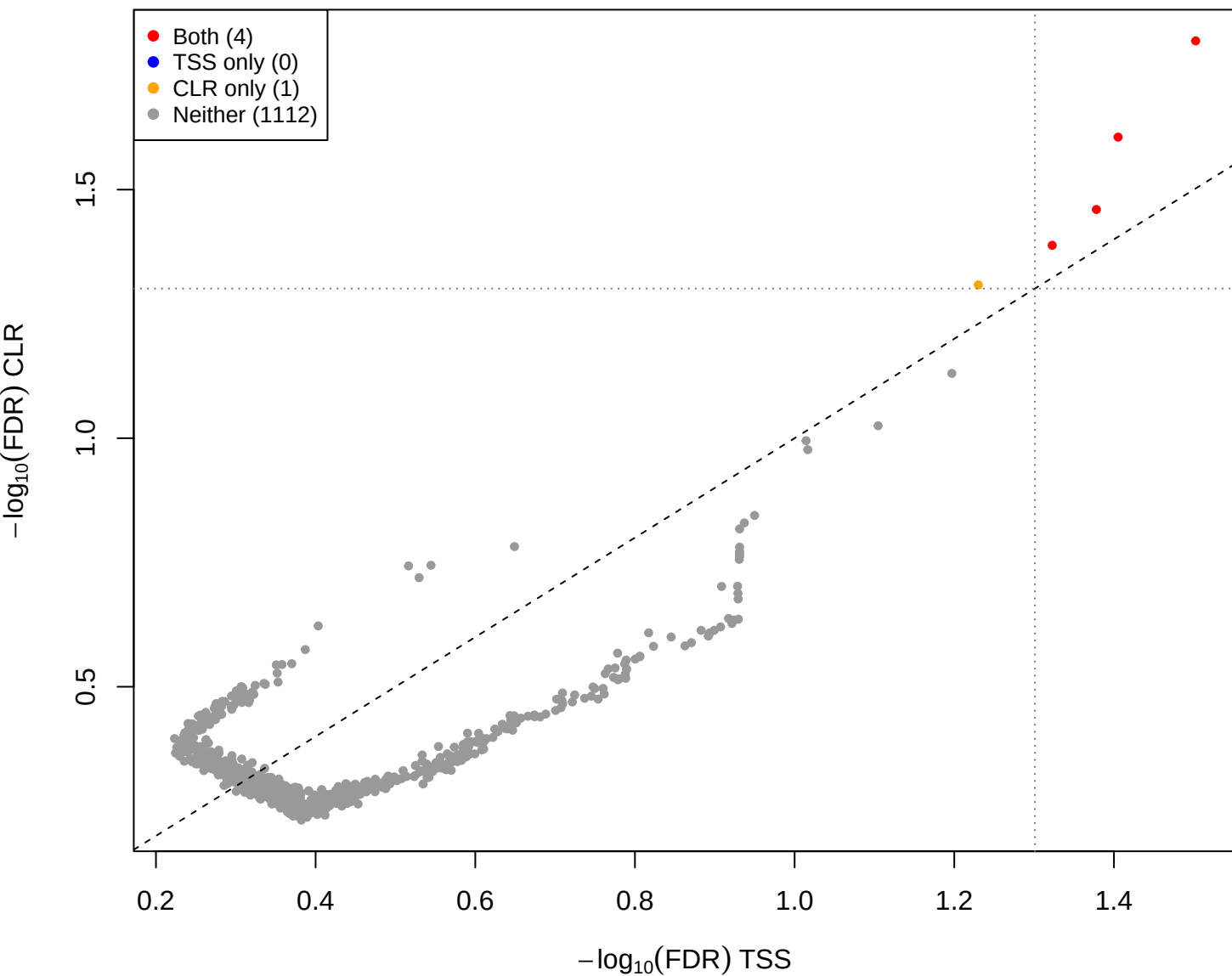
cent vs mid – CLR vs TSS(const=1) (gamma = 3)
