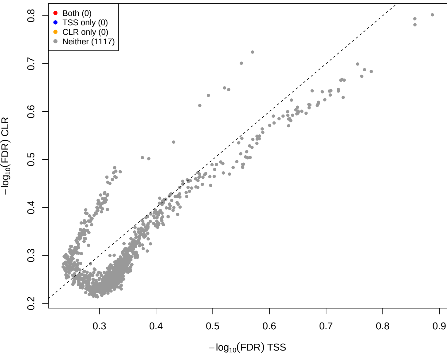
cent vs mage - CLR vs TSS(const=1) (gamma = 3)
