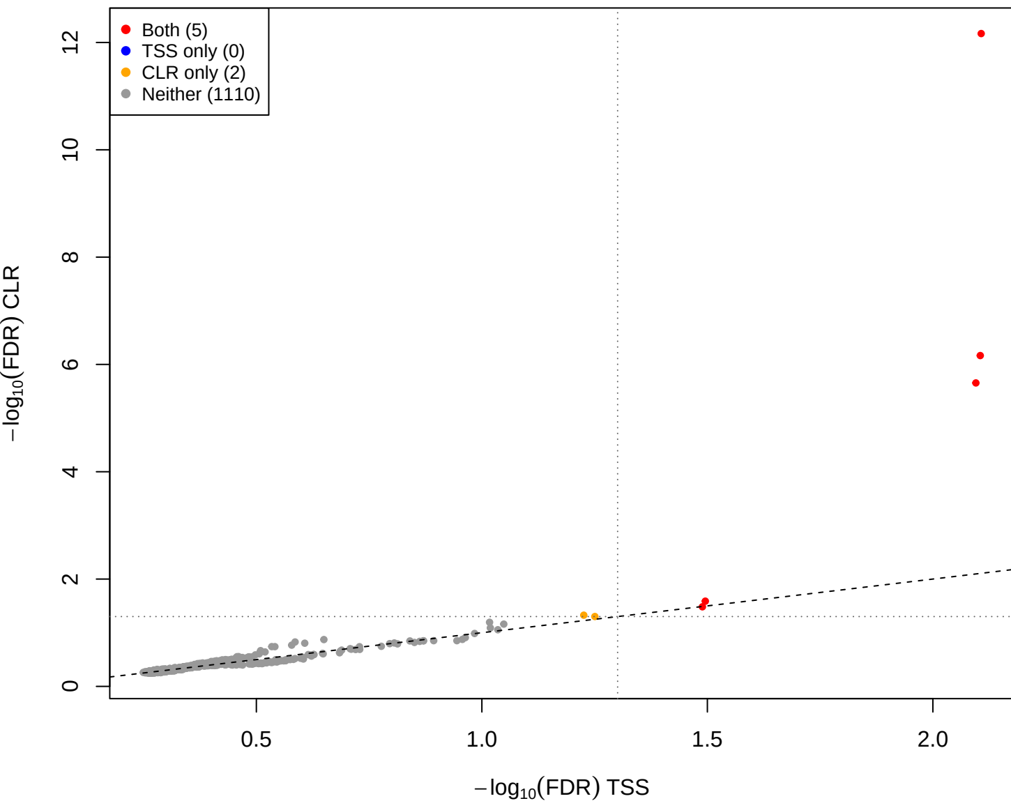
cent vs pup – CLR vs TSS(const=1) (gamma = 3)
