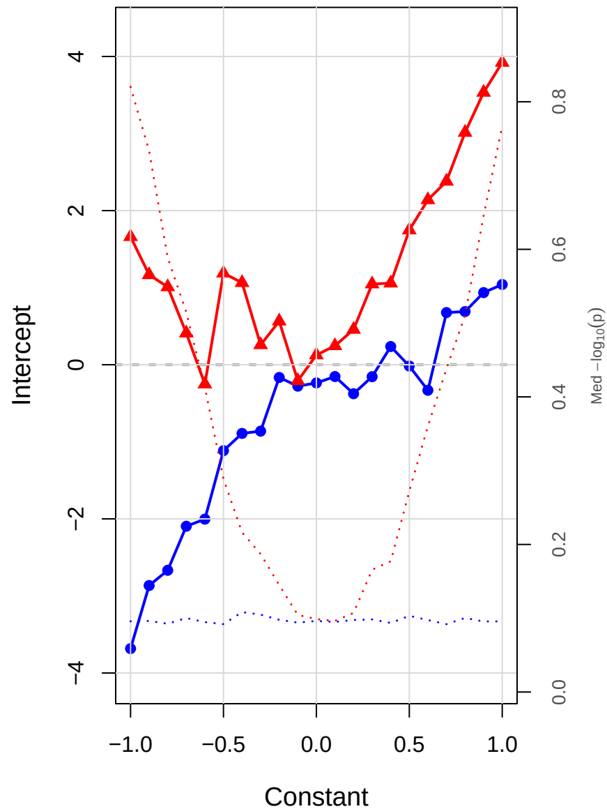
CLR_const | eld vs kin | gamma=0.1 Intercept
