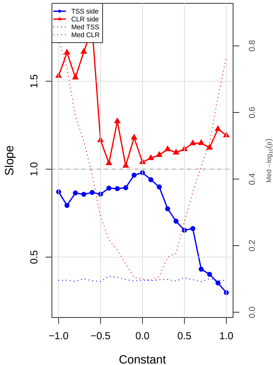
CLR_const | eld vs kin | gamma=0.1 Slope
