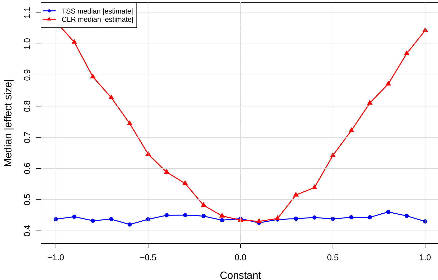
CLR_const | eld vs kin | gamma=0.1 Median absolute effect size across all features
