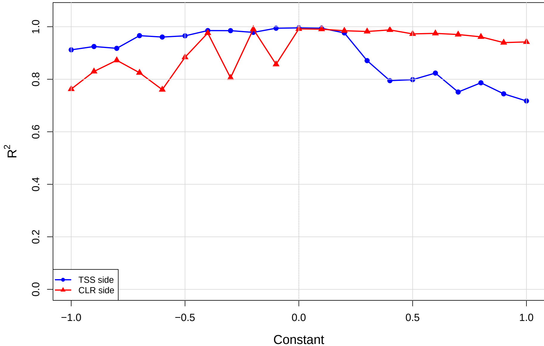
CLR_const | eld vs kin | gamma=0.1 R-squared of red-dot regression
