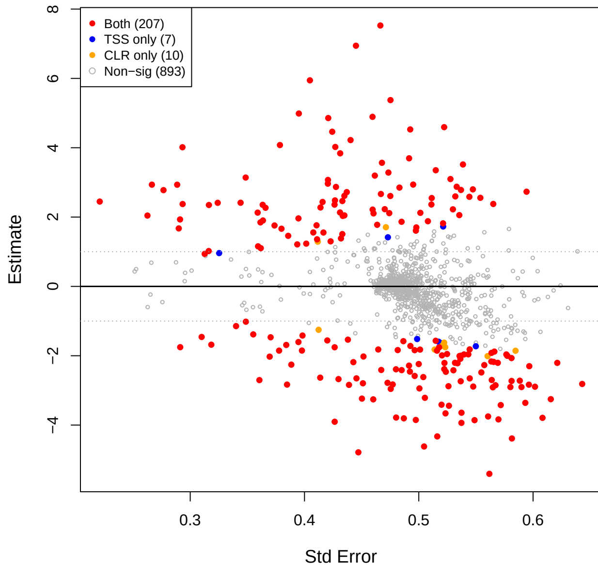
eld vs kin – CLR(const=0) effect space
