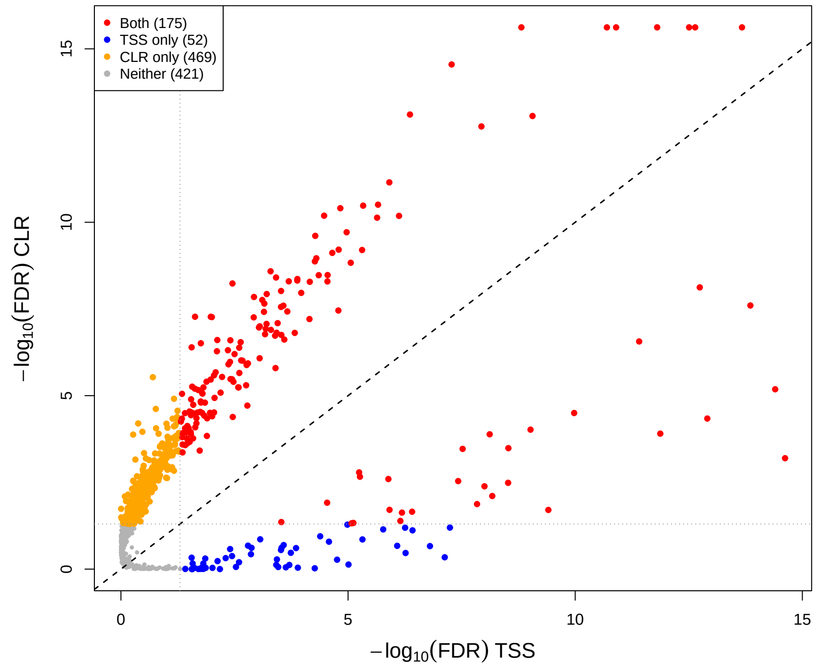
cent vs mage – CLR(const=-0.9) vs TSS (gamma = 0.1)
