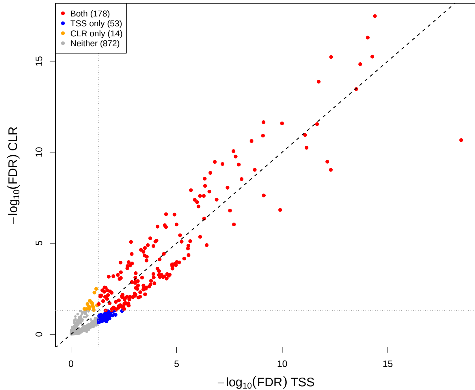
cent vs mage – CLR(const=0.2) vs TSS (gamma = 0.1)
