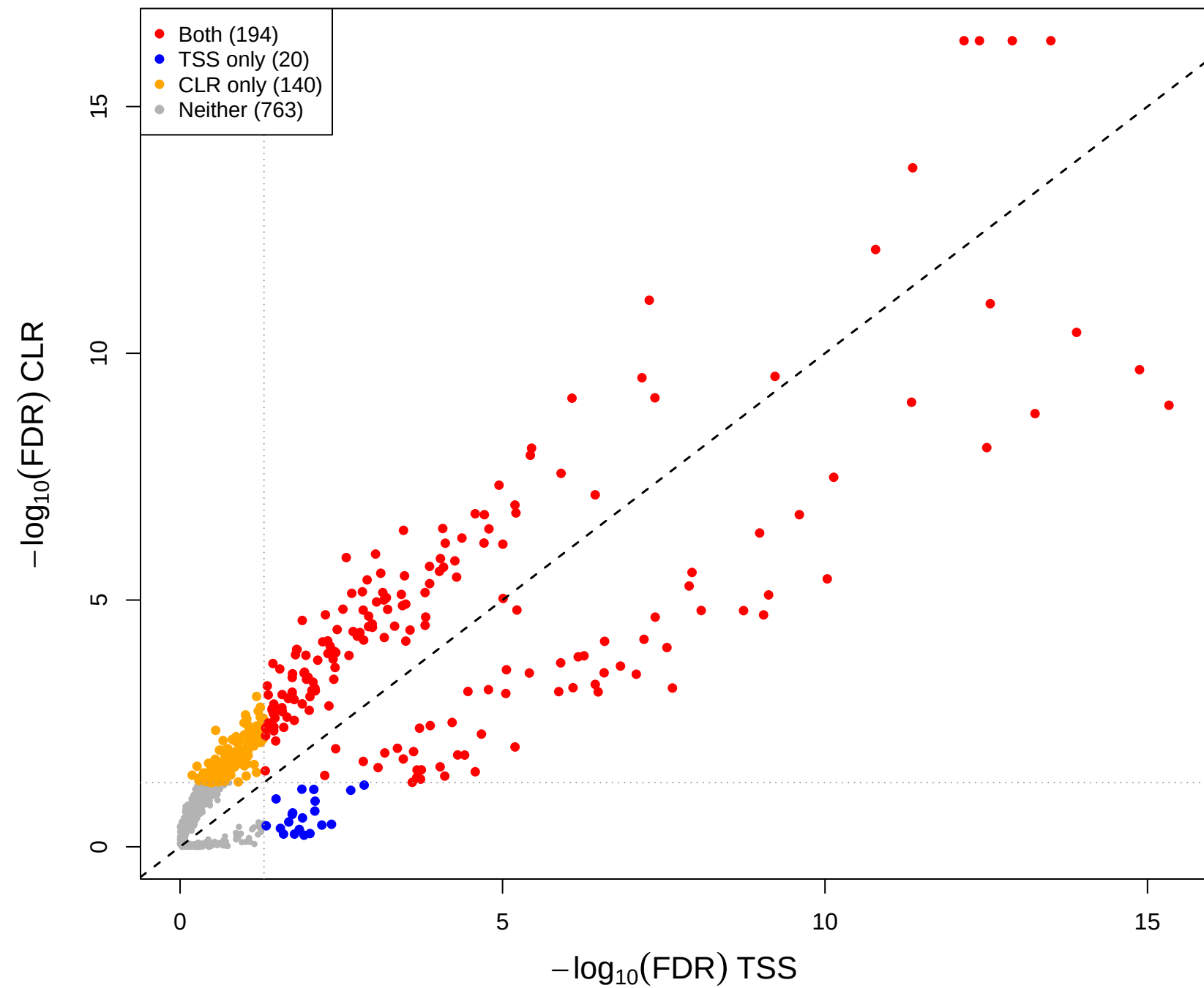
cent vs mage – CLR(const=-0.4) vs TSS (gamma = 0.1)
