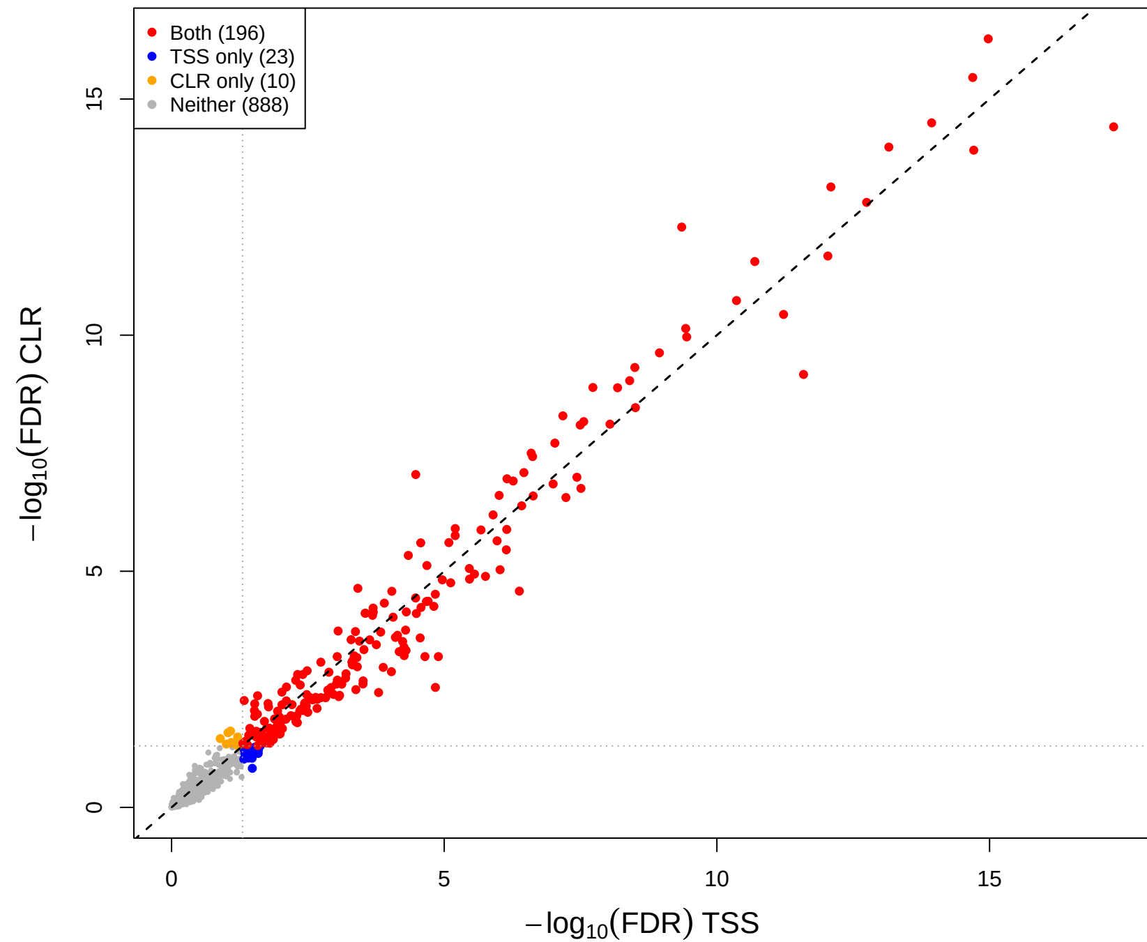
cent vs mage – CLR(const=0.1) vs TSS (gamma = 0.1)
