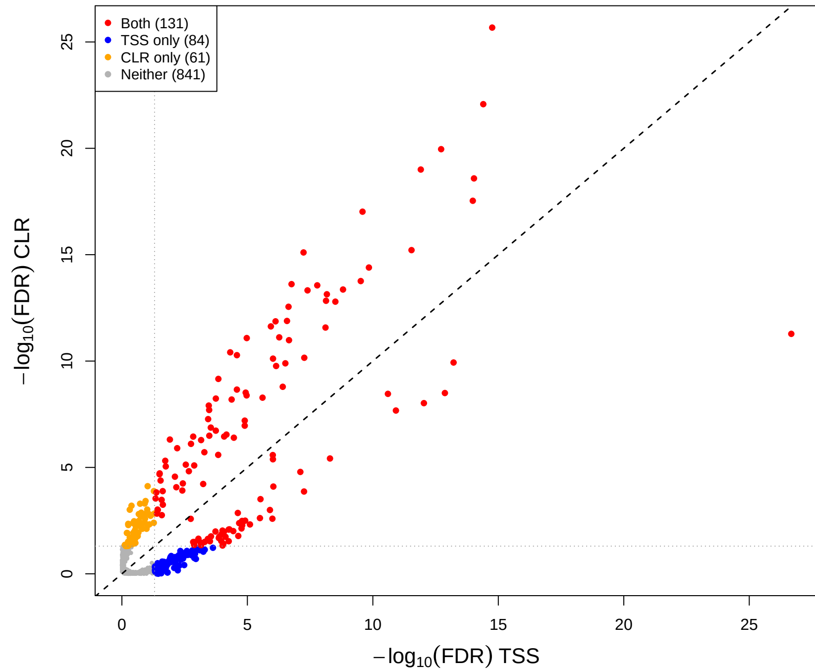
cent vs mage – CLR(const=0.6) vs TSS (gamma = 0.1)
