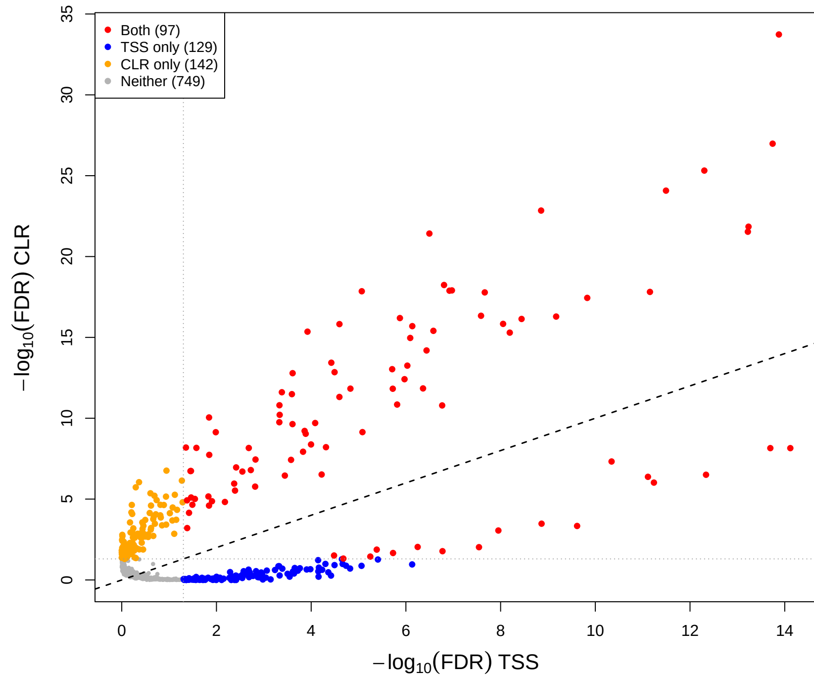
cent vs mage – CLR(const=1) vs TSS (gamma = 0.1)
