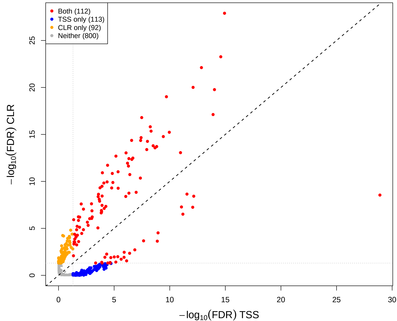
cent vs mage – CLR(const=0.8) vs TSS (gamma = 0.1)
