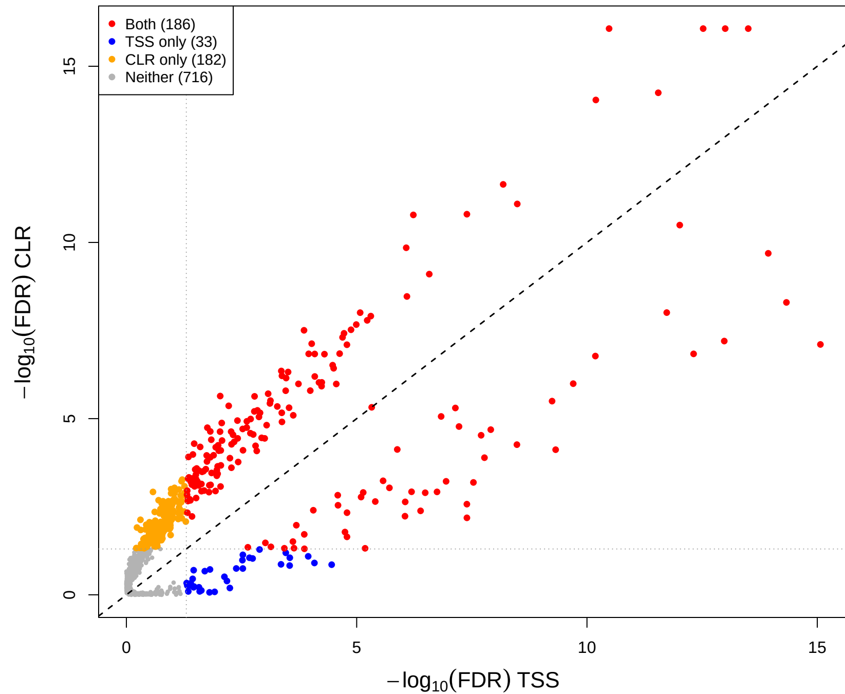
cent vs mage – CLR(const=-0.5) vs TSS (gamma = 0.1)
