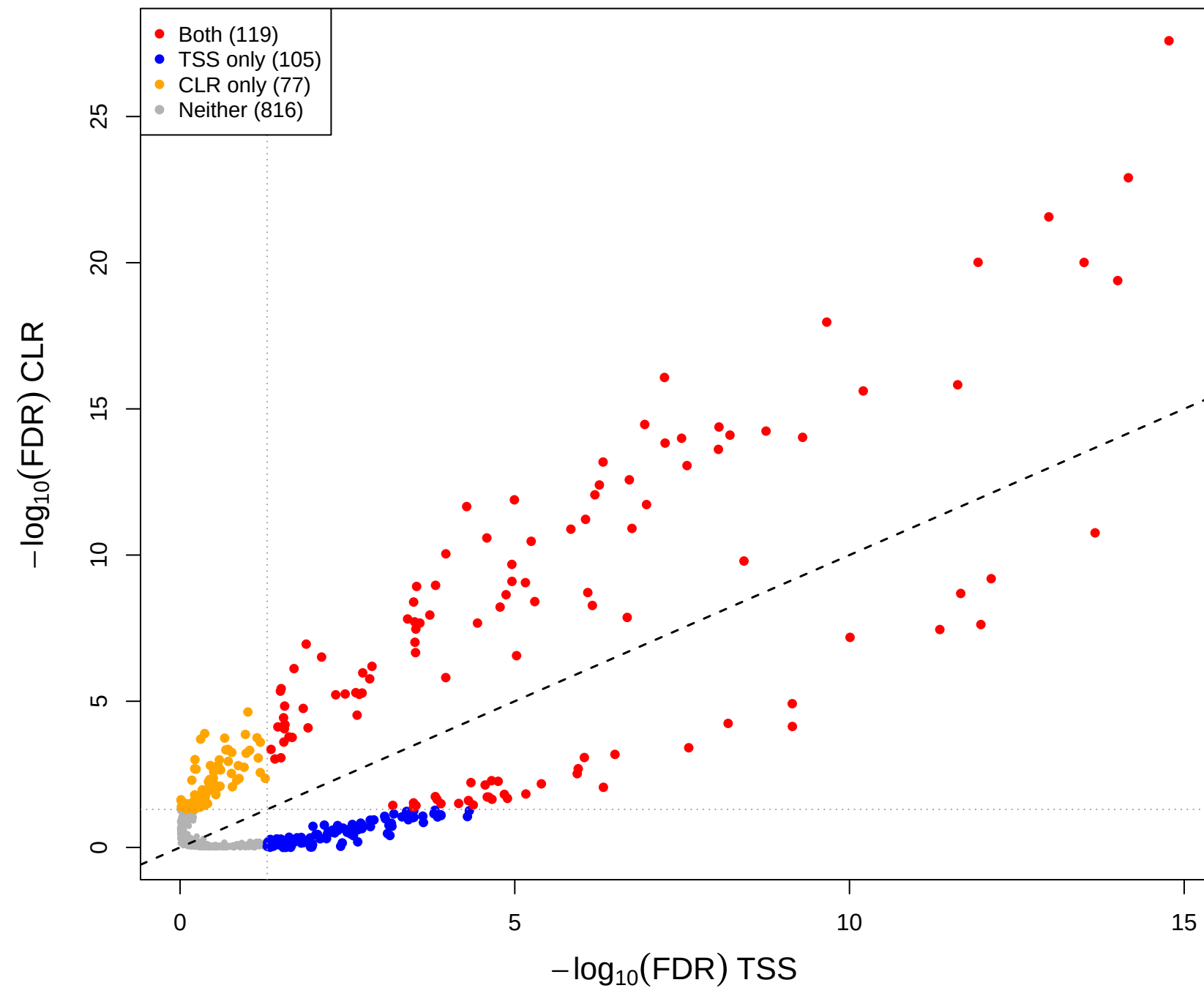
cent vs mage – CLR(const=0.7) vs TSS (gamma = 0.1)
