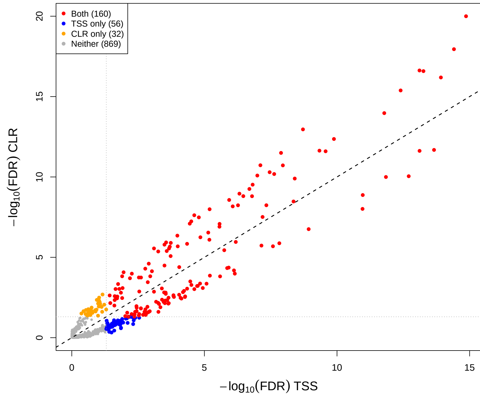
cent vs mage – CLR(const=0.3) vs TSS (gamma = 0.1)
