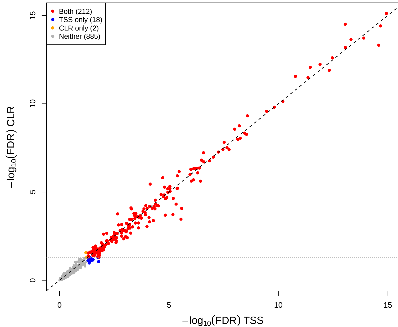
cent vs mage – CLR(const=0) vs TSS (gamma = 0.1)
