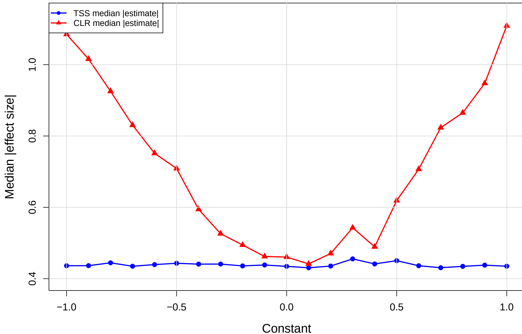
CLR_const | eld vs kin | gamma=0.3 Median absolute effect size across all features
