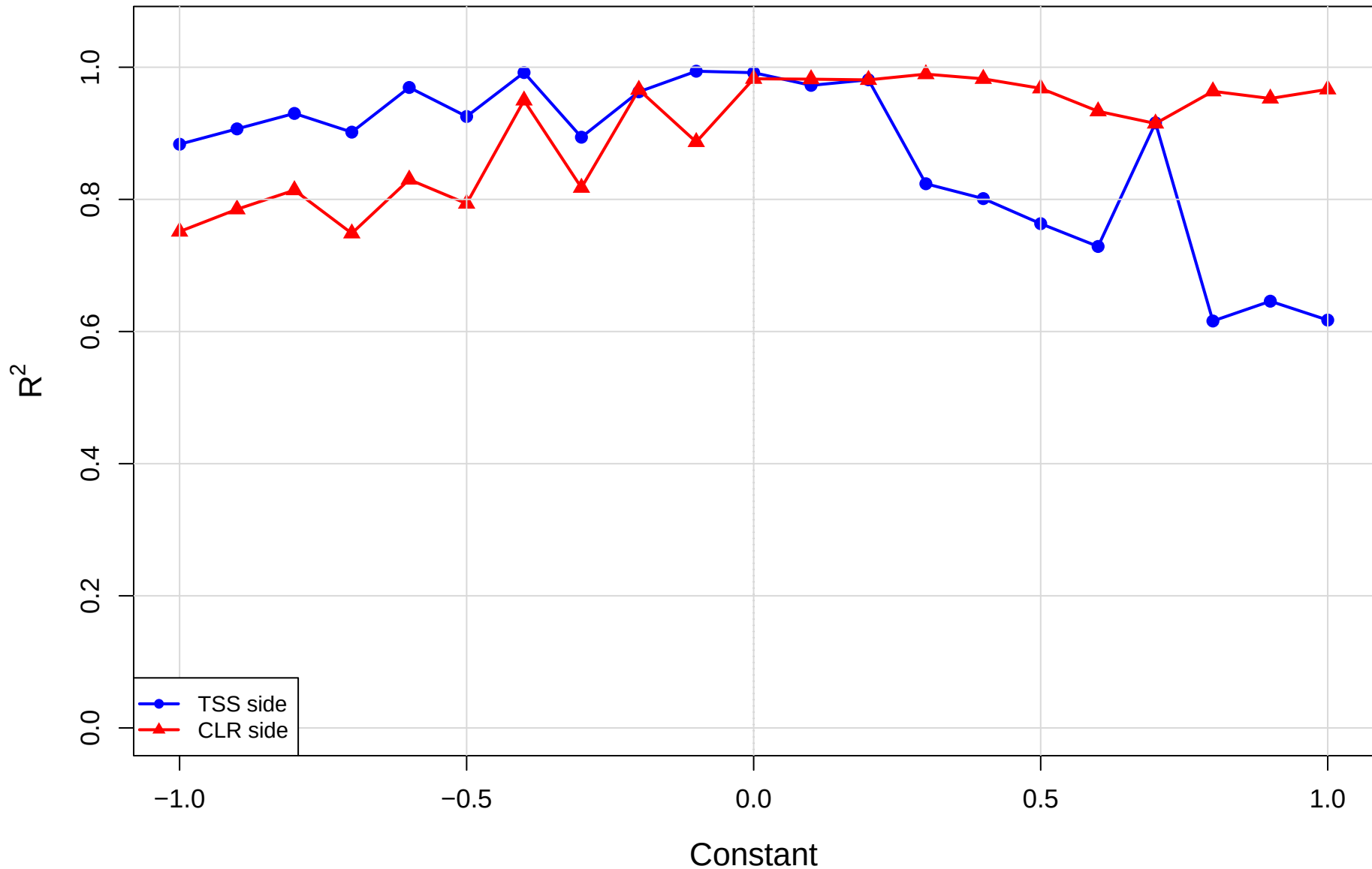
CLR_const | eld vs kin | gamma=0.3 R-squared of red-dot regression
