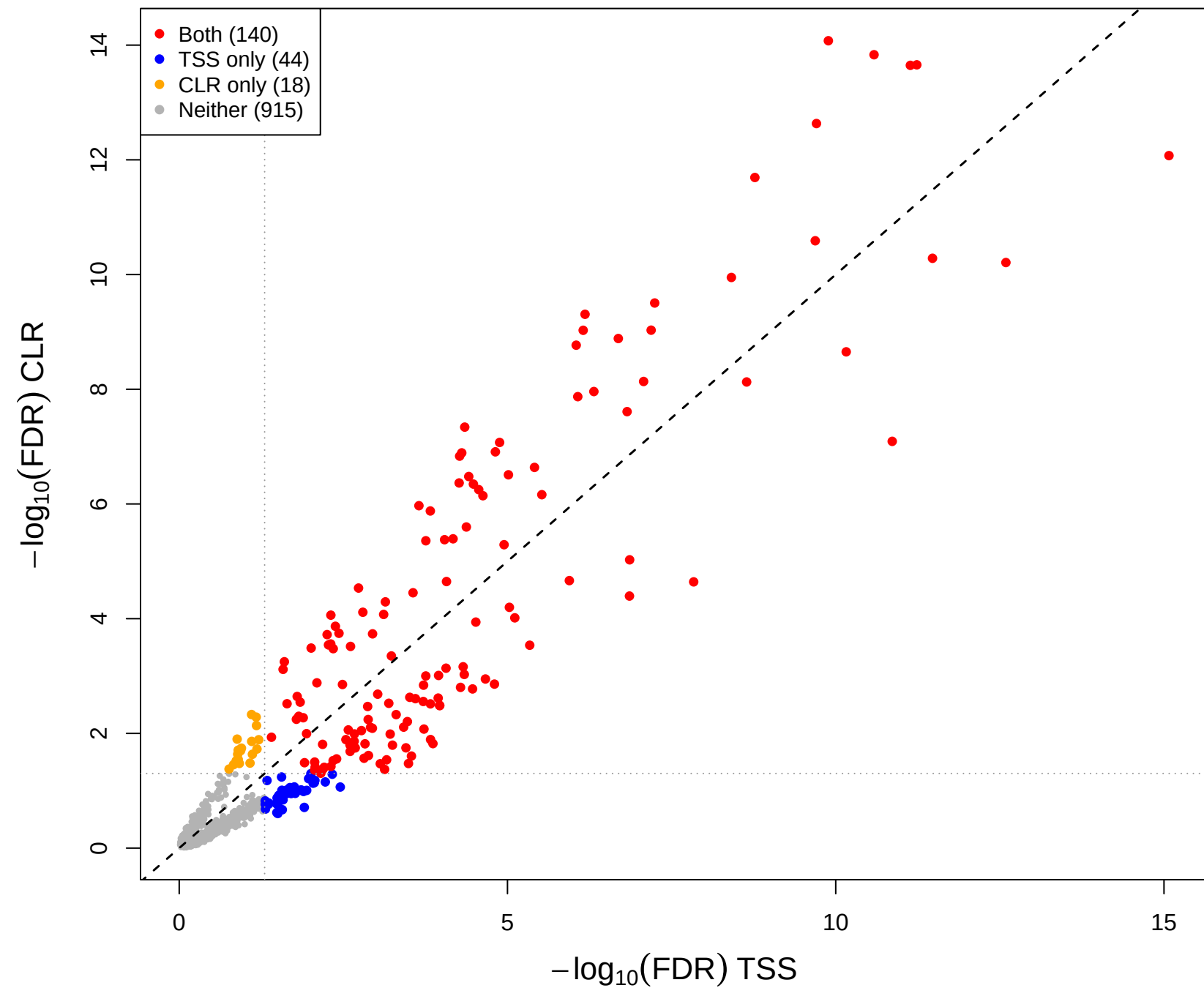
cent vs mage – CLR(const=0.2) vs TSS (gamma = 0.3)
