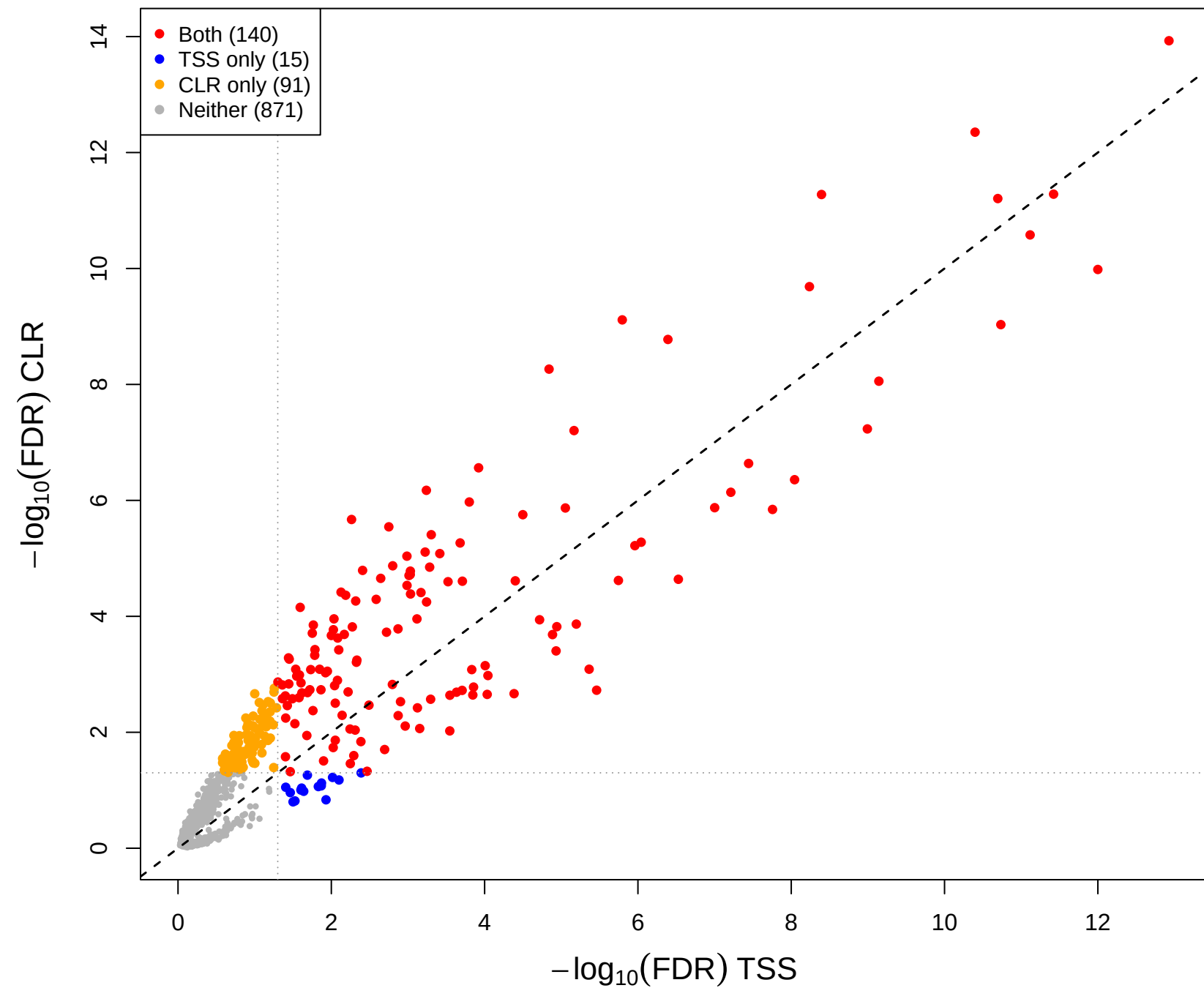
cent vs mage – CLR(const=-0.3) vs TSS (gamma = 0.3)
