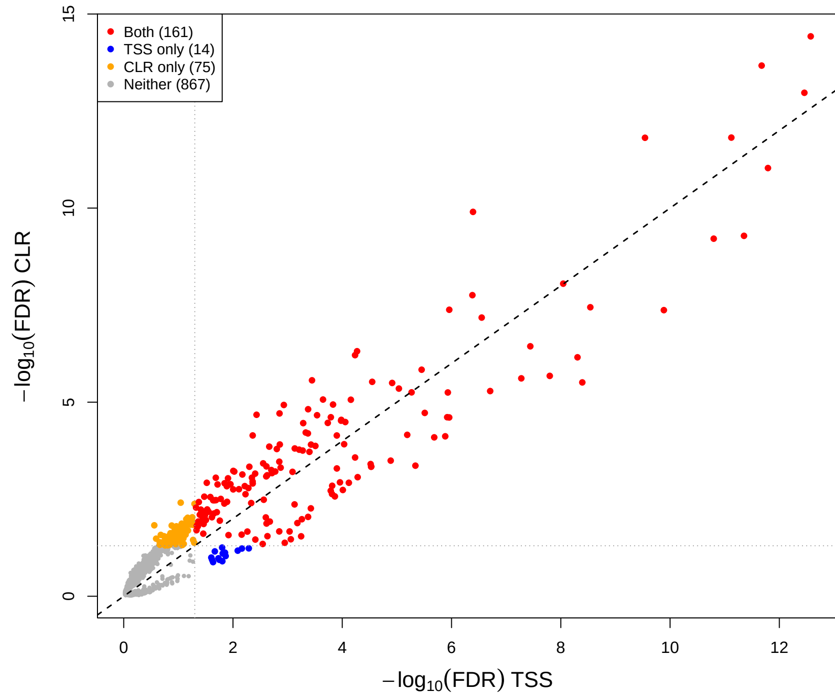
cent vs mage – CLR(const=-0.4) vs TSS (gamma = 0.3)
