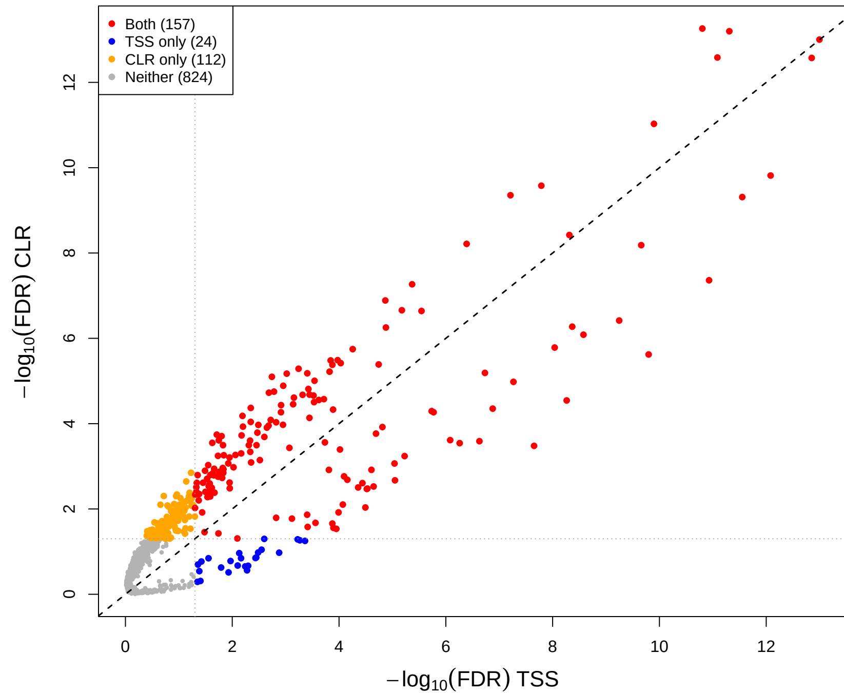
cent vs mage – CLR(const=-0.5) vs TSS (gamma = 0.3)
