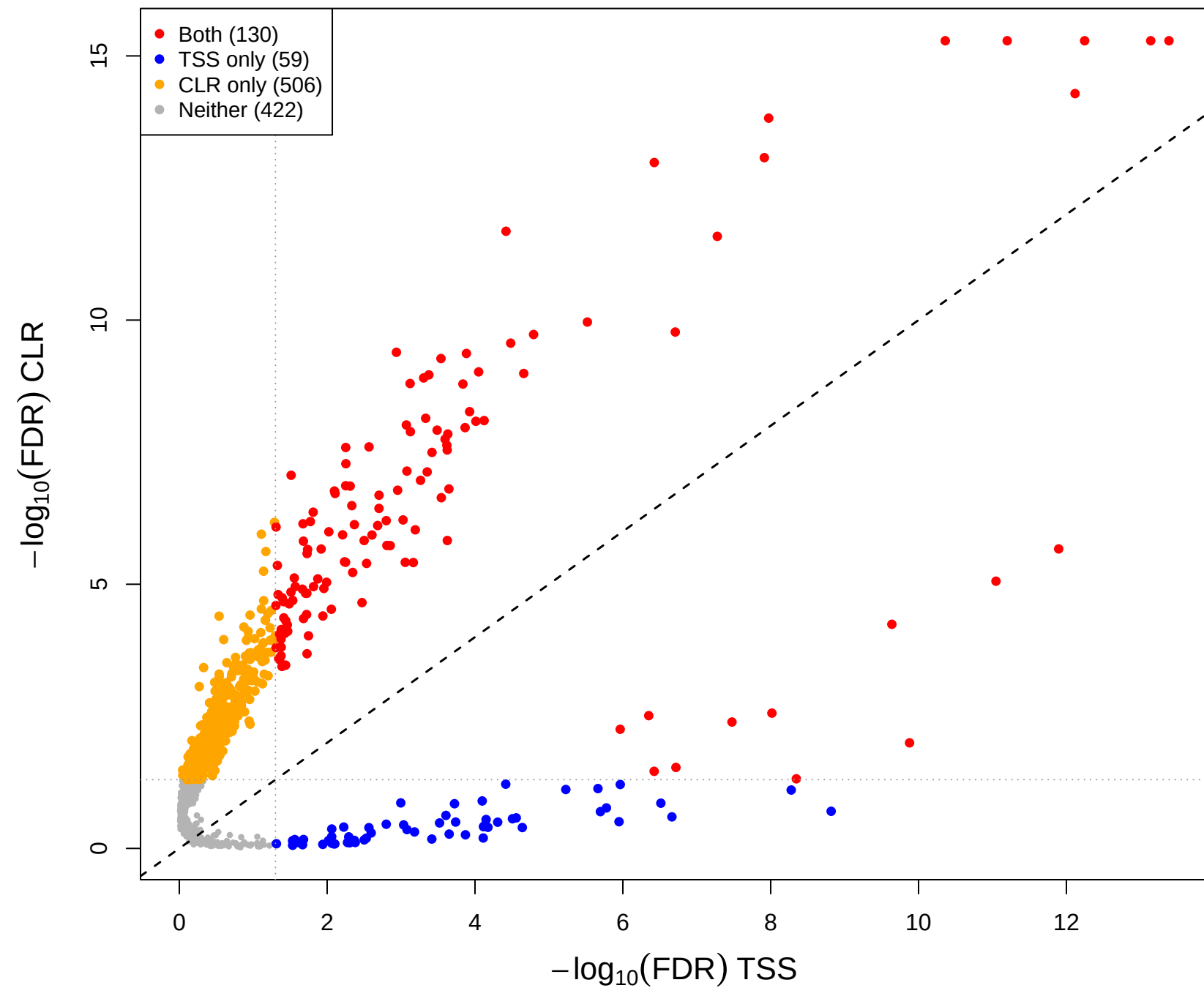
cent vs mage – CLR(const=-1) vs TSS (gamma = 0.3)
