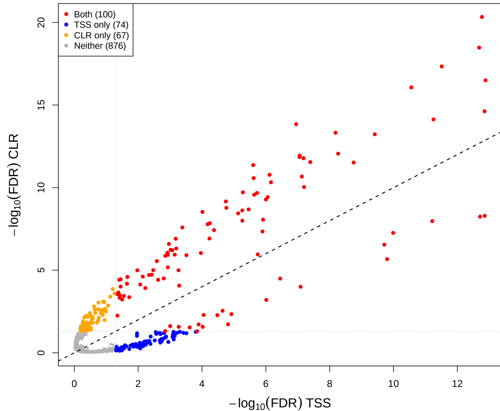
cent vs mage – CLR(const=0.8) vs TSS (gamma = 0.3)
