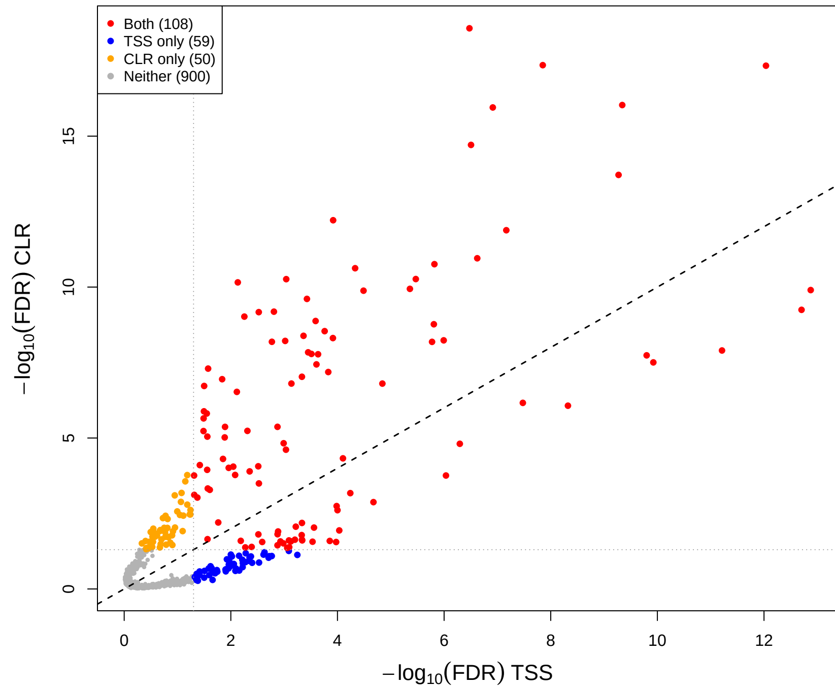
cent vs mage – CLR(const=0.6) vs TSS (gamma = 0.3)
