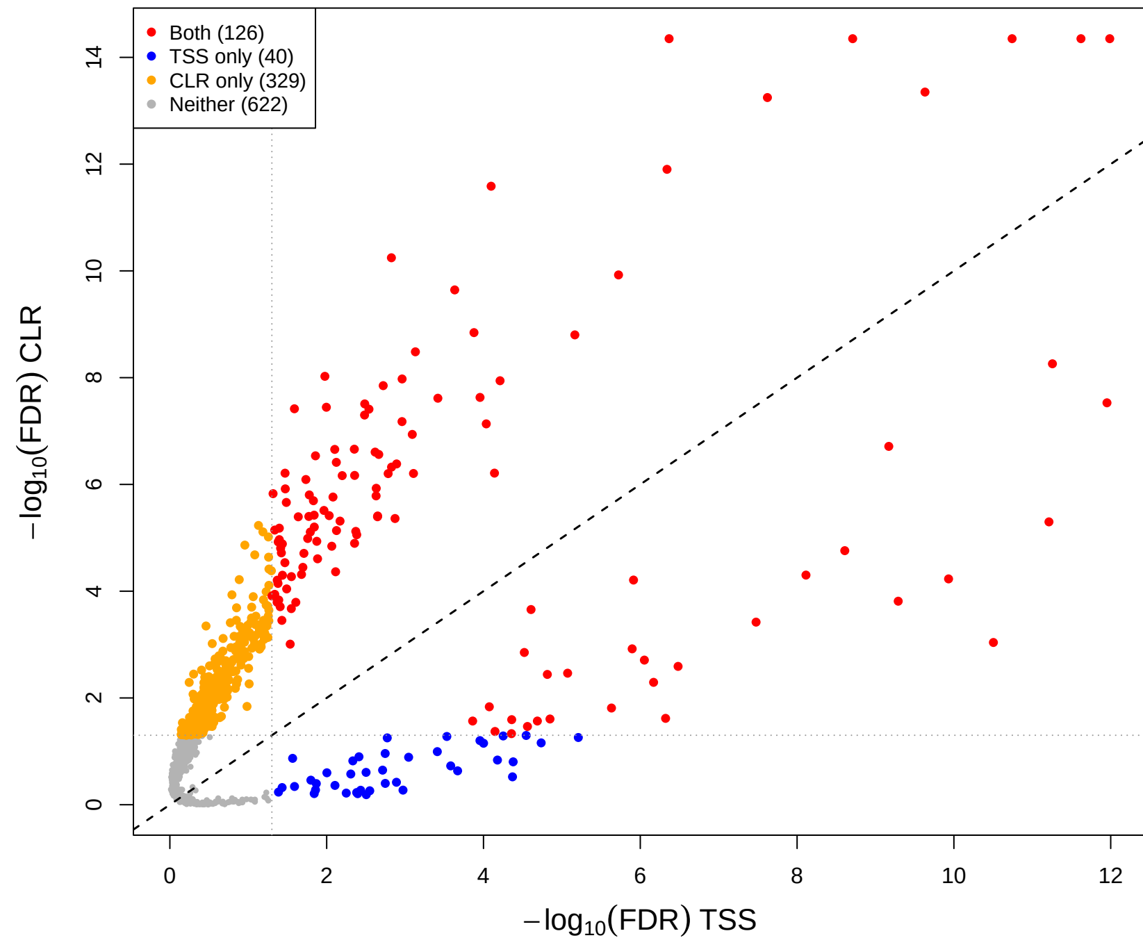
cent vs mage – CLR(const=-0.7) vs TSS (gamma = 0.3)
