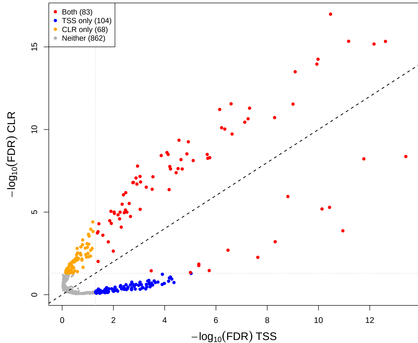
cent vs mage – CLR(const=0.9) vs TSS (gamma = 0.3)
