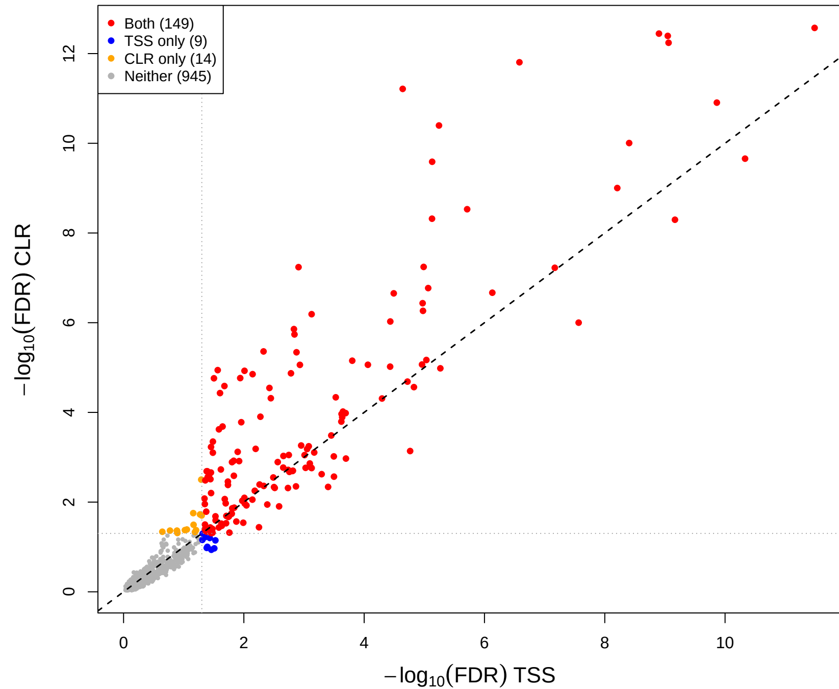
cent vs mage – CLR(const=0.1) vs TSS (gamma = 0.3)
