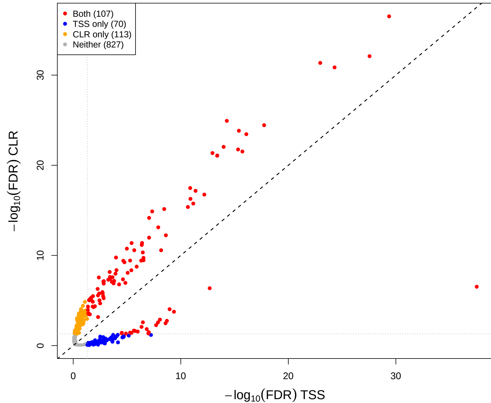
eld vs kin – CLR(const=1) vs TSS (gamma = 0.3)
