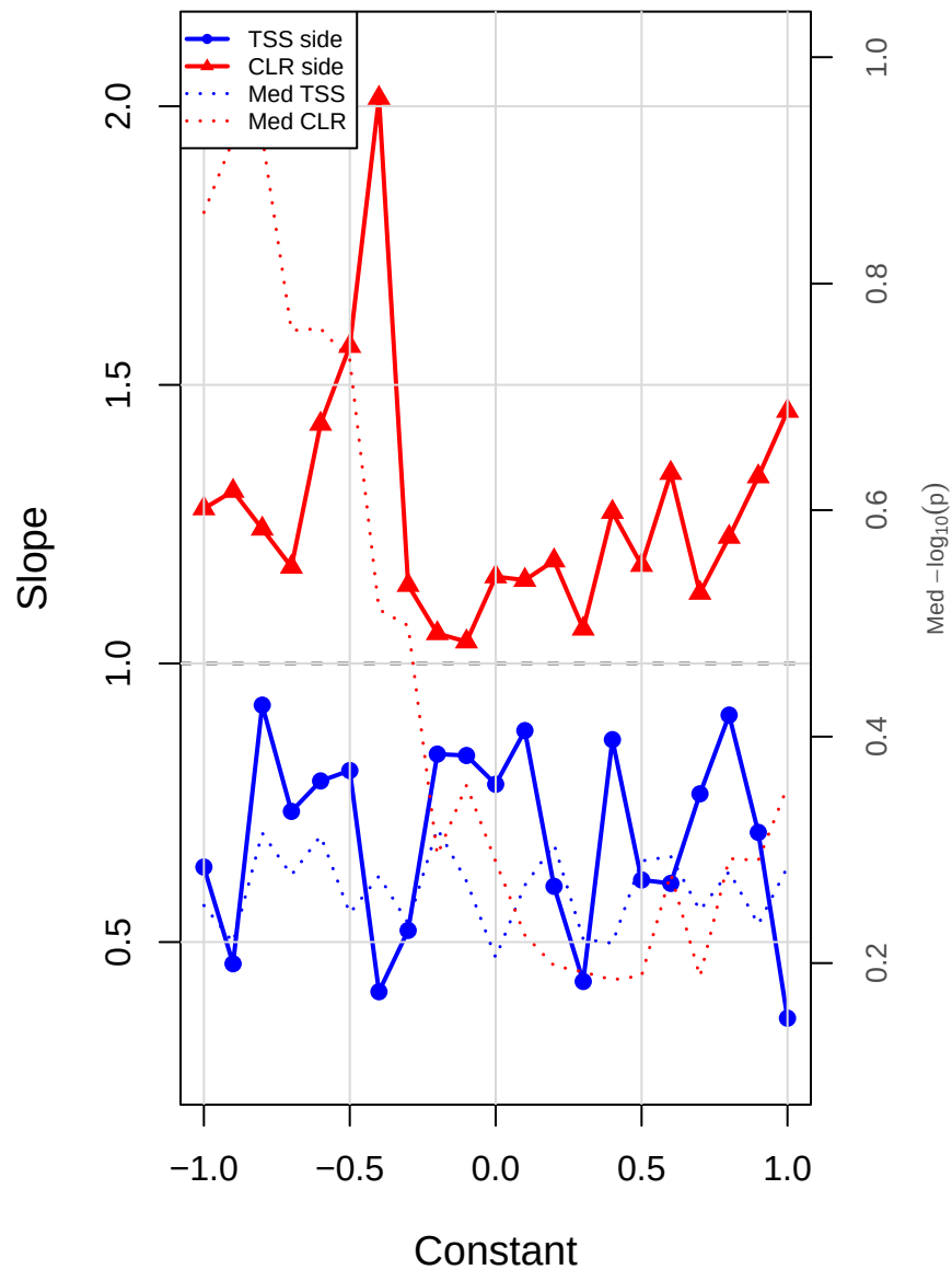
CLR_const | cent vs mage | gamma=0.5
