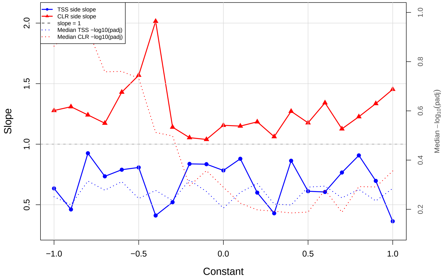
CLR_const | cent vs mage | gamma=0.5 Slope of red-dot regression
