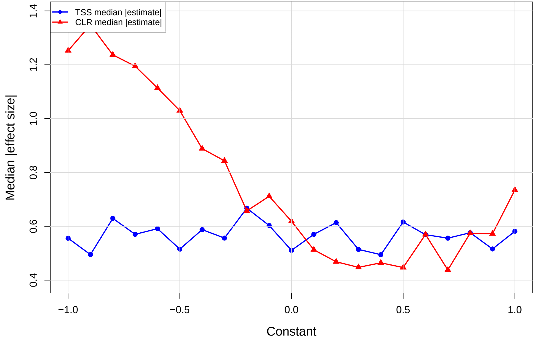
CLR_const | cent vs mage | gamma=0.5 Median absolute effect size across all features
