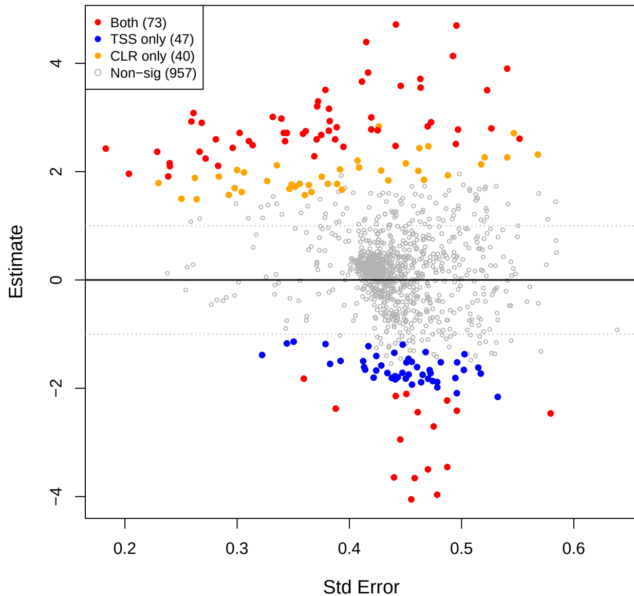
cent vs mage – CLR(const=0.7) effect space
