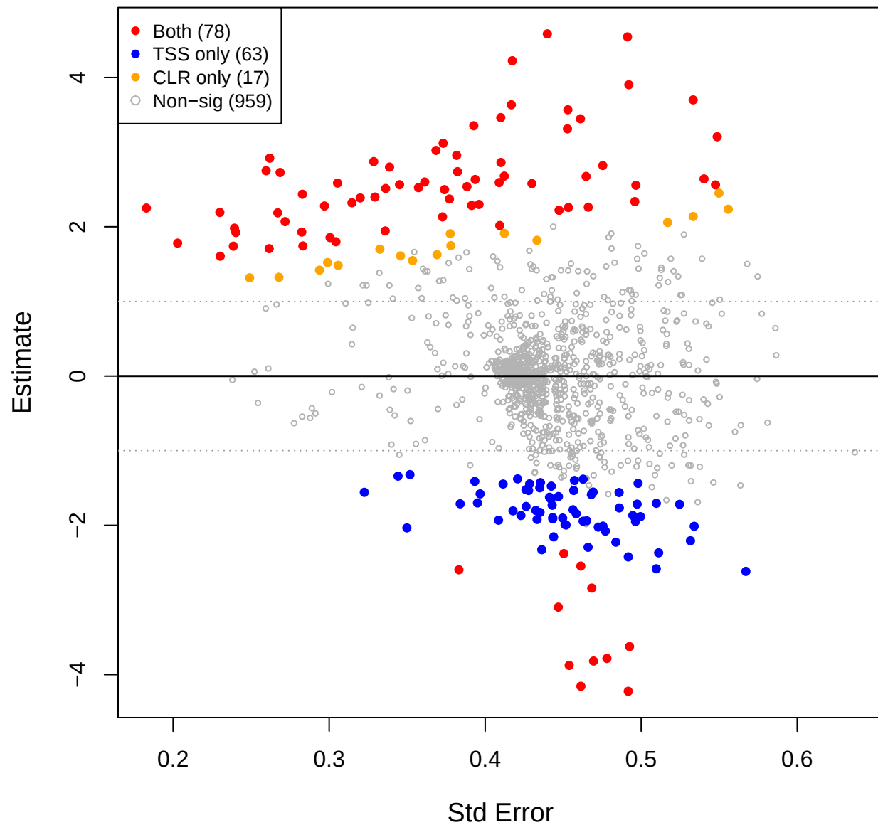
cent vs mage – CLR(const=0.3) effect space
