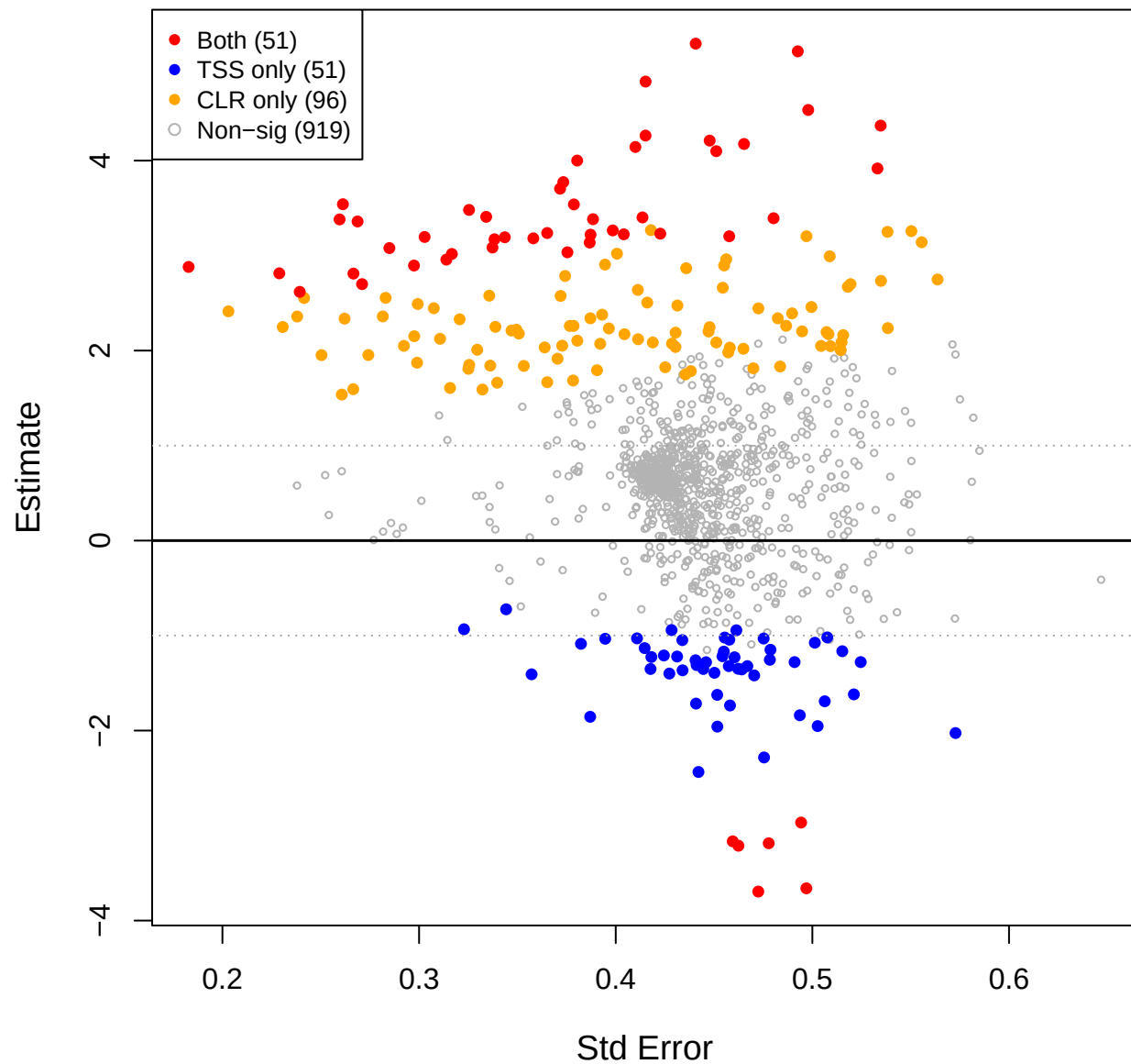
cent vs mage – CLR(const=1) effect space
