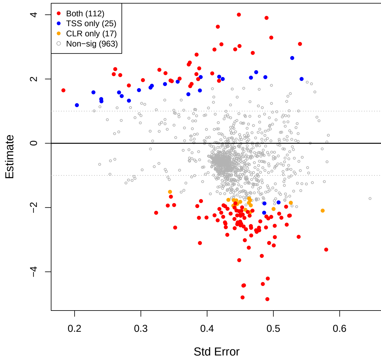
cent vs mage – CLR(const=-0.1) effect space
