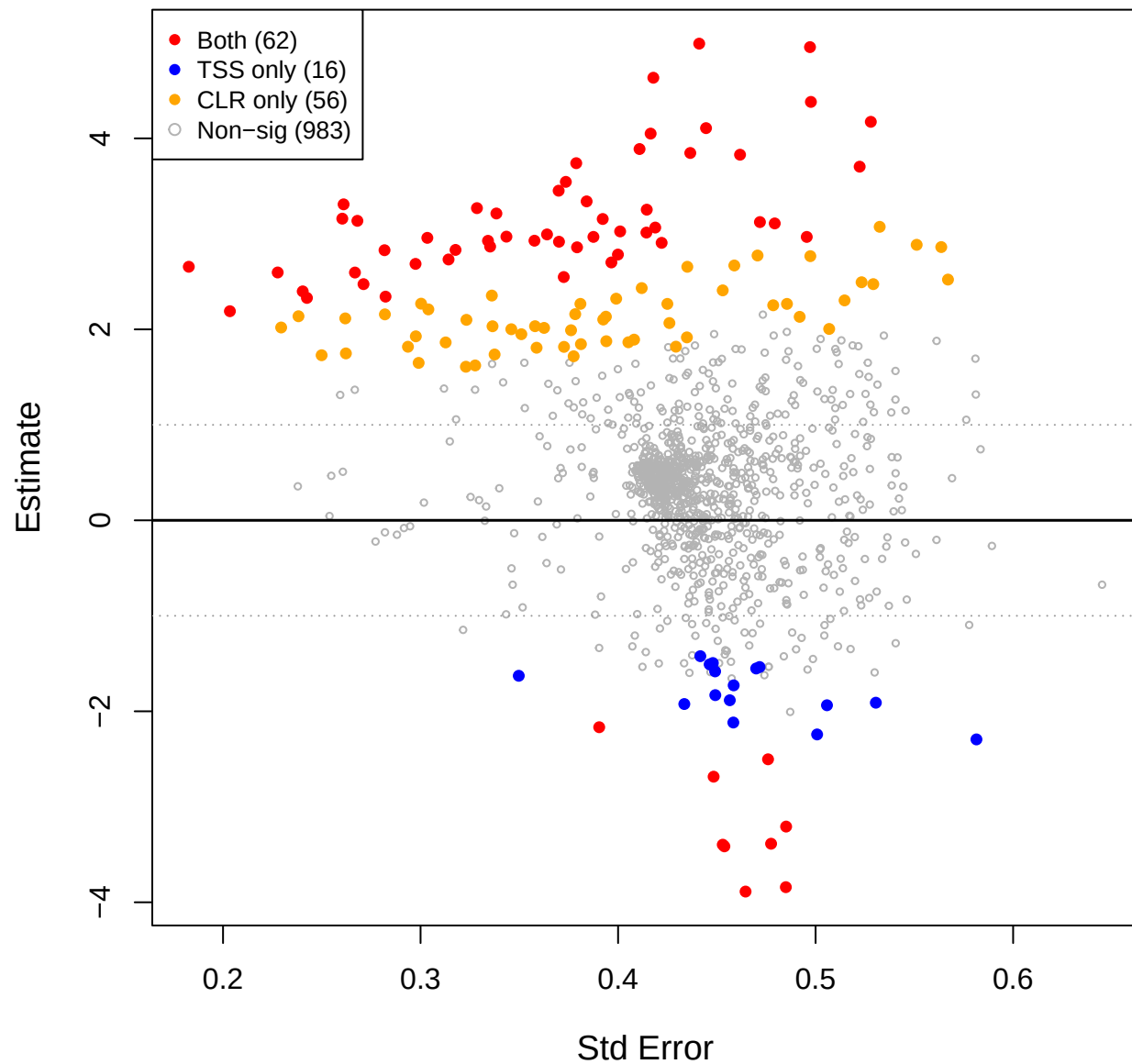
cent vs mage – CLR(const=0.6) effect space
