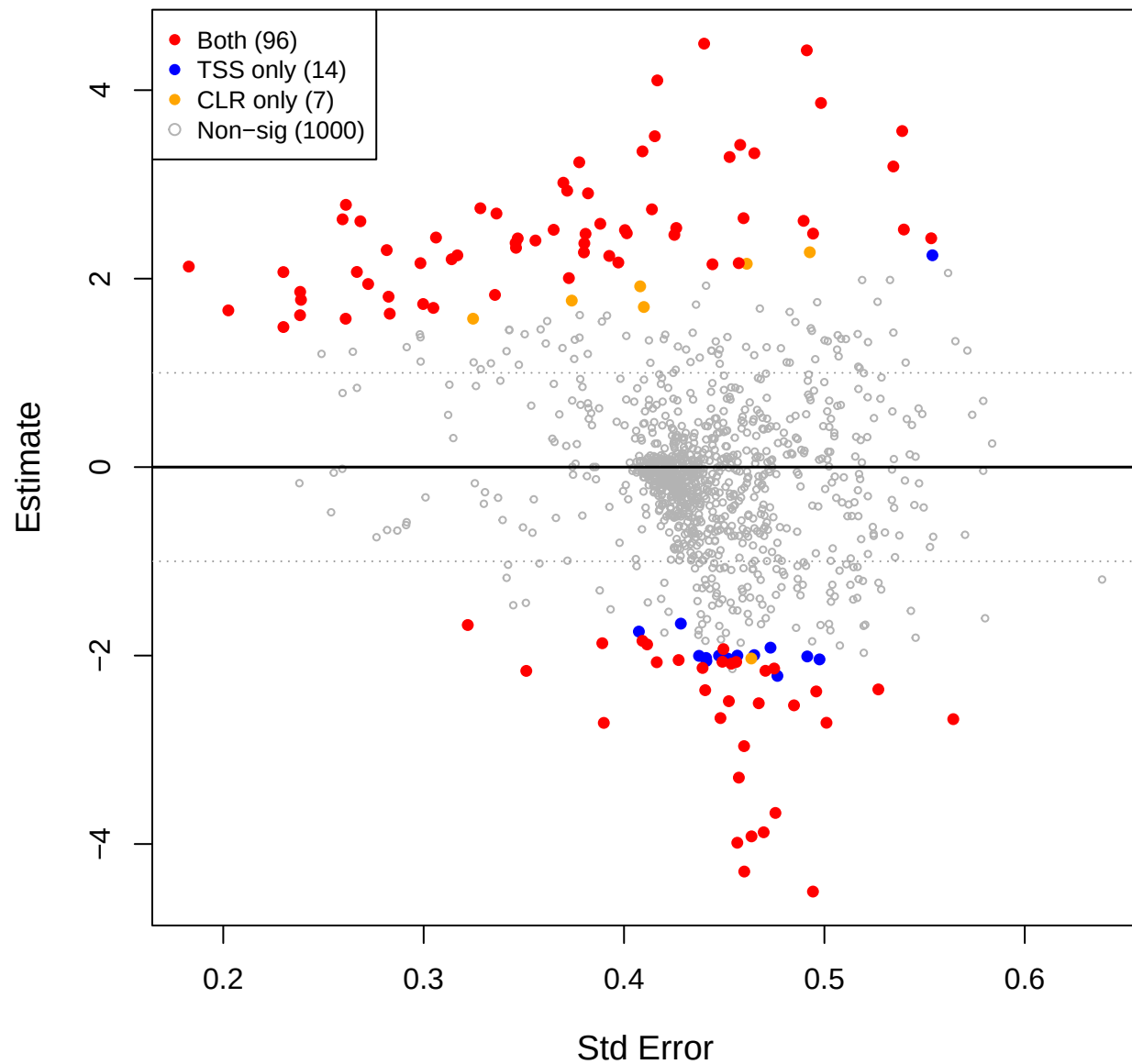
cent vs mage – CLR(const=0.4) effect space
