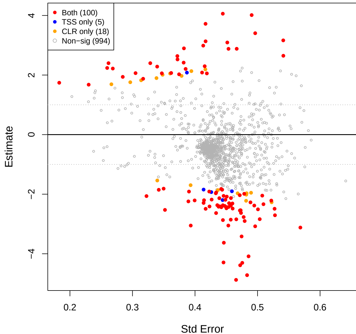
cent vs mage – CLR(const=-0.2) effect space
