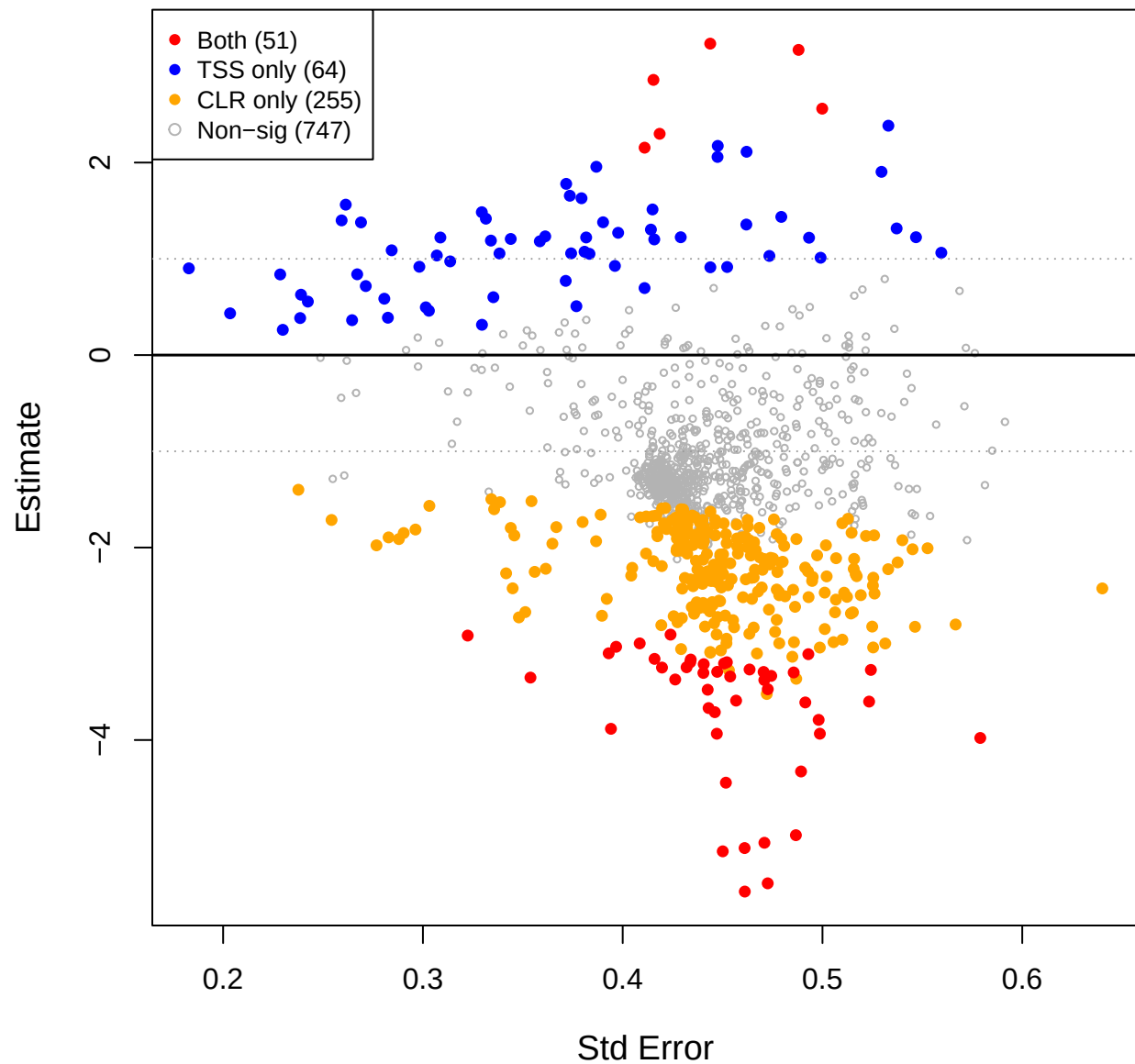
cent vs mage – CLR(const=-0.9) effect space
