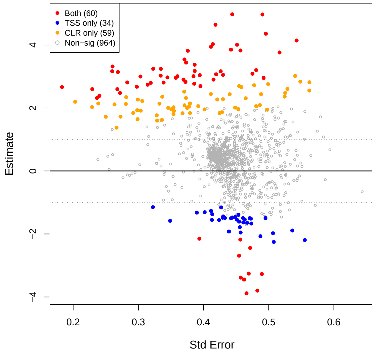
cent vs mage – CLR(const=0.8) effect space
