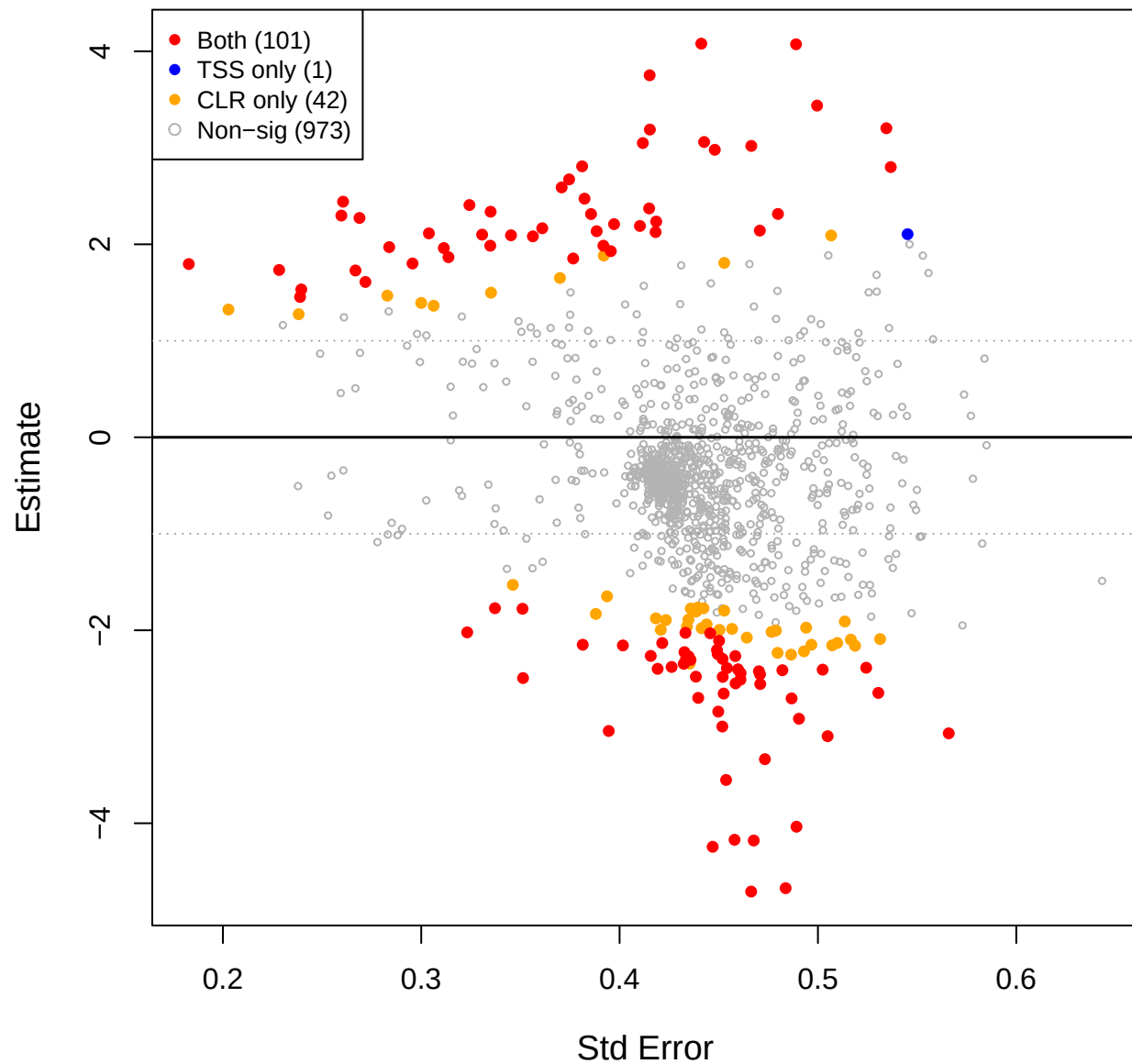
cent vs mage – CLR(const=0) effect space
