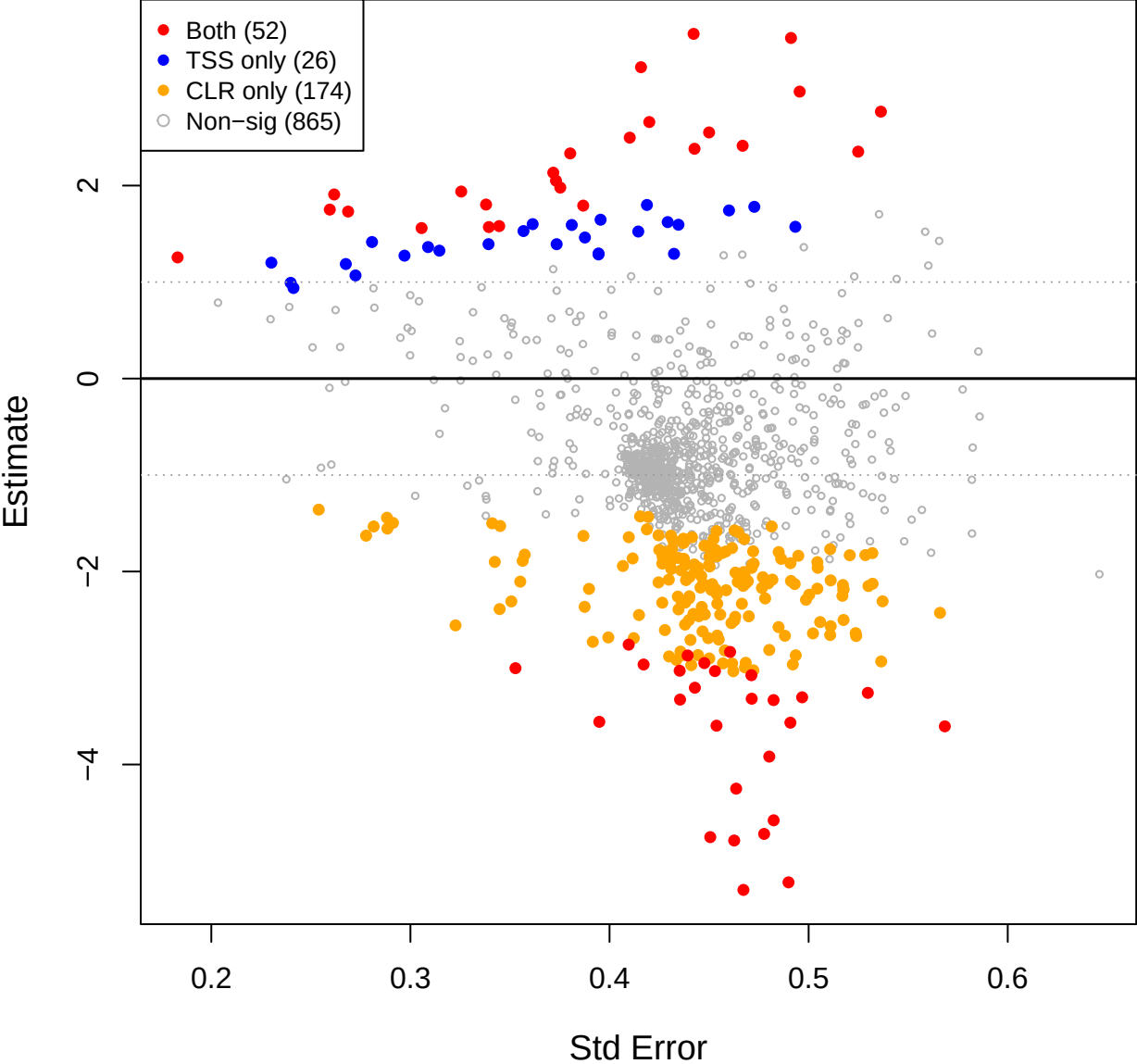
cent vs mage – CLR(const=-0.5) effect space
