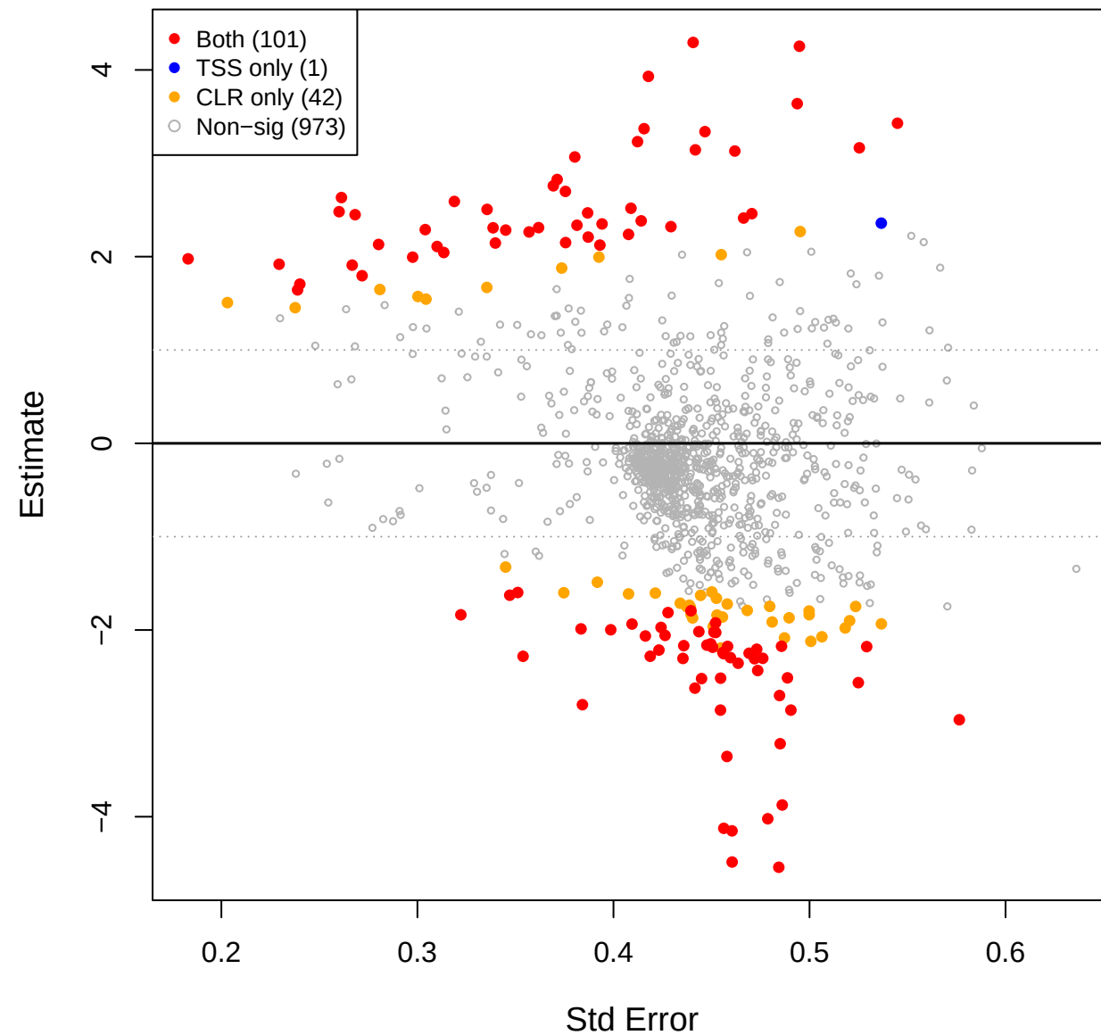
cent vs mage – TSS effect space
