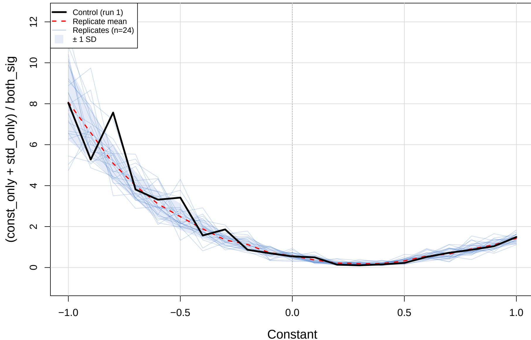
CLR(const) vs CLR(std) – cent_vs_mage (gamma=0.3) Robustness ratio
