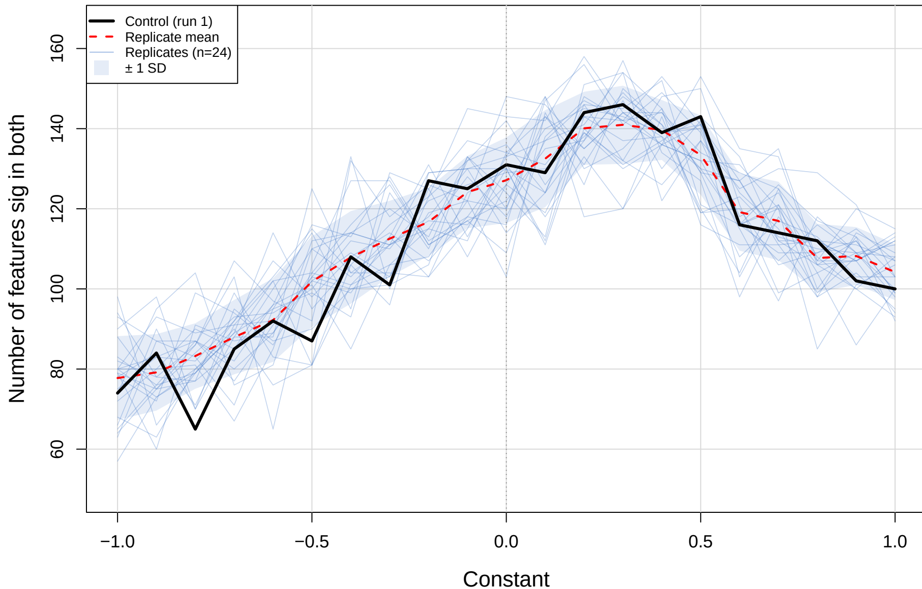
CLR(const) vs CLR(std) – cent_vs_mage (gamma=0.3) Both-significant count
