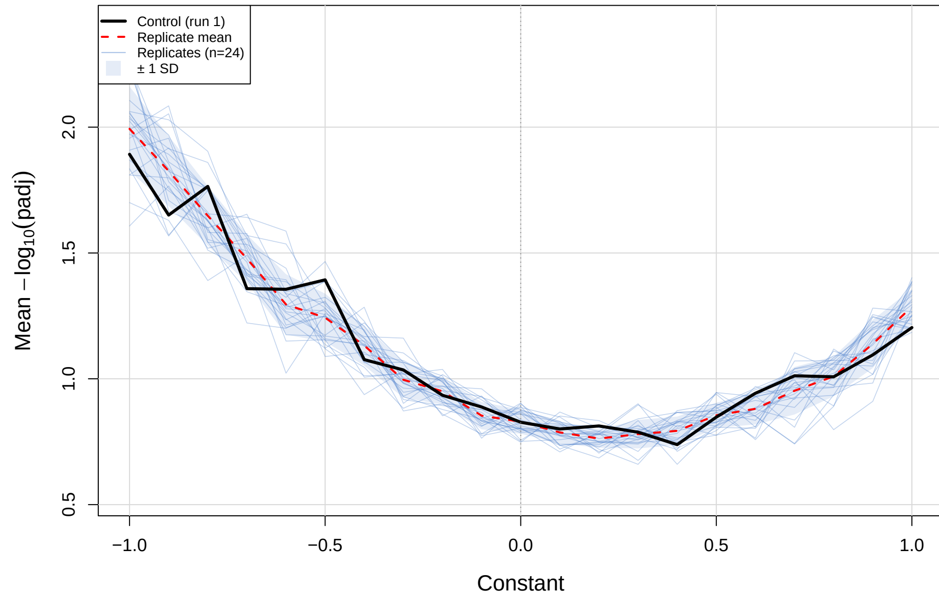
CLR(const) vs CLR(std) - cent_vs_mage (gamma=0.3) Mean -\log_{10}(\text{padj}) CLR(const)
