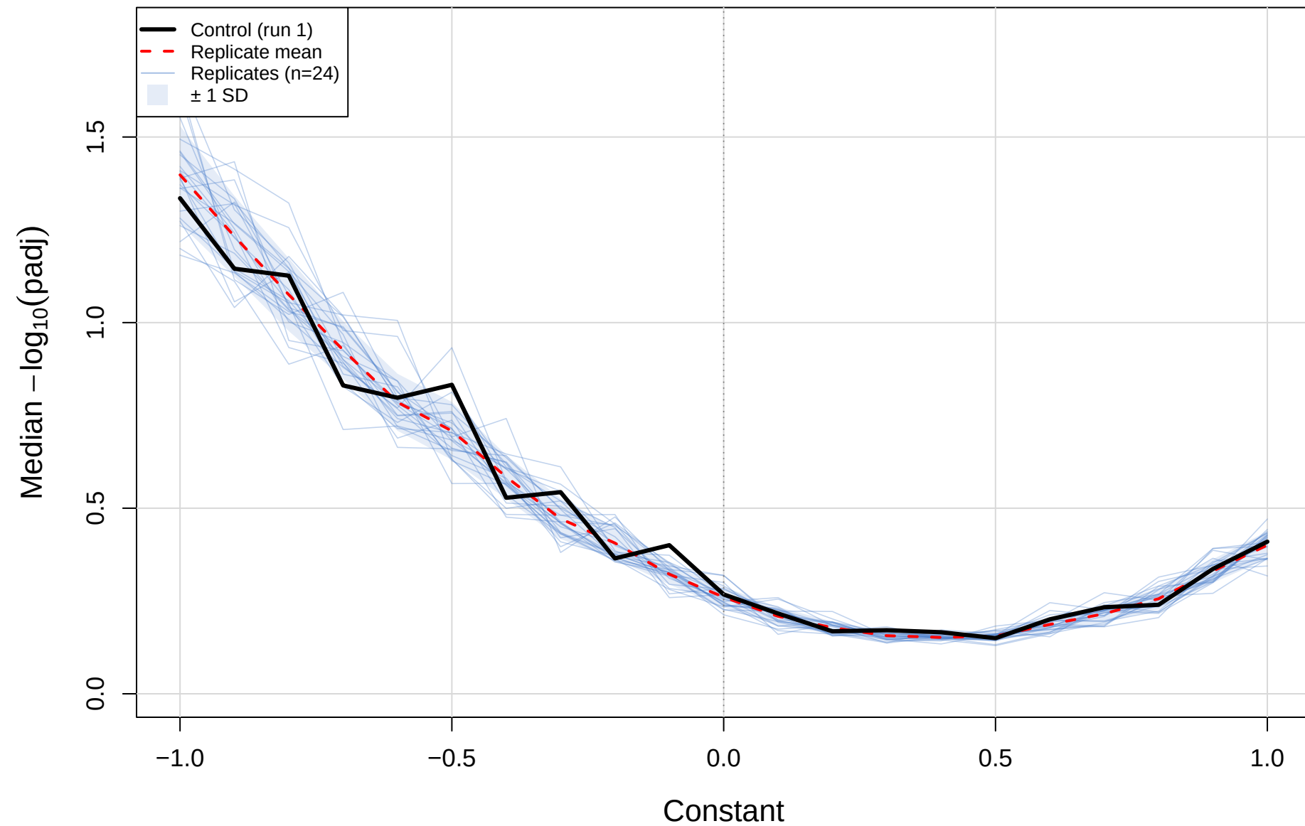
CLR(const) vs CLR(std) – cent_vs_mage (gamma=0.3) Median -\log_{10}(\text{padj}) CLR(const)
