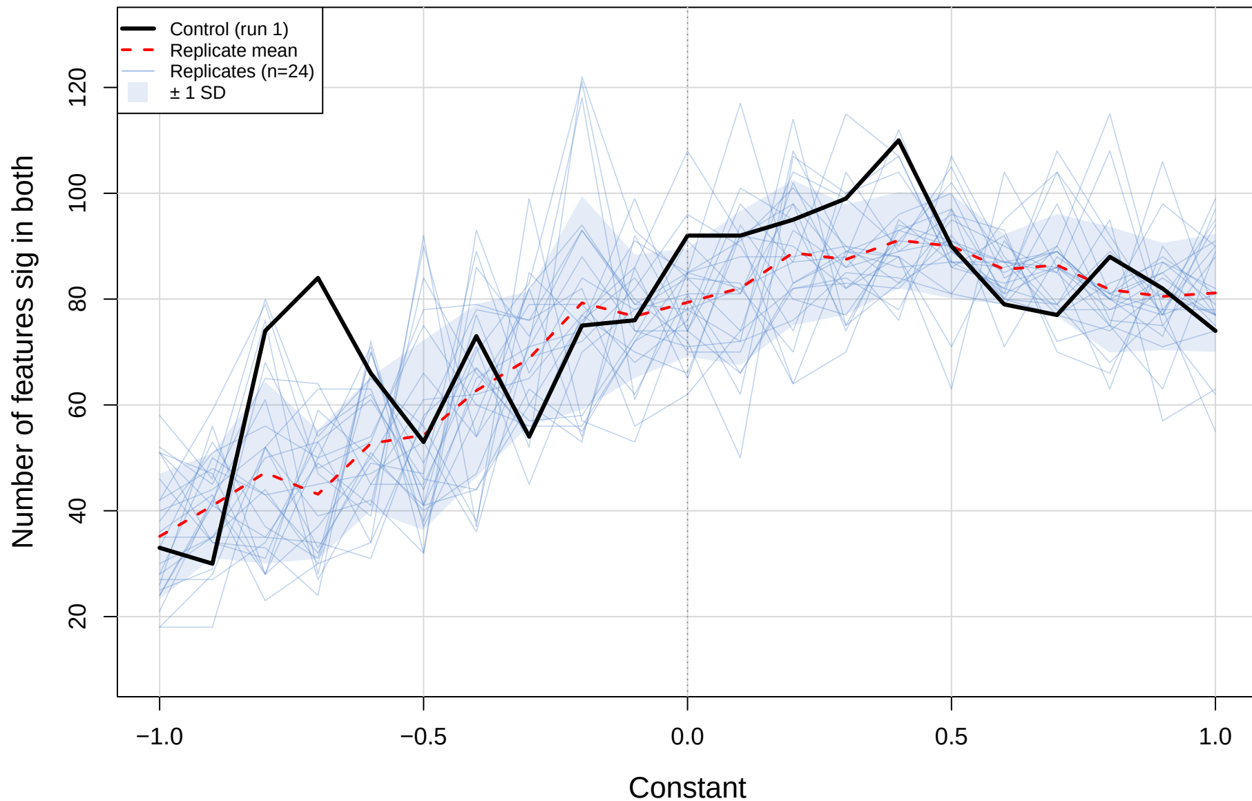
CLR(const) vs CLR(std) – cent_vs_mage (gamma=0.5) Both-significant count
