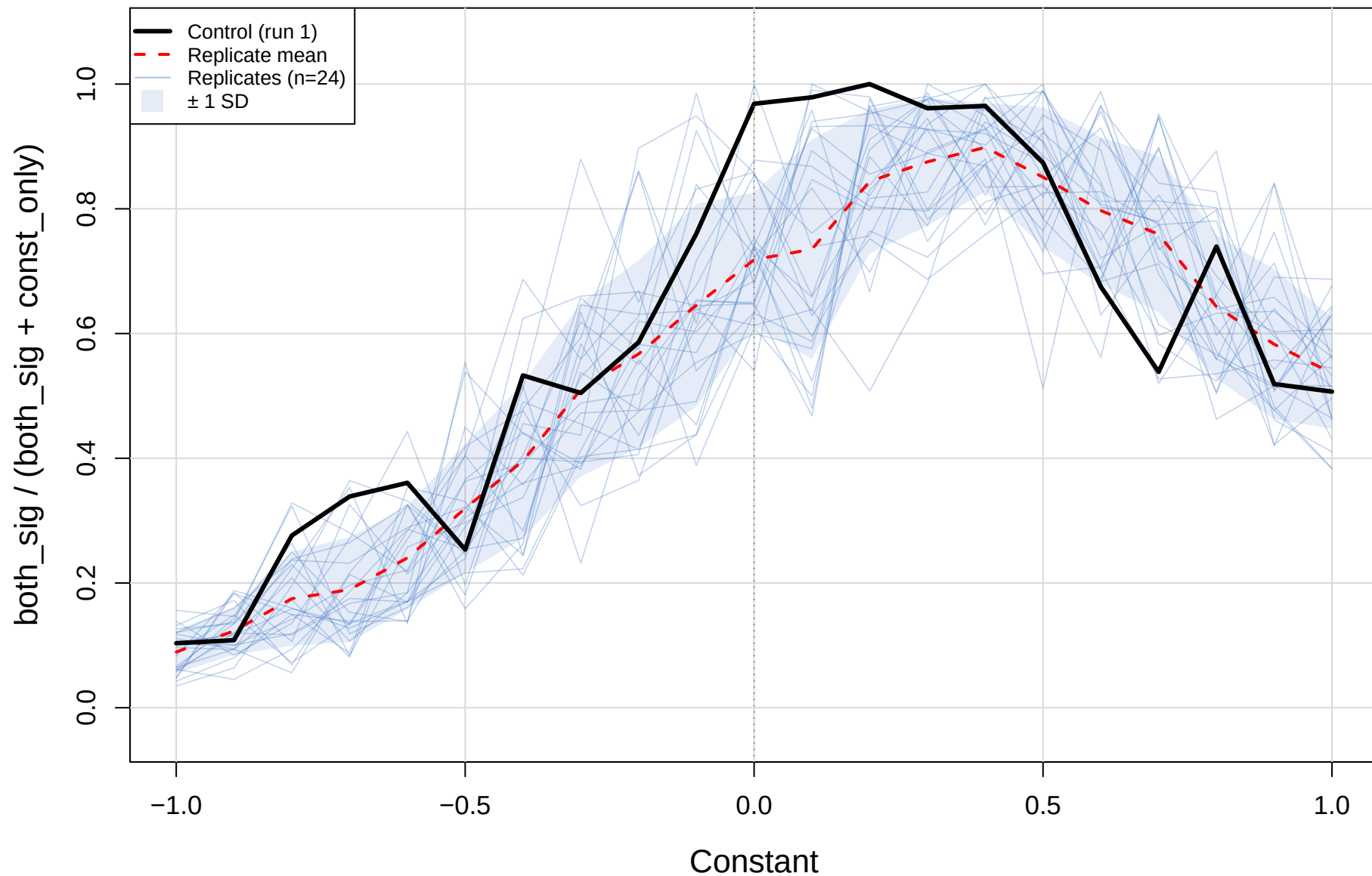
CLR(const) vs CLR(std) – cent_vs_mage (gamma=0.5) Robustness ratio
