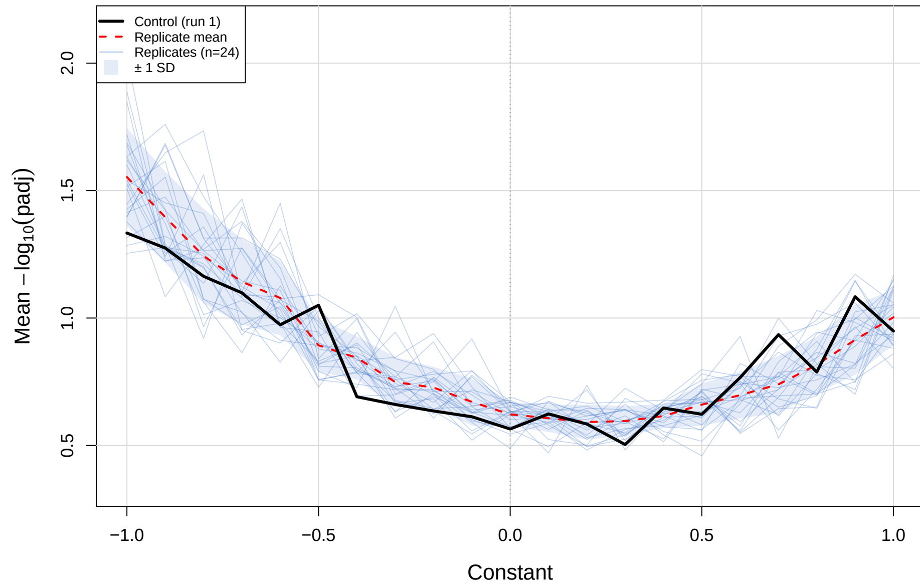
CLR(const) vs CLR(std) – cent_vs_mage (gamma=0.5) Mean -\log_{10}(\text{padj}) CLR(const)
