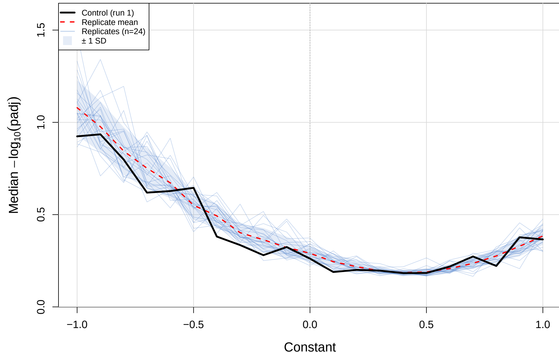
CLR(const) vs CLR(std) – cent_vs_mage (gamma=0.5) Median -\log_{10}(\text{padj}) CLR(const)
