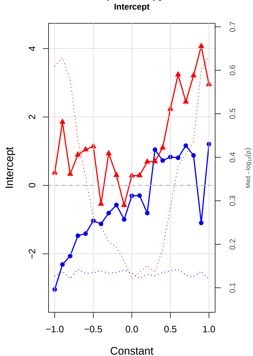
CLR_const | eld vs kin | gamma=0.3
