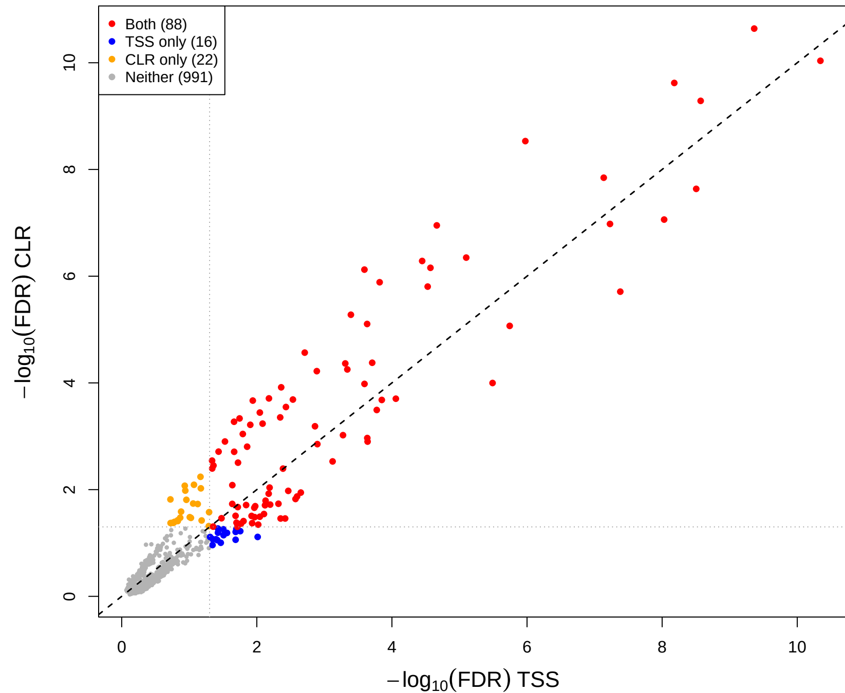
cent vs mage – CLR(const=0.1) vs TSS (gamma = 0.5)
