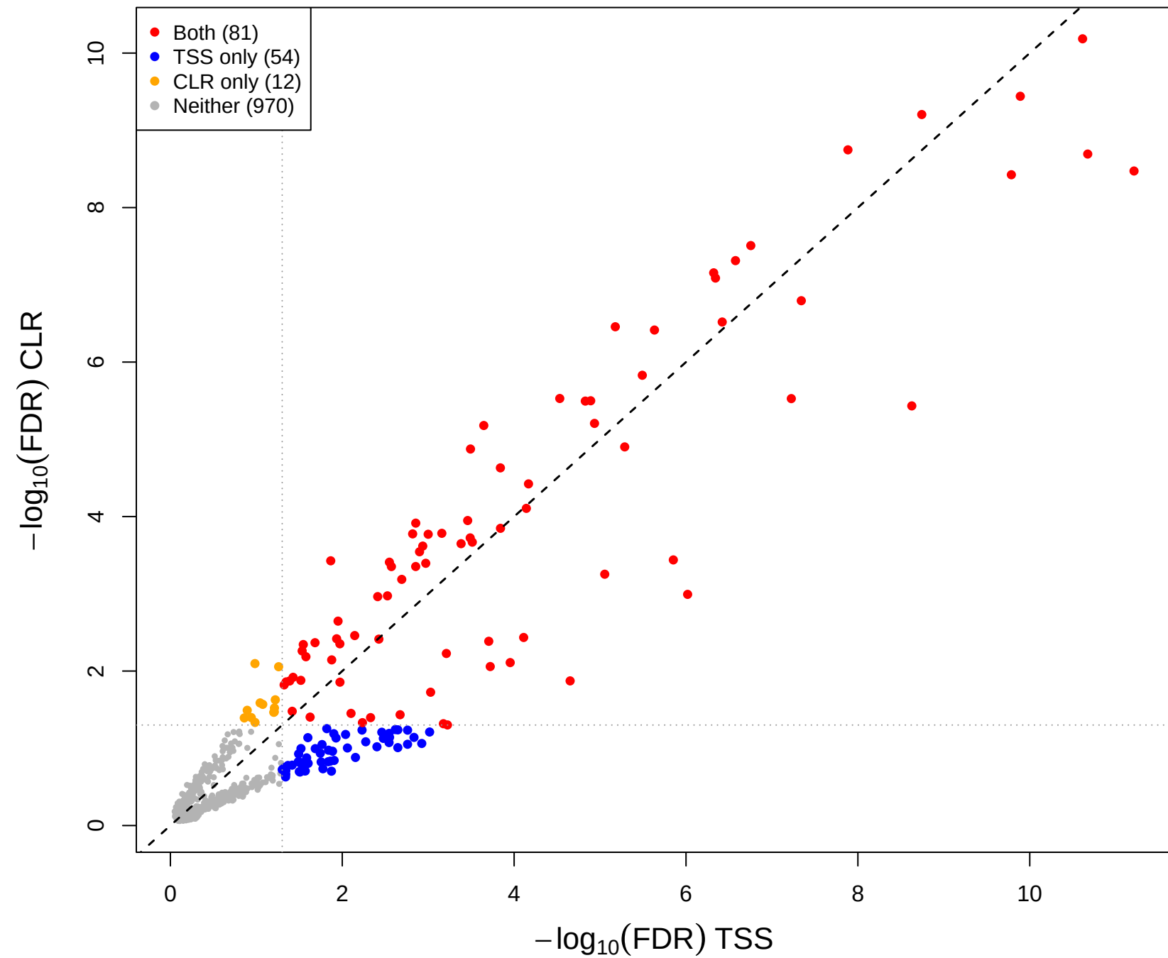
cent vs mage – CLR(const=0.3) vs TSS (gamma = 0.5)
