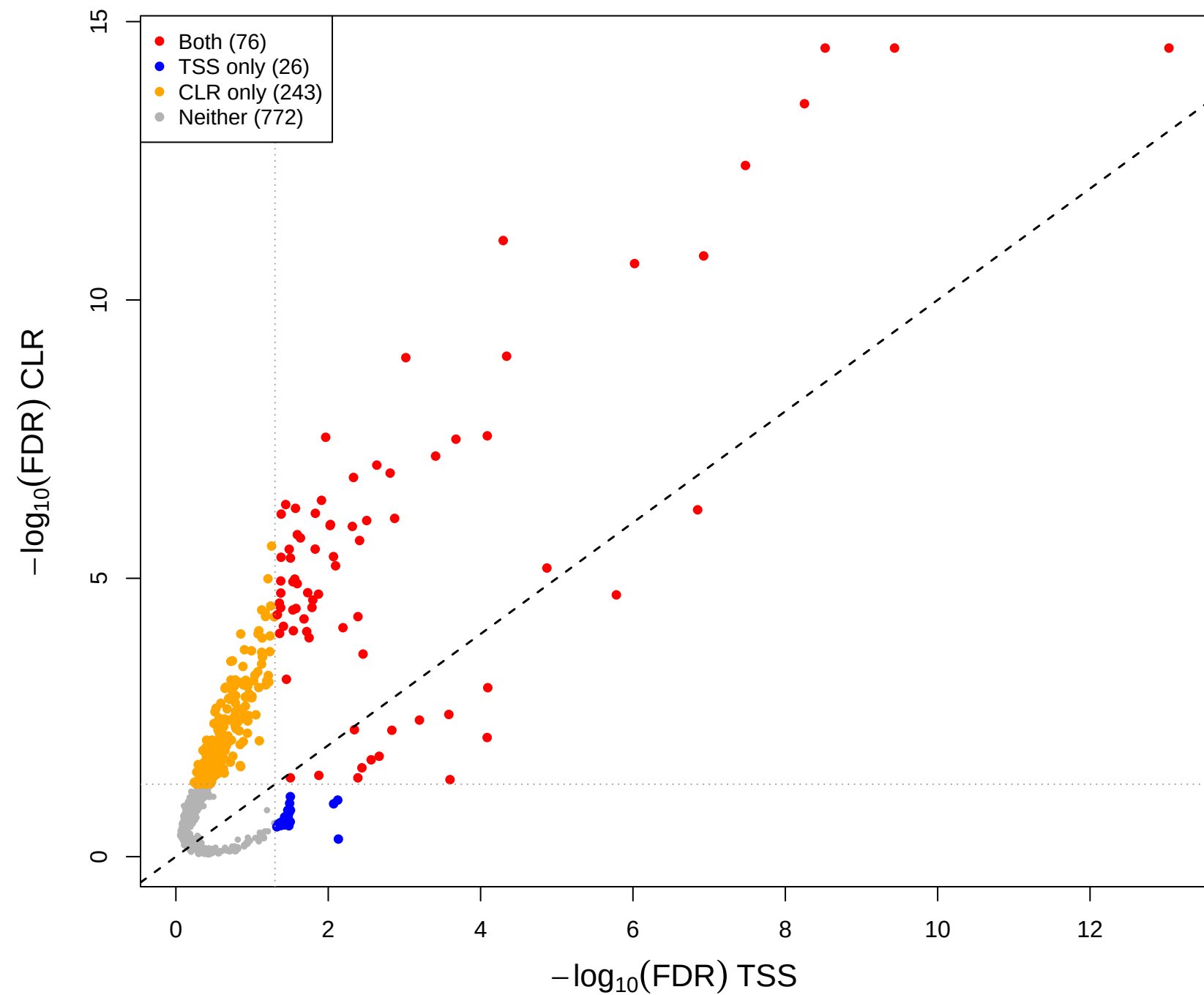
cent vs mage – CLR(const=-0.7) vs TSS (gamma = 0.5)
