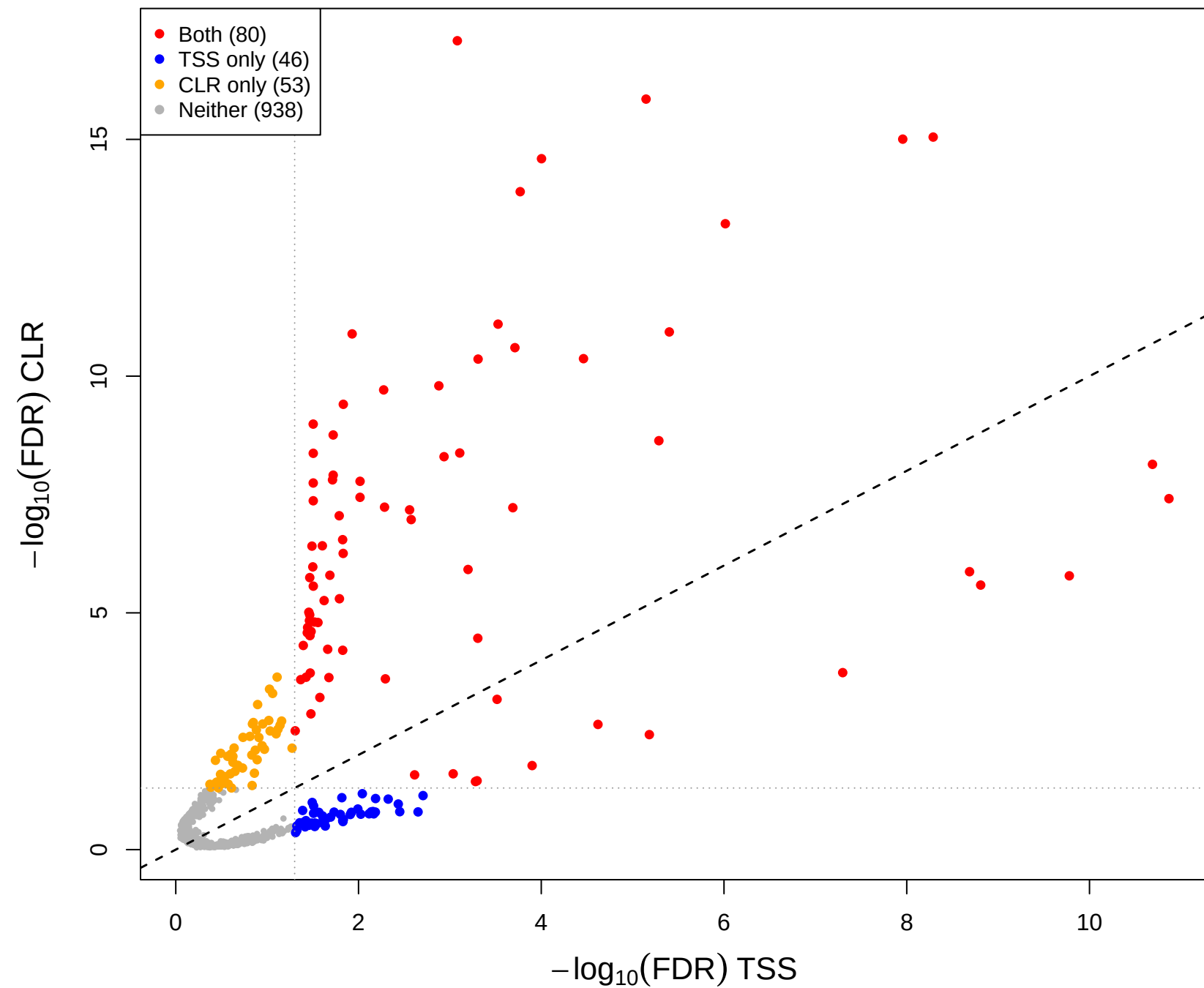
cent vs mage – CLR(const=0.6) vs TSS (gamma = 0.5)
