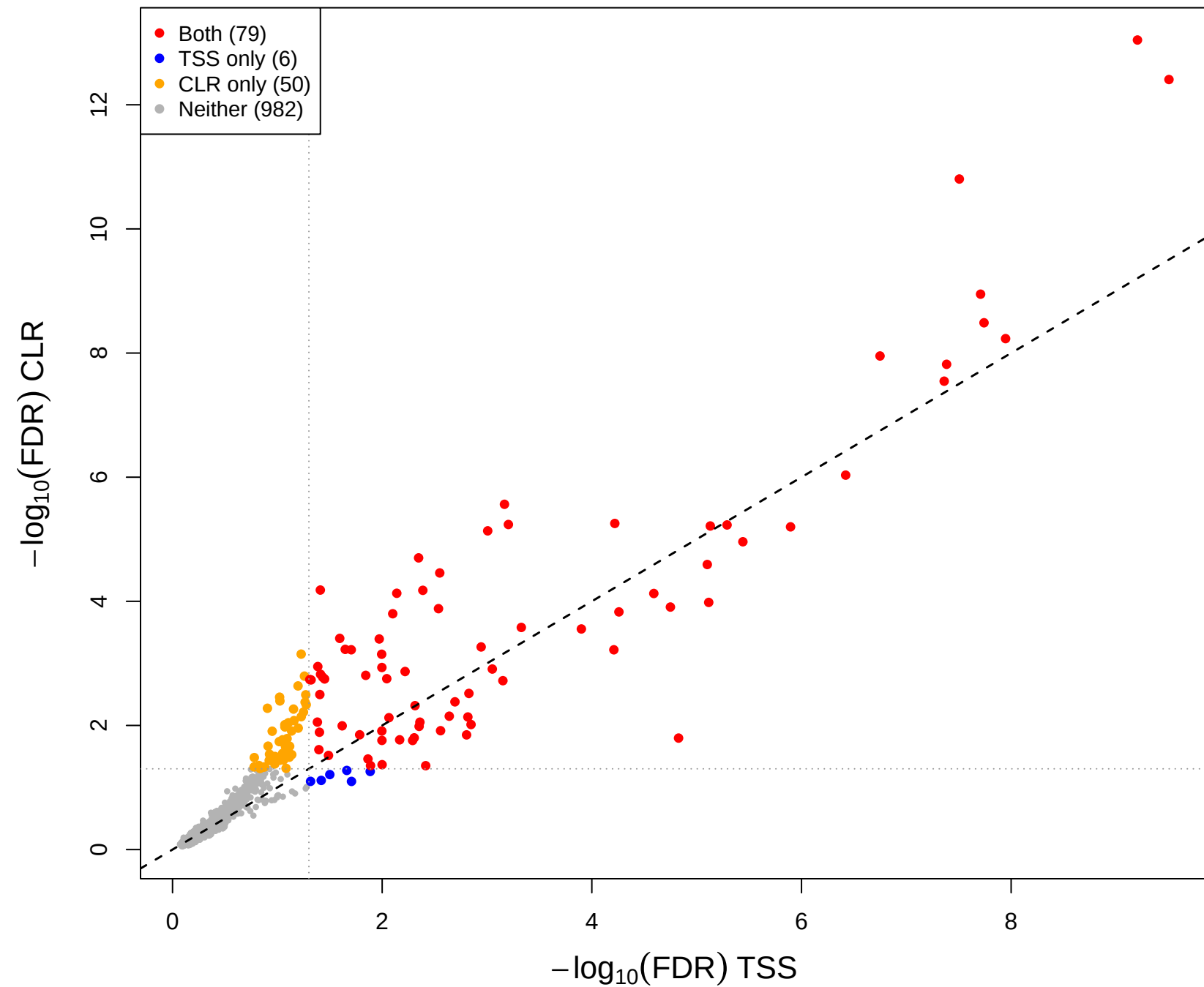
cent vs mage – CLR(const=0) vs TSS (gamma = 0.5)
