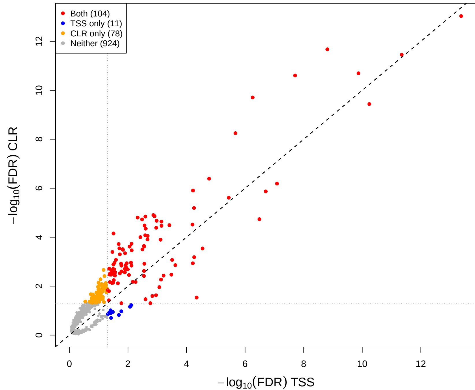
cent vs mage – CLR(const=-0.5) vs TSS (gamma = 0.5)
