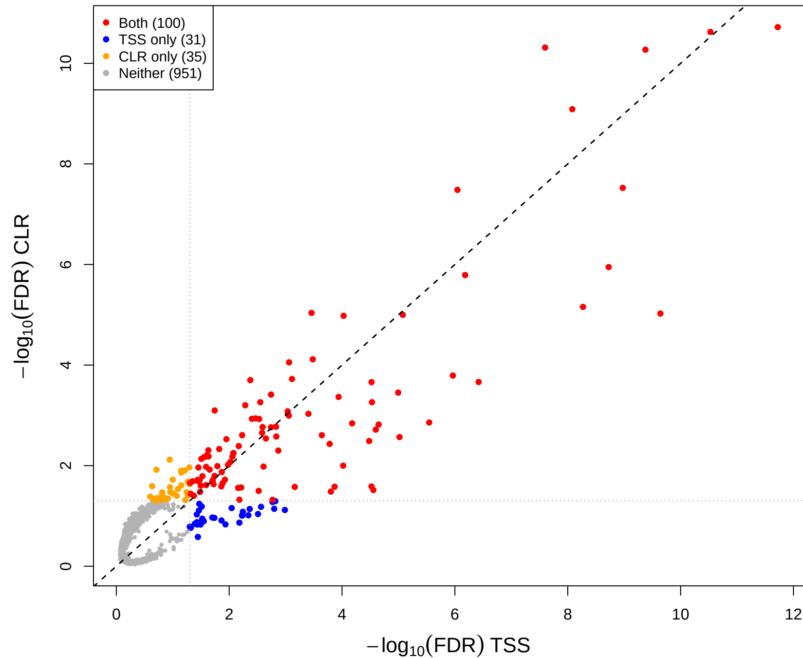
cent vs mage – CLR(const=-0.4) vs TSS (gamma = 0.5)
