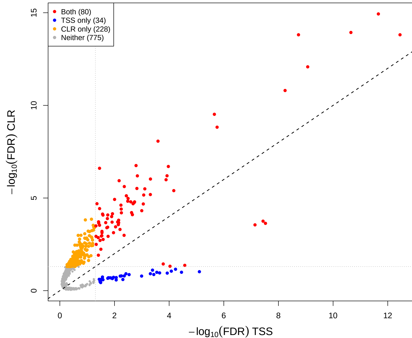
cent vs mage – CLR(const=-1) vs TSS (gamma = 0.5)
