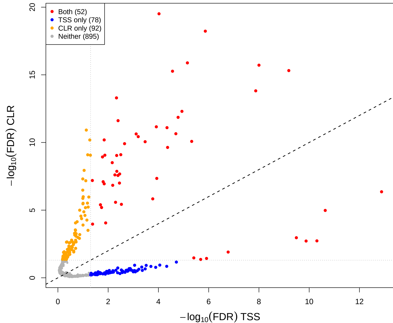
cent vs mage – CLR(const=0.9) vs TSS (gamma = 0.5)
