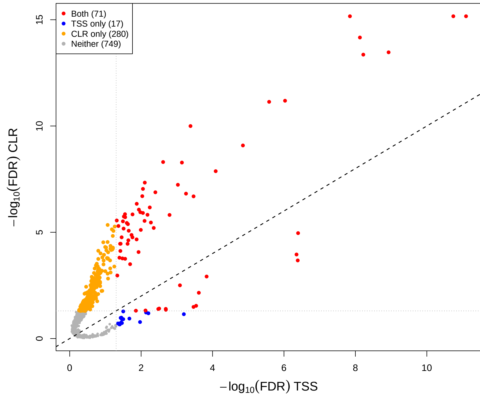
cent vs mage – CLR(const=-0.8) vs TSS (gamma = 0.5)
