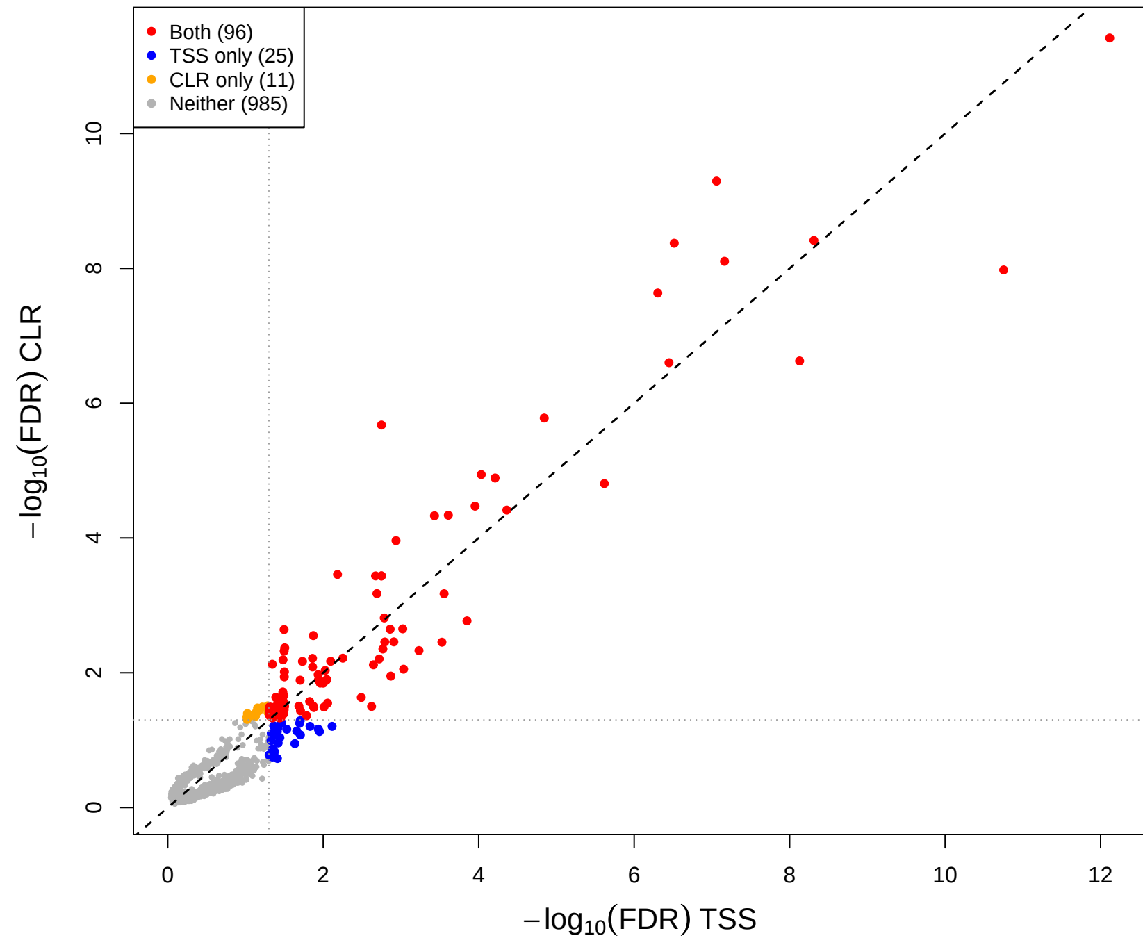
cent vs mage – CLR(const=0.2) vs TSS (gamma = 0.5)
