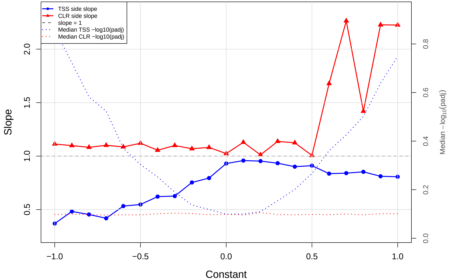
TSS_const | eld vs kin | gamma=0.1 Slope of red-dot regression
