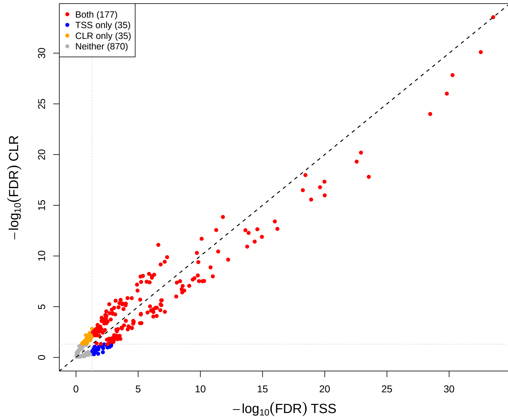
eld vs kin – CLR vs TSS(const=0.4) (gamma = 0.1)
